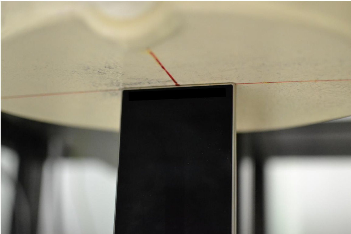
SAR Test Setup Photo 10 – Phablet, Bottom Edge at 0mm
