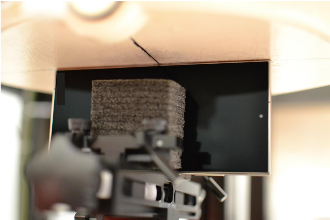
SAR Test Setup Photo 16 – Phablet, Left Edge at 0mm
