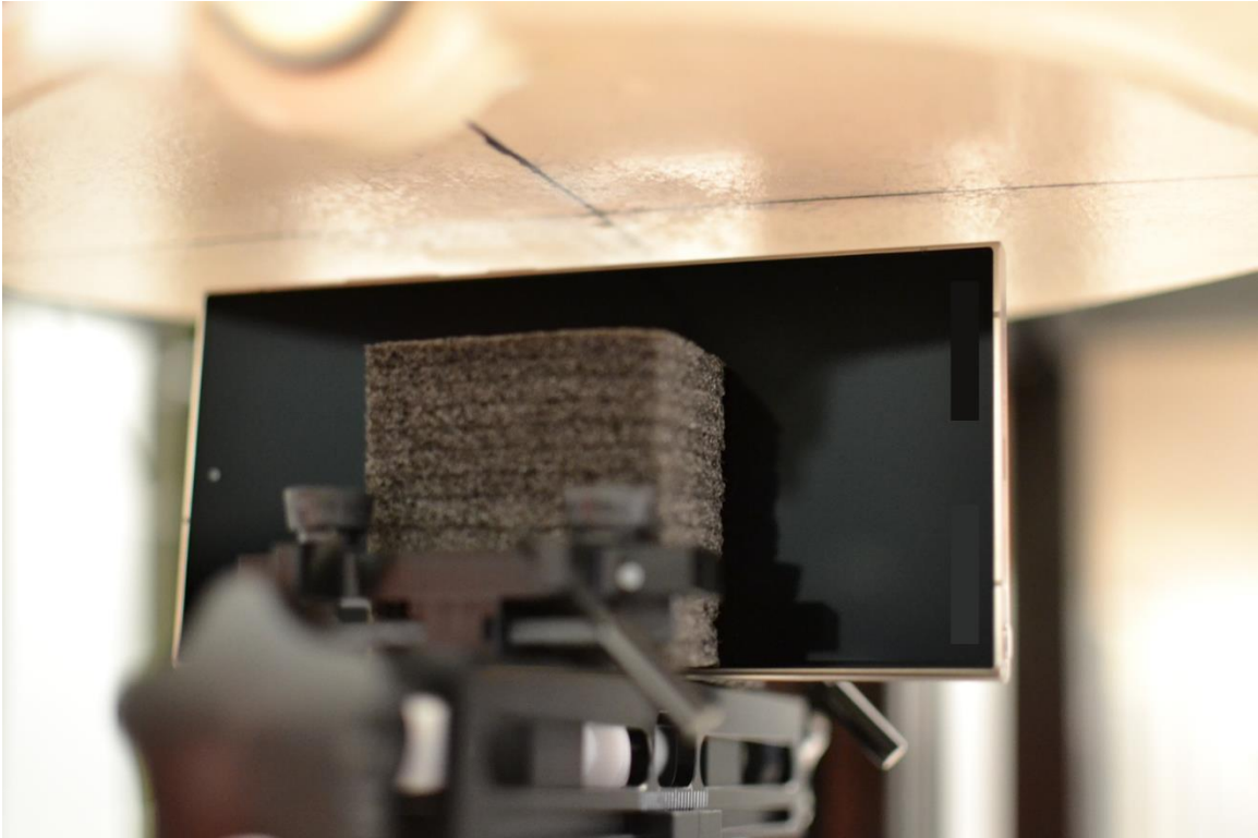
SAR Test Setup Photo 13 – Hotspot, Right Edge at 10mm
