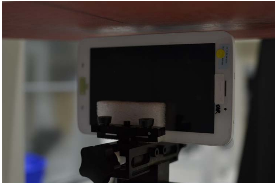
SAR Test Setup Photo 10: Left Edge at 0.4 cm
