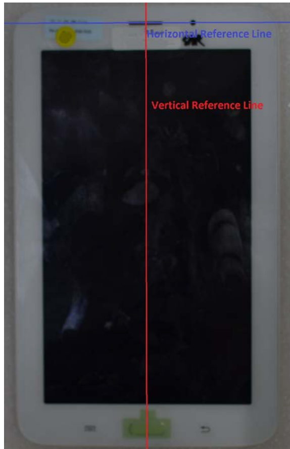
SAR Test Setup Photo 12: Vertical and Horizontal Reference Lines
