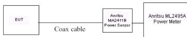
Figure 6-1 Power Measurement Setup
