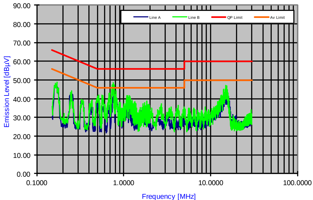
Plot 6-62. Line Conducted Plot with 802.11a
