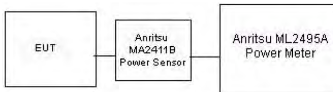
Figure 8-2 Power Measurement Setup
