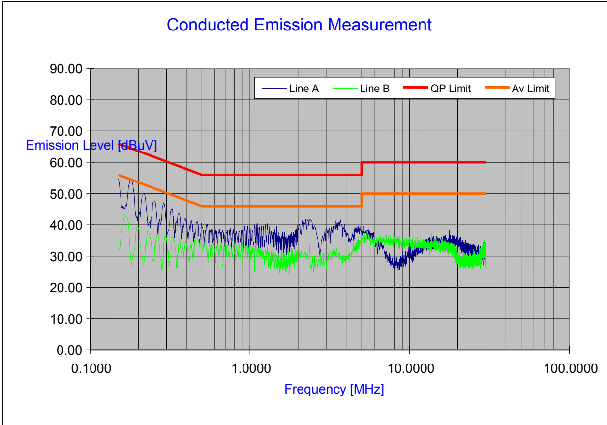
Plot 6-44. Line Conducted Plot with Bluetooth
