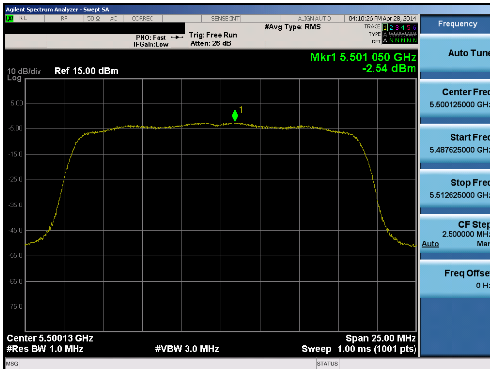
Plot 6-49. Peak Power Spectral Density Plot (20MHz BW 802.11n (UNII Band 2C) – Ch. 100)
