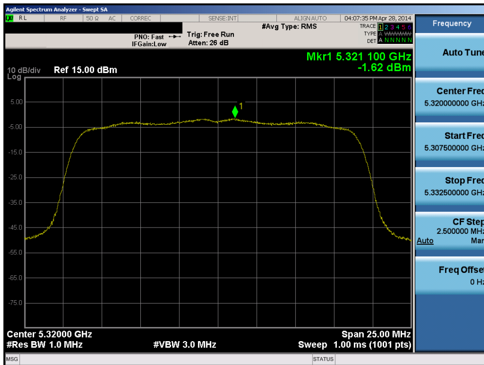
Plot 6-43. Peak Power Spectral Density Plot (20MHz BW 802.11n (UNII Band 2A) – Ch. 64)
