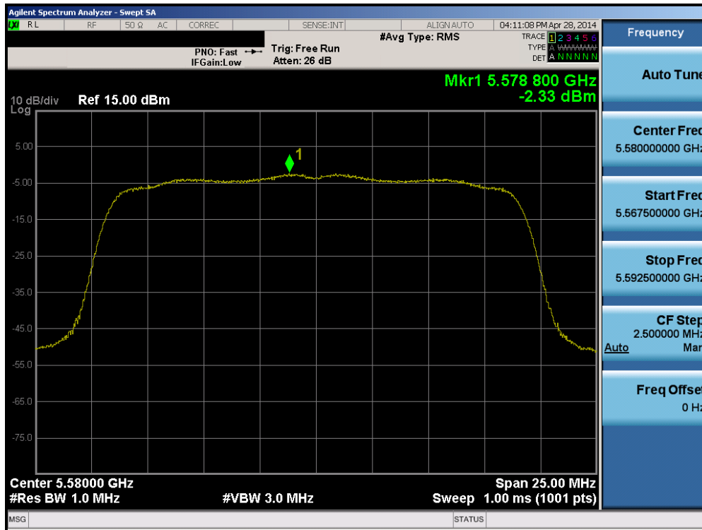
Plot 6-50. Peak Power Spectral Density Plot (20MHz BW 802.11n (UNII Band 2C) – Ch. 116)
