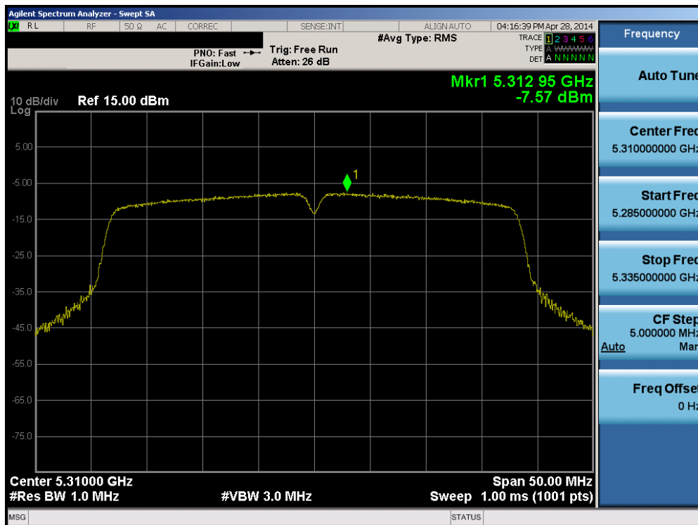
Plot 6-45. Peak Power Spectral Density Plot (40MHz BW 802.11n (UNII Band 2A) – Ch. 62)
