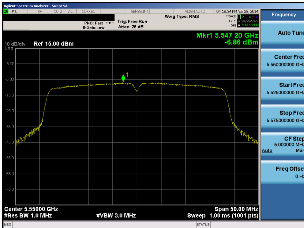
Plot 6-53. Peak Power Spectral Density Plot (40MHz BW 802.11n (UNII Band 2C) – Ch. 110)
