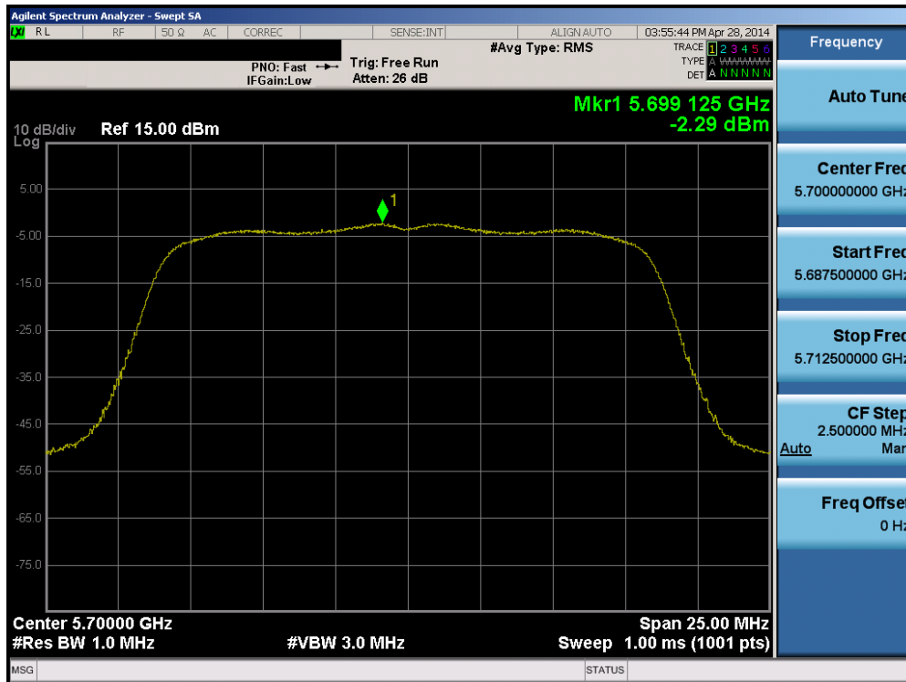
Plot 6-48. Peak Power Spectral Density Plot (802.11a (UNII Band 2C) – Ch. 140)
