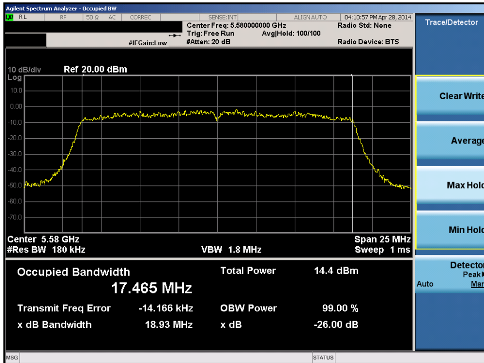
Plot 6-22. 26dB Bandwidth Plot (20MHz BW 802.11n (UNII Band 2C) – Ch. 116)
