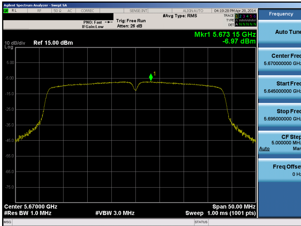
Plot 6-54. Peak Power Spectral Density Plot (40MHz BW 802.11n (UNII Band 2C) – Ch. 134)
