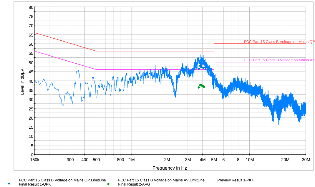
Plot 6-73. Line Conducted Plot with 802.11a UNII Band 1 (N)
