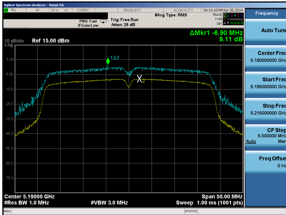
Plot 6-55. Peak Excursion Ratio Plot (40MHz BW 802.11n (UNII Band 1) – Ch. 38)
