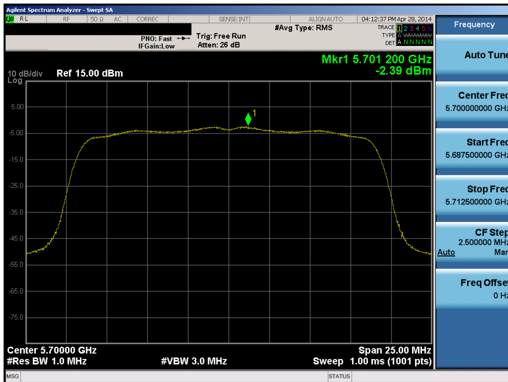
Plot 6-51. Peak Power Spectral Density Plot (20MHz BW 802.11a/n (UNII Band 2C) – Ch. 140)
