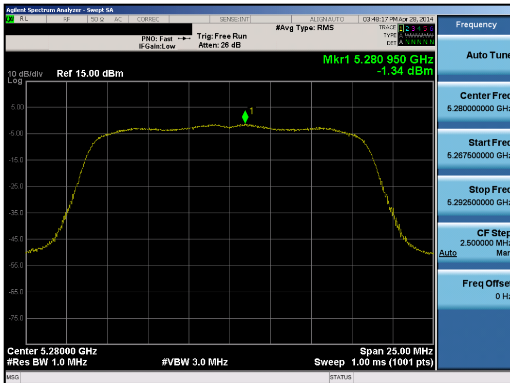
Plot 6-39. Peak Power Spectral Density Plot (802.11a (UNII Band 2A) – Ch. 56)
