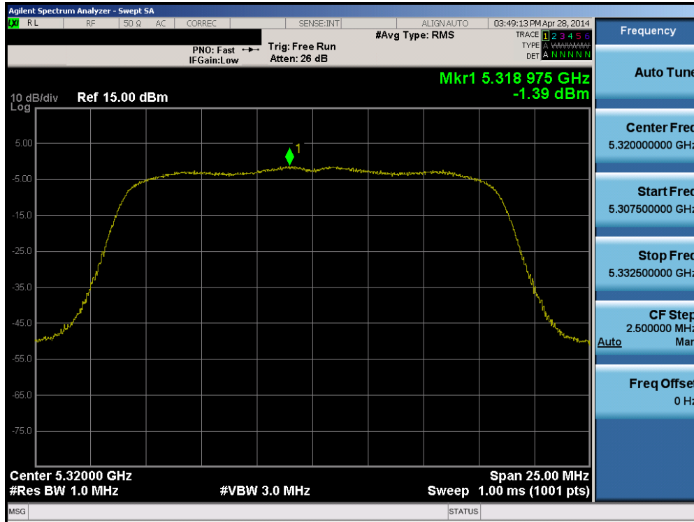
Plot 6-40. Peak Power Spectral Density Plot (802.11a (UNII Band 2A) – Ch. 64)
