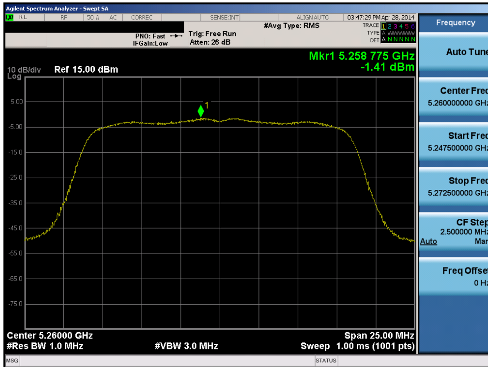
Plot 6-38. Peak Power Spectral Density Plot (802.11a (UNII Band 2A) – Ch. 52)
