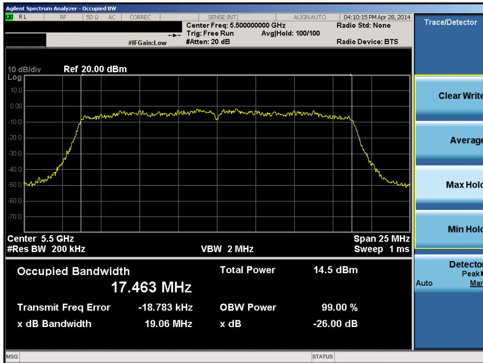
Plot 6-21. 26dB Bandwidth Plot (20MHz BW 802.11n (UNII Band 2C) – Ch. 100)
