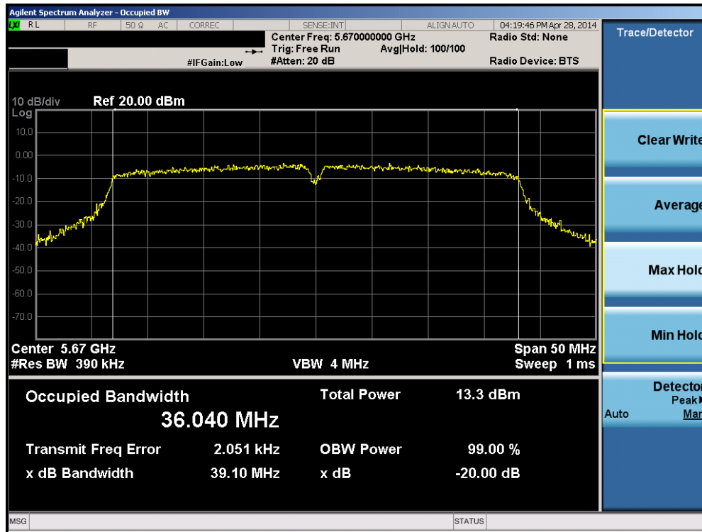
Plot 6-29. 20dB Bandwidth Plot (40MHz BW 802.11n (UNII Band 2C) – Ch. 134)
