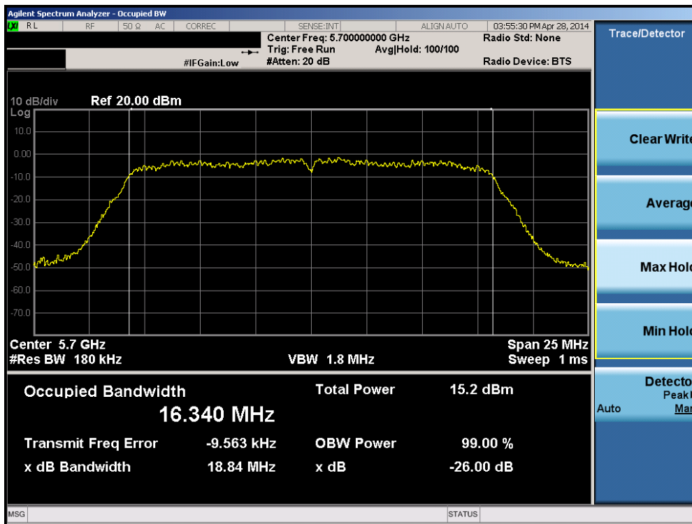
Plot 6-20. 26dB Bandwidth Plot (802.11a (UNII Band 2C) – Ch. 140)
