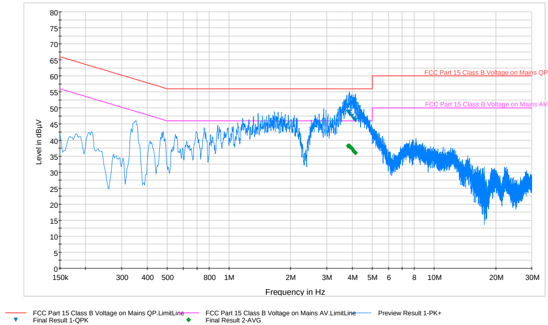
Plot 6-75. Line Conducted Plot with 802.11a UNII Band 2A (N)
