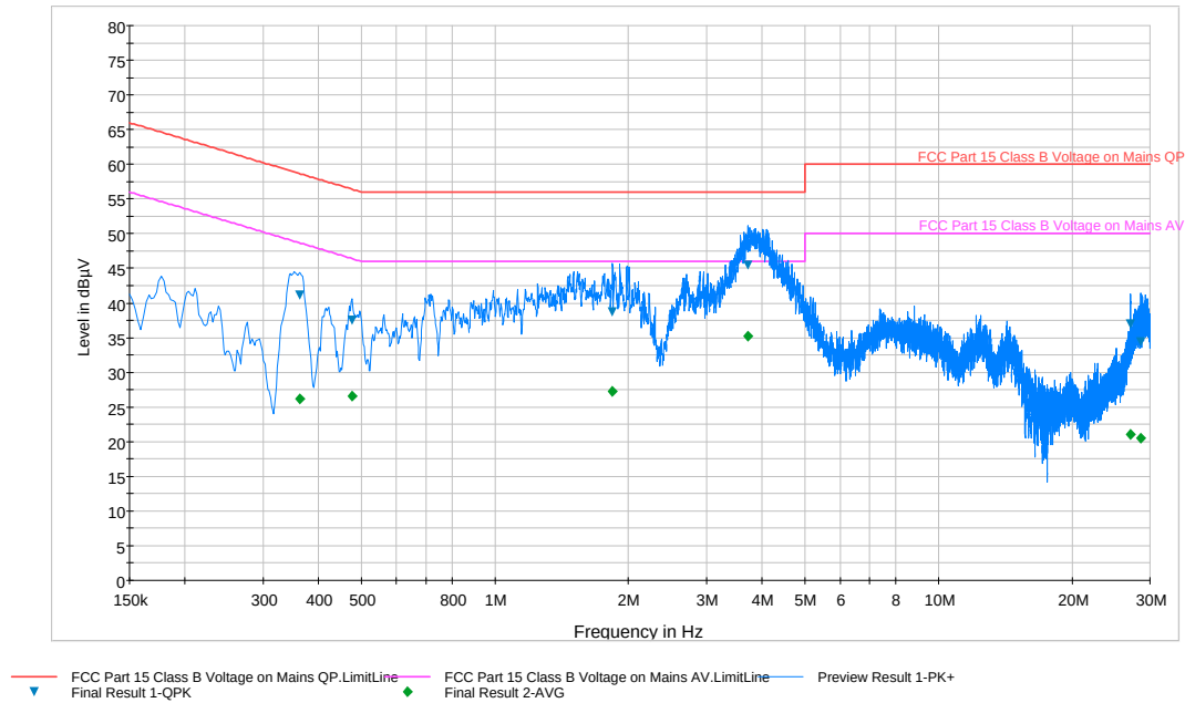
Plot 6-74. Line Conducted Plot with 802.11a UNII Band 2A (L1)
