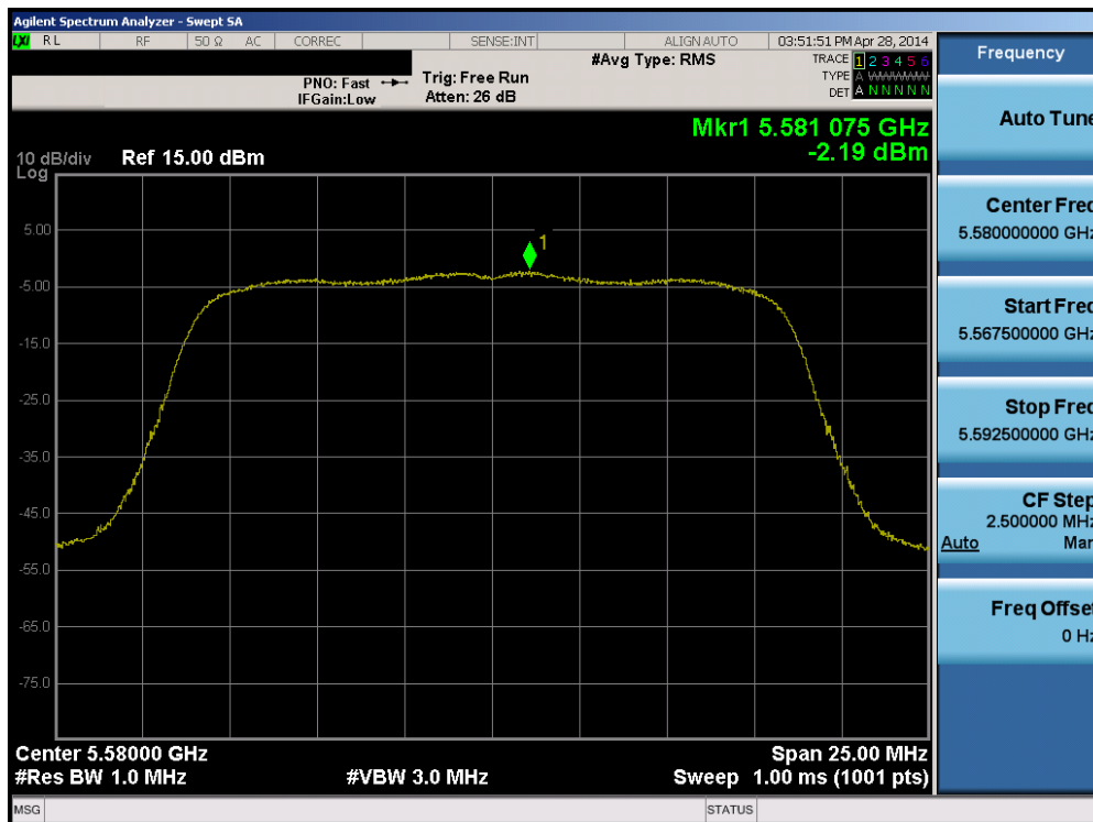
Plot 6-47. Peak Power Spectral Density Plot (802.11a (UNII Band 2C) – Ch. 116)
