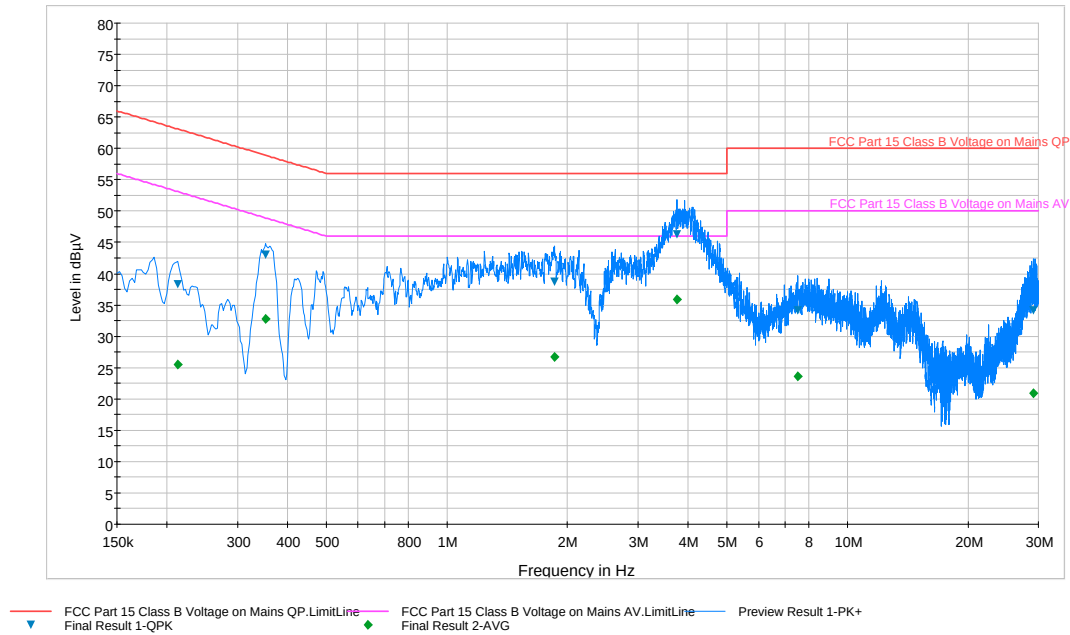
Plot 6-76. Line Conducted Plot with 802.11a UNII Band 2C (L1)
