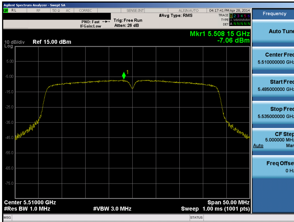
Plot 6-52. Peak Power Spectral Density Plot (40MHz BW 802.11n (UNII Band 2C) – Ch. 102)
