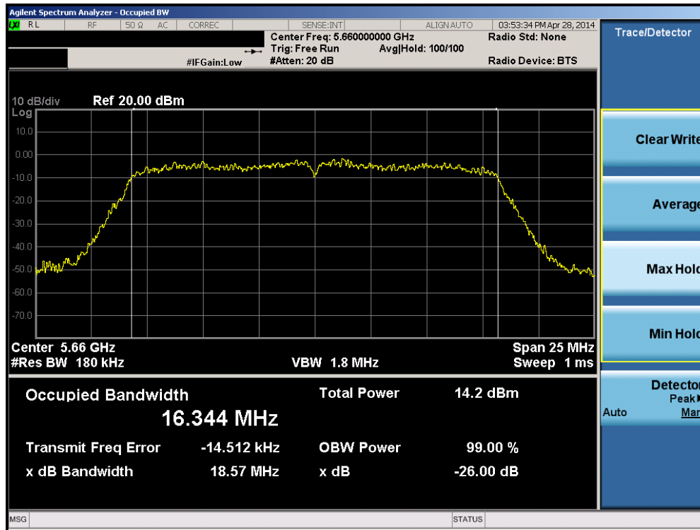
Plot 6-19. 26dB Bandwidth Plot (802.11a (UNII Band 2C) – Ch. 132)
