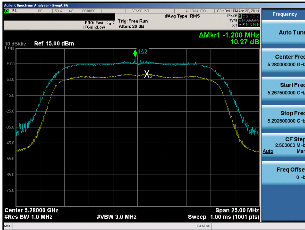
Plot 6-56. Peak Excursion Ratio Plot (802.11a (UNII Band 2A) – Ch. 56)
