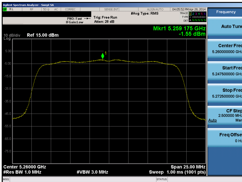
Plot 6-41. Peak Power Spectral Density Plot (20MHz BW 802.11n (UNII Band 2A) – Ch. 52)
