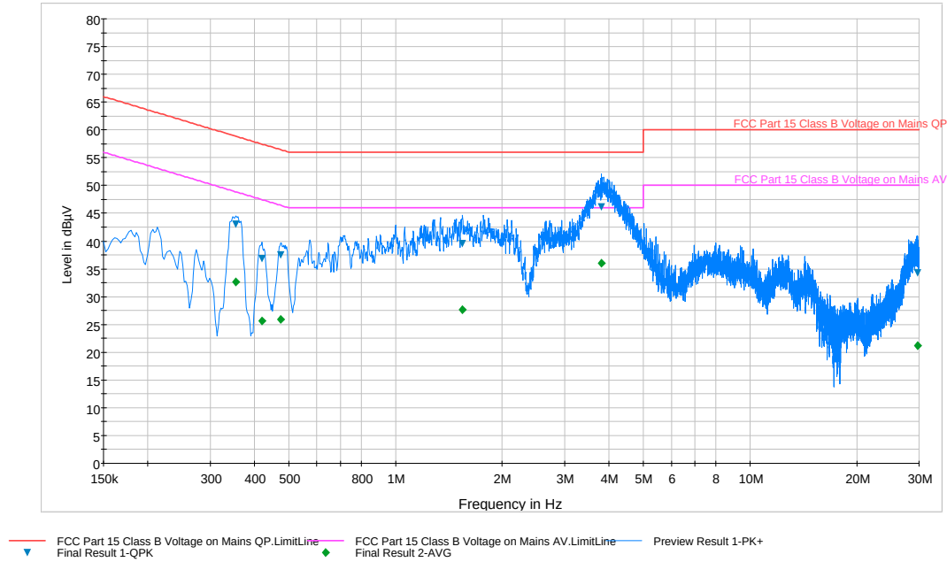
Plot 6-72. Line Conducted Plot with 802.11a UNII Band 1 (L1)
