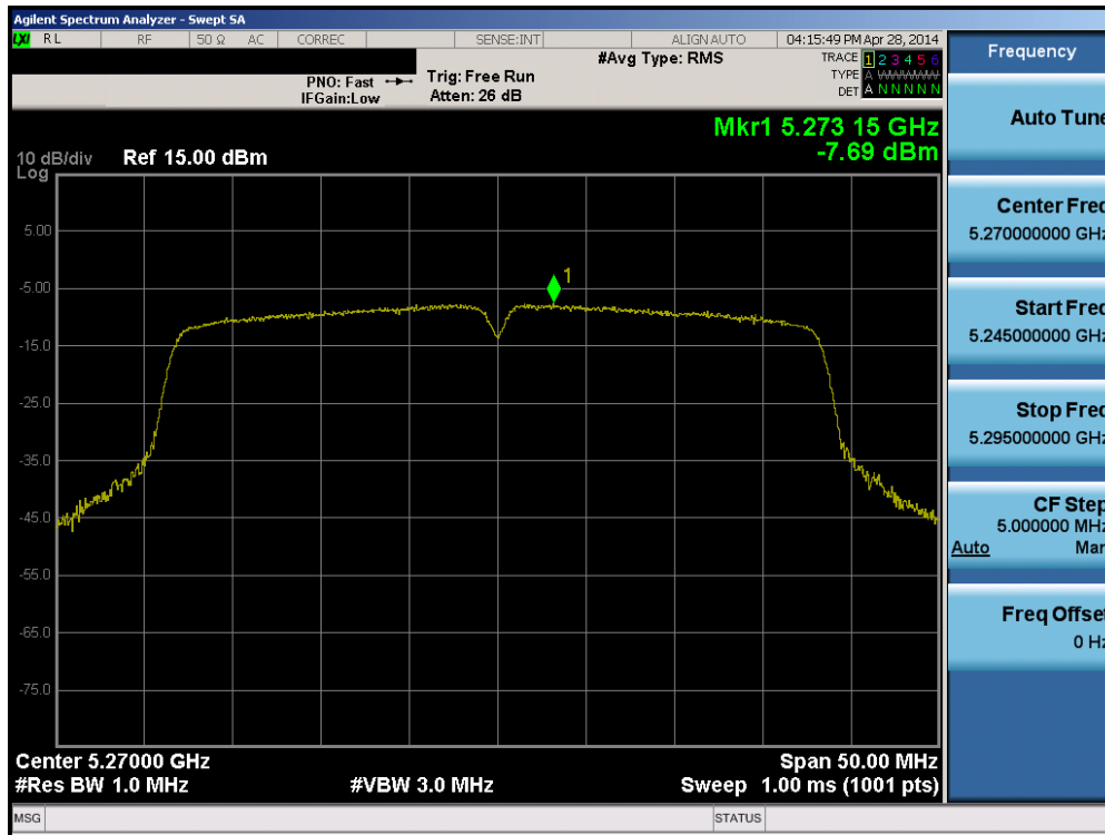
Plot 6-44. Peak Power Spectral Density Plot (40MHz BW 802.11n (UNII Band 2A) – Ch. 54)
