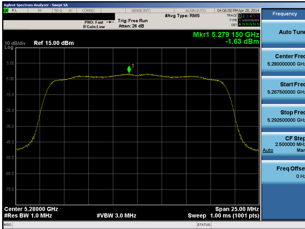
Plot 6-42. Peak Power Spectral Density Plot (20MHz BW 802.11n (UNII Band 2A) – Ch. 56)
