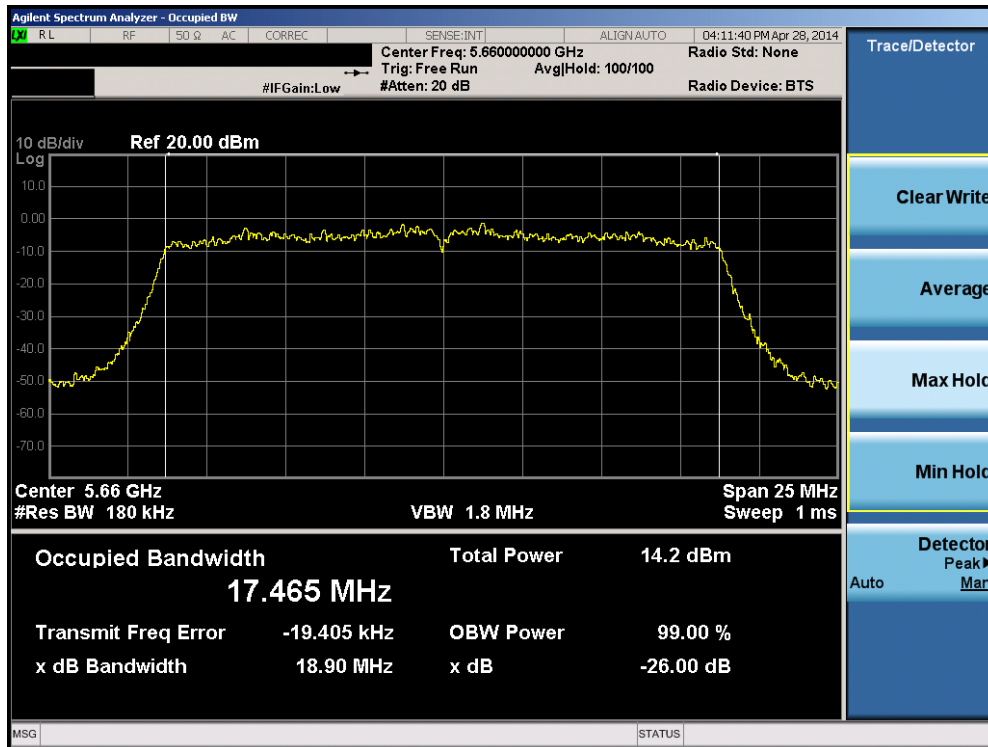
Plot 6-23. 26dB Bandwidth Plot (20MHz BW 802.11n (UNII Band 2C) – Ch. 132)
