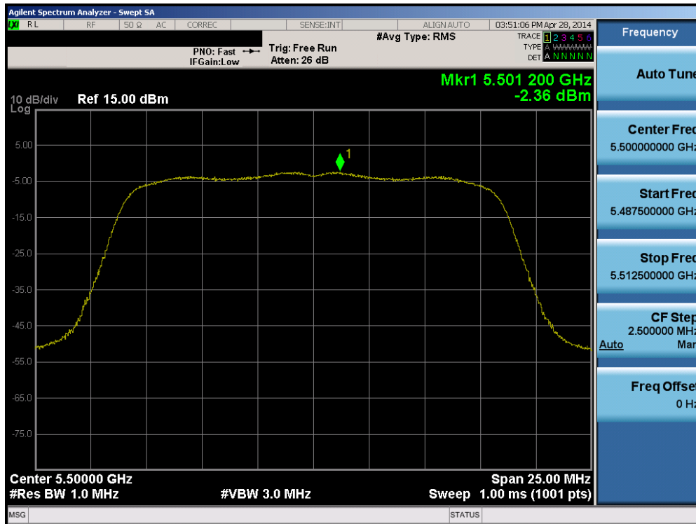
Plot 6-46. Peak Power Spectral Density Plot (802.11a (UNII Band 2C) – Ch. 100)
