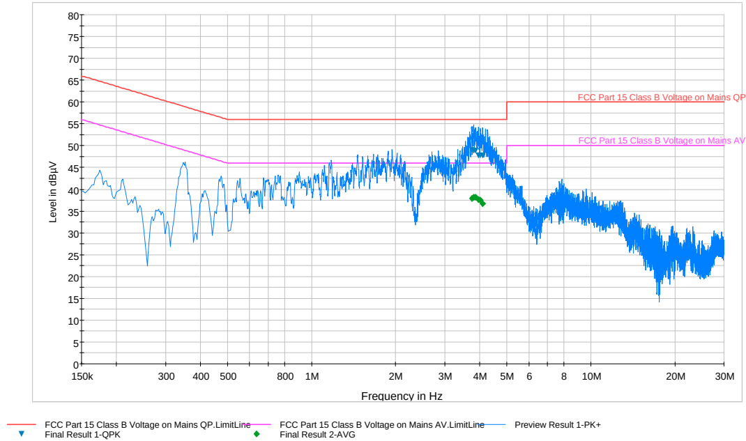
Plot 6-77. Line Conducted Plot with 802.11a UNII Band 2C (N)
