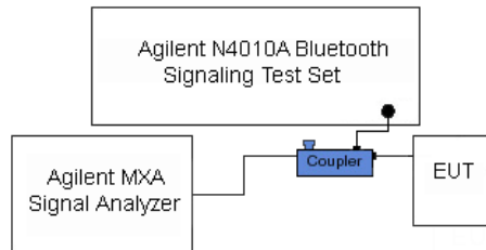
Figure 7-2 Power Measurement Setup
