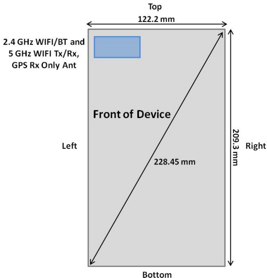
Figure 1-1 DUT Antenna Locations
