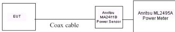
Figure 7-1 Power Measurement Setup
