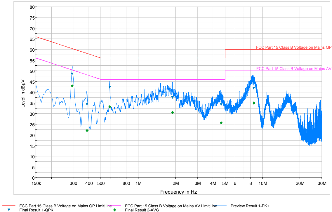
Plot 6-65. Line Conducted Plot with 802.11a (L1)
