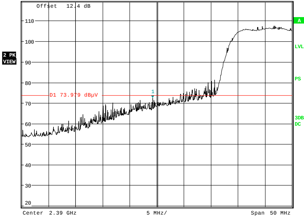
Plot 6-60. Radiated Restricted Lower Band Edge Measurement (Peak)
