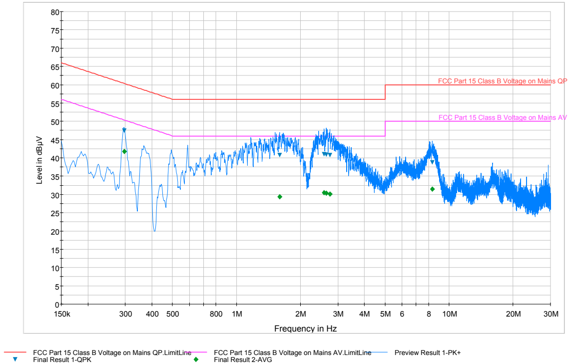
Plot 6-66. Line Conducted Plot with 802.11a (N)
