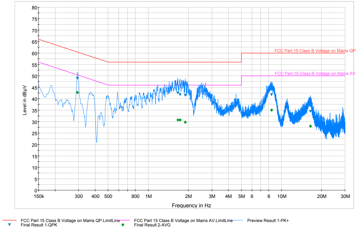
Plot 6-64. Line Conducted Plot with 802.11b (N)
