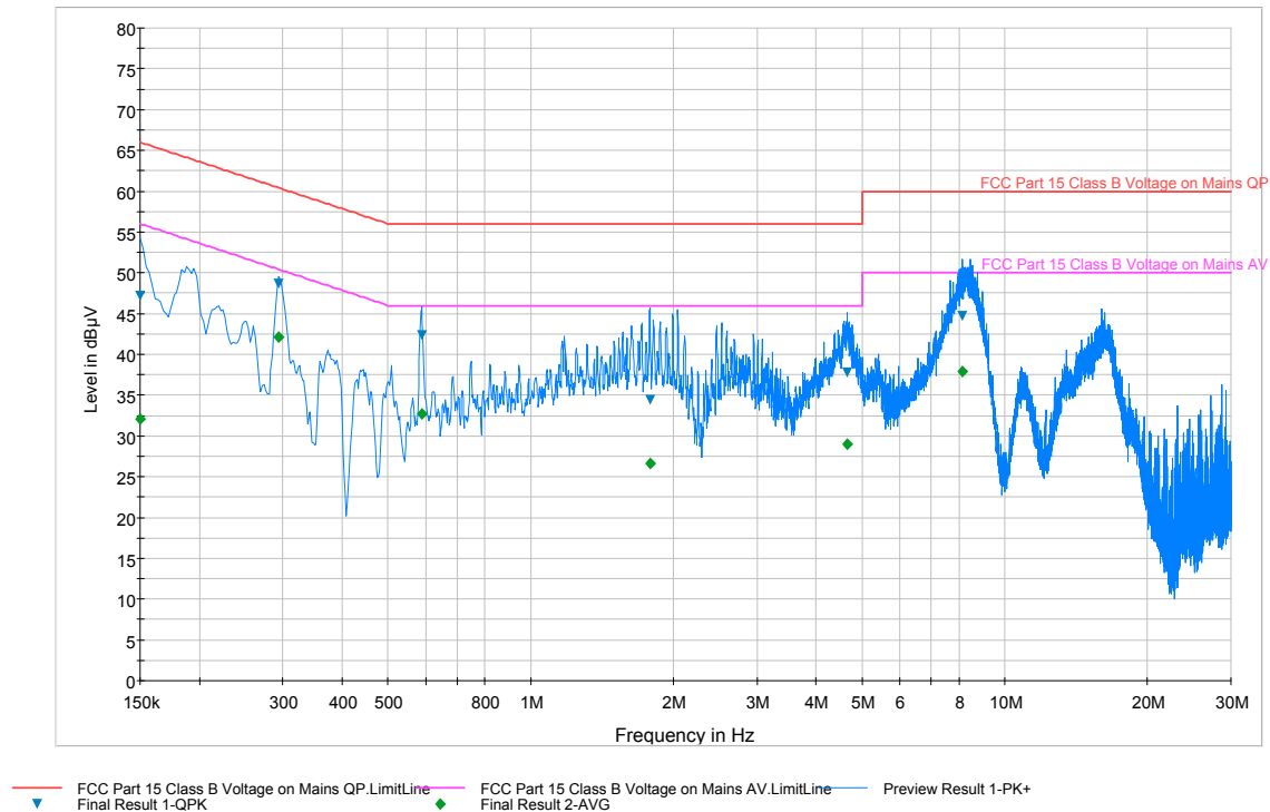
Plot 6-63. Line Conducted Plot with 802.11b (L1)
