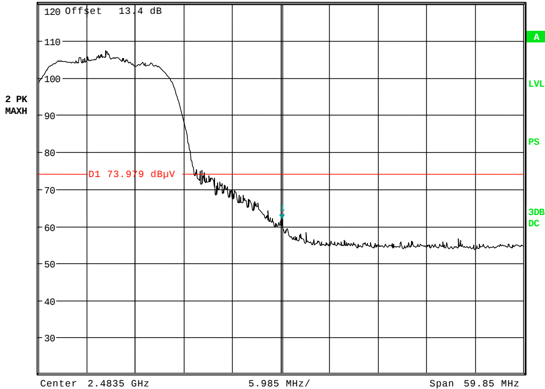
Plot 6-62. Radiated Restricted Upper Band Edge Measurement (Peak)
