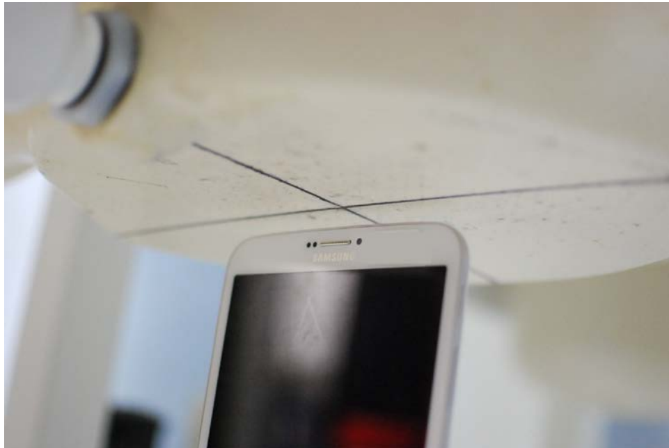
SAR Test Setup Photo 8 - Top Edge at 0.7 cm
