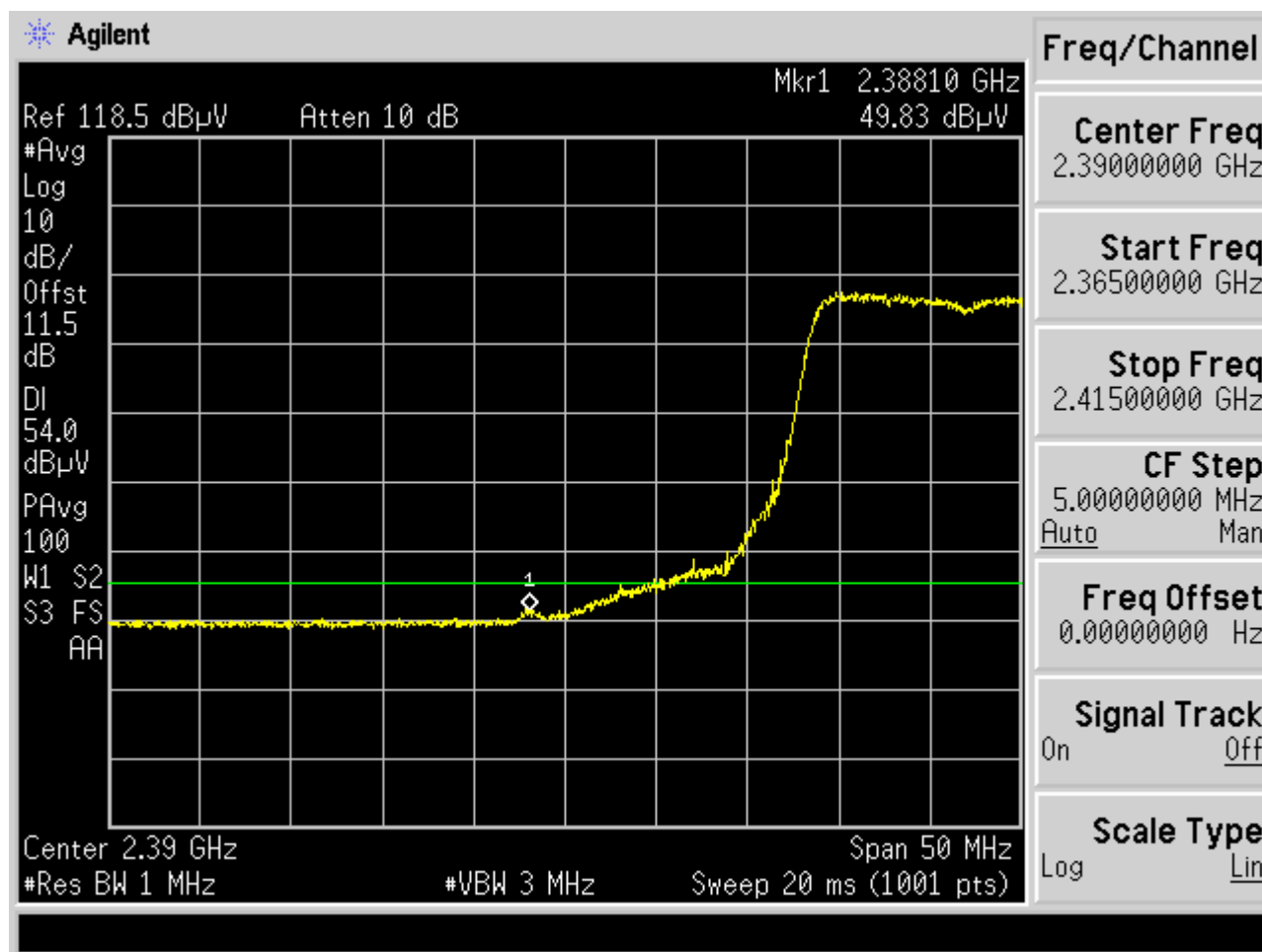
Plot 6-59. Radiated Restricted Lower Band Edge Measurement (Average)
