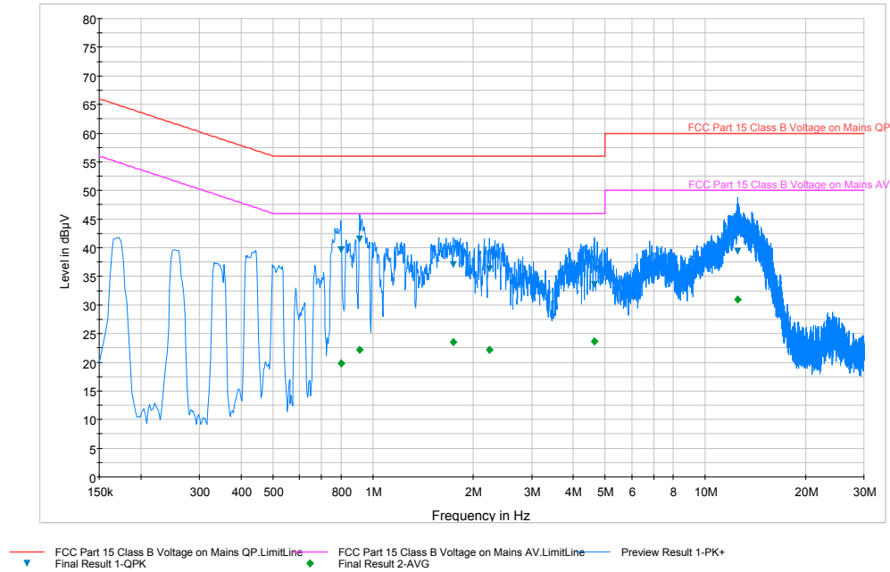
Plot 6-65. Line Conducted Plot with 802.11a (L1)
