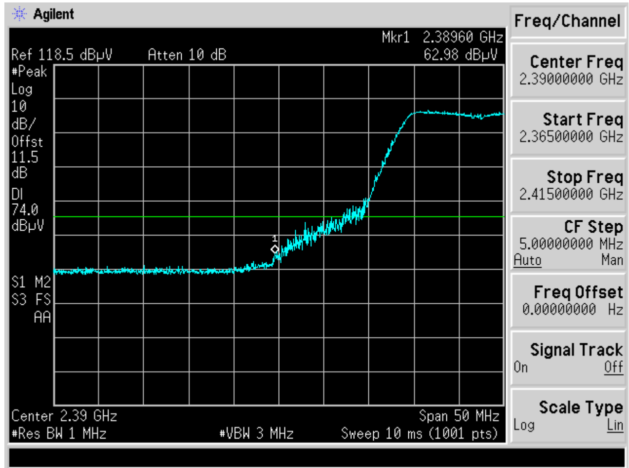
Plot 6-60. Radiated Restricted Lower Band Edge Measurement (Peak)
