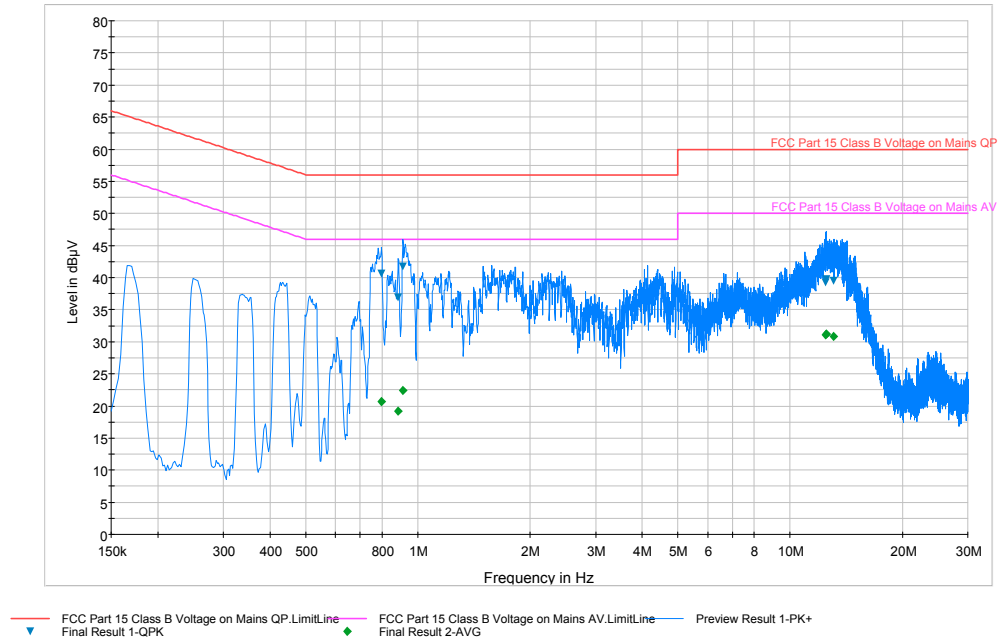
Plot 6-64. Line Conducted Plot with 802.11b (N)
