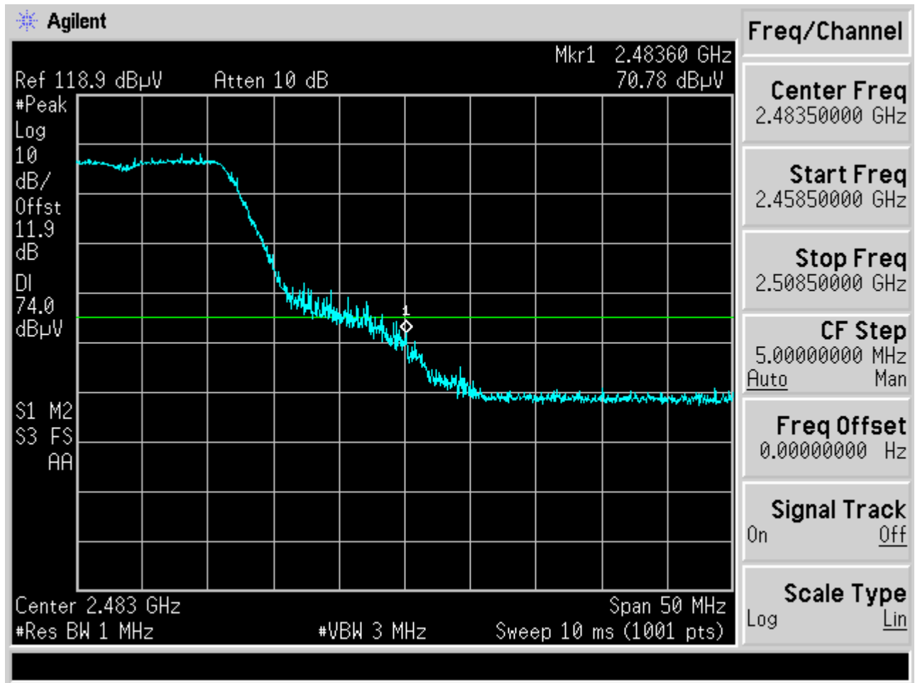
Plot 6-62. Radiated Restricted Upper Band Edge Measurement (Peak)
