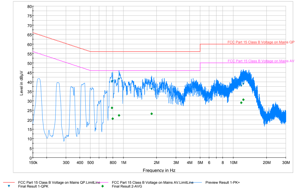
Plot 6-66. Line Conducted Plot with 802.11a (N)
