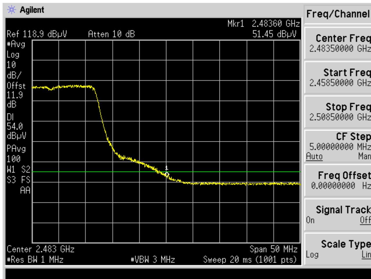
Plot 6-61. Radiated Restricted Upper Band Edge Measurement (Average)
