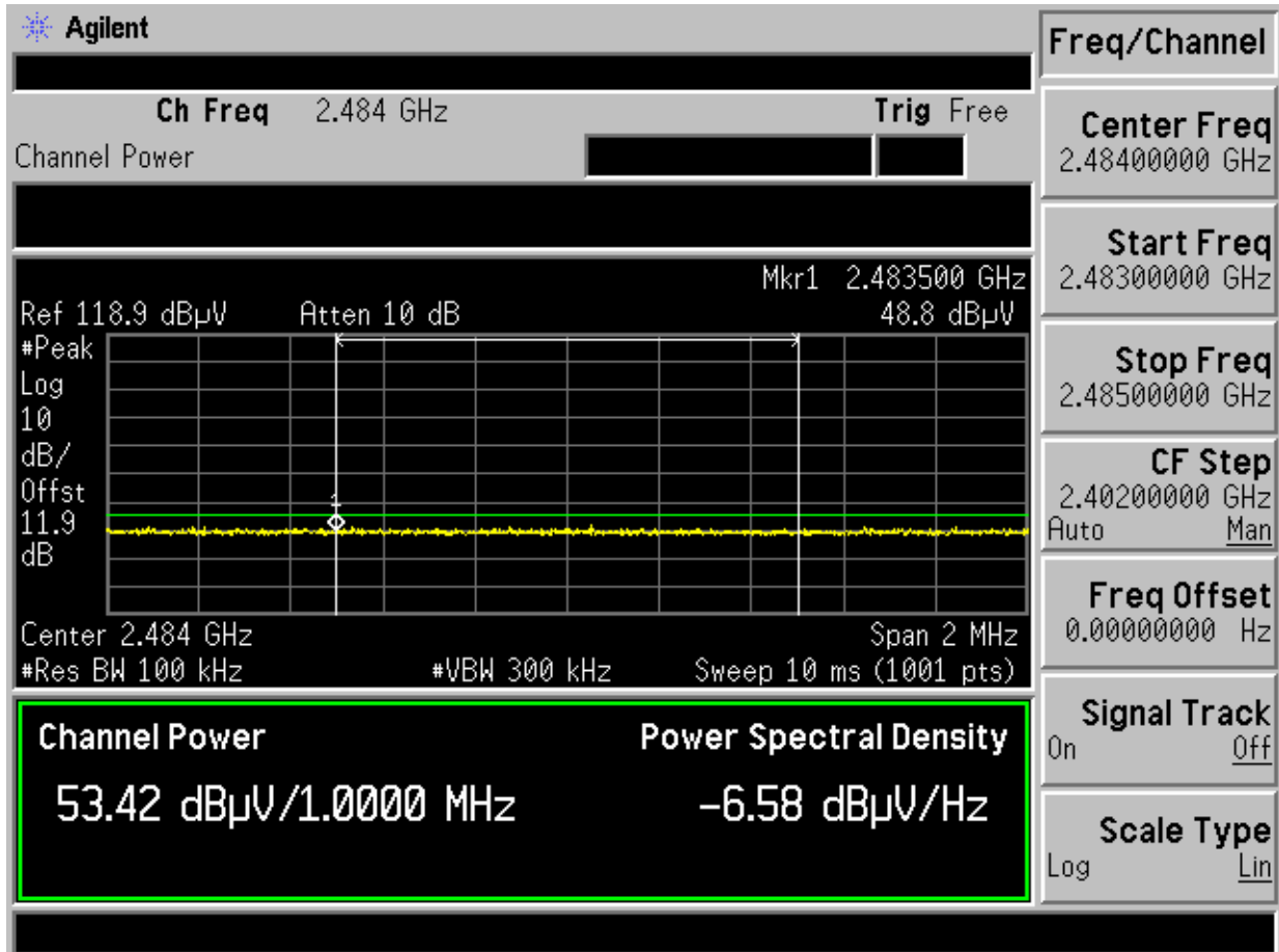
Plot 6-18. Radiated Restricted Band Edge Measurements (Average)
