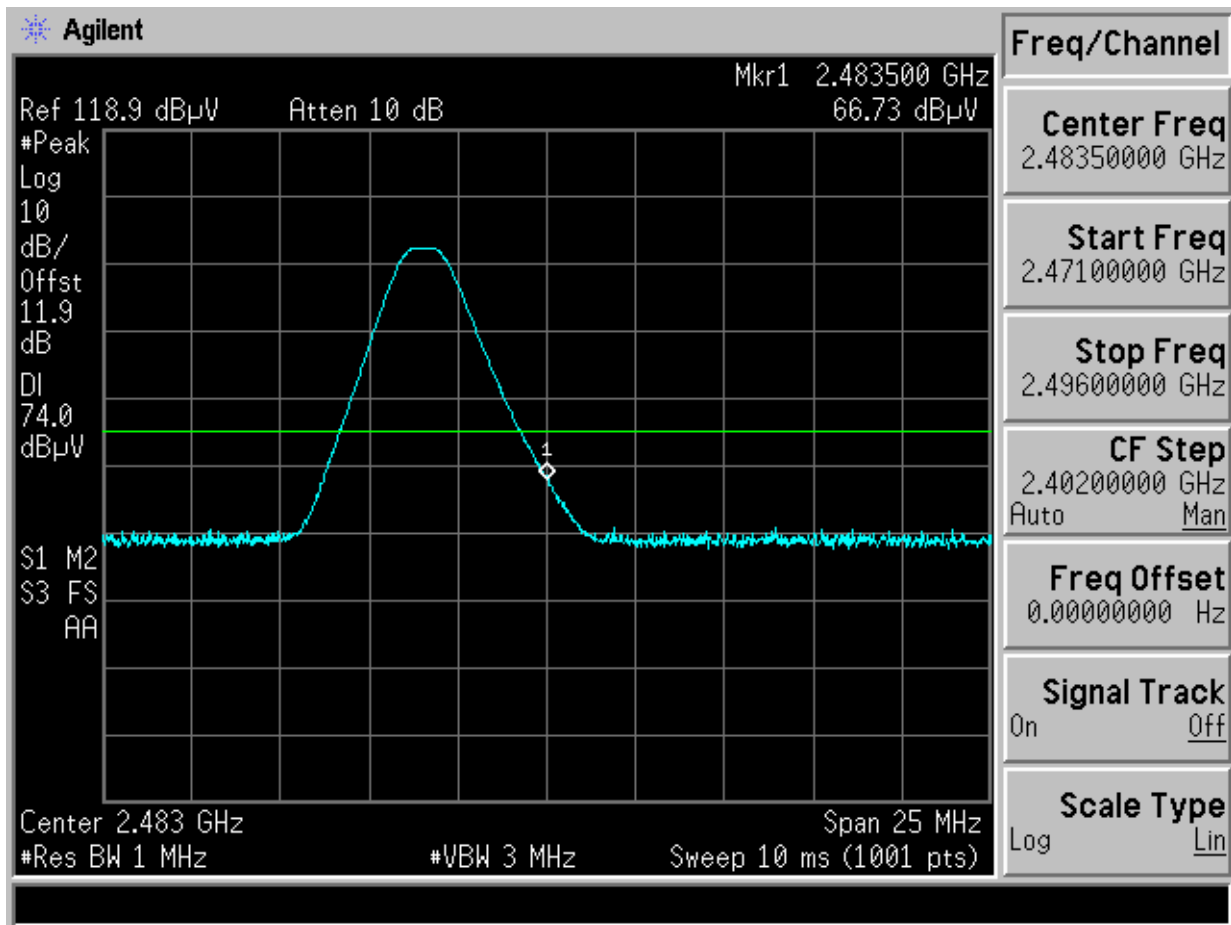
Plot 6-19. Radiated Restricted Band Edge Measurements (Peak)
