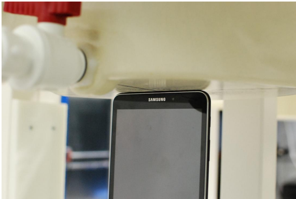
SAR Test Setup Photo 2: Top Edge at 0.0 cm
