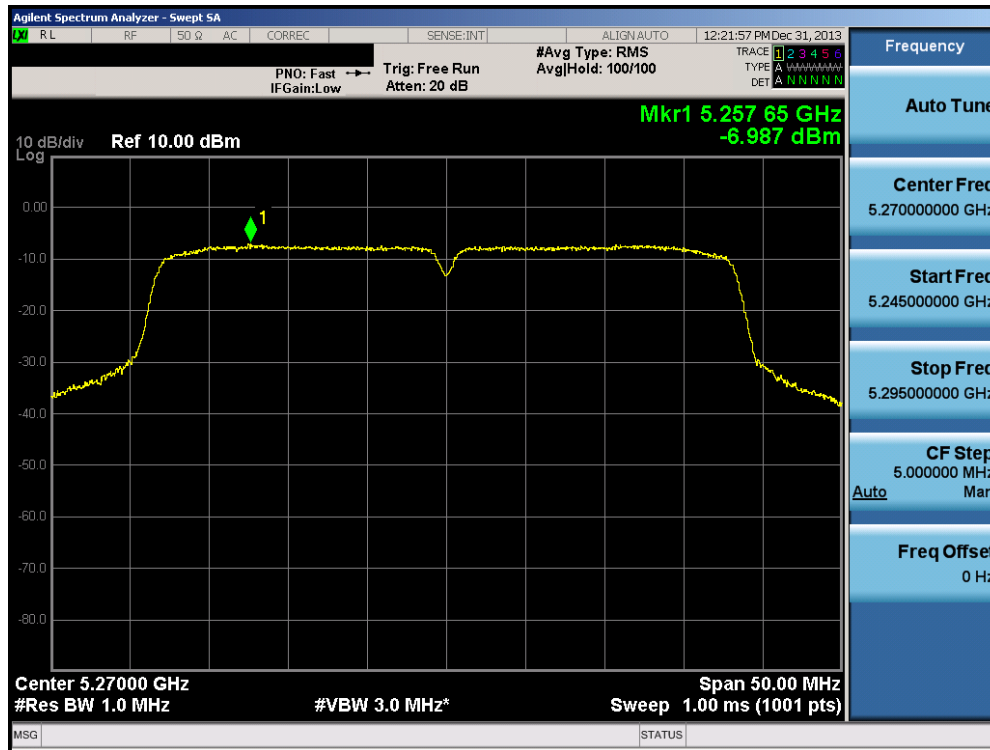
Plot 6-46. Peak Power Spectral Density Plot (40MHz BW 802.11n (UNII Band 2A) – Ch. 54)
