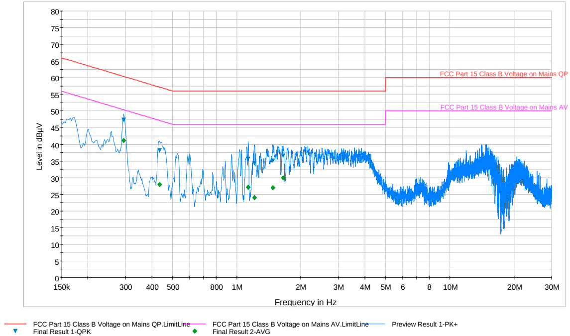
Plot 6-77. Line Conducted Plot with 802.11a UNII Band 2A (N)
