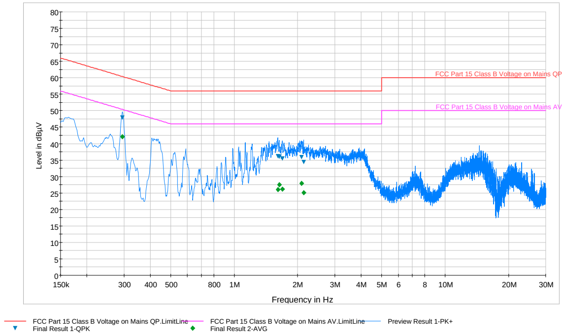
Plot 6-75. Line Conducted Plot with 802.11a UNII Band 1 (N)
