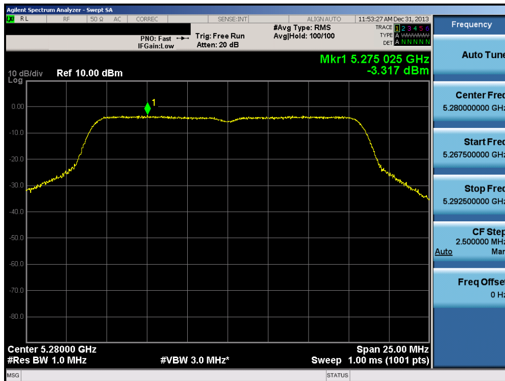
Plot 6-41. Peak Power Spectral Density Plot (802.11a (UNII Band 2A) – Ch. 56)
