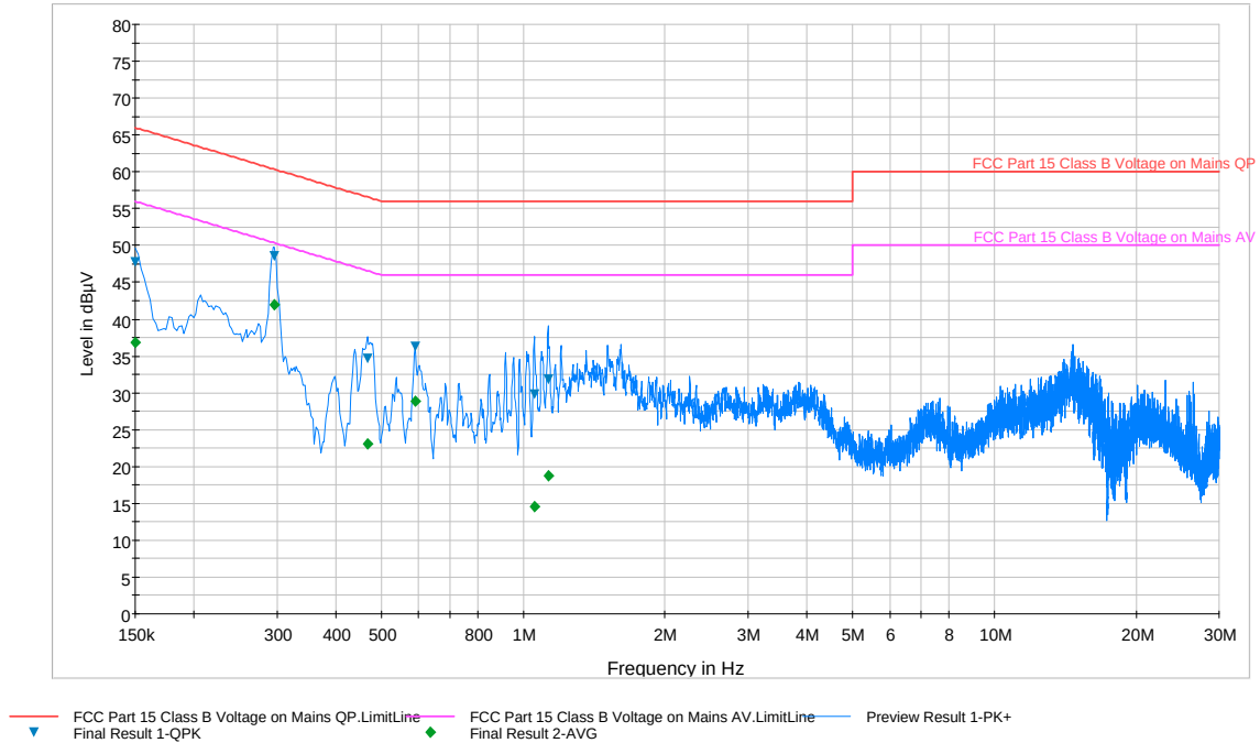
Plot 6-78. Line Conducted Plot with 802.11a UNII Band 2C (L1)
