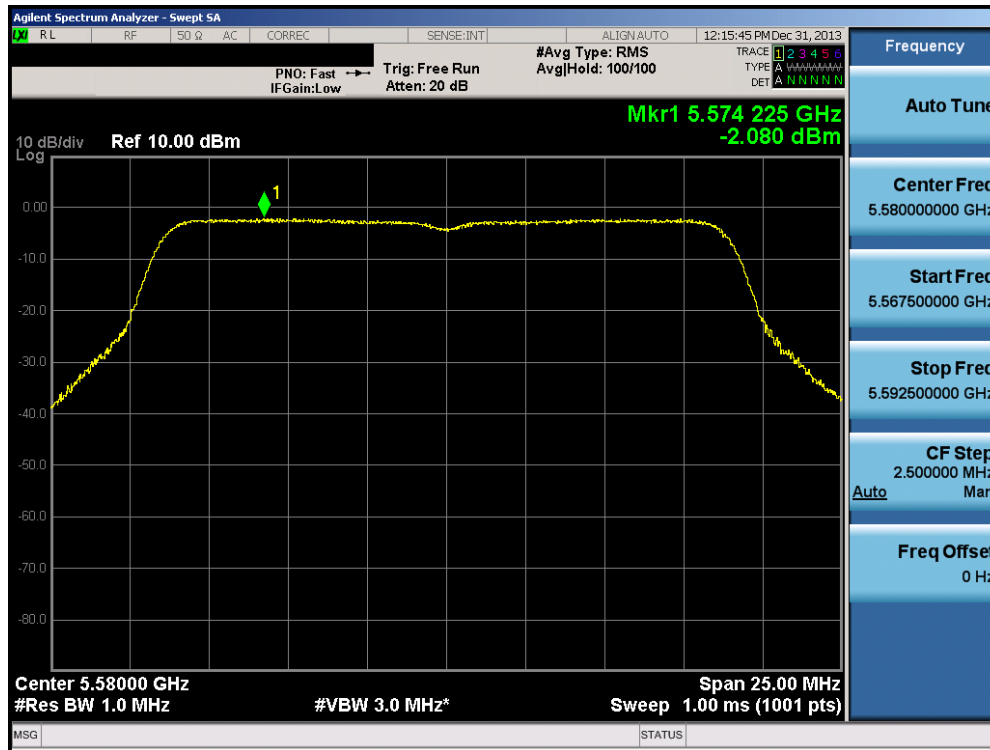
Plot 6-52. Peak Power Spectral Density Plot (20MHz BW 802.11n (UNII Band 2C) – Ch. 116)
