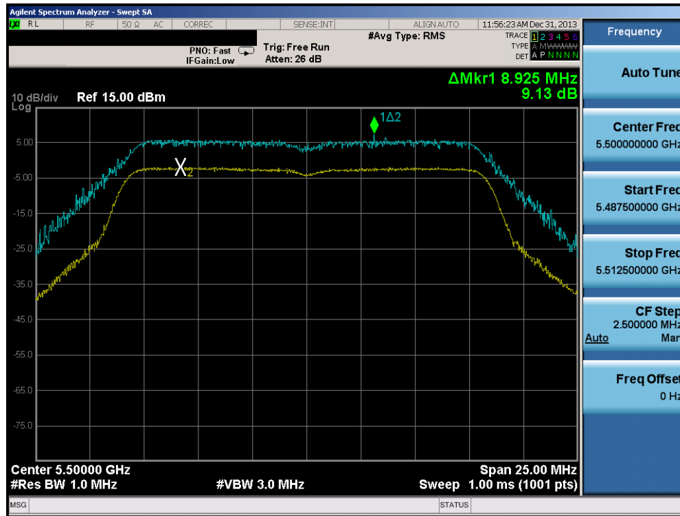
Plot 6-57. Peak Excursion Ratio Plot (802.11a)
