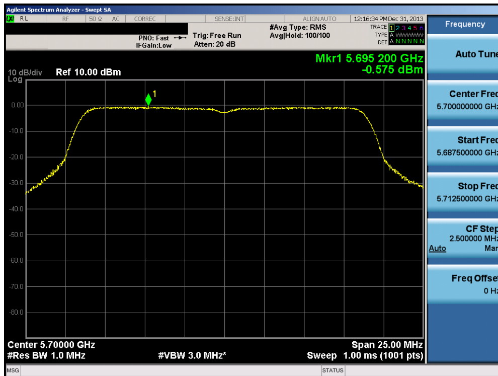
Plot 6-53. Peak Power Spectral Density Plot (20MHz BW 802.11a/n (UNII Band 2C) – Ch. 140)
