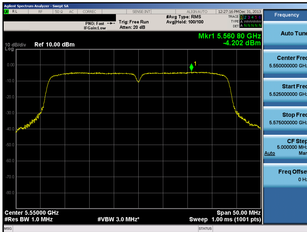
Plot 6-55. Peak Power Spectral Density Plot (40MHz BW 802.11a/n (UNII Band 2C) – Ch. 110)
