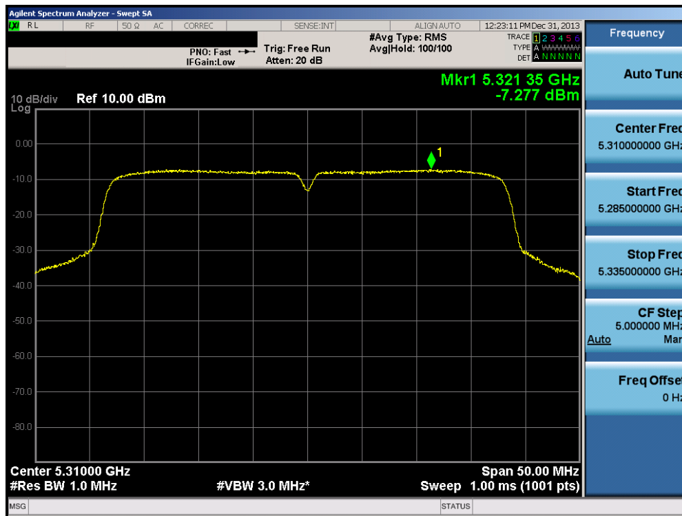
Plot 6-47. Peak Power Spectral Density Plot (40MHz BW 802.11a/n (UNII Band 2A) – Ch. 62)
