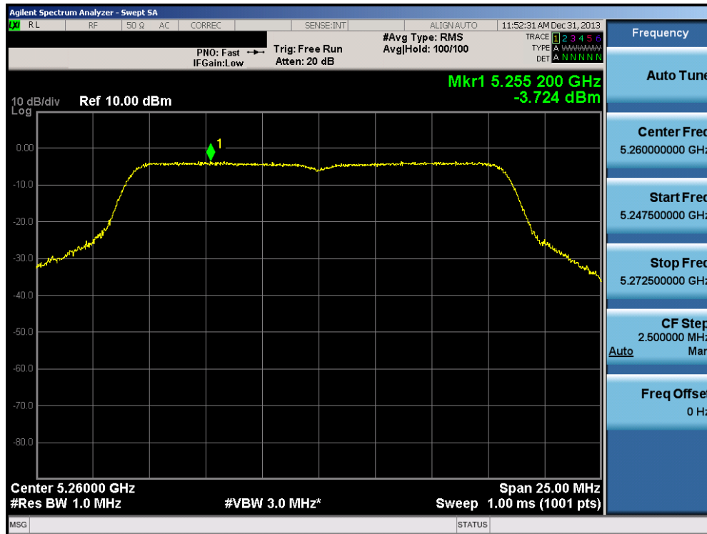
Plot 6-40. Peak Power Spectral Density Plot (802.11a (UNII Band 2A) – Ch. 52)
