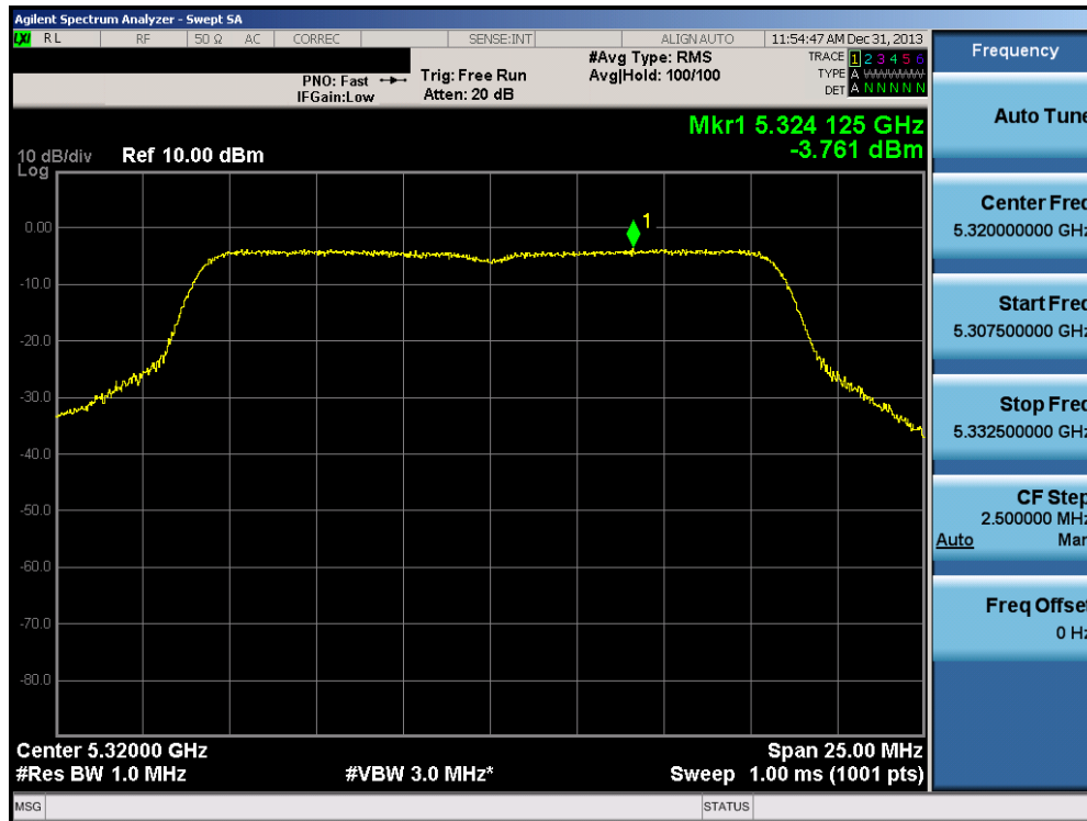
Plot 6-42. Peak Power Spectral Density Plot (802.11a (UNII Band 2A) – Ch. 64)
