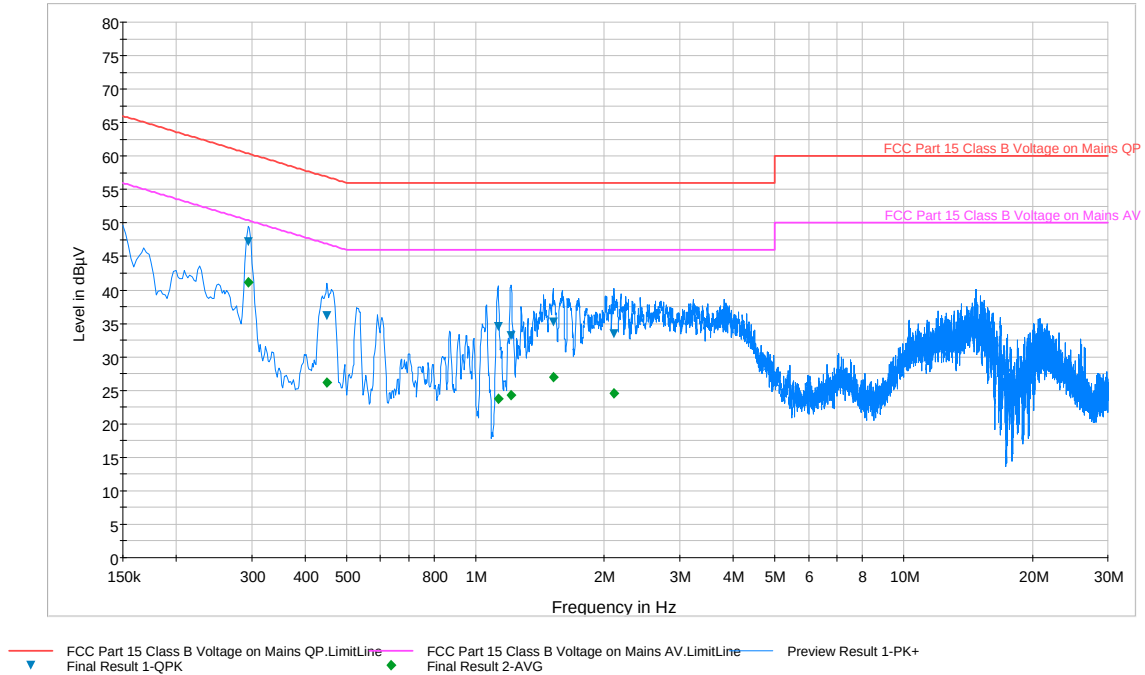
Plot 6-79. Line Conducted Plot with 802.11a UNII Band 2C (N)
