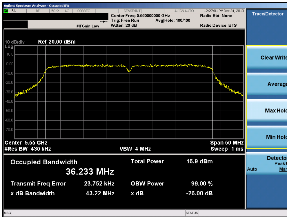
Plot 6-24. 26dB Bandwidth Plot (40MHz BW 802.11a/n (UNII Band 2C) – Ch. 110)
