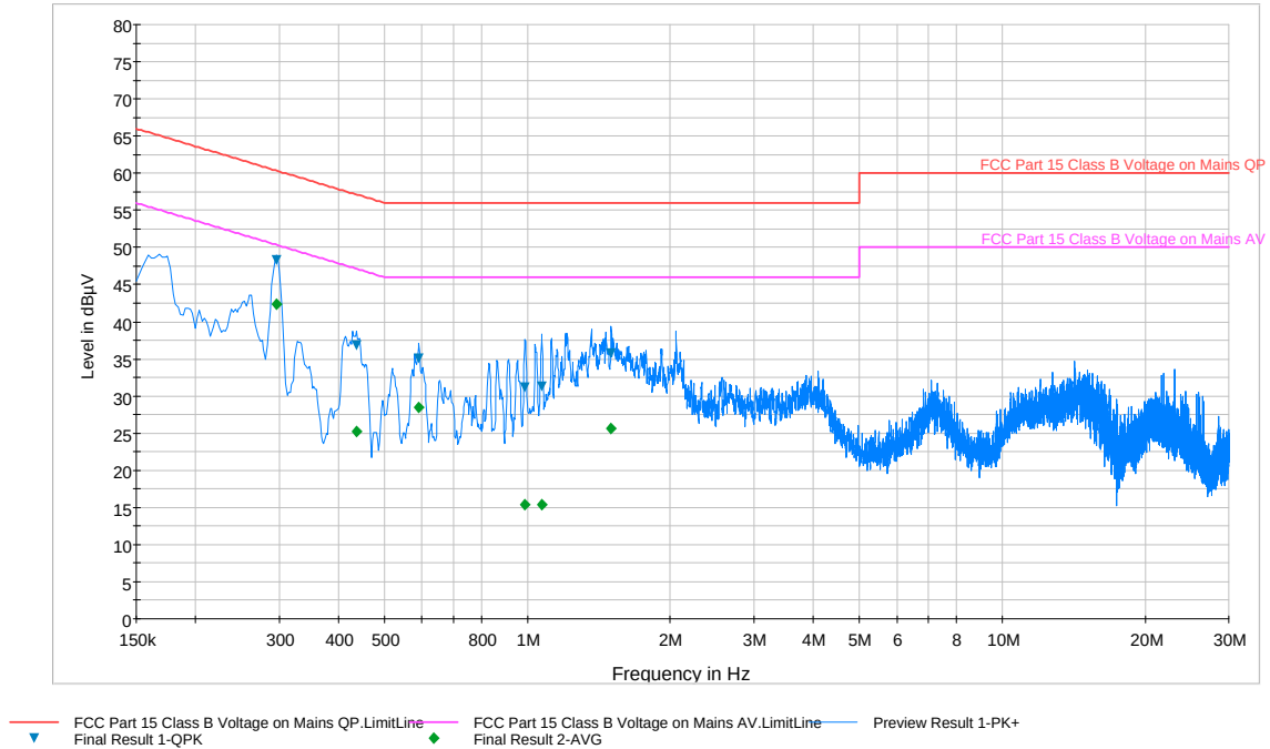
Plot 6-74. Line Conducted Plot with 802.11a UNII Band 1 (L1)
