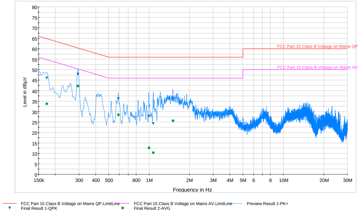
Plot 6-76. Line Conducted Plot with 802.11a UNII Band 2A (L1)
