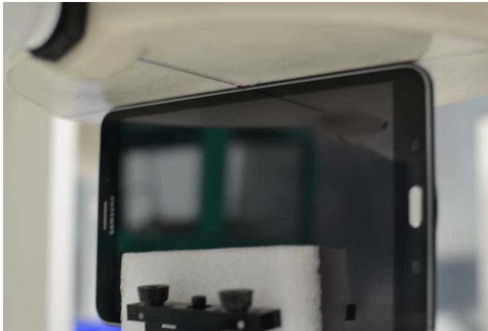
SAR Test Setup Photo 10 – Right Edge at 0.0 cm
