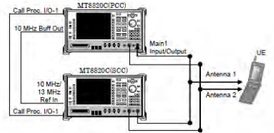
Figure 8-2 Power Measurement Setup
