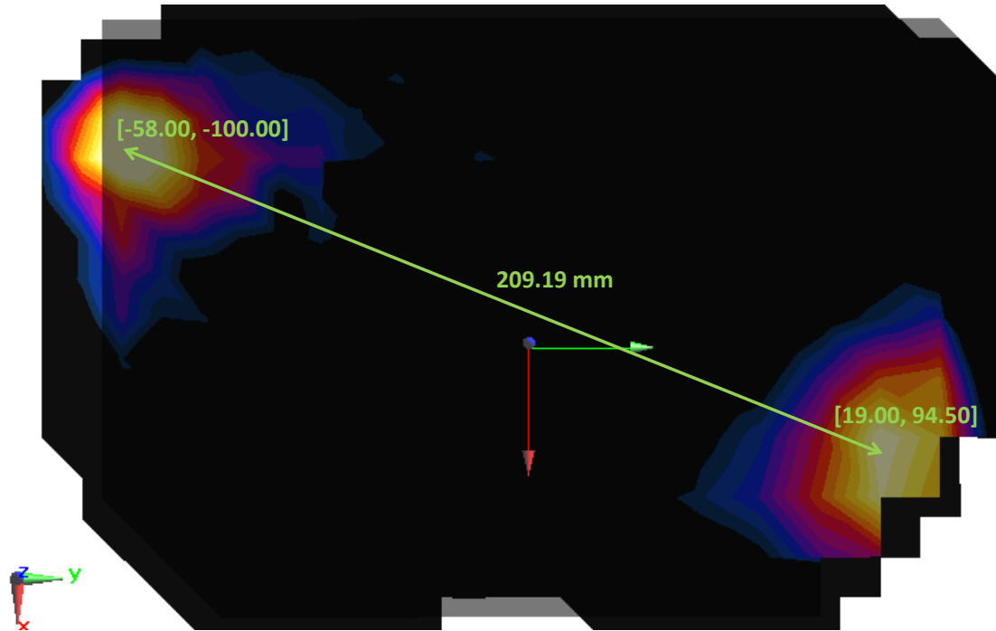
Figure 11-2 Peak SAR Locations for Body Back Side at 0 mm LTE B2 and 5 GHz WLAN Antenna
