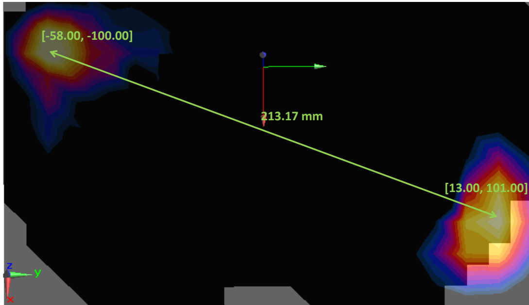
Figure 11-3 Peak SAR Locations for Body Back Side at 17 mm LTE B2 and 5 GHz WLAN Antenna
