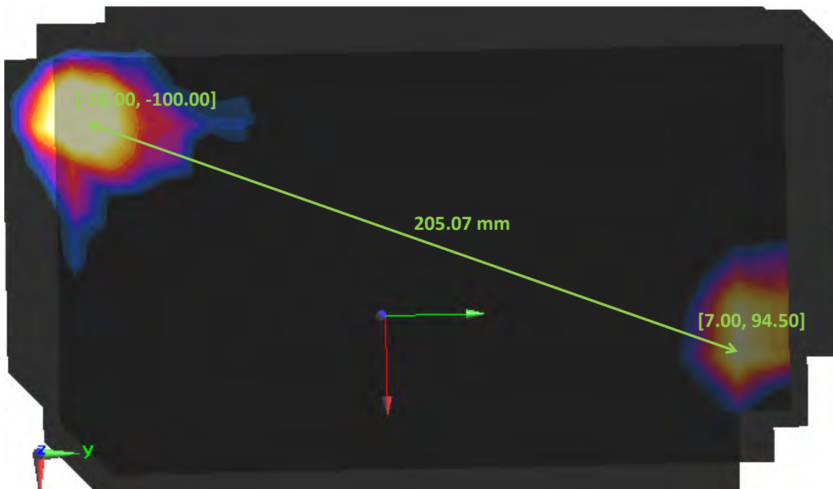
Figure 11-1 Peak SAR Locations for Body Back Side at 0 mm UMTS 1900 and 5 GHz WLAN Antenna
