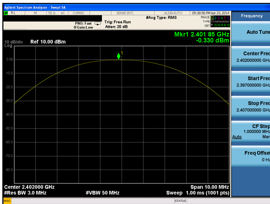
Plot 6-4. Peak Power Plot (Bluetooth (LE) – Ch. 0)
