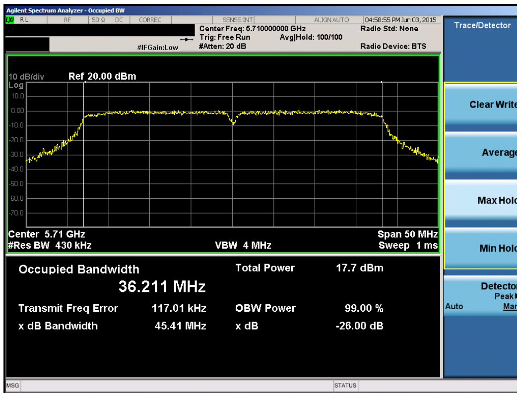
Plot 6-25. 26dB Bandwidth Plot (40MHz BW 802.11n (UNII Band 2C) – Ch. 142)
