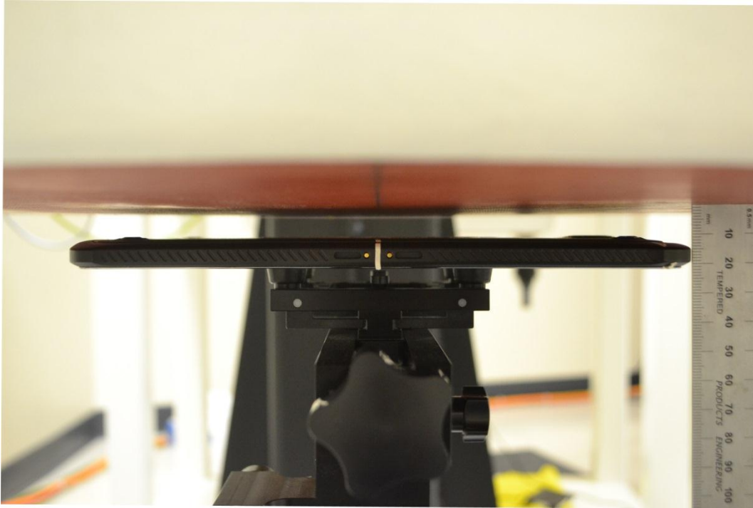
Rear at 12 mm spacing
