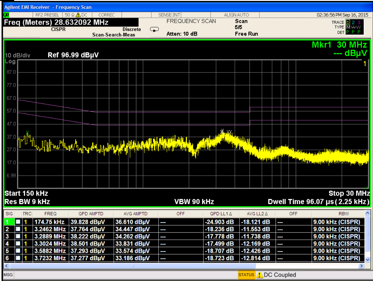
Plot 6-46. Line Conducted Plot with 802.11b (N)
