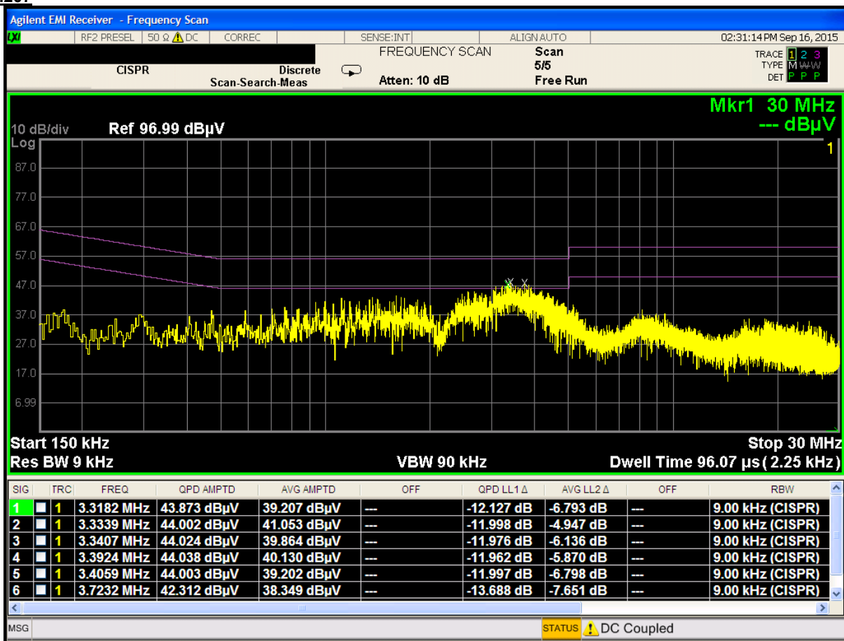
Plot 6-45. Line Conducted Plot with 802.11b (L1)
