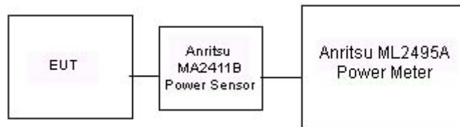
Figure 6-1 Power Measurement Setup for Bandwidths < 50 MHz
