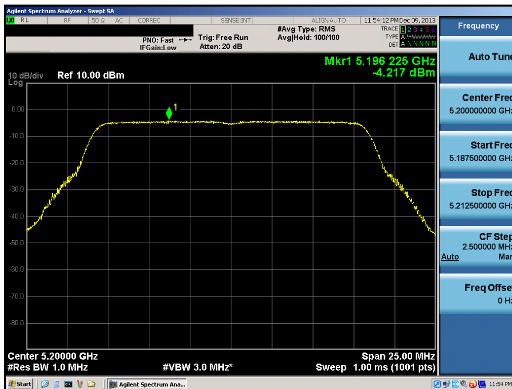
Plot 6-33. Peak Power Spectral Density Plot (802.11a (UNII Band 1) – Ch. 40)
