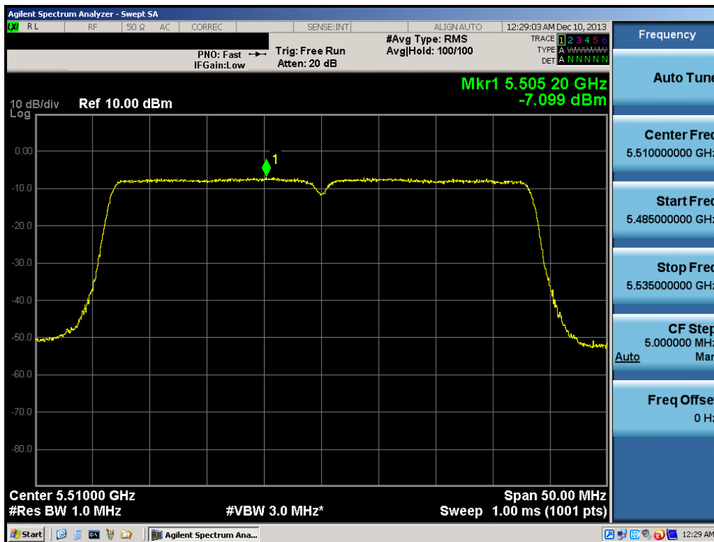
Plot 6-56. Peak Power Spectral Density Plot (40MHz BW 802.11n (UNII Band 2C) – Ch. 102)
