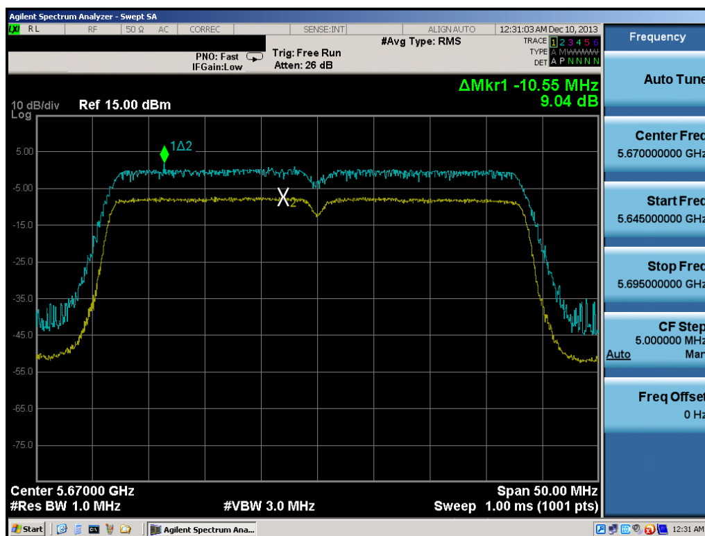
Plot 6-62. Peak Excursion Ratio Plot (40MHz BW 802.11n)
