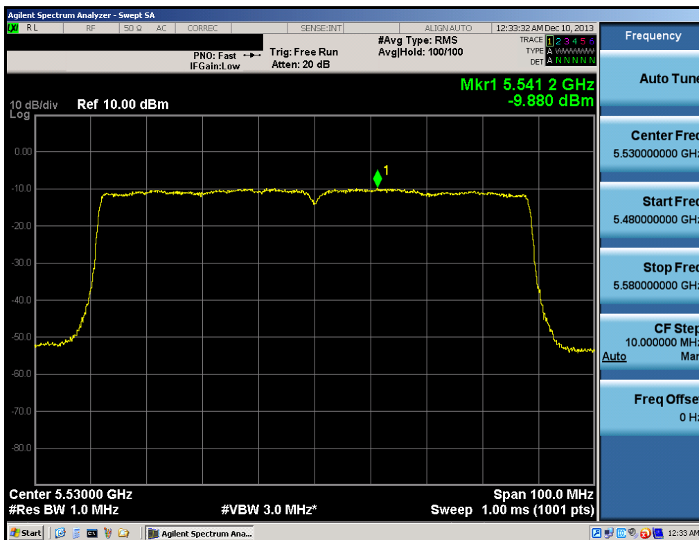
Plot 6-59. Peak Power Spectral Density Plot (80MHz BW 802.11ac (UNII Band 2C) – Ch. 106)
