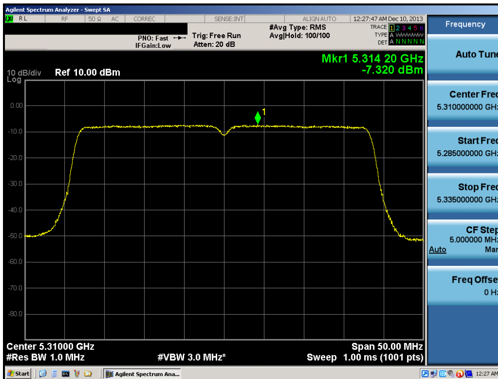
Plot 6-48. Peak Power Spectral Density Plot (40MHz BW 802.11n (UNII Band 2A) – Ch. 62)
