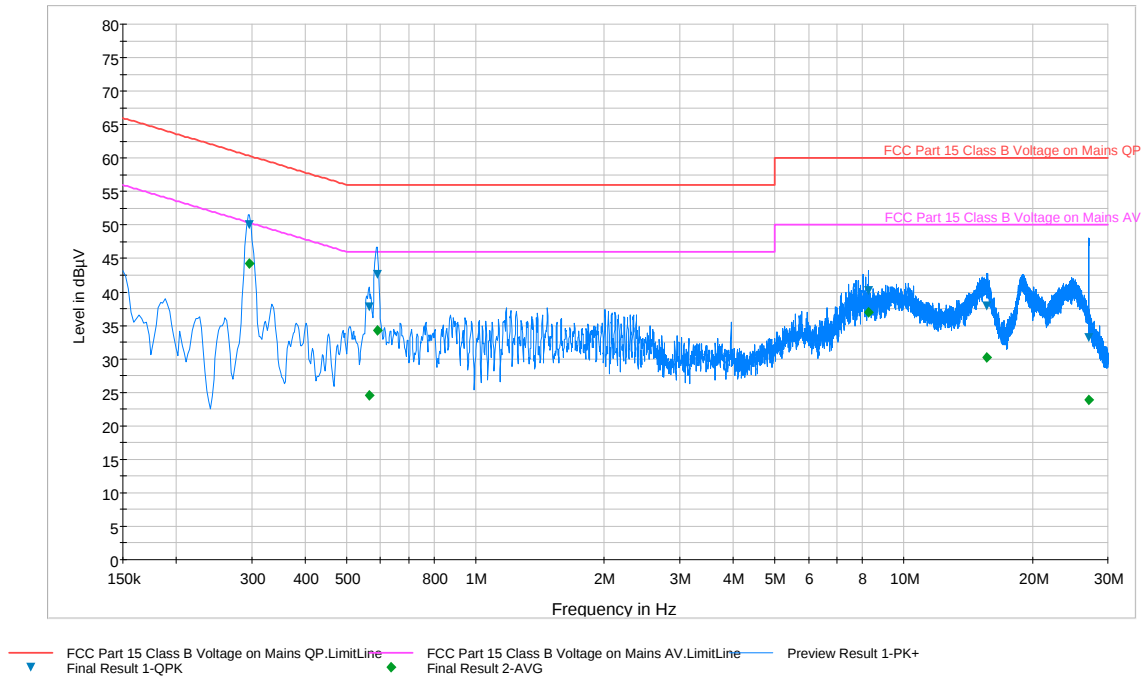
Plot 6-87. Line Conducted Plot with 802.11a UNII Band 2A (N)
