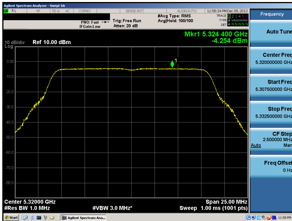
Plot 6-43. Peak Power Spectral Density Plot (802.11a (UNII Band 2A) – Ch. 64)
