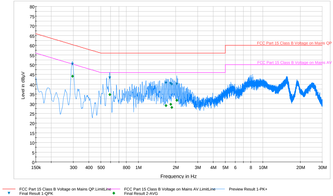
Plot 6-86. Line Conducted Plot with 802.11a UNII Band 2A (L1)
