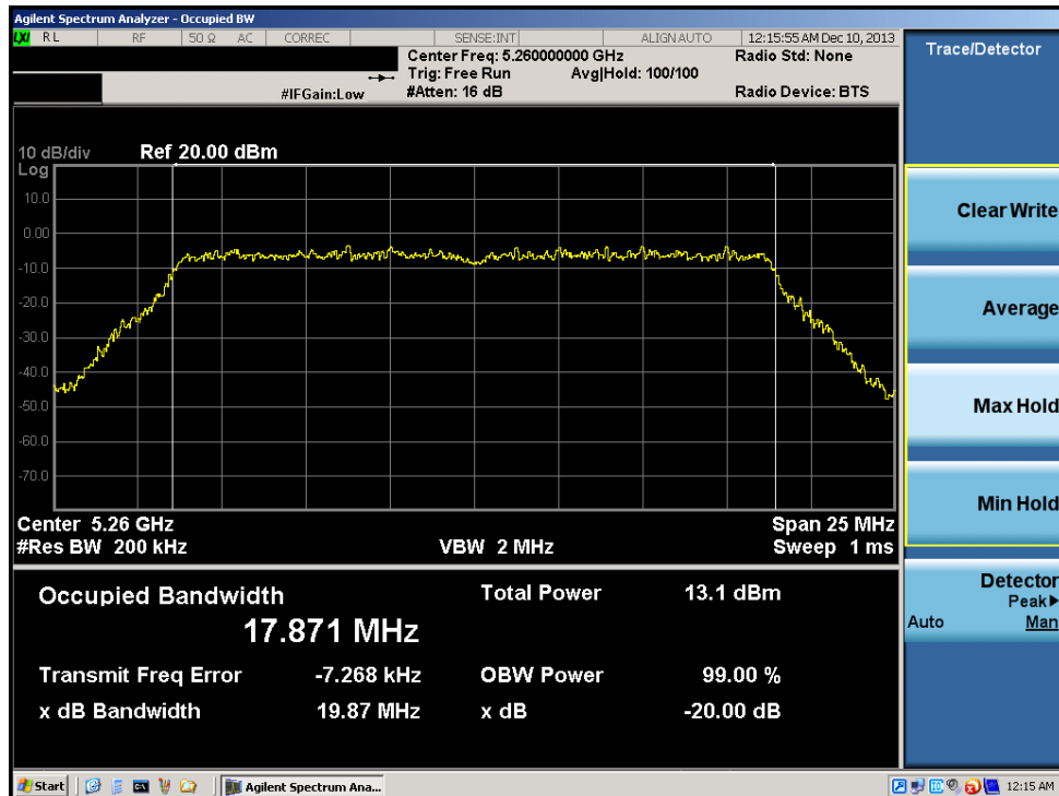
Plot 6-30. 20dB Bandwidth Plot (20MHz BW 802.11n (UNII Band 2A) – Ch. 52)
