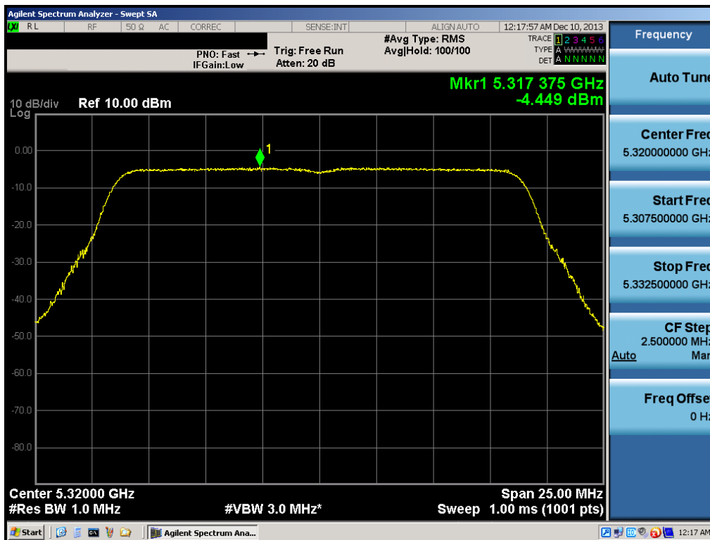
Plot 6-46. Peak Power Spectral Density Plot (20MHz BW 802.11n (UNII Band 2A) – Ch. 64)
