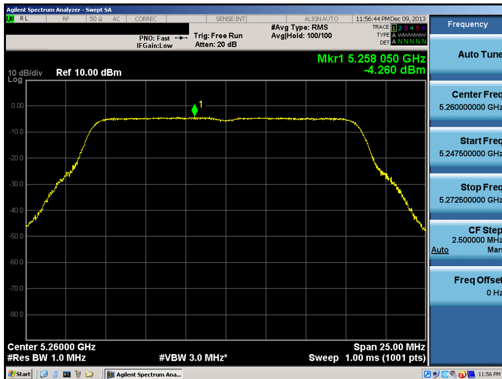
Plot 6-41. Peak Power Spectral Density Plot (802.11a (UNII Band 2A) – Ch. 52)
