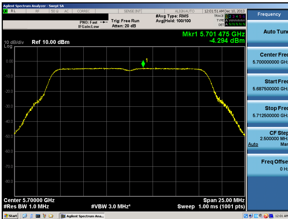
Plot 6-52. Peak Power Spectral Density Plot (802.11a (UNII Band 2C) – Ch. 140)
