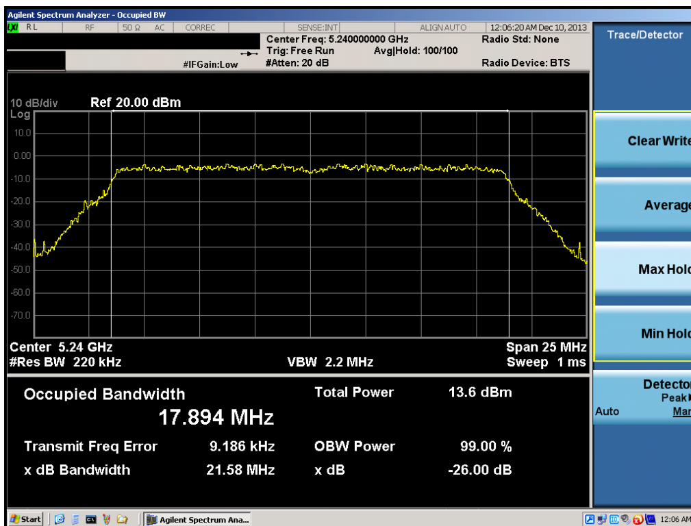
Plot 6-6. 26dB Bandwidth Plot (20MHz BW 802.11n (UNII Band 1) – Ch. 48)
