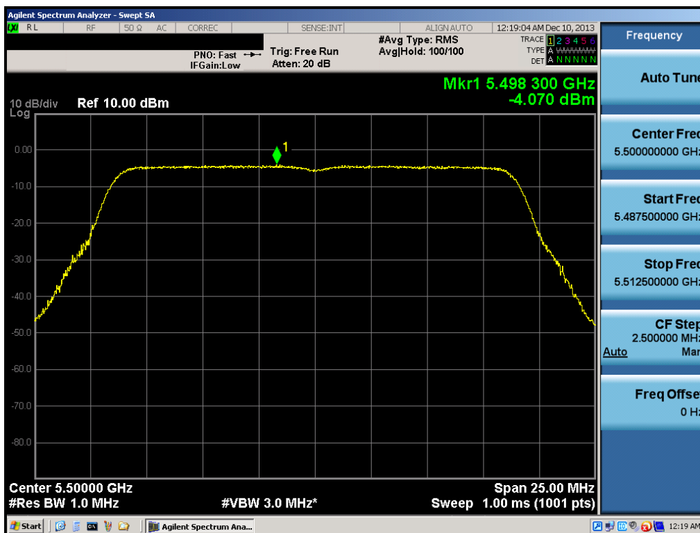
Plot 6-53. Peak Power Spectral Density Plot (20MHz BW 802.11n (UNII Band 2C) – Ch. 100)
