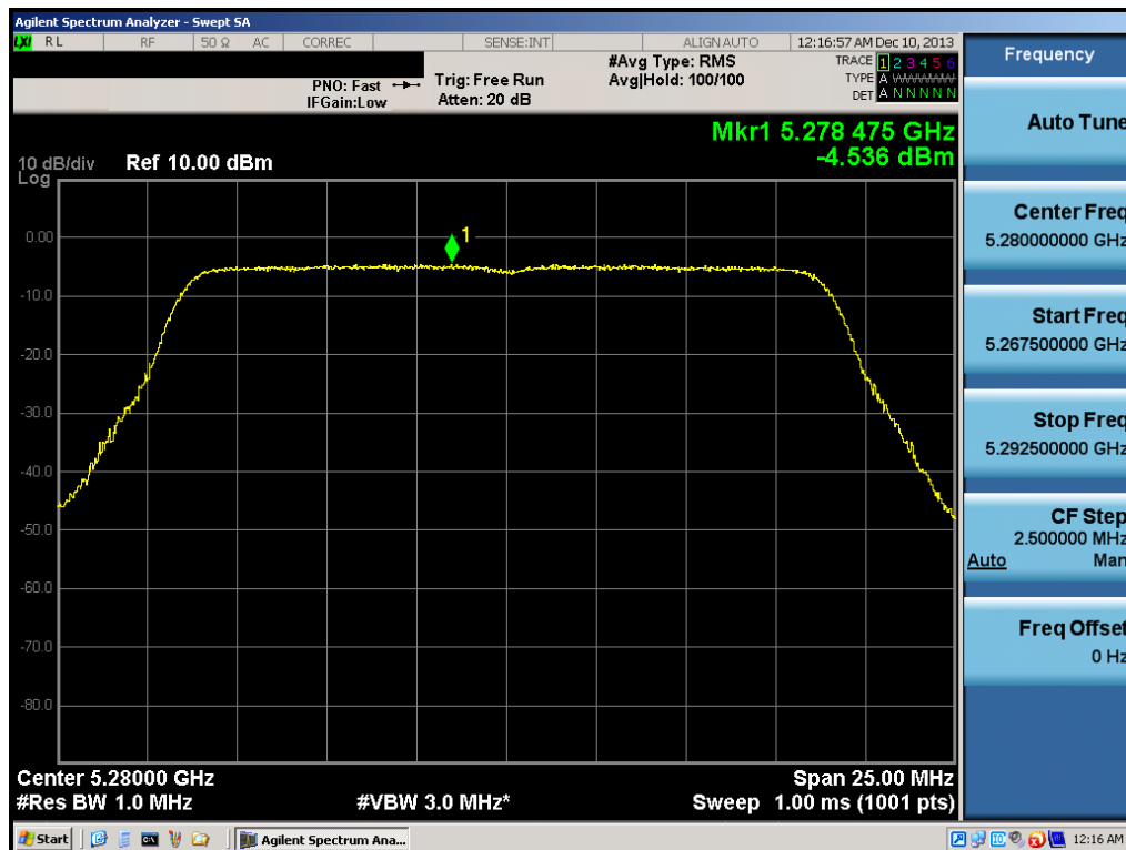
Plot 6-45. Peak Power Spectral Density Plot (20MHz BW 802.11n (UNII Band 2A) – Ch. 56)
