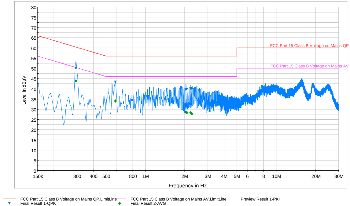
Plot 6-84. Line Conducted Plot with 802.11a UNII Band 1 (L1)
