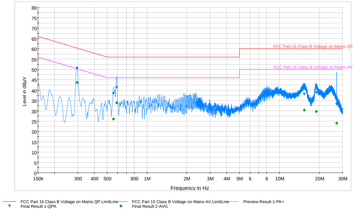
Plot 6-89. Line Conducted Plot with 802.11a UNII Band 2C (N)
