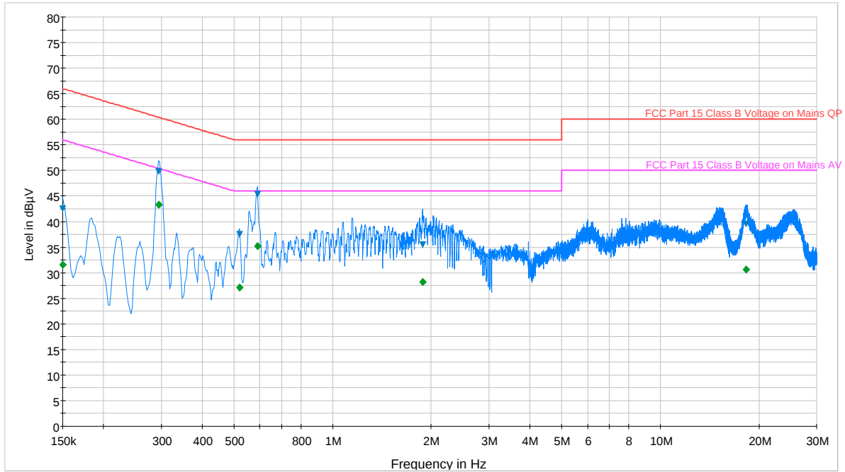
Plot 6-88. Line Conducted Plot with 802.11a UNII Band 2C (L1)
