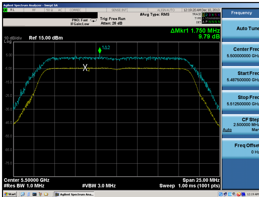
Plot 6-61. Peak Excursion Ratio Plot (20MHz BW 802.11n)
