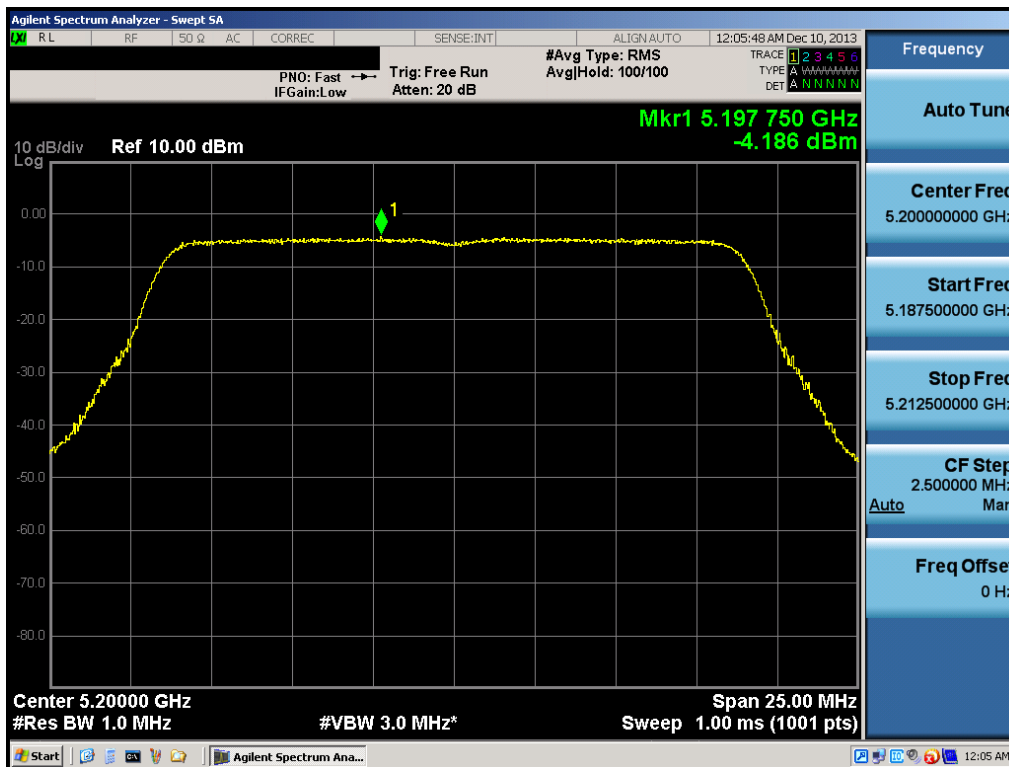
Plot 6-36. Peak Power Spectral Density Plot (20MHz BW 802.11n (UNII Band 1) – Ch. 40)
