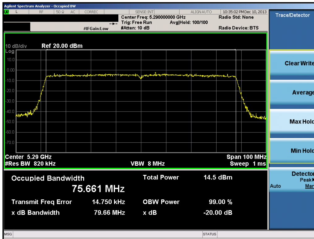
Plot 6-31. 20dB Bandwidth Plot (80MHz BW 802.11ac (UNII Band 2A) – Ch. 58)
