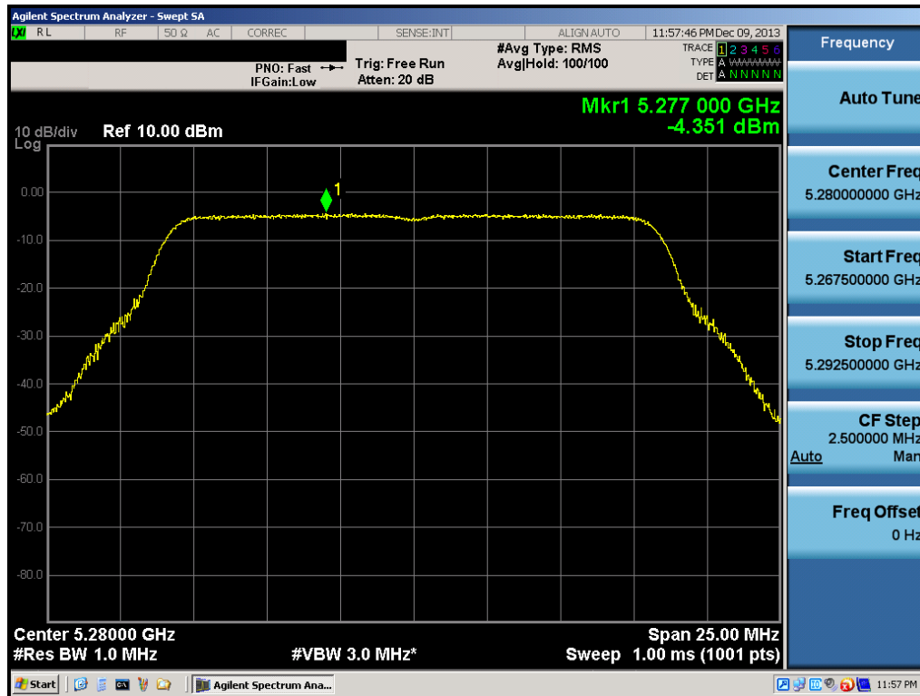
Plot 6-42. Peak Power Spectral Density Plot (802.11a (UNII Band 2A) – Ch. 56)
