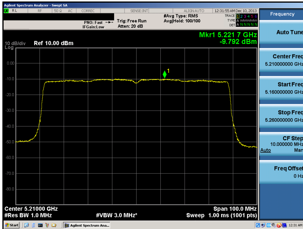
Plot 6-40. Peak Power Spectral Density Plot (80MHz BW 802.11ac (UNII Band 1) – Ch. 42)
