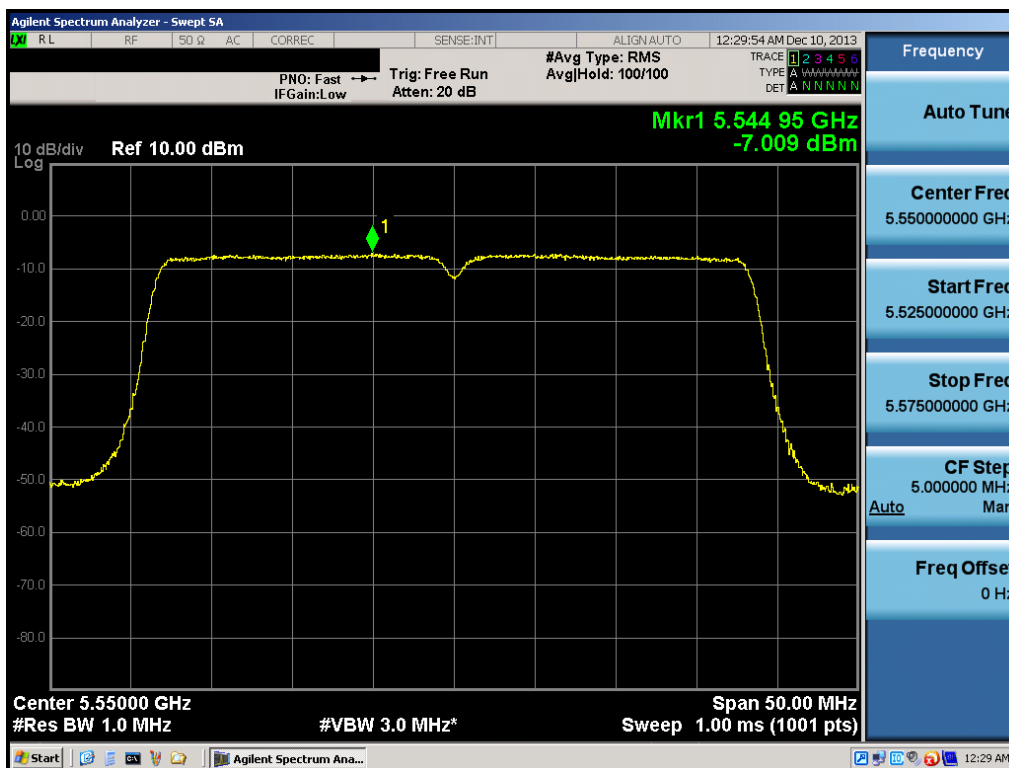
Plot 6-57. Peak Power Spectral Density Plot (40MHz BW 802.11n (UNII Band 2C) – Ch. 110)
