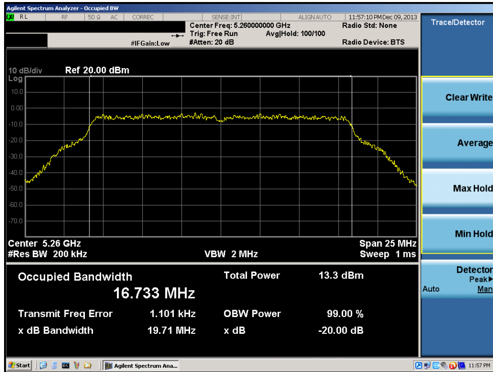
Plot 6-29. 20dB Bandwidth Plot (20MHz BW 802.11a (UNII Band 2A) – Ch. 52)
