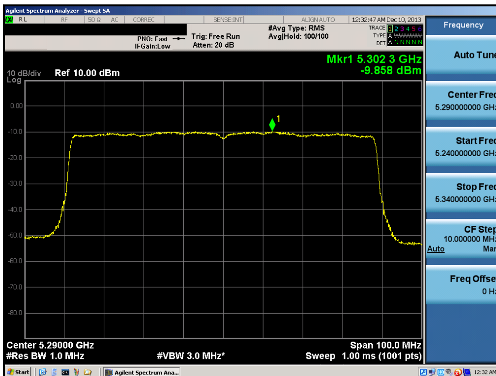
Plot 6-49. Peak Power Spectral Density Plot (80MHz BW 802.11ac (UNII Band 2A) – Ch. 58)
