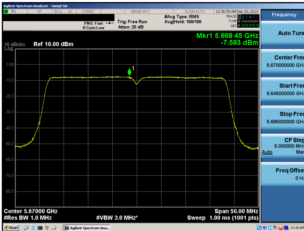
Plot 6-58. Peak Power Spectral Density Plot (40MHz BW 802.11n (UNII Band 2C) – Ch. 134)
