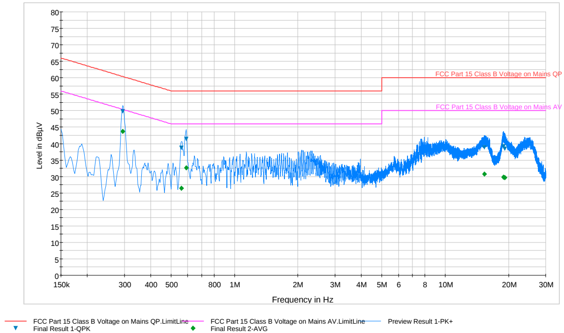
Plot 6-85. Line Conducted Plot with 802.11a UNII Band 1 (N)
