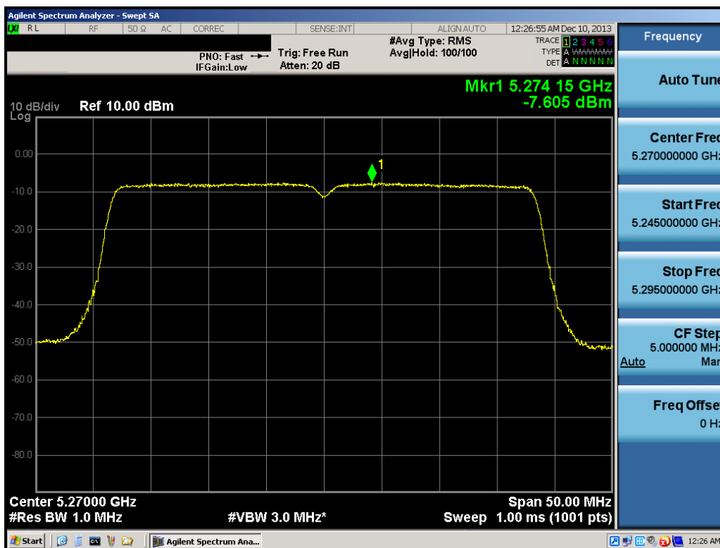
Plot 6-47. Peak Power Spectral Density Plot (40MHz BW 802.11n (UNII Band 2A) – Ch. 54)
