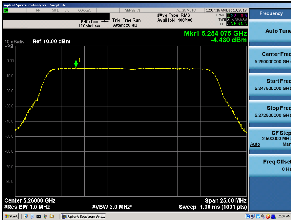
Plot 6-44. Peak Power Spectral Density Plot (20MHz BW 802.11n (UNII Band 2A) – Ch. 52)
