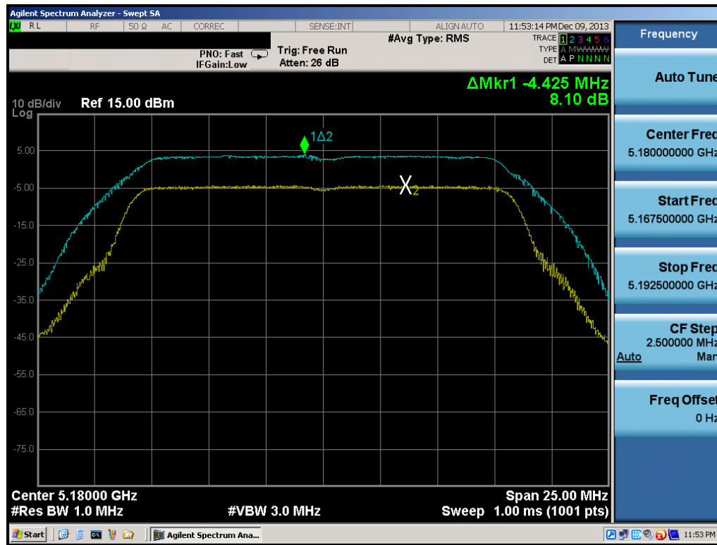
Plot 6-60. Peak Excursion Ratio Plot (802.11a)
