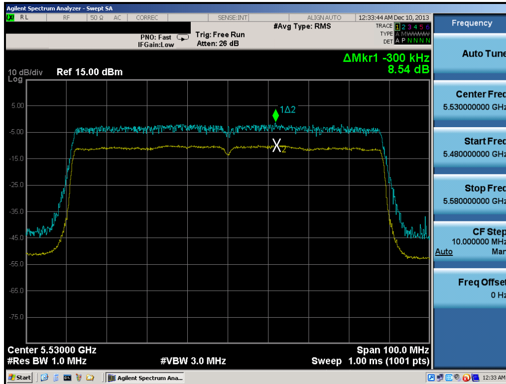
Plot 6-63. Peak Excursion Ratio Plot (80MHz BW 802.11ac)
