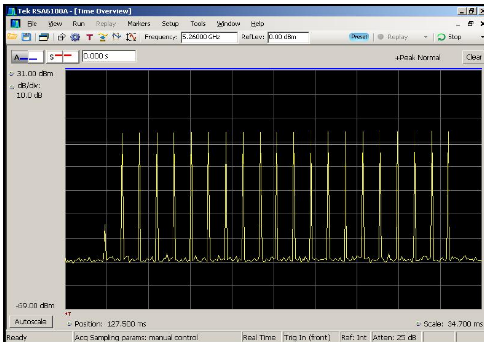
Figure 5-1. Type 1 Radar Pulse
