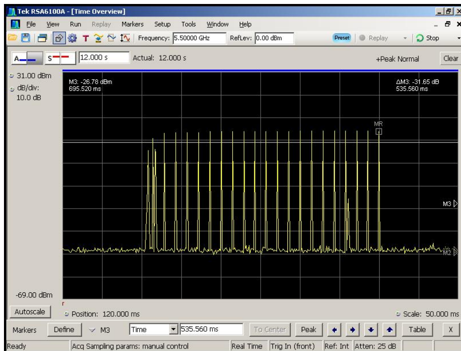
Figure 6-1. Type 1 Radar Pulse
