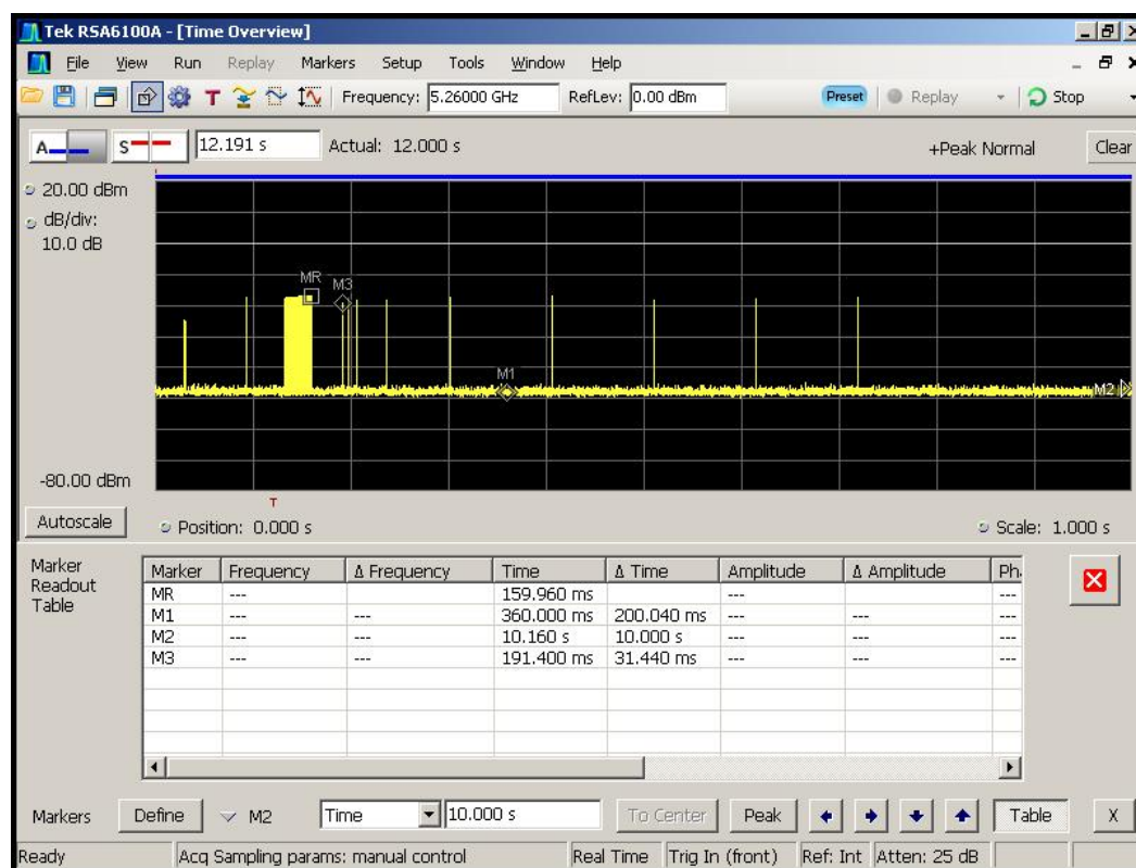
Figure 5-5. Aggregate Time using Pulse Table Capability
