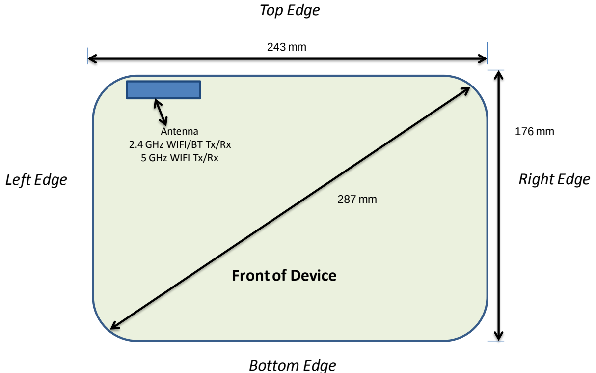
Figure 1-1 DUT Antenna Locations
