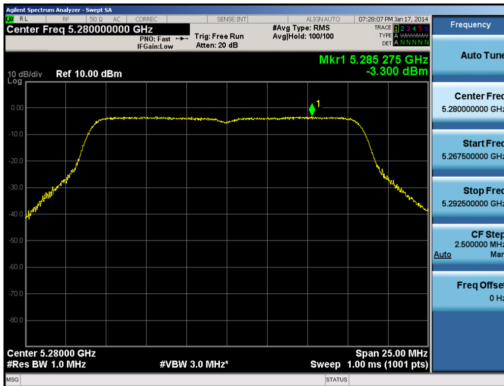
Plot 6-40. Peak Power Spectral Density Plot (802.11a (UNII Band 2A) – Ch. 56)
