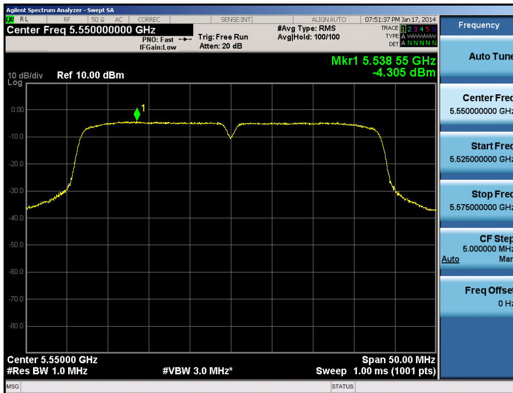
Plot 6-54. Peak Power Spectral Density Plot (40MHz BW 802.11n (UNII Band 2C) – Ch. 110)
