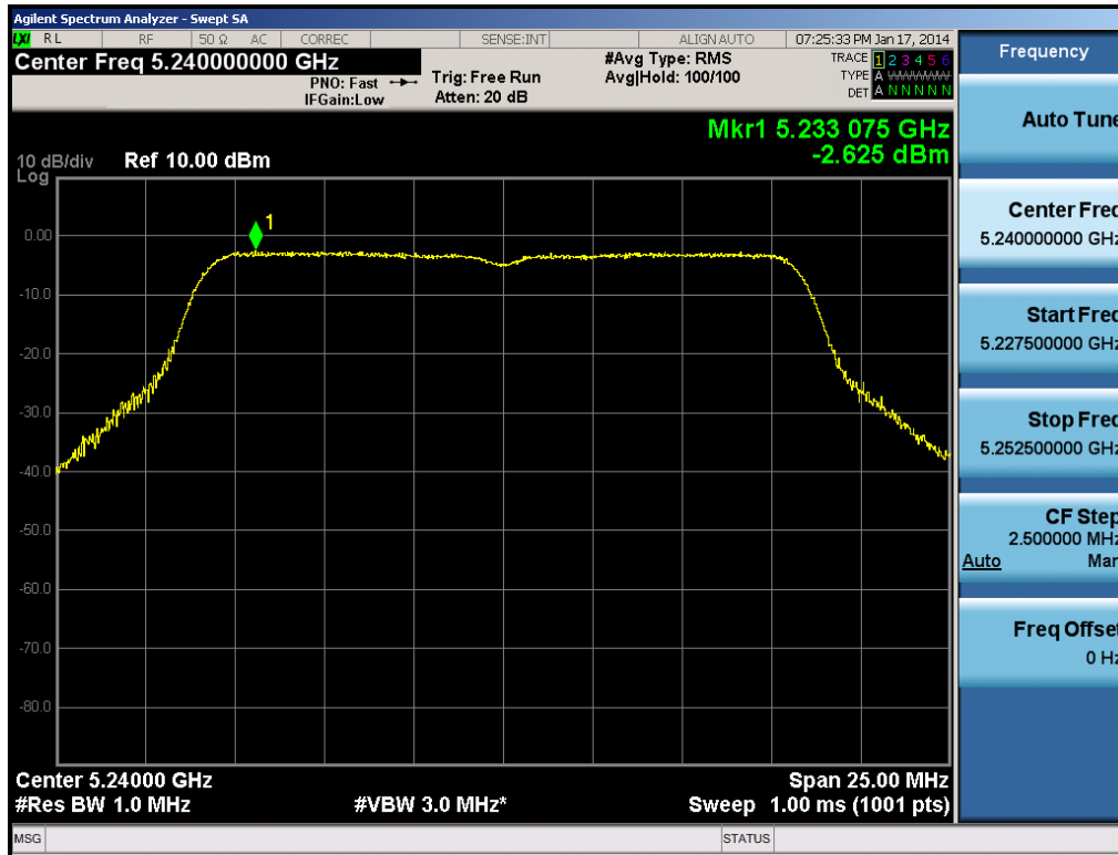
Plot 6-33. Peak Power Spectral Density Plot (802.11a (UNII Band 1) – Ch. 48)
