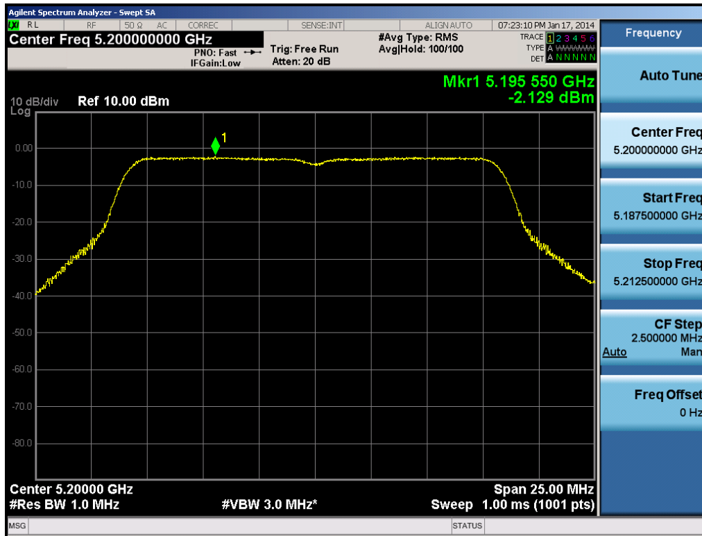
Plot 6-32. Peak Power Spectral Density Plot (802.11a (UNII Band 1) – Ch. 40)
