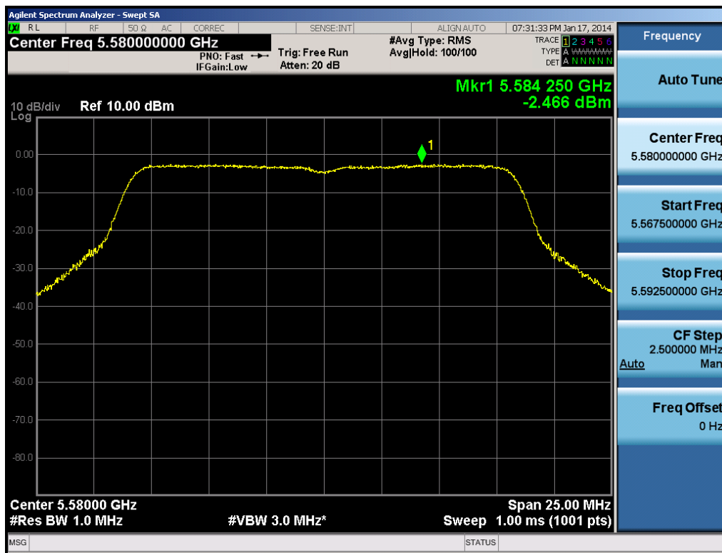
Plot 6-48. Peak Power Spectral Density Plot (802.11a (UNII Band 2C) – Ch. 116)
