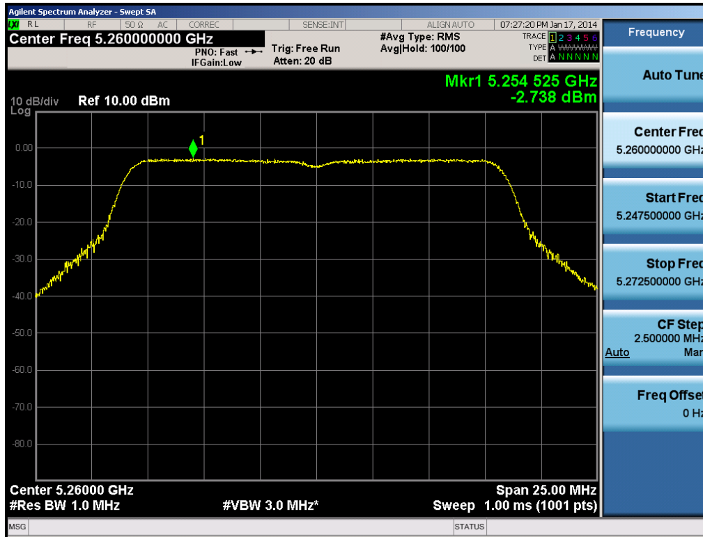
Plot 6-39. Peak Power Spectral Density Plot (802.11a (UNII Band 2A) – Ch. 52)
