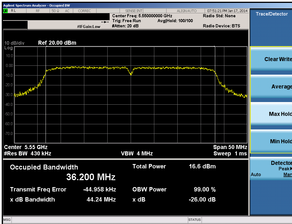
Plot 6-24. 26dB Bandwidth Plot (40MHz BW 802.11n (UNII Band 2C) – Ch. 110)
