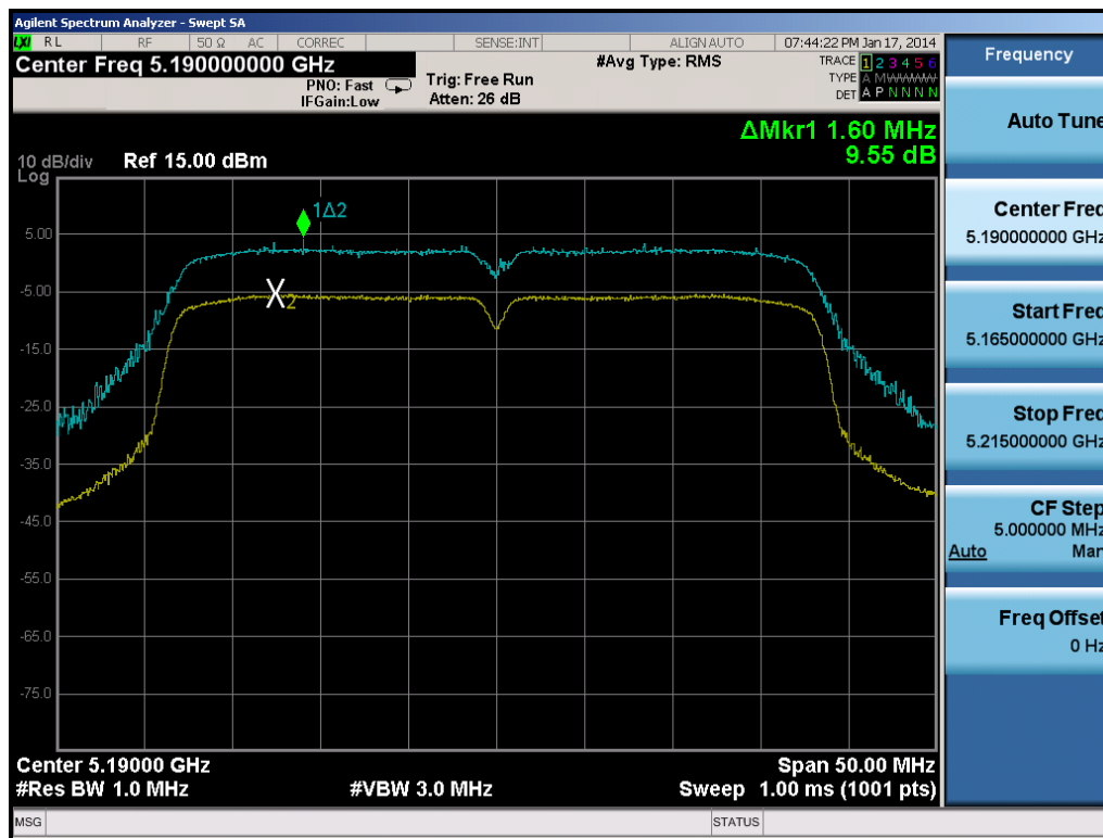
Plot 6-58. Peak Excursion Ratio Plot (40MHz BW 802.11n)
