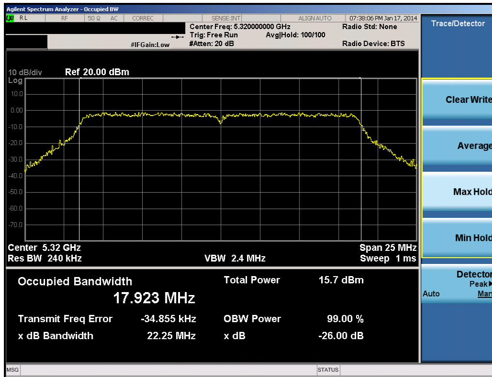
Plot 6-14. 26dB Bandwidth Plot (20MHz BW 802.11n (UNII Band 2A) – Ch. 64)
