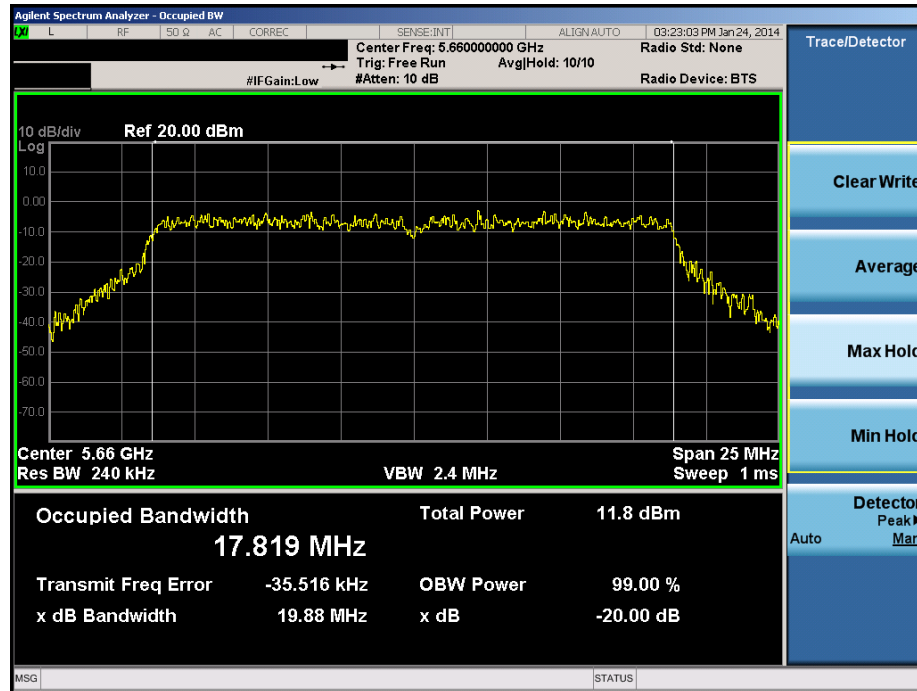
Plot 6-29. 20dB Bandwidth Plot (20MHz BW 802.11n (UNII Band 2C) – Ch. 132)
