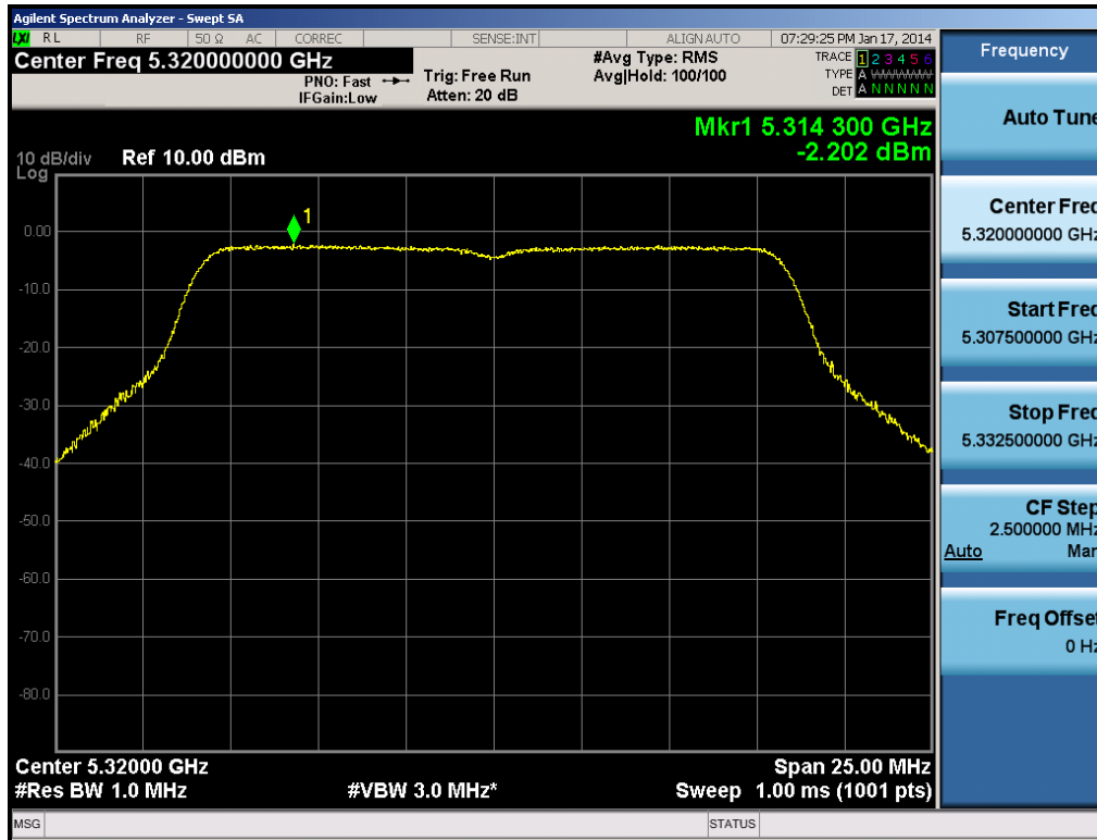
Plot 6-41. Peak Power Spectral Density Plot (802.11a (UNII Band 2A) – Ch. 64)
