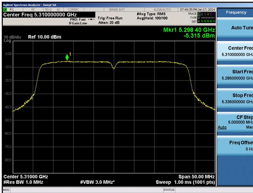
Plot 6-46. Peak Power Spectral Density Plot (40MHz BW 802.11n (UNII Band 2A) – Ch. 62)
