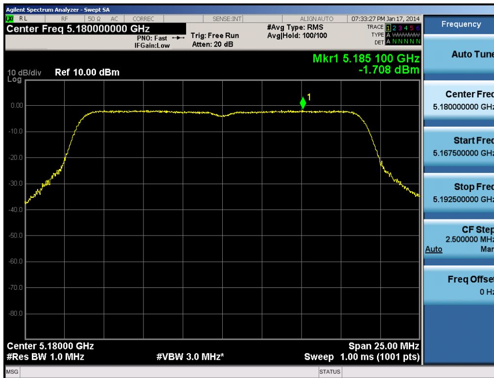
Plot 6-34. Peak Power Spectral Density Plot (20MHz BW 802.11n (UNII Band 1) – Ch. 36)
