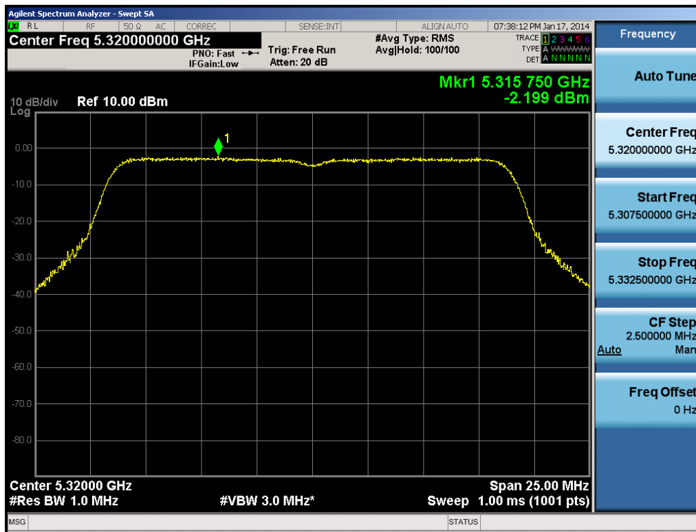
Plot 6-44. Peak Power Spectral Density Plot (20MHz BW 802.11n (UNII Band 2A) – Ch. 64)
