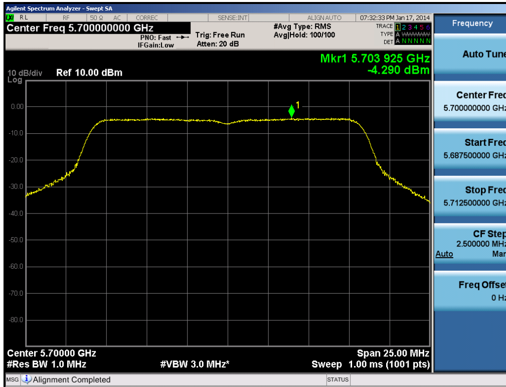
Plot 6-49. Peak Power Spectral Density Plot (802.11a (UNII Band 2C) – Ch. 140)
