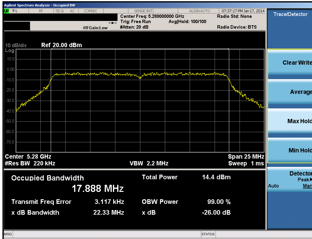
Plot 6-13. 26dB Bandwidth Plot (20MHz BW 802.11n (UNII Band 2A) – Ch. 56)
