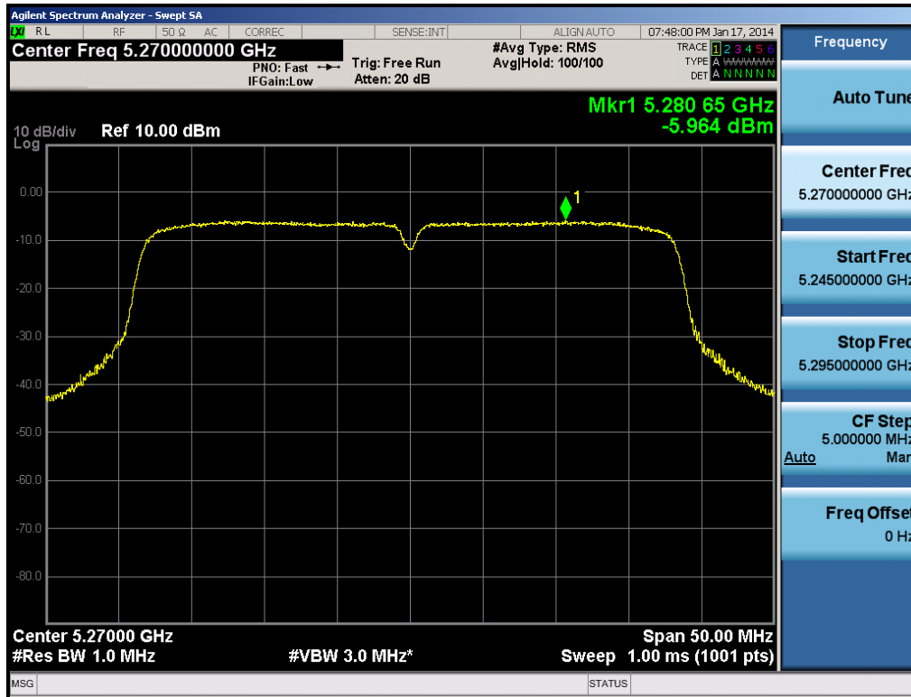
Plot 6-45. Peak Power Spectral Density Plot (40MHz BW 802.11n (UNII Band 2A) – Ch. 54)
