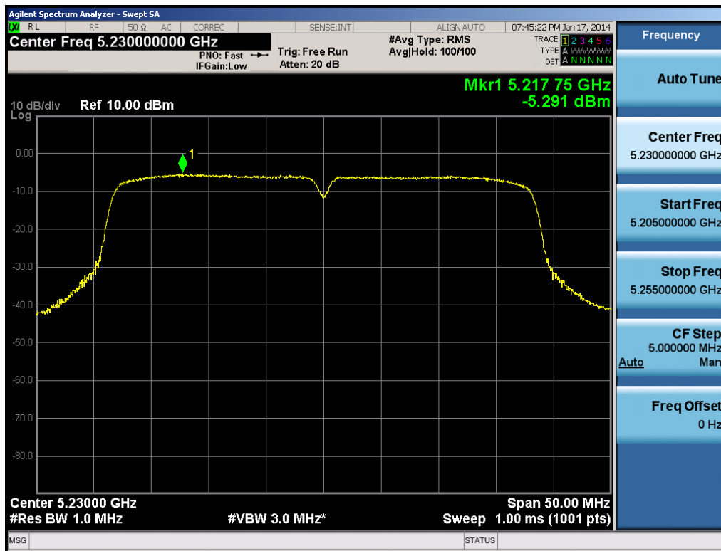
Plot 6-38. Peak Power Spectral Density Plot (40MHz BW 802.11n (UNII Band 1) – Ch. 46)
