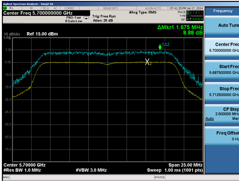
Plot 6-57. Peak Excursion Ratio Plot (20MHz BW 802.11n)
