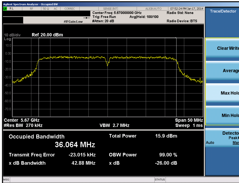
Plot 6-25. 26dB Bandwidth Plot (40MHz BW 802.11n (UNII Band 2C) – Ch. 134)
