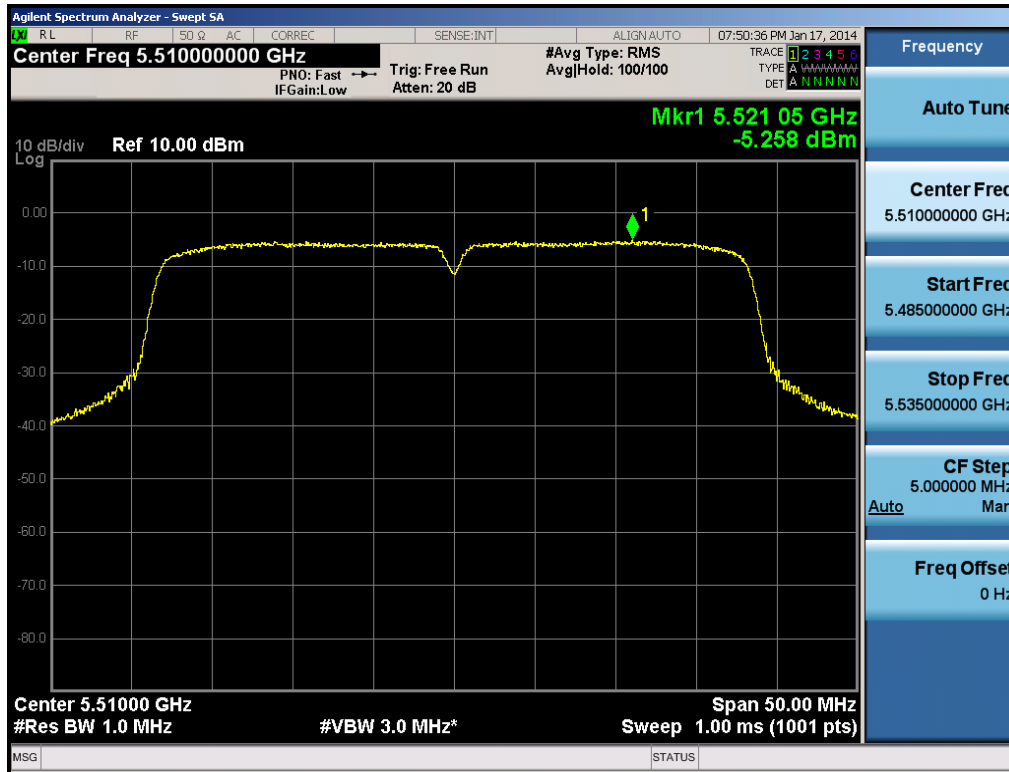
Plot 6-53. Peak Power Spectral Density Plot (40MHz BW 802.11n (UNII Band 2C) – Ch. 102)
