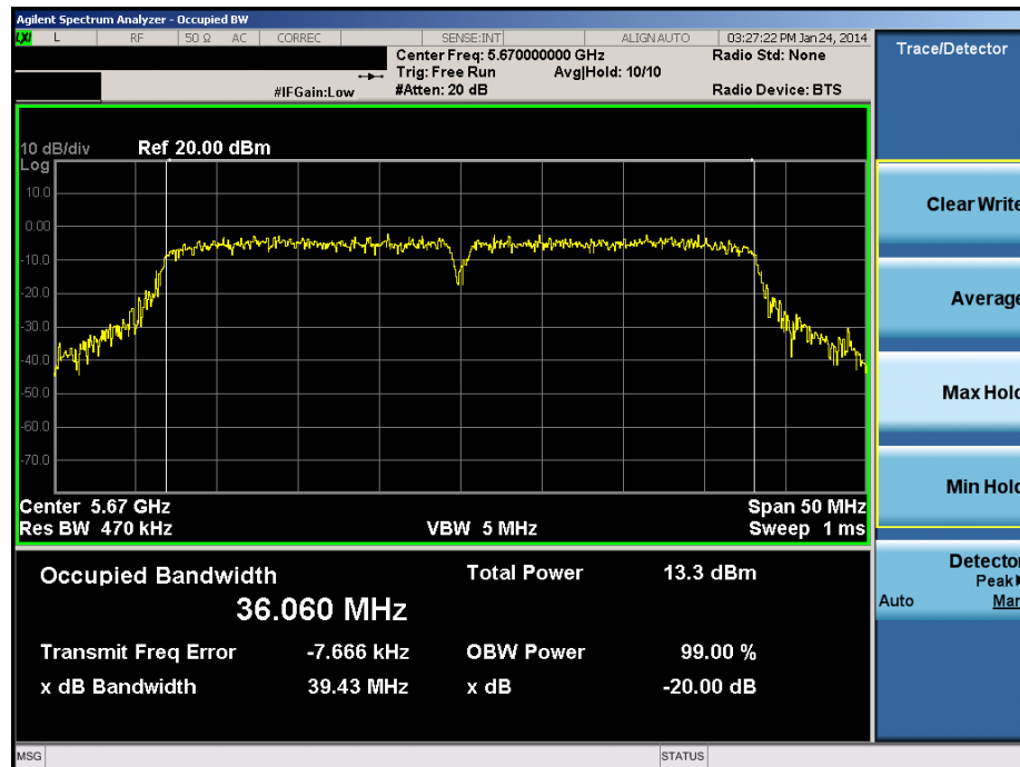
Plot 6-30. 20dB Bandwidth Plot (40MHz BW 802.11a/n UNII Band 2C) – Ch. 134)
