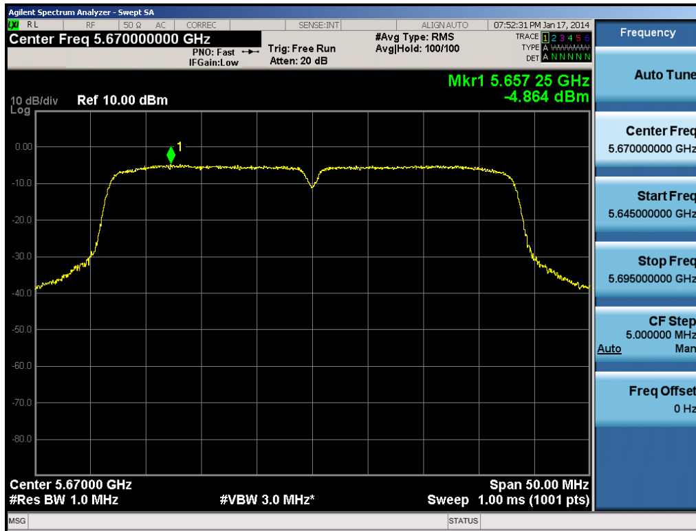
Plot 6-55. Peak Power Spectral Density Plot (40MHz BW 802.11n (UNII Band 2C) – Ch. 134)
