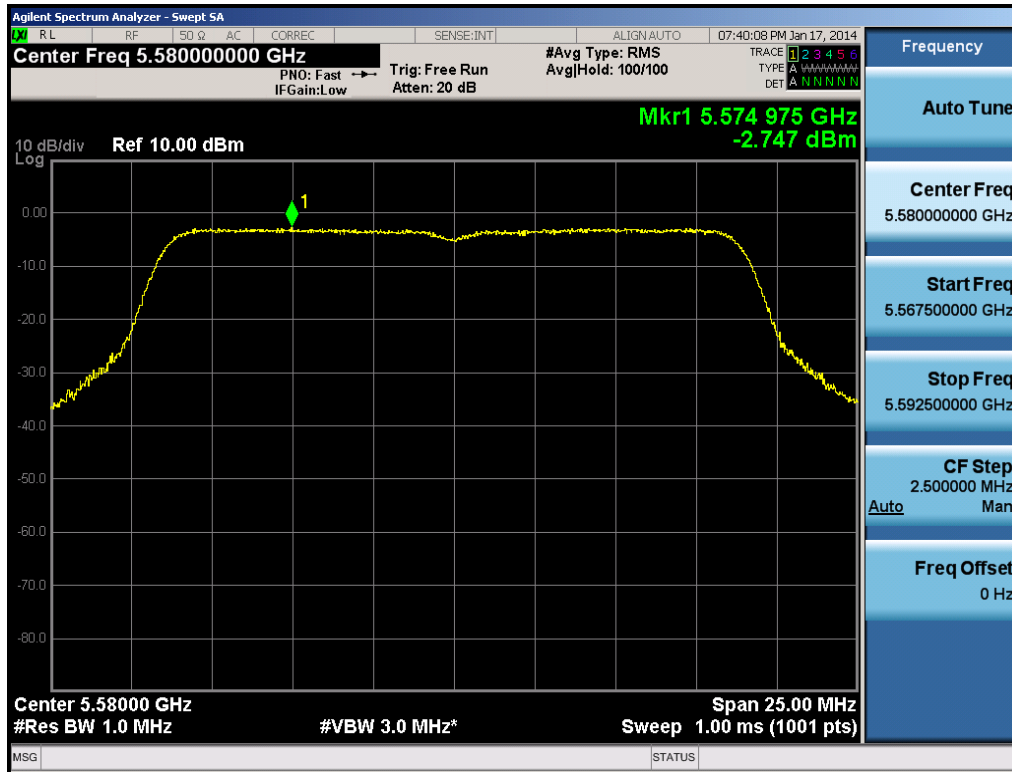
Plot 6-51. Peak Power Spectral Density Plot (20MHz BW 802.11n (UNII Band 2C) – Ch. 116)
