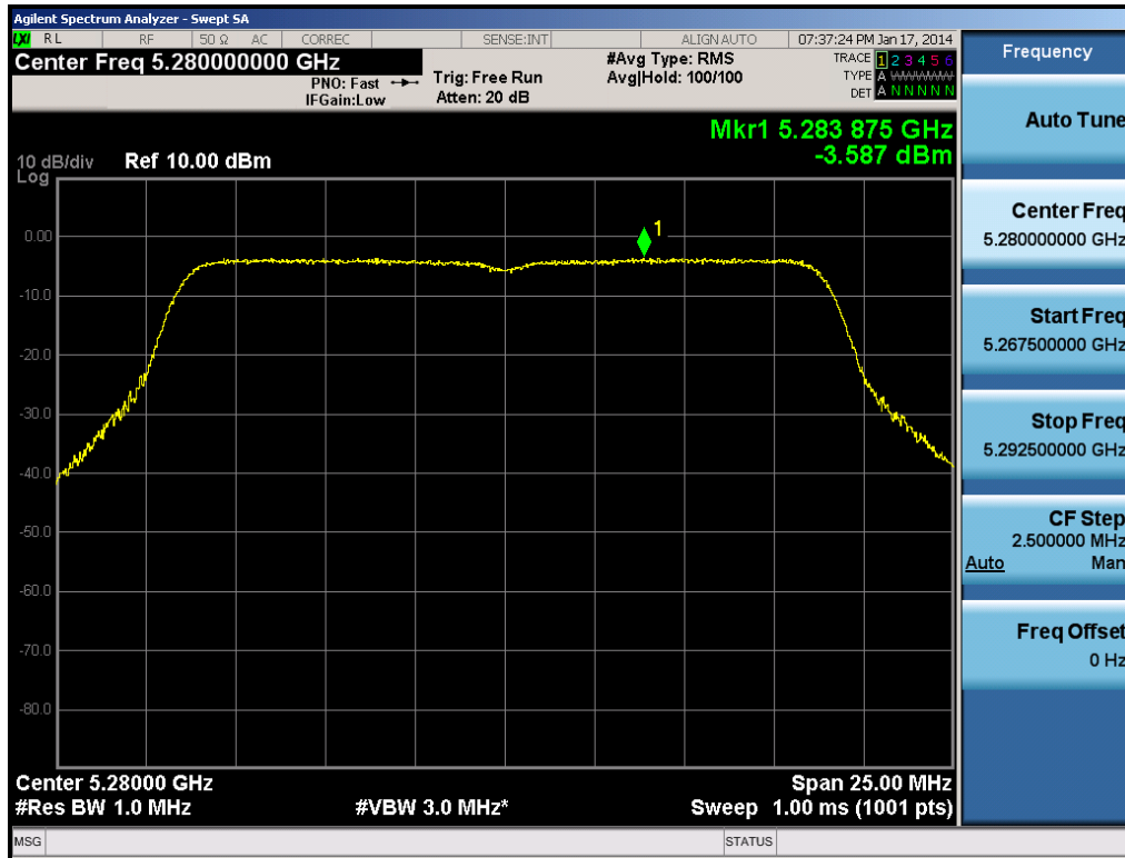
Plot 6-43. Peak Power Spectral Density Plot (20MHz BW 802.11n (UNII Band 2A) – Ch. 56)
