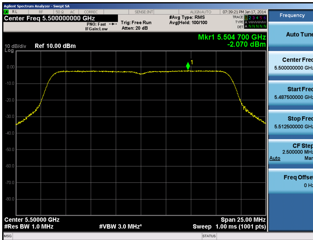
Plot 6-50. Peak Power Spectral Density Plot (20MHz BW 802.11n (UNII Band 2C) – Ch. 100)
