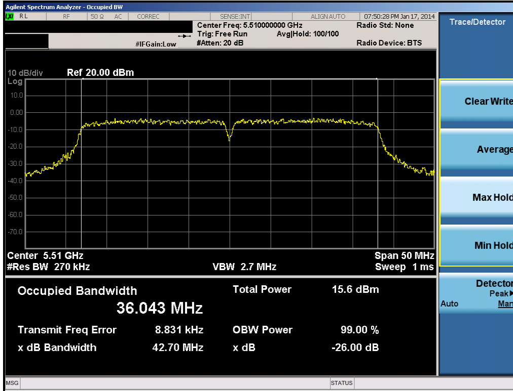
Plot 6-23. 26dB Bandwidth Plot (40MHz BW 802.11n (UNII Band 2C) – Ch. 102)
