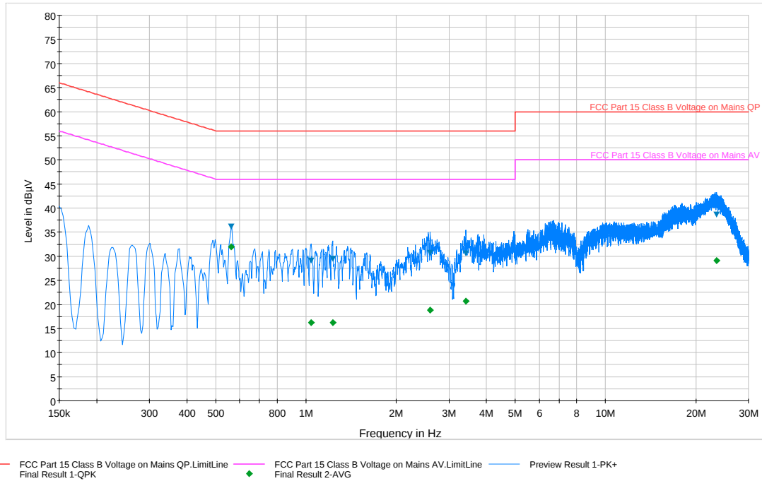
Plot 6-73. Line Conducted Plot with 802.11a UNII Band 1 (L1)
