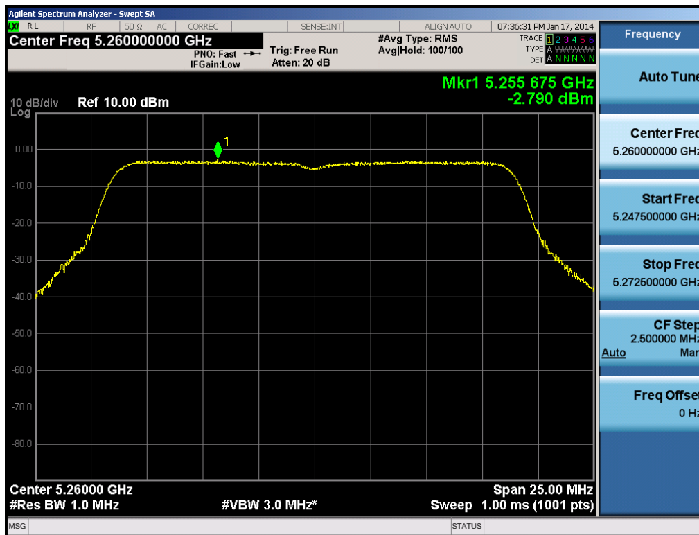
Plot 6-42. Peak Power Spectral Density Plot (20MHz BW 802.11n (UNII Band 2A) – Ch. 52)
