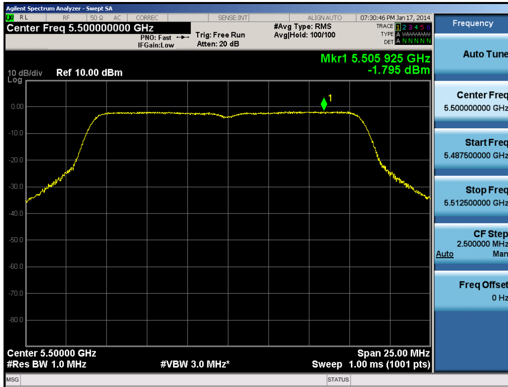
Plot 6-47. Peak Power Spectral Density Plot (802.11a (UNII Band 2C) – Ch. 100)
