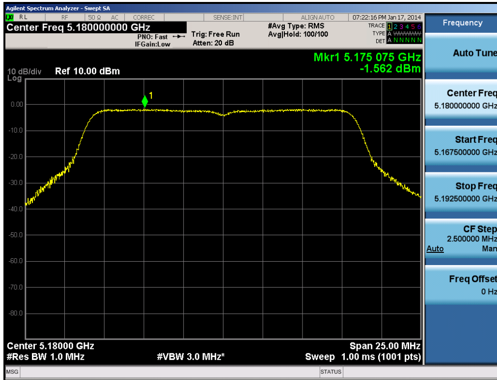
Plot 6-31. Peak Power Spectral Density Plot (802.11a (UNII Band 1) – Ch. 36)
