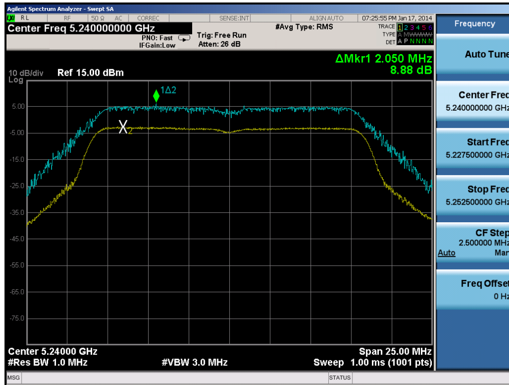
Plot 6-56. Peak Excursion Ratio Plot (802.11a)
