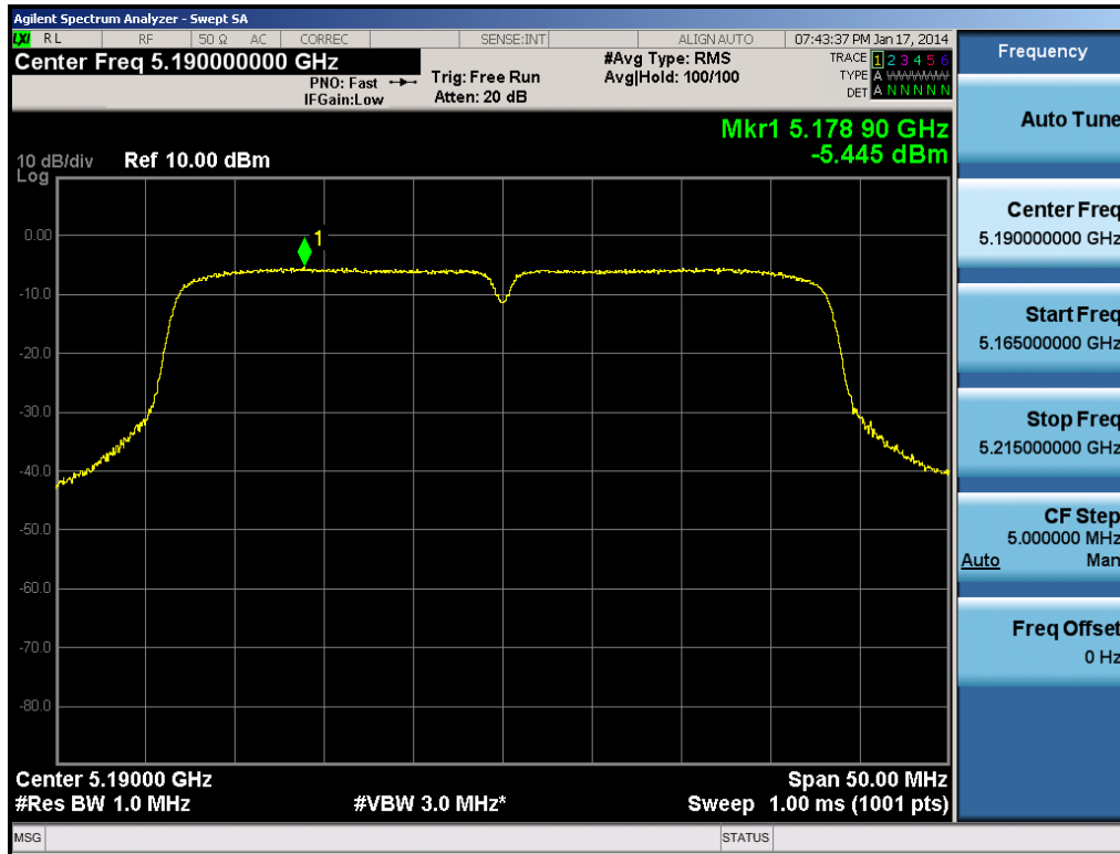
Plot 6-37. Peak Power Spectral Density Plot (40MHz BW 802.11n (UNII Band 1) – Ch. 38)
