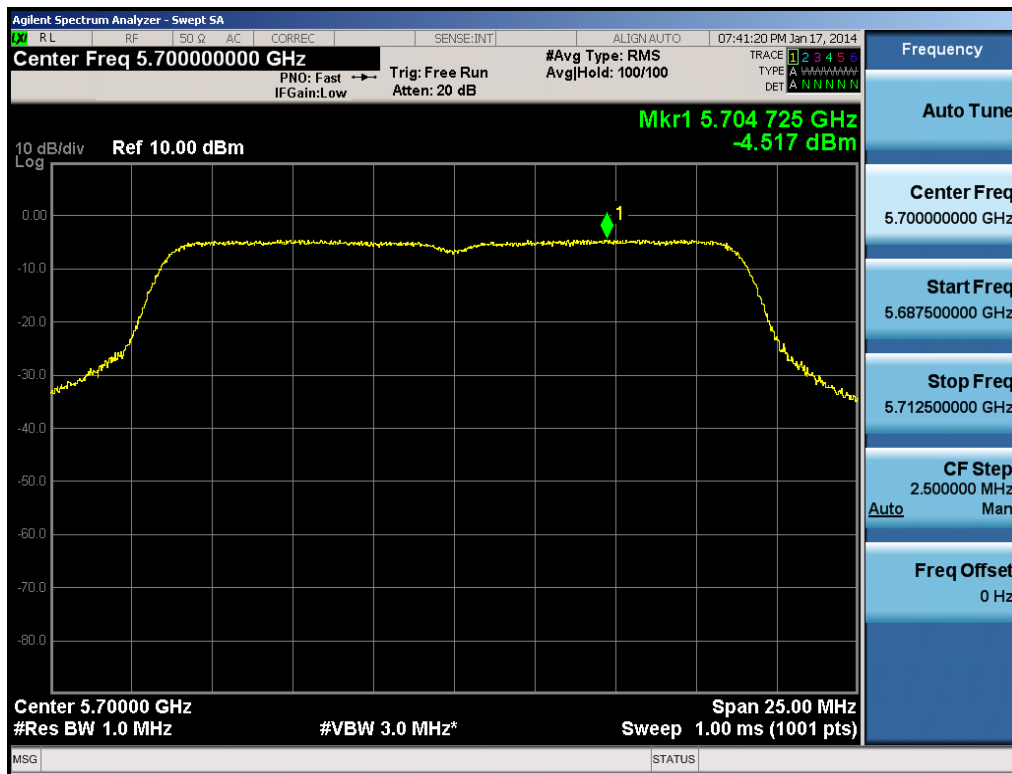
Plot 6-52. Peak Power Spectral Density Plot (20MHz BW 802.11n (UNII Band 2C) – Ch. 140)
