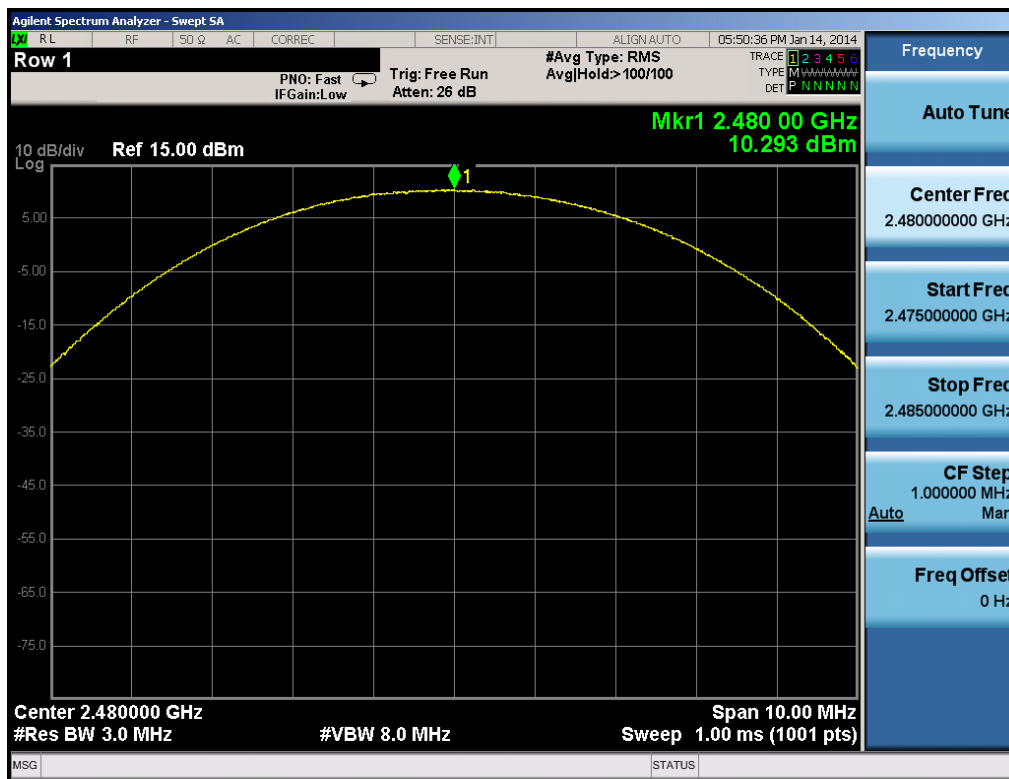
Plot 6-15. Peak Conducted Power (2Mbps – Ch. 78)
