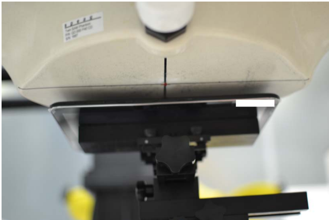
SAR Test Setup Photo 2: Back at 15.0 mm
