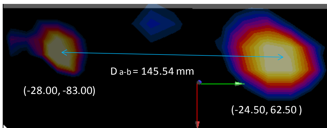
Figure 11-12 Peak SAR Locations of 5 GHz WLAN and LTE Band 2
