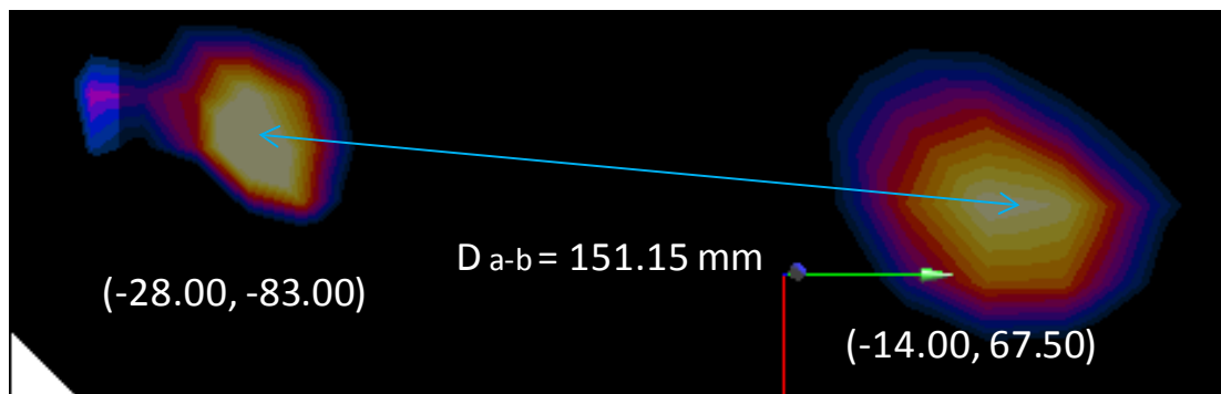
Figure 11-10 Peak SAR Locations of 5 GHz WLAN and GPRS 1900 MHz
