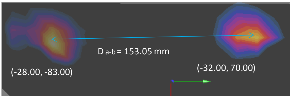
Figure 11-6 Peak SAR Locations of 5 GHz WLAN and GRPS 1900 MHz
