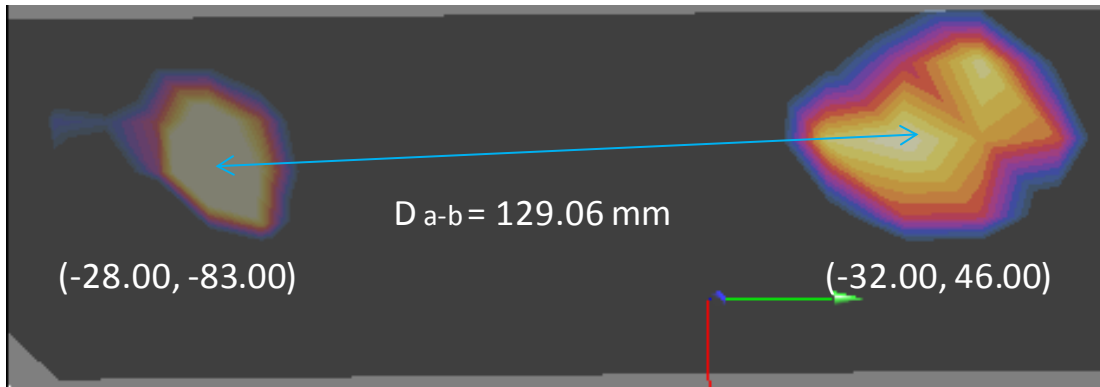
Figure 11-5 Peak SAR Locations of 5 GHz WLAN and UMTS 850 MHz
