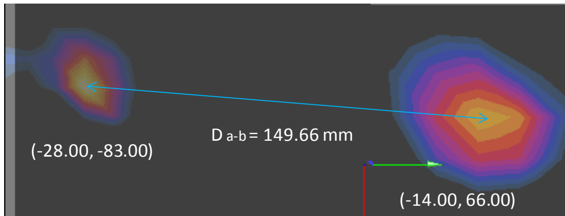
Figure 11-11 Peak SAR Locations of 5 GHz WLAN and UMTS 1900 MHz
