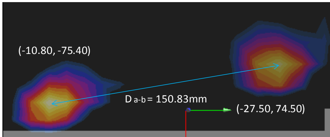
Figure 11-4 Peak SAR Locations of 2.4 GHz WLAN and LTE Band 2
