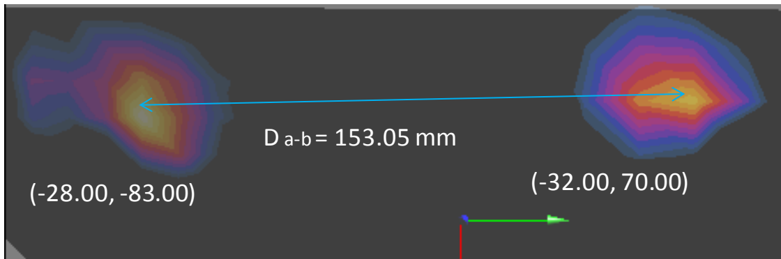
Figure 11-7 Peak SAR Locations of 5 GHz WLAN and UMTS 1900 MHz
