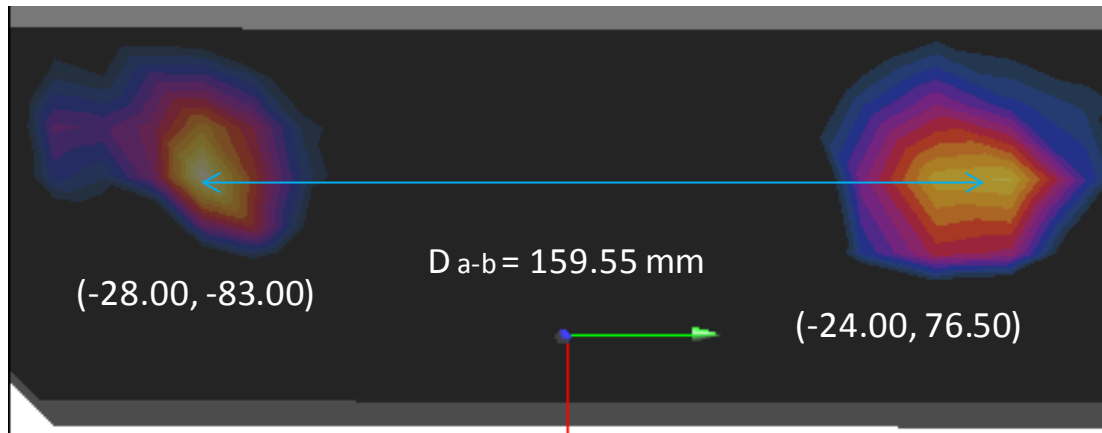
Figure 11-8 Peak SAR Locations of 5 GHz WLAN and LTE Band 4
