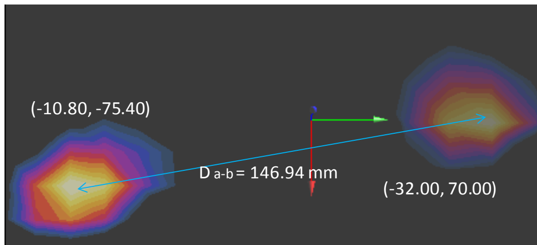
Figure 11-2 Peak SAR Locations of 2.4 GHz WLAN and UMTS 1900 MHz
