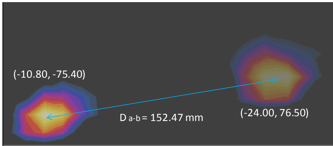
Figure 11-3 Peak SAR Locations of 2.4 GHz WLAN and LTE Band 4
