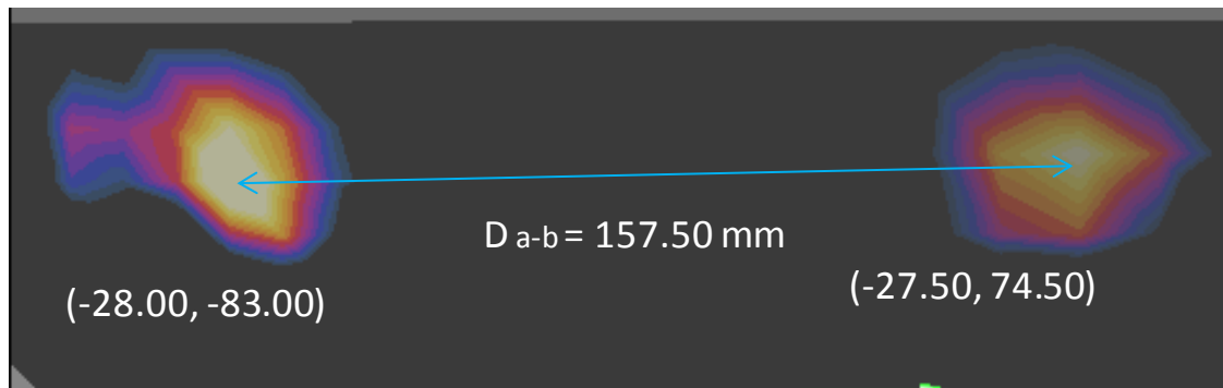
Figure 11-9 Peak SAR Locations of 5 GHz WLAN and LTE Band 2
