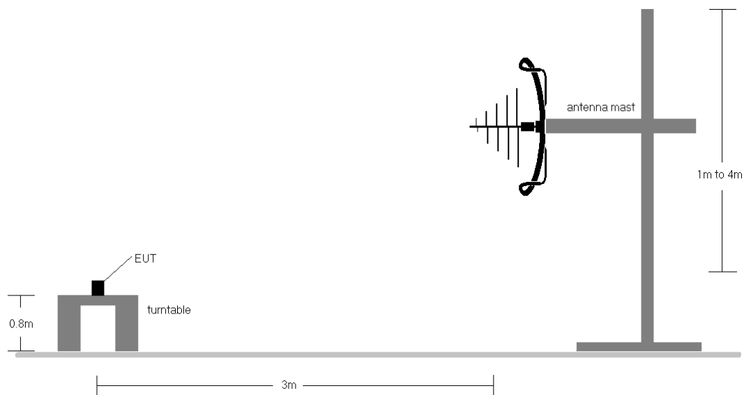
Figure 7-10. Radiated Test Setup <1000MHz
