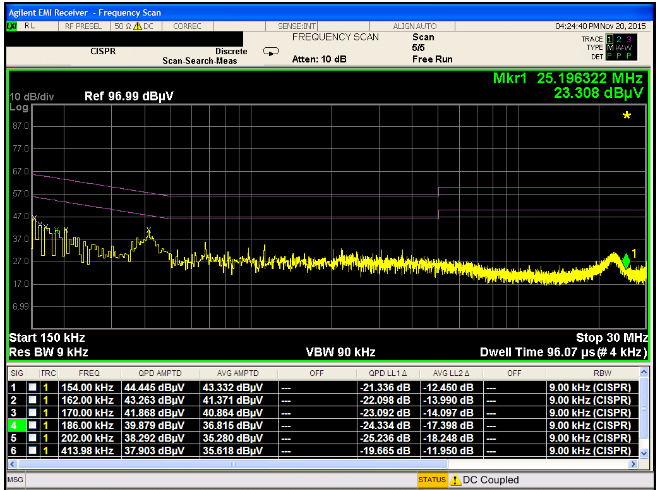
Plot 7-54. Line-Conducted Test Plot (L1)
