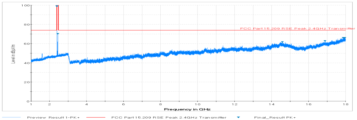
Plot 7-43. Radiated Spurious Plot above 1GHz (BT – Ch. 0, Ant. Pol. V)
