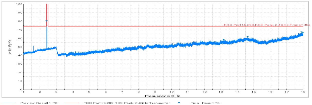
Plot 7-44. Radiated Spurious Plot above 1GHz (BT – Ch. 39, Ant. Pol. H)
