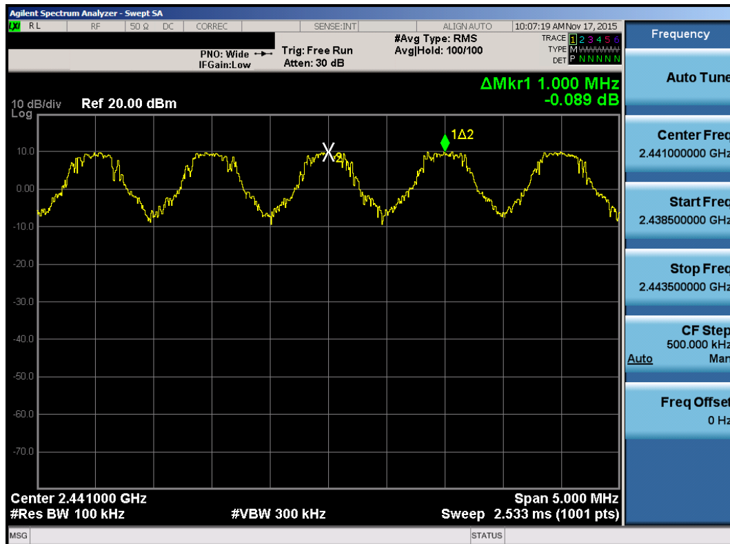
Plot 7-32. Channel Spacing Plot (Bluetooth)
