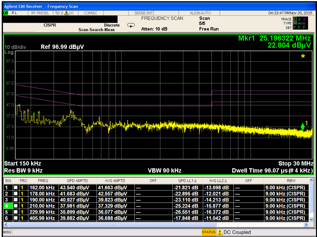
Plot 7-55. Line-Conducted Test Plot (N)
