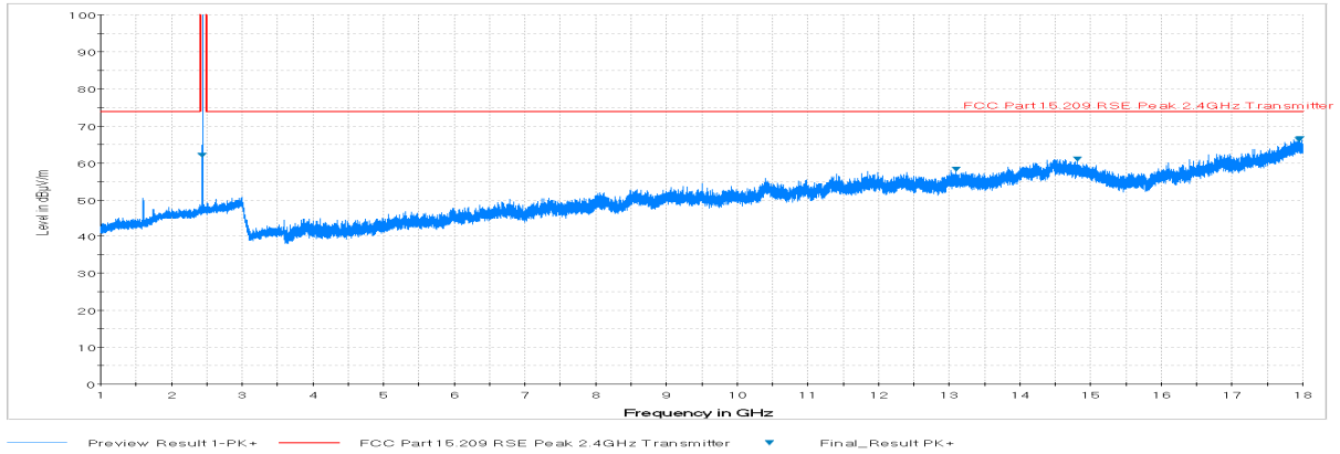
Plot 7-45. Radiated Spurious Plot above 1GHz (BT – Ch. 39, Ant. Pol. V)
