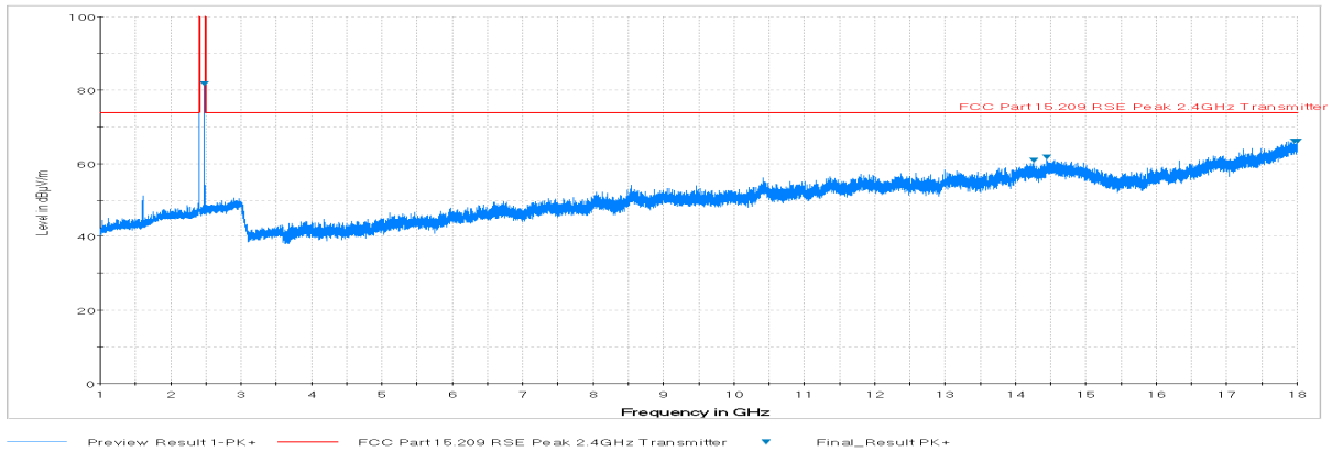
Plot 7-42. Radiated Spurious Plot above 1GHz (BT – Ch. 0, Ant. Pol. H)
