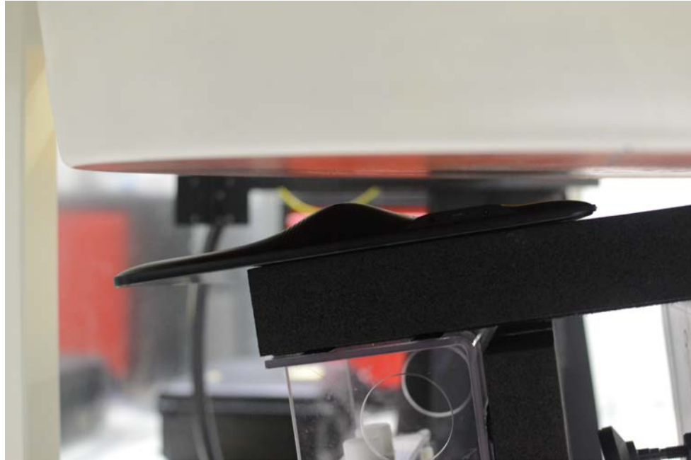
SAR Test Setup Photo 1 – Back Side (Bottom Touch, Main Antenna) at 1.4 cm
