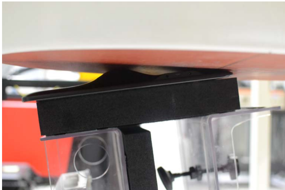
SAR Test Setup Photo 2 – Back Side (Bottom Touch, Main Antenna) at 0.0 cm
