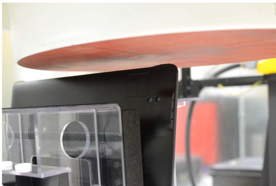
SAR Test Setup Photo 6 – Bottom Edge (Main Antenna) at 1.2 cm
