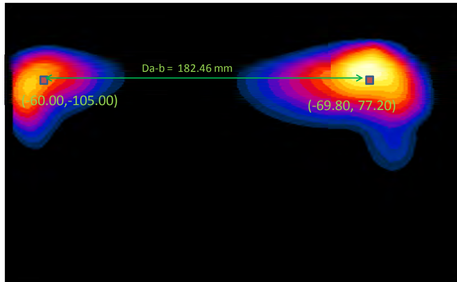
Figure 12-7 Peak SAR Locations of 2.4 GHz WLAN Ant. 2 and UMTS 1900 at 0 mm
