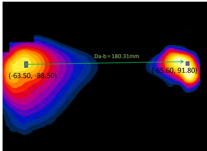
Figure 12-1 Peak SAR Locations of 2.4 GHz WLAN Ant. 1 and UMTS 850 at 0 mm
