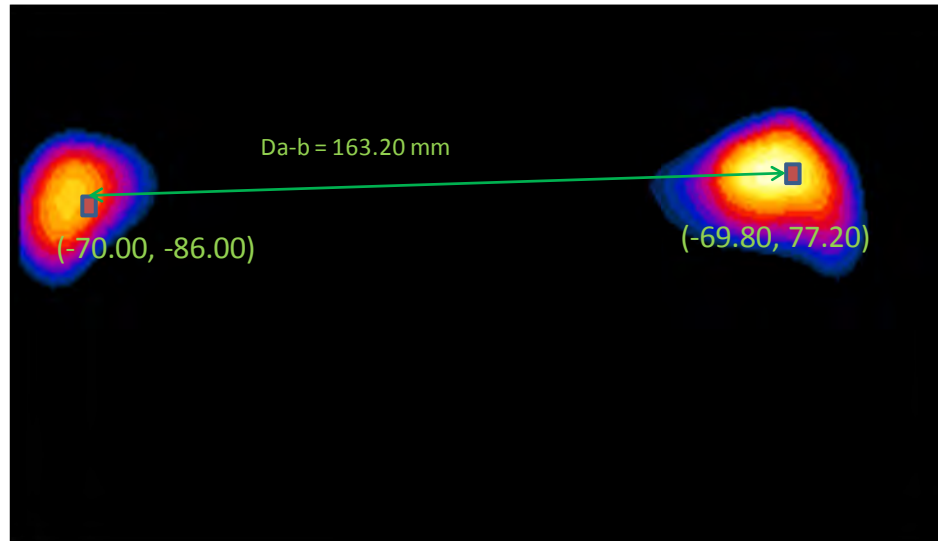
Figure 12-8 Peak SAR Locations of 2.4 GHz WLAN Ant. 2 and LTE Band 5 at 0 mm
