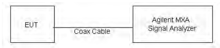
Figure 9-4 Power Measurement Setup for SISO Bandwidths > 50 MHz
