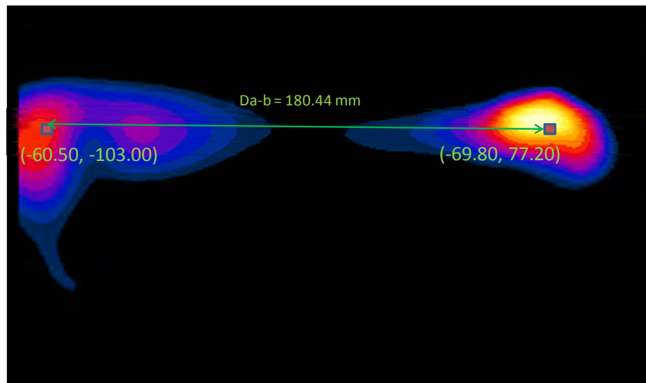
Figure 12-12 Peak SAR Locations of 2.4 GHz WLAN Ant. 2 and UMTS 1900 at 15 mm
