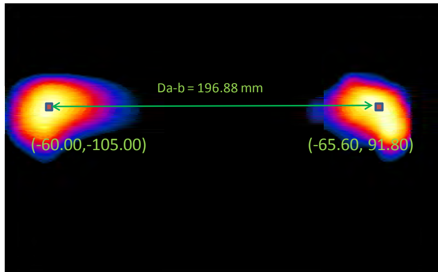
Figure 12-3 Peak SAR Locations of 2.4 GHz WLAN Ant. 1 and UMTS 1900 at 0 mm
