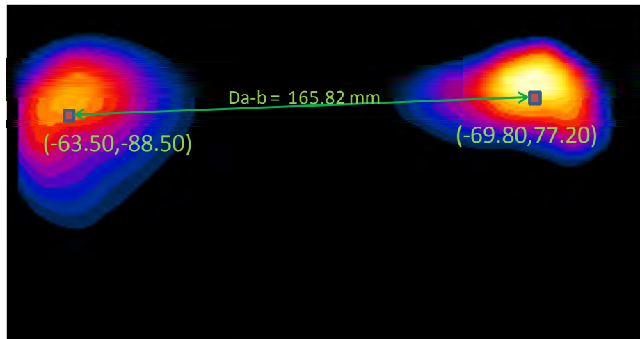
Figure 12-5 Peak SAR Locations of 2.4 GHz WLAN Ant. 2 and UMTS 850 at 0 mm
