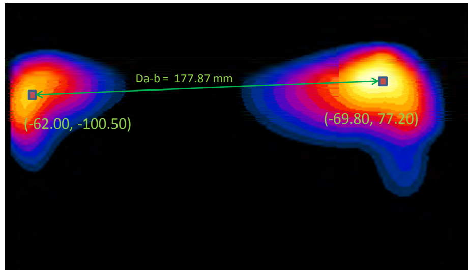
Figure 12-6 Peak SAR Locations of 2.4 GHz WLAN Ant. 2 and GPRS 1900 at 0 mm
