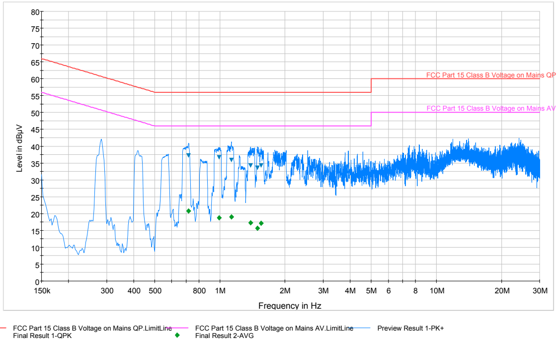
Plot 6-7. Line-Conducted Test Plot (N)
