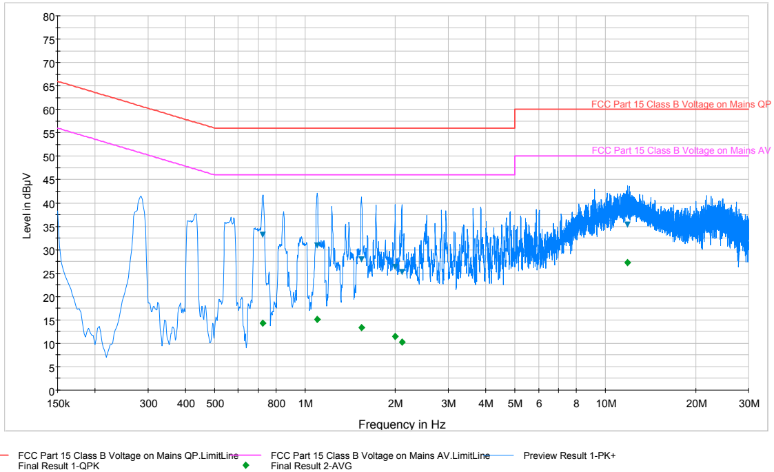
Plot 6-6. Line-Conducted Test Plot (L1)
