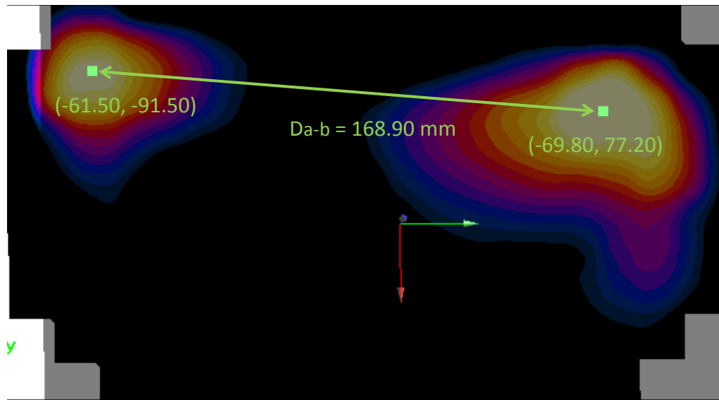
Figure 12-5 Peak SAR Locations of 2.4 GHz WLAN Ant. 2 and UMTS 1900 at 0 mm
