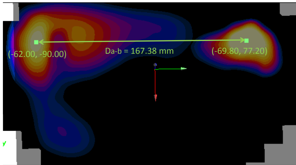
Figure 12-10 Peak SAR Locations of 2.4 GHz WLAN Ant. 2 and UMTS 1900 at 15 mm
