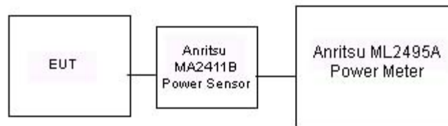
Figure 9-3 Power Measurement Setup for SISO Bandwidths < 50 MHz
