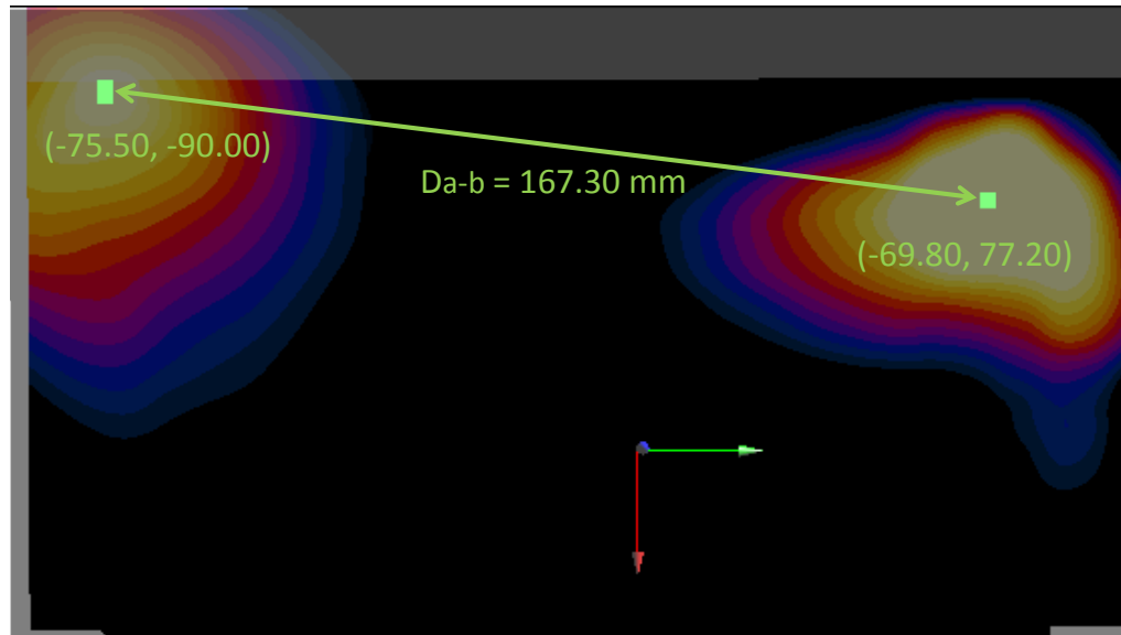
Figure 12-6 Peak SAR Locations of 2.4 GHz WLAN Ant. 2 and LTE B5 at 0 mm
