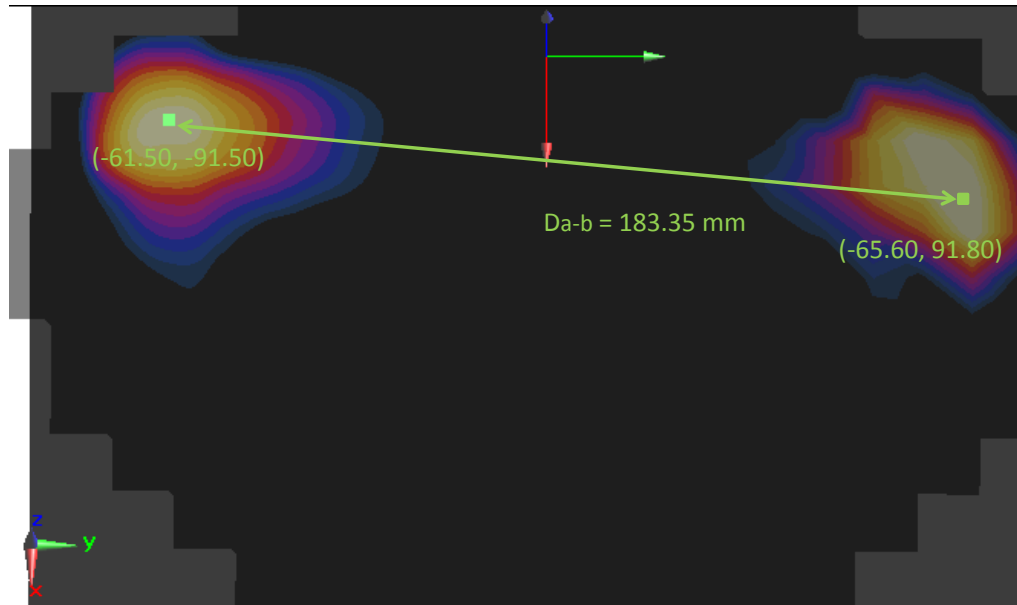
Figure 12-2 Peak SAR Locations of 2.4 GHz WLAN Ant. 1 and UMTS 1900 at 0 mm
