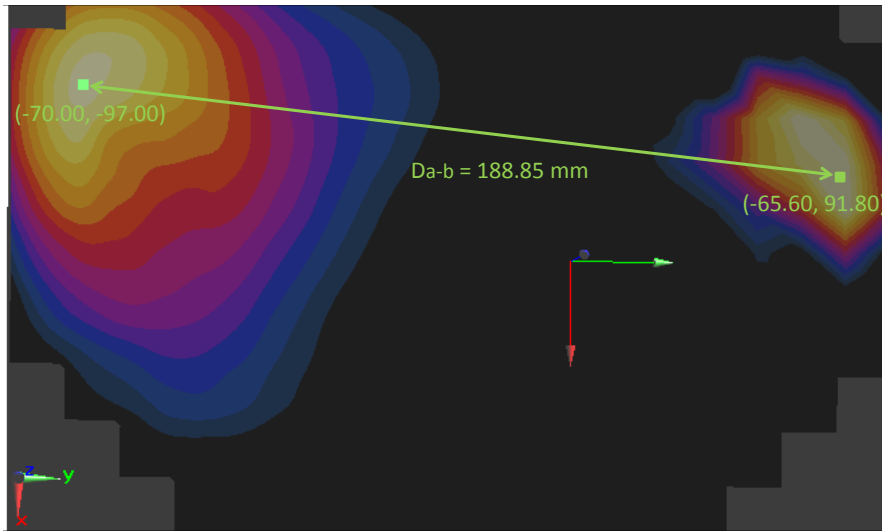
Figure 12-1 Peak SAR Locations of 2.4 GHz WLAN Ant. 1 and GPRS 850 at 0 mm
