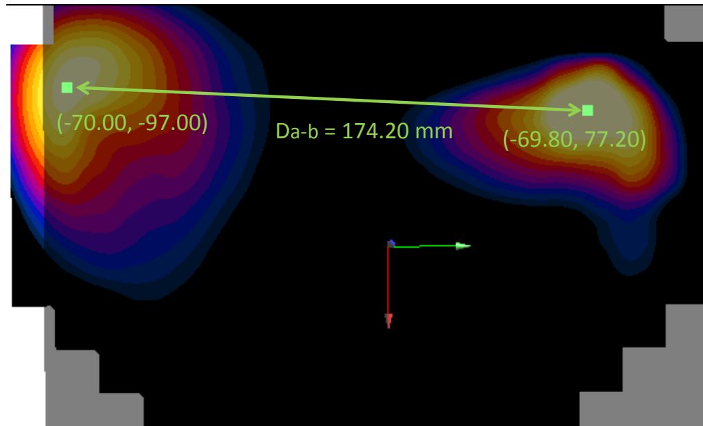
Figure 12-3 Peak SAR Locations of 2.4 GHz WLAN Ant. 2 and GPRS 850 at 0 mm
