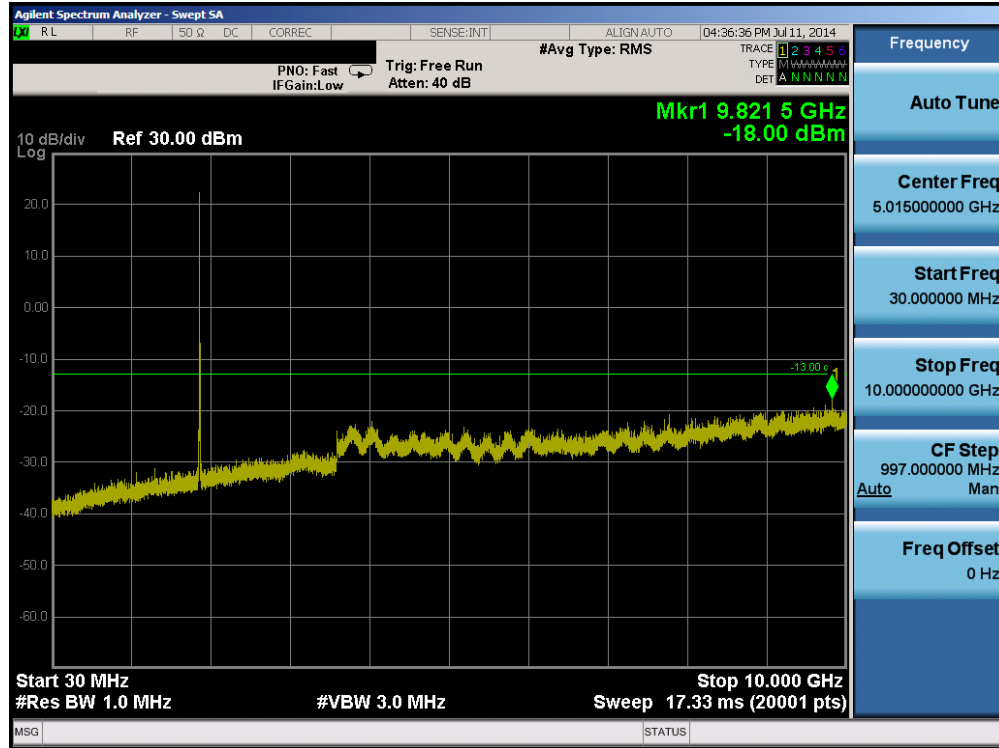
Plot 6-11. Conducted Spurious Plot (PCS WCDMA Mode – Ch. 9400)
