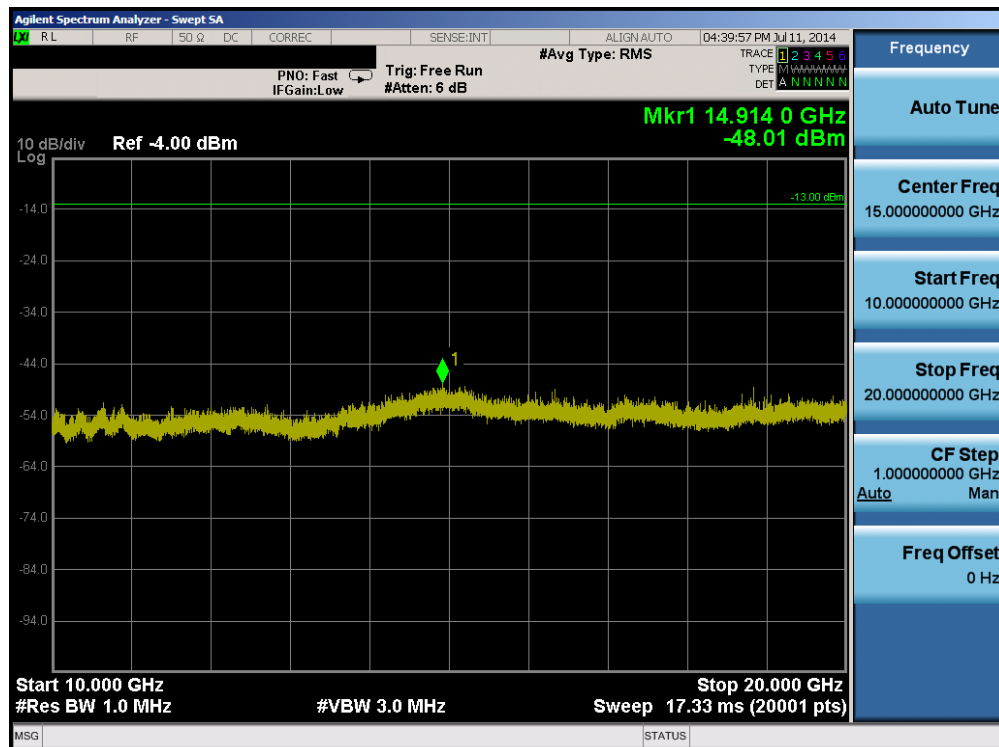
Plot 6-10. Conducted Spurious Plot (PCS WCDMA Mode – Ch. 9262)
