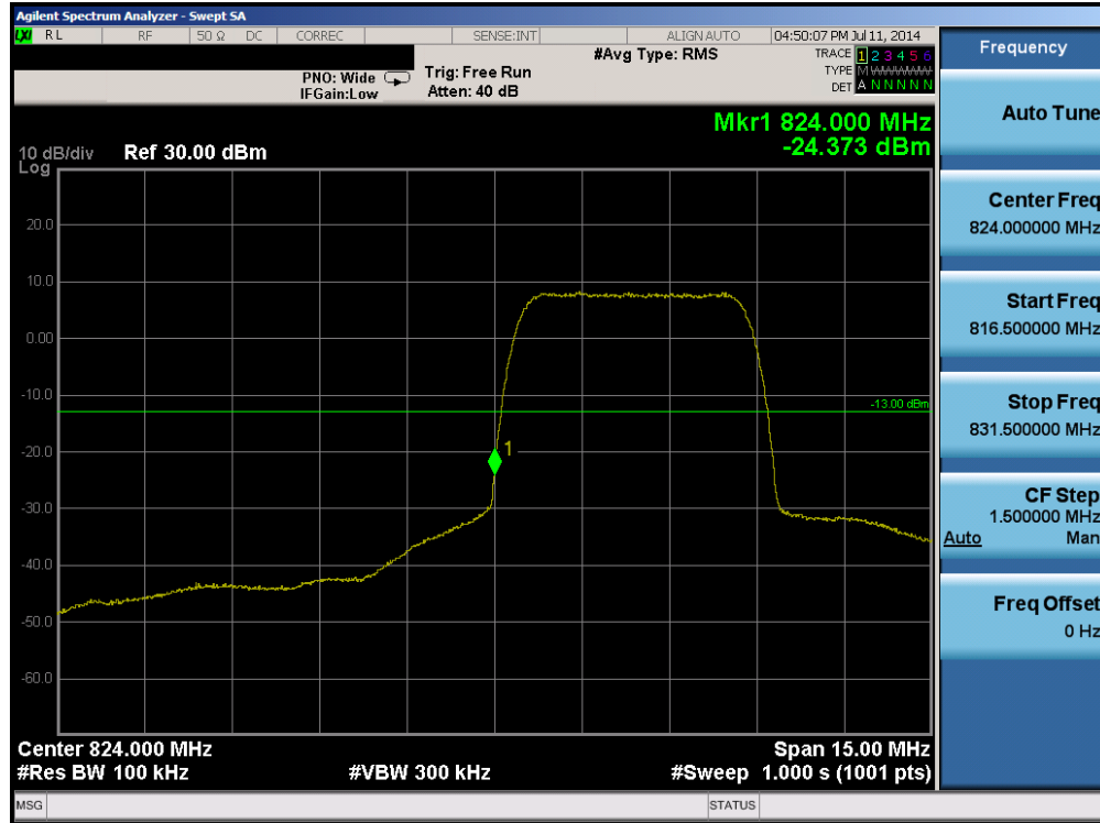
Plot 6-15. Band Edge Plot (Cellular WCDMA Mode – Ch. 4132)
