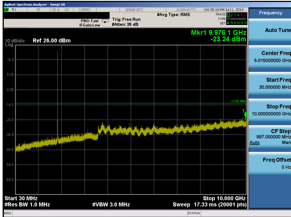
Plot 6-9. Conducted Spurious Plot (PCS WCDMA Mode – Ch. 9262)
