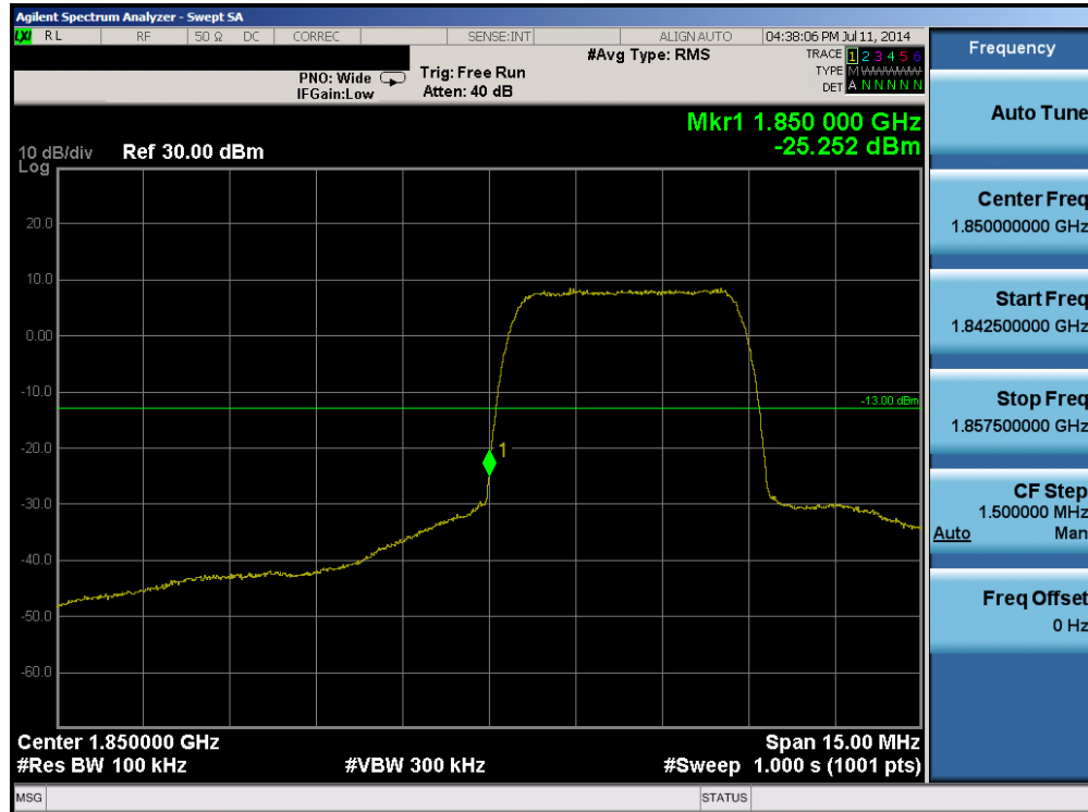
Plot 6-17. Band Edge Plot (PCS WCDMA Mode – Ch. 9262)
