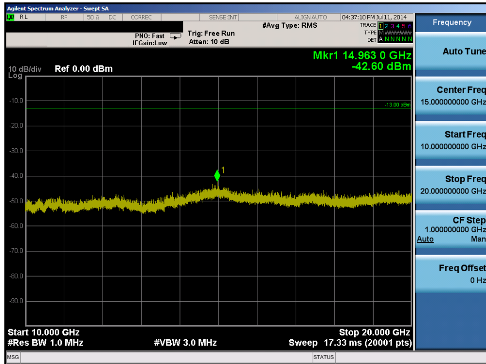
Plot 6-12. Conducted Spurious Plot (PCS WCDMA Mode – Ch. 9400)
