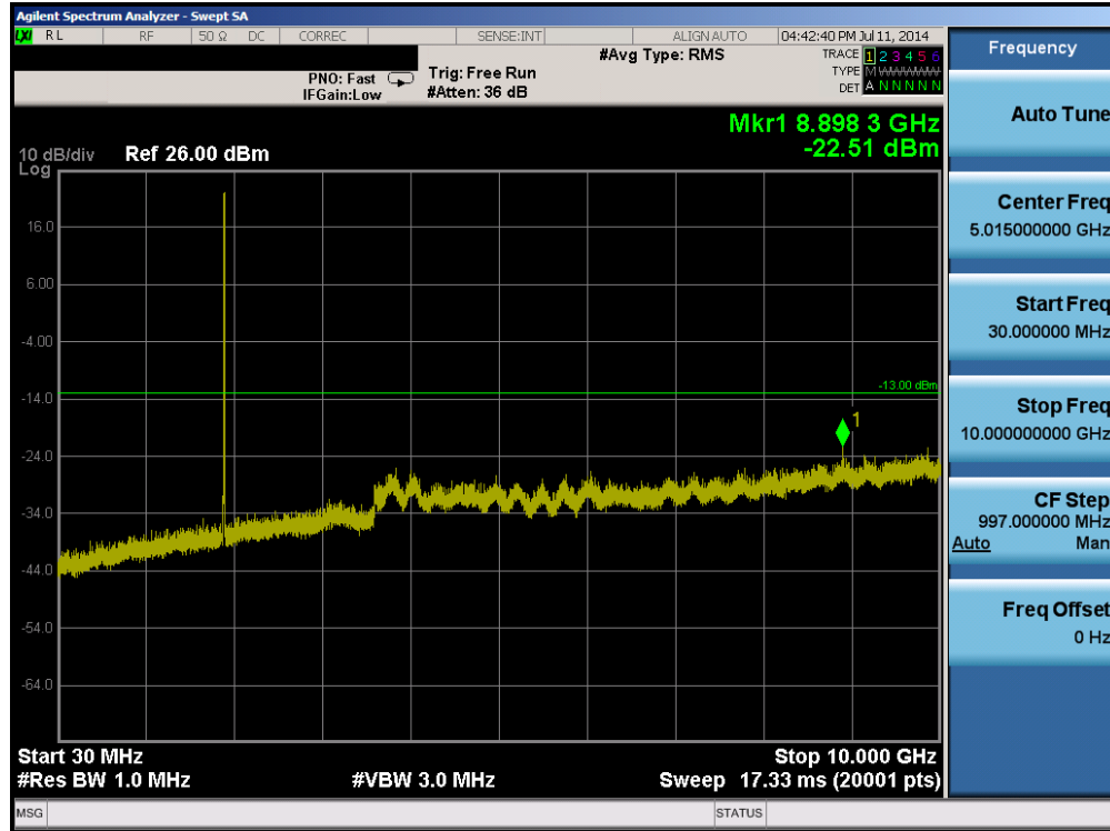
Plot 6-13. Conducted Spurious Plot (PCS WCDMA Mode – Ch. 9538)
