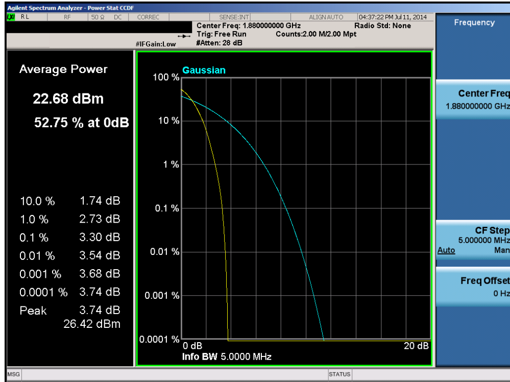
Plot 6-21. Peak-Average Ratio Plot (PCS WCDMA Mode – Ch. 9400)
