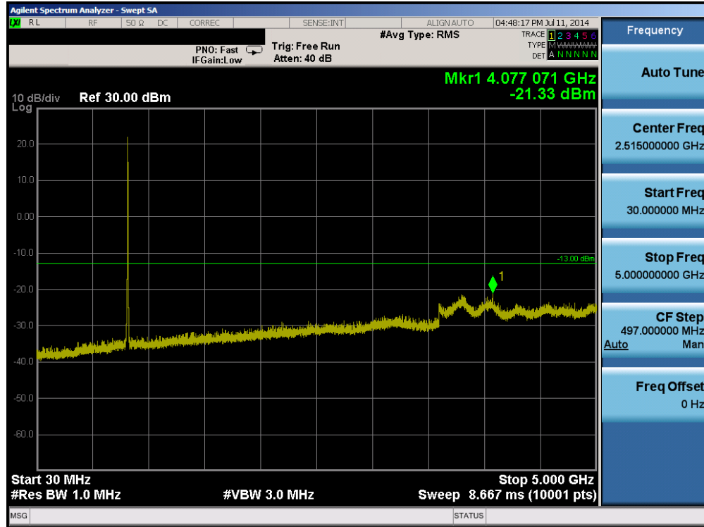
Plot 6-5. Conducted Spurious Plot (Cellular WCDMA Mode – Ch. 4183)
