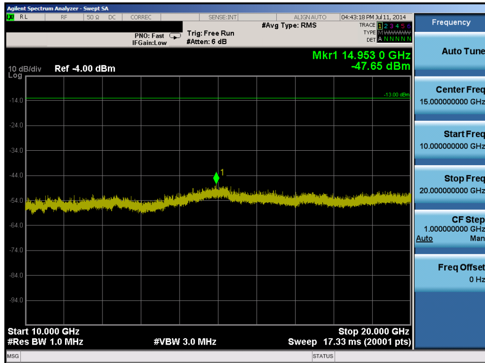
Plot 6-14. Conducted Spurious Plot (PCS WCDMA Mode – Ch. 9538)
