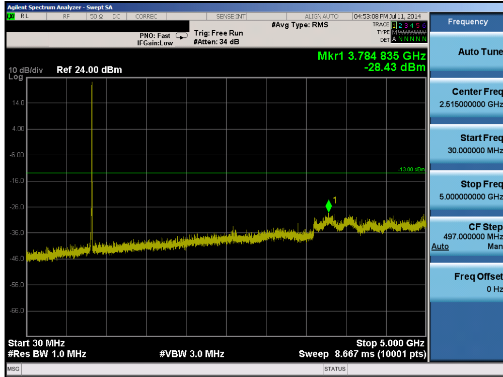
Plot 6-7. Conducted Spurious Plot (Cellular WCDMA Mode – Ch. 4233)
