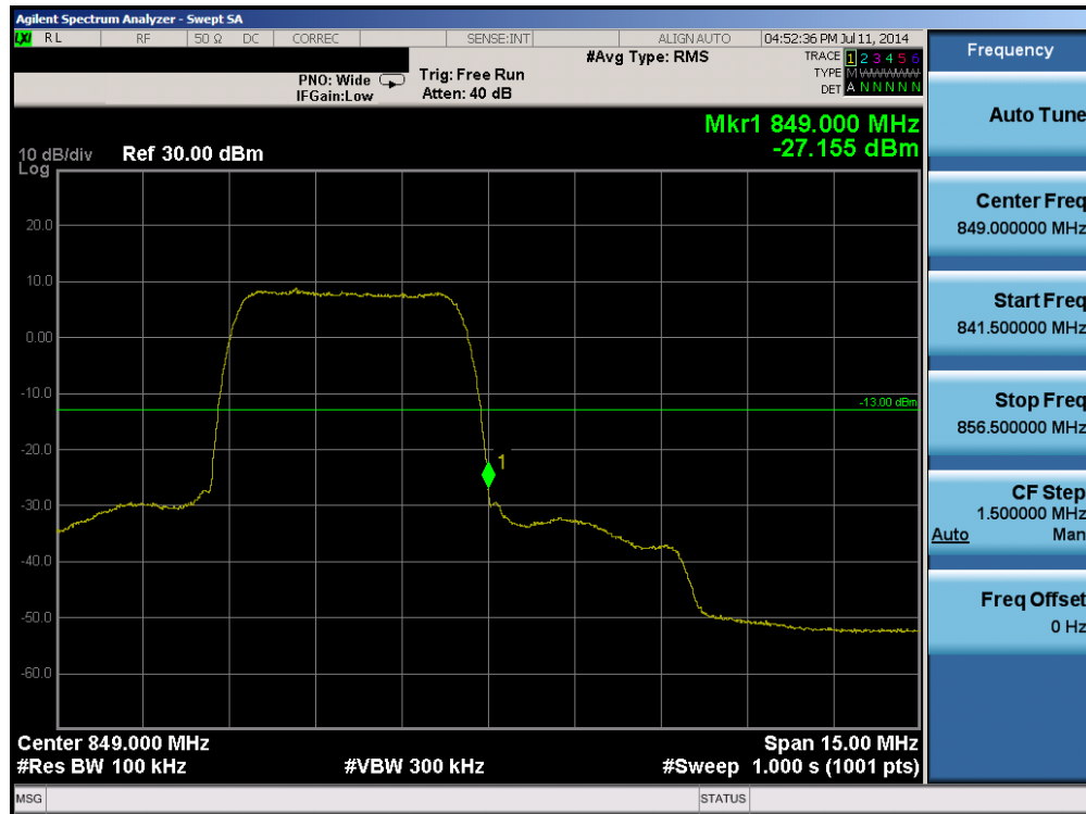
Plot 6-16. Band Edge Plot (Cellular WCDMA Mode – Ch. 4233)
