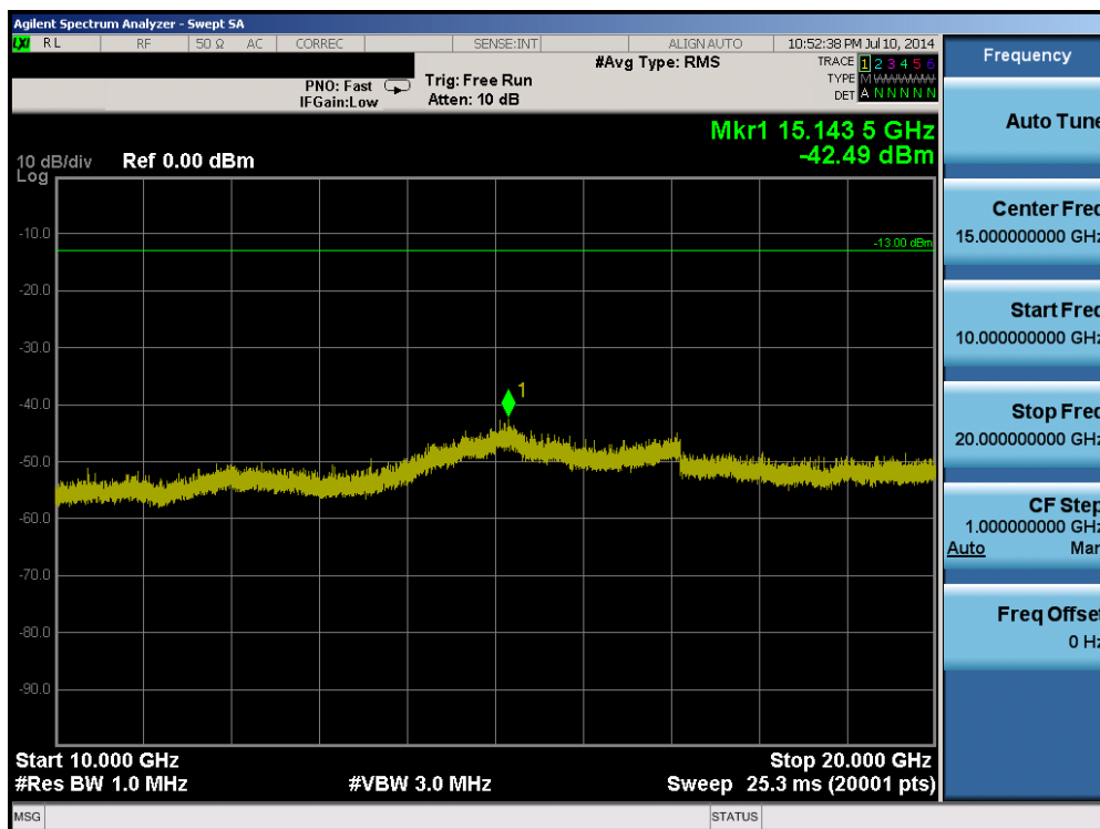
Plot 6-58. Conducted Spurious Plot (Band 2 – 1.4MHz QPSK – RB Size 1, RB Offset 0 – Mid Channel)
