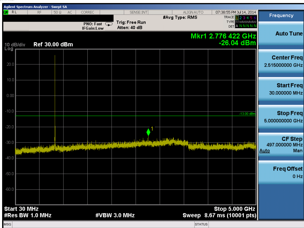
Plot 6-47. Conducted Spurious Plot (Band 5 – 1.4MHz QPSK – RB Size 1, RB Offset 0 – High Channel)
