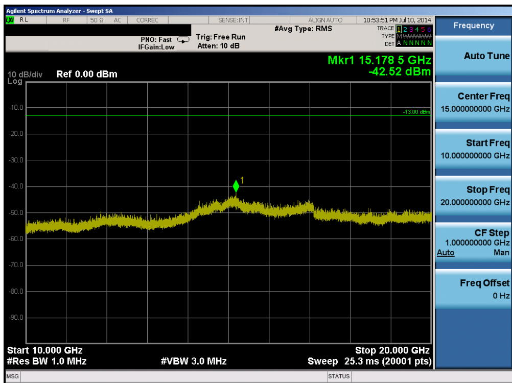
Plot 6-56. Conducted Spurious Plot (Band 2 – 1.4MHz QPSK – RB Size 1, RB Offset 0 – Low Channel)
