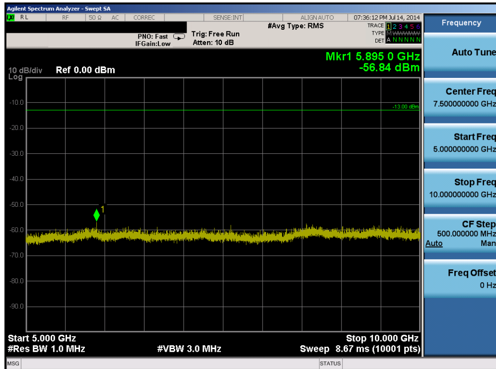
Plot 6-44. Conducted Spurious Plot (Band 5 – 1.4MHz QPSK – RB Size 1, RB Offset 0 – Low Channel)
