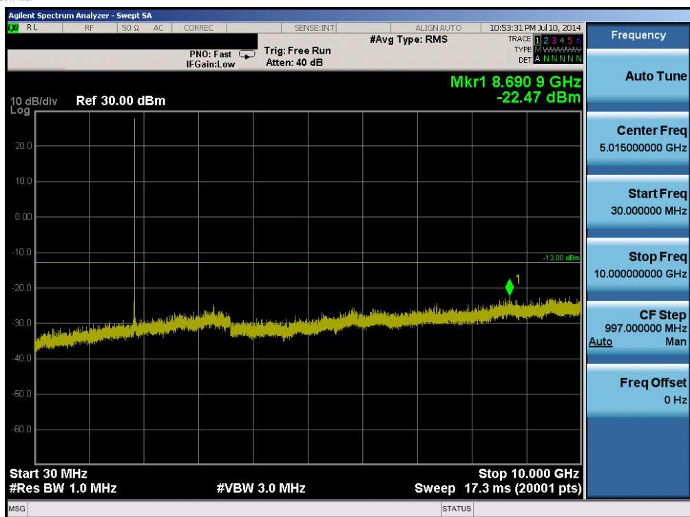
Plot 6-55. Conducted Spurious Plot (Band 2 – 1.4MHz QPSK – RB Size 1, RB Offset 0 – Low Channel)
