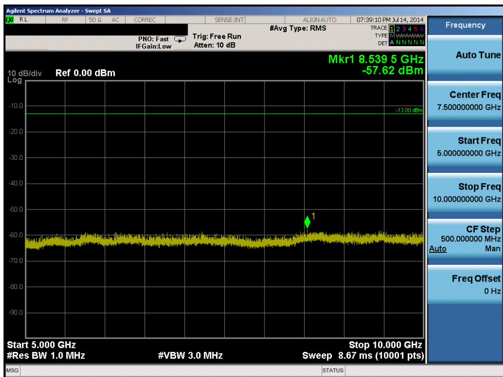
Plot 6-48. Conducted Spurious Plot (Band 5 – 1.4MHz QPSK – RB Size 1, RB Offset 0 – High Channel)
