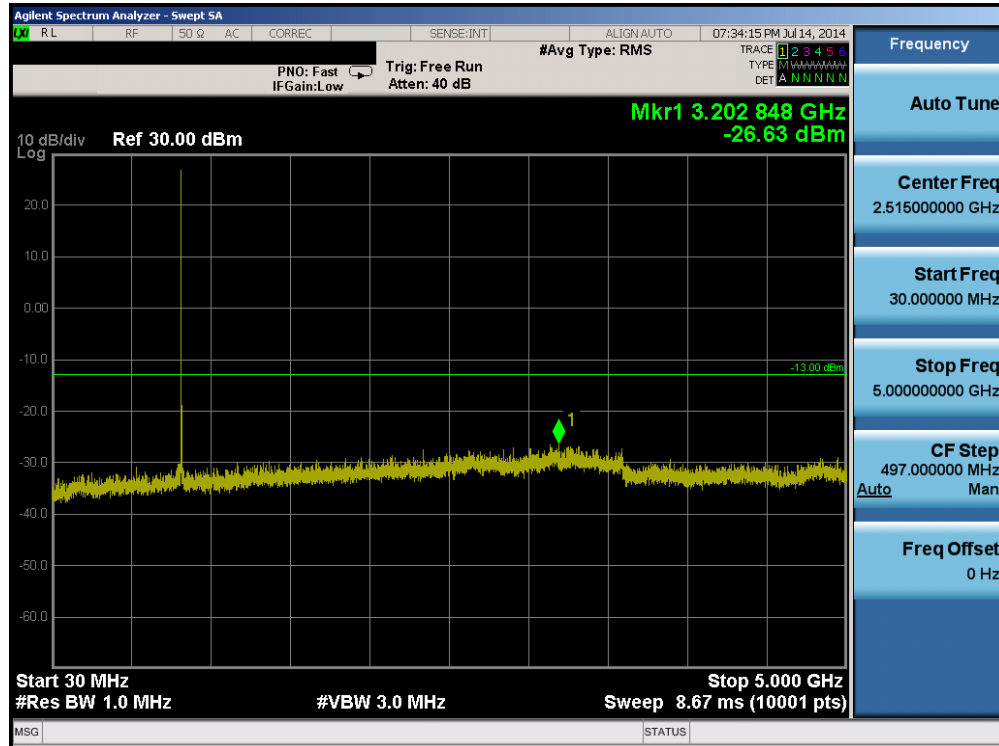
Plot 6-45. Conducted Spurious Plot (Band 5 – 1.4MHz QPSK – RB Size 1, RB Offset 0 – Mid Channel)
