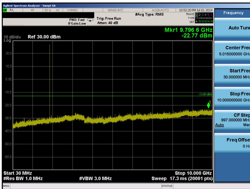
Plot 6-57. Conducted Spurious Plot (Band 2 – 1.4MHz QPSK – RB Size 1, RB Offset 0 – Mid Channel)
