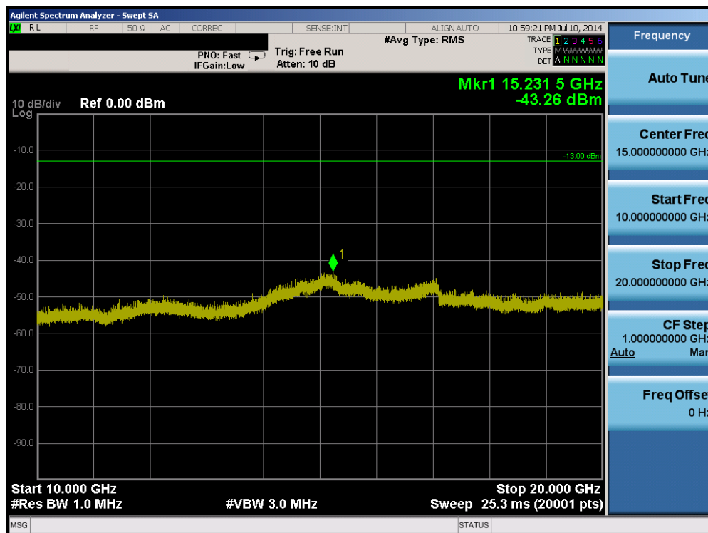
Plot 6-60. Conducted Spurious Plot (Band 2 – 1.4MHz QPSK – RB Size 1, RB Offset 0 – High Channel)
