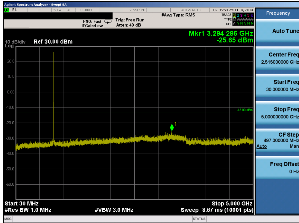
Plot 6-43. Conducted Spurious Plot (Band 5 – 1.4MHz QPSK – RB Size 1, RB Offset 0 – Low Channel)
