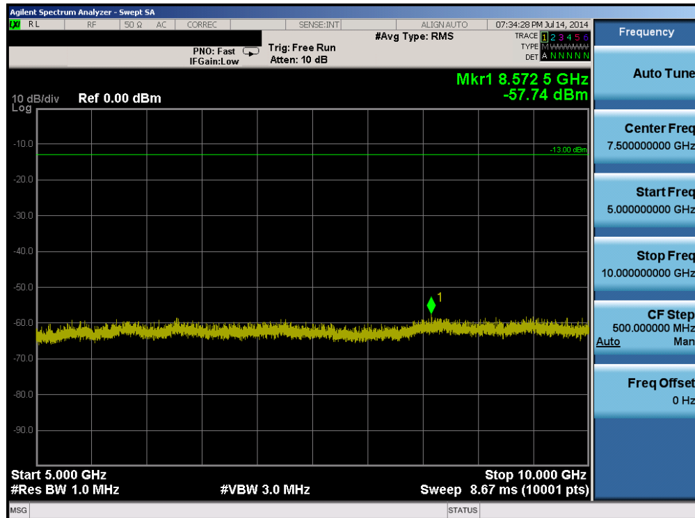
Plot 6-46. Conducted Spurious Plot (Band 5 – 1.4MHz QPSK – RB Size 1, RB Offset 0 – Mid Channel)
