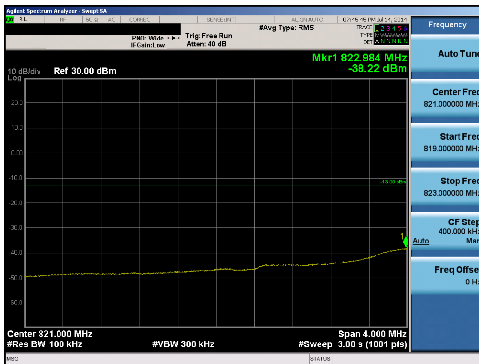
Plot 6-72. Lower Extended Band Edge Plot (Band 5 – 3.0MHz QPSK – RB Size 15)
