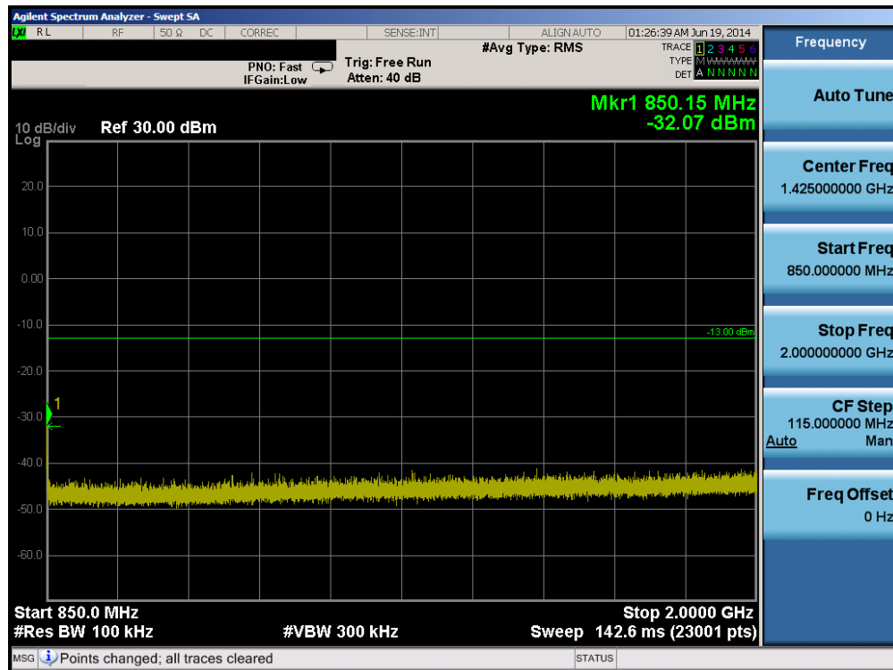
Plot 6-14. Conducted Spurious Plot (Cellular GPRS Mode – Ch. 251)
