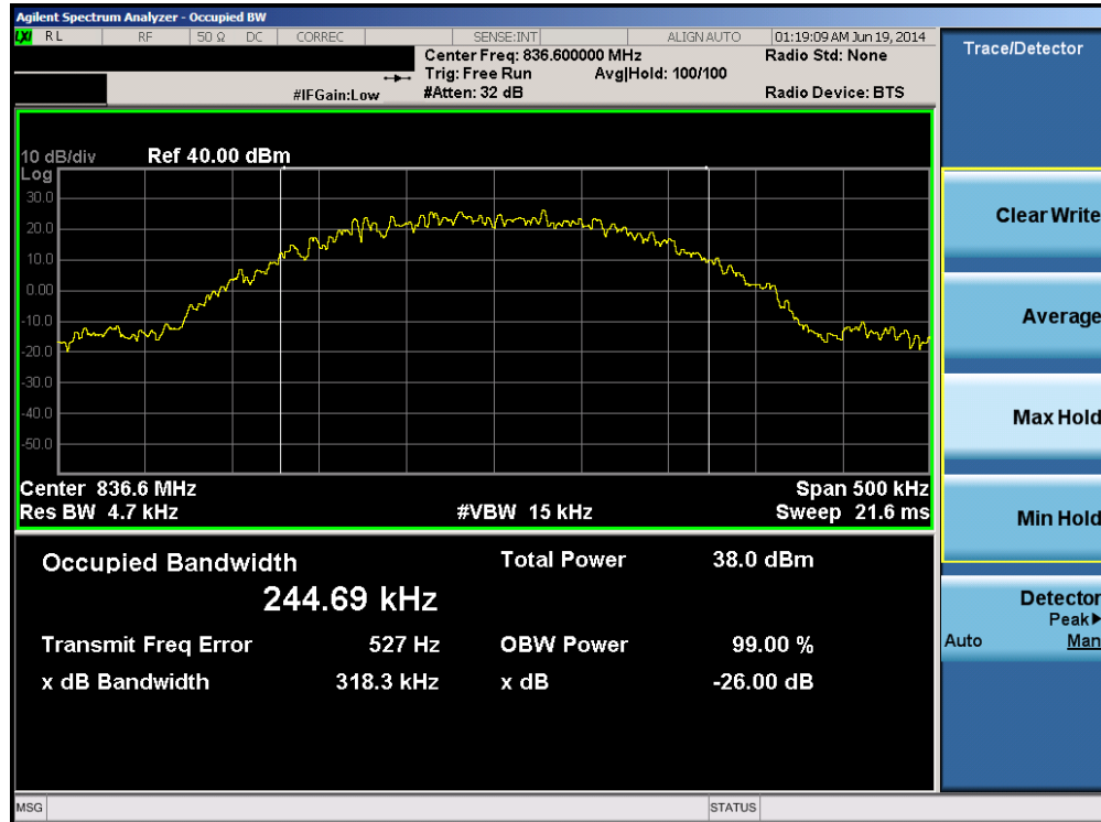
Plot 6-1. Occupied Bandwidth Plot (Cellular GPRS Mode – Ch. 190)
