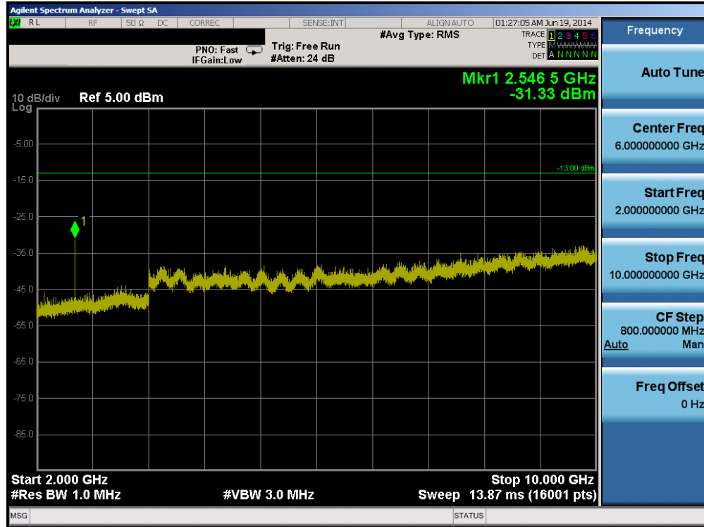
Plot 6-15. Conducted Spurious Plot (Cellular GPRS Mode – Ch. 251)
