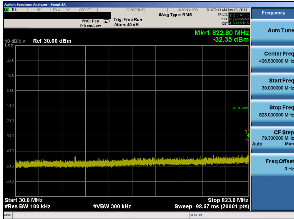
Plot 6-7. Conducted Spurious Plot (Cellular GPRS Mode – Ch. 128)
