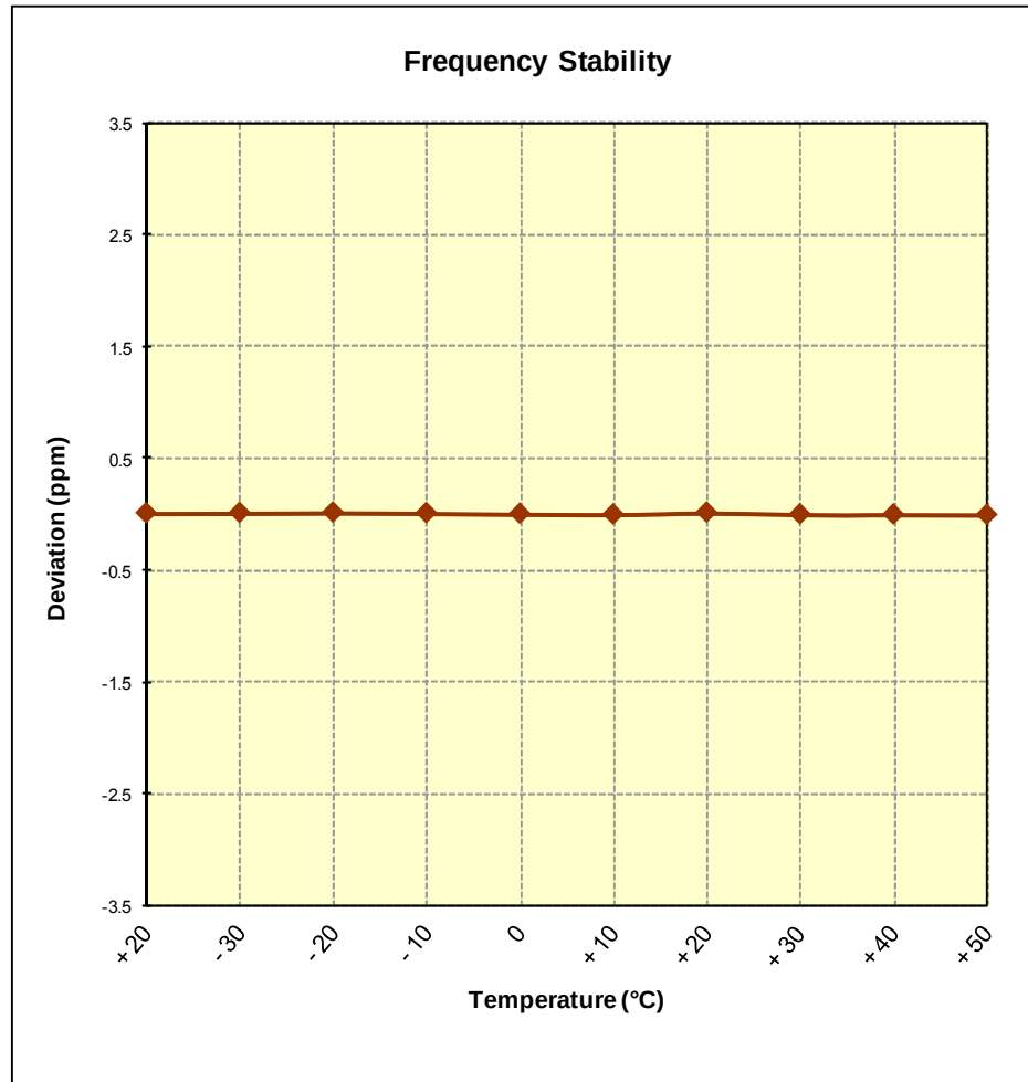
Figure 6-9. Frequency Stability Graph (PCS GPRS Mode – Ch. 661)
