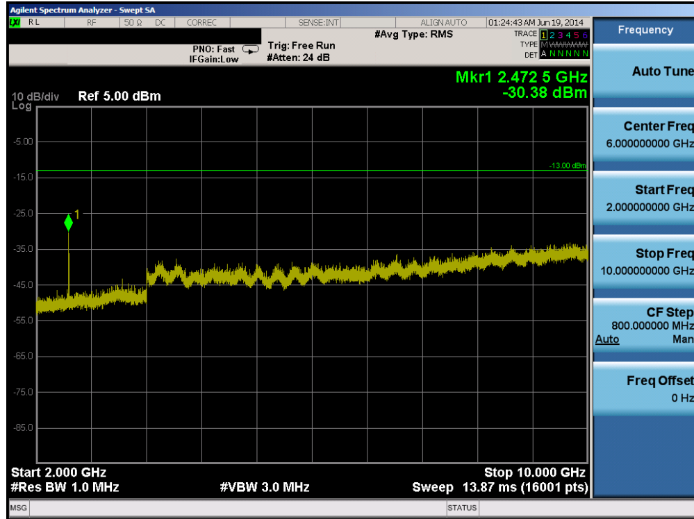
Plot 6-9. Conducted Spurious Plot (Cellular GPRS Mode – Ch. 128)
