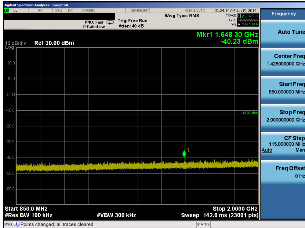
Plot 6-8. Conducted Spurious Plot (Cellular GPRS Mode – Ch. 128)
