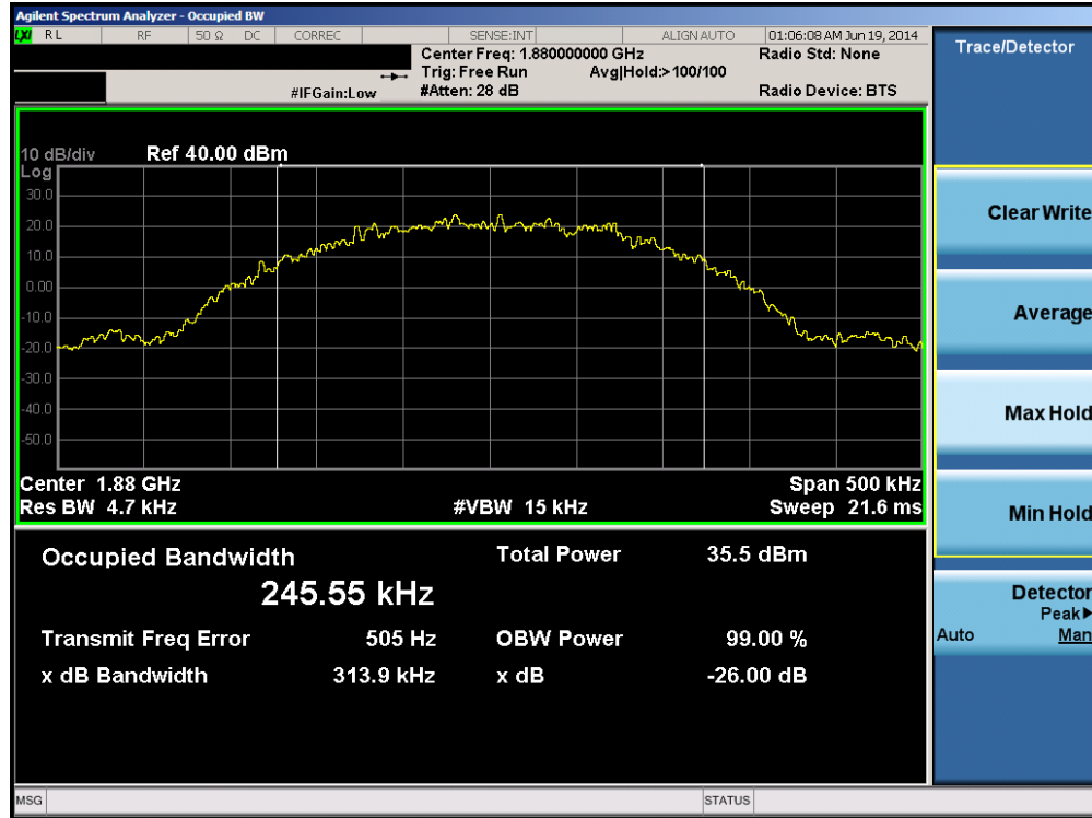
Plot 6-3. Occupied Bandwidth Plot (PCS GPRS Mode – Ch. 661)
