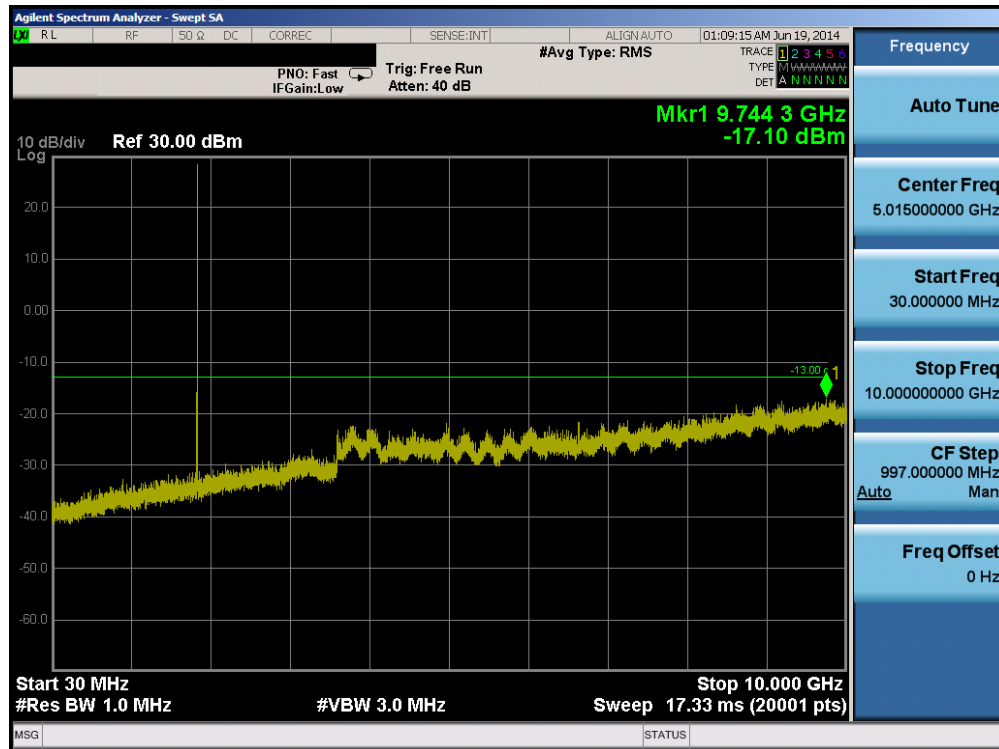
Plot 6-16. Conducted Spurious Plot (PCS GPRS Mode – Ch. 512)
