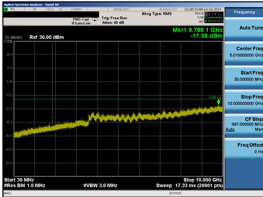
Plot 6-18. Conducted Spurious Plot (PCS GPRS Mode – Ch. 661)
