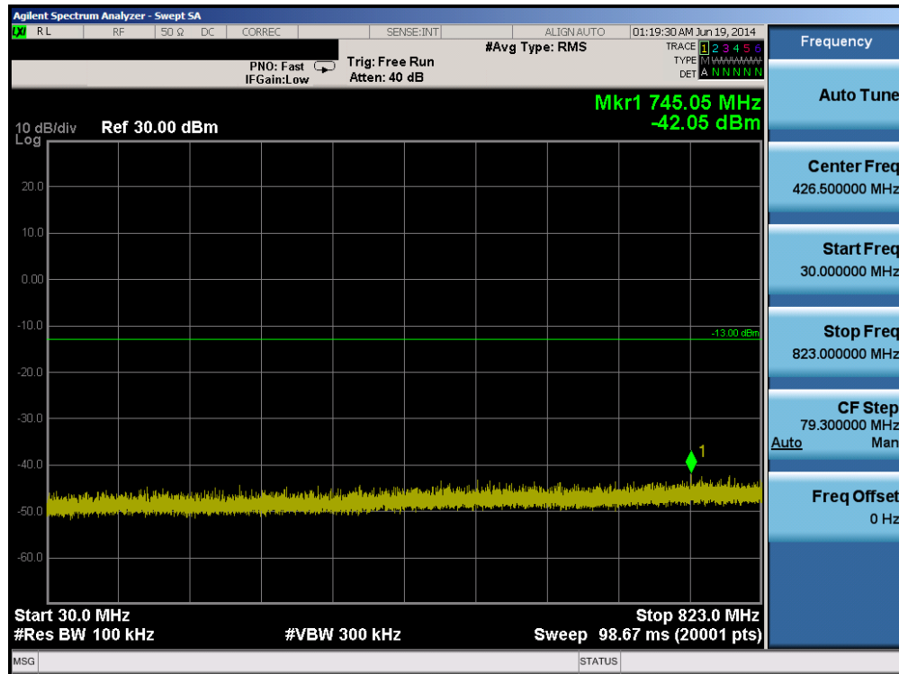
Plot 6-10. Conducted Spurious Plot (Cellular GPRS Mode – Ch. 190)
