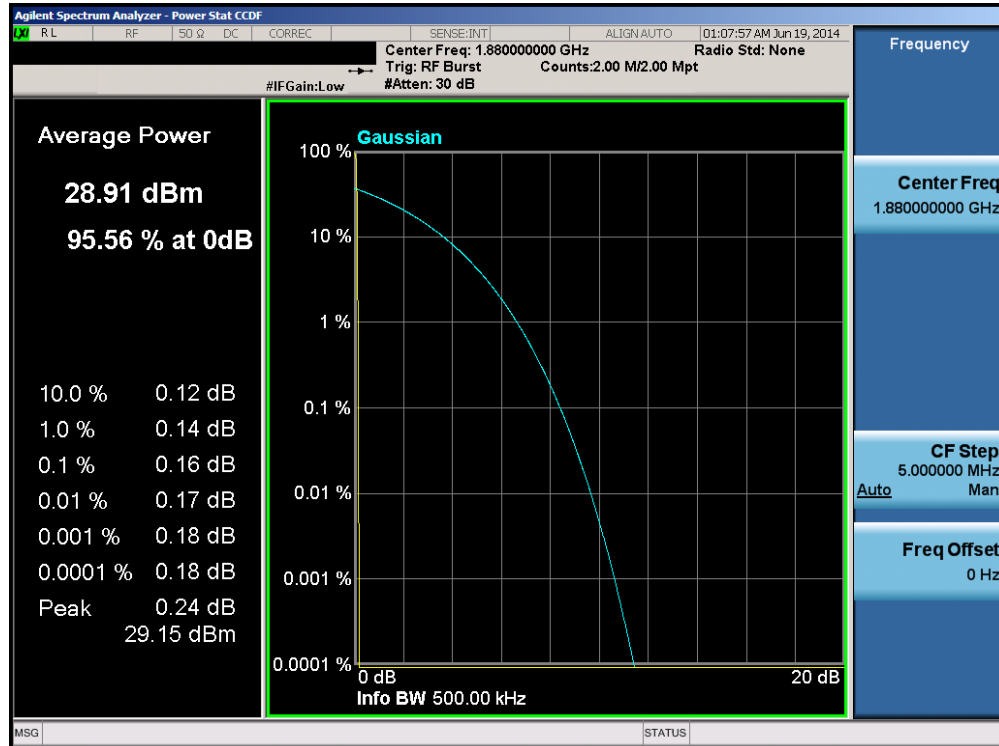
Plot 6-44. Peak-Average Ratio Plot (PCS GPRS Mode – Ch. 661)
