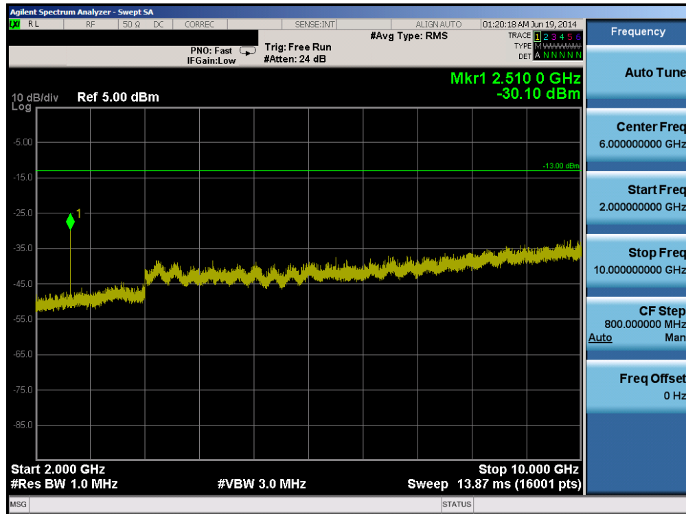
Plot 6-12. Conducted Spurious Plot (Cellular GPRS Mode – Ch. 190)
