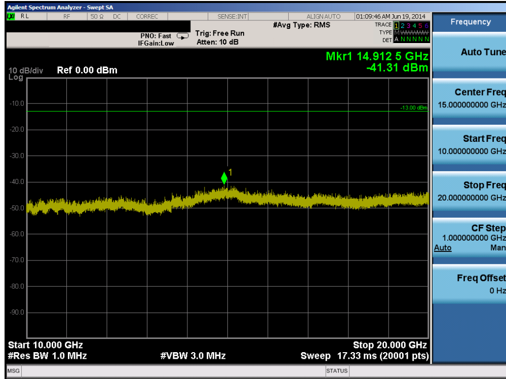
Plot 6-17. Conducted Spurious Plot (PCS GPRS Mode – Ch. 512)
