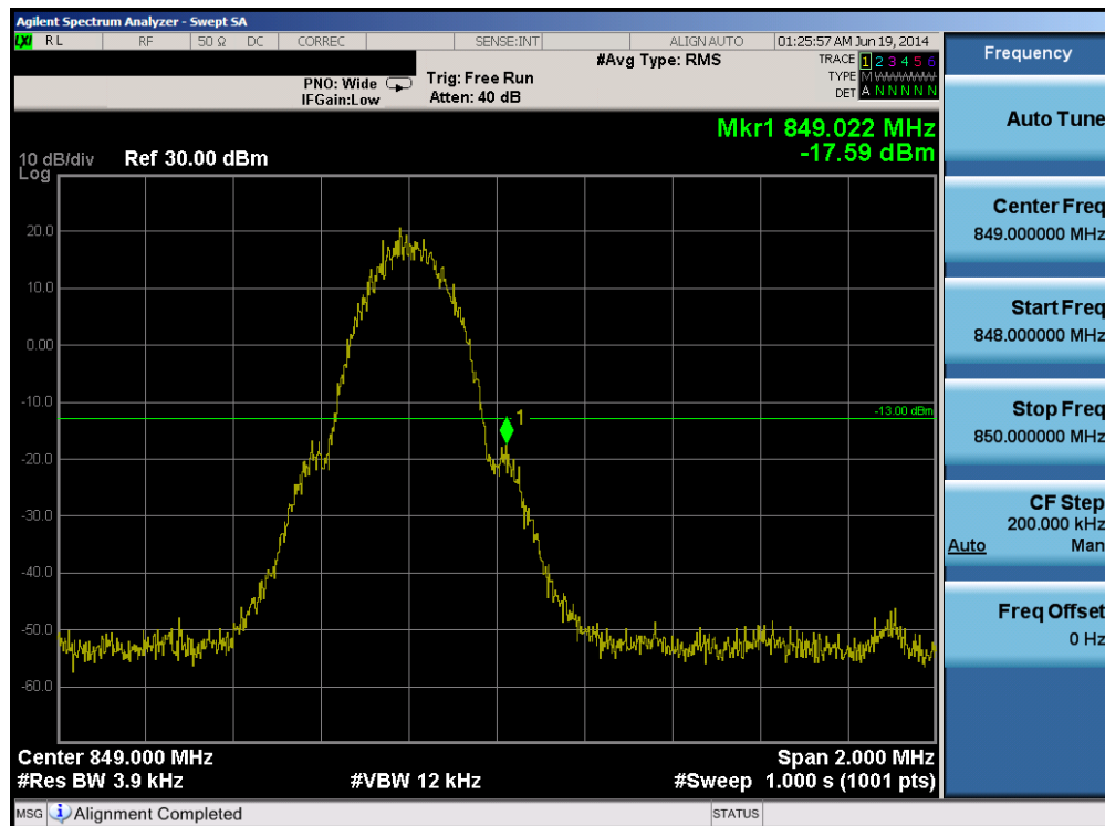
Plot 6-35. Band Edge Plot (Cellular GPRS Mode – Ch. 251)
