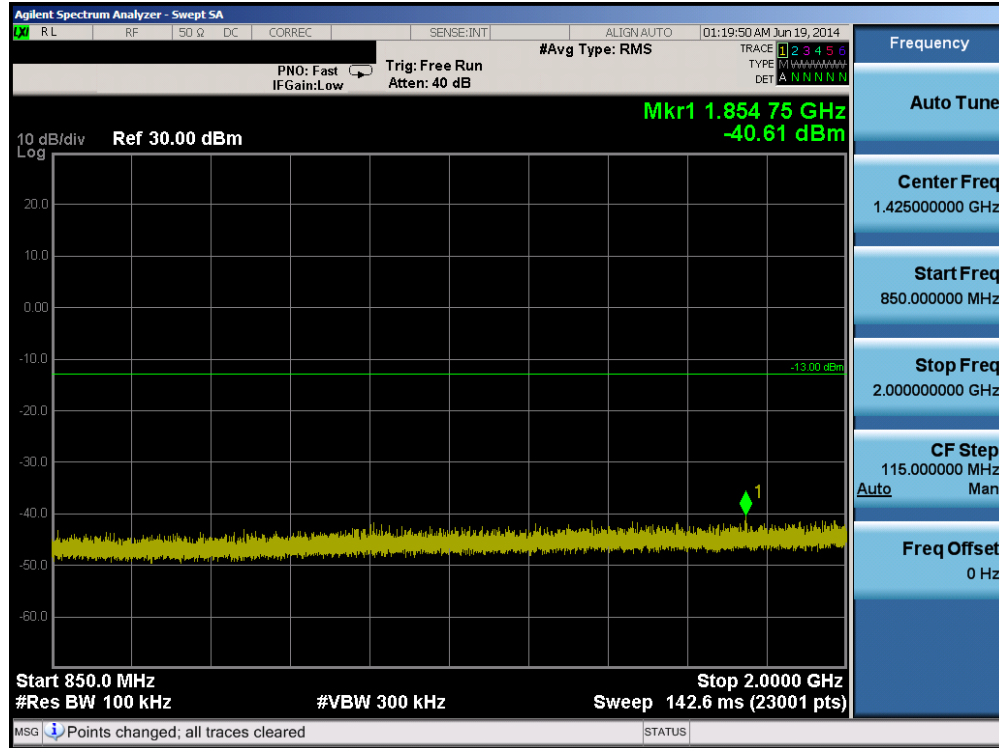
Plot 6-11. Conducted Spurious Plot (Cellular GPRS Mode – Ch. 190)
