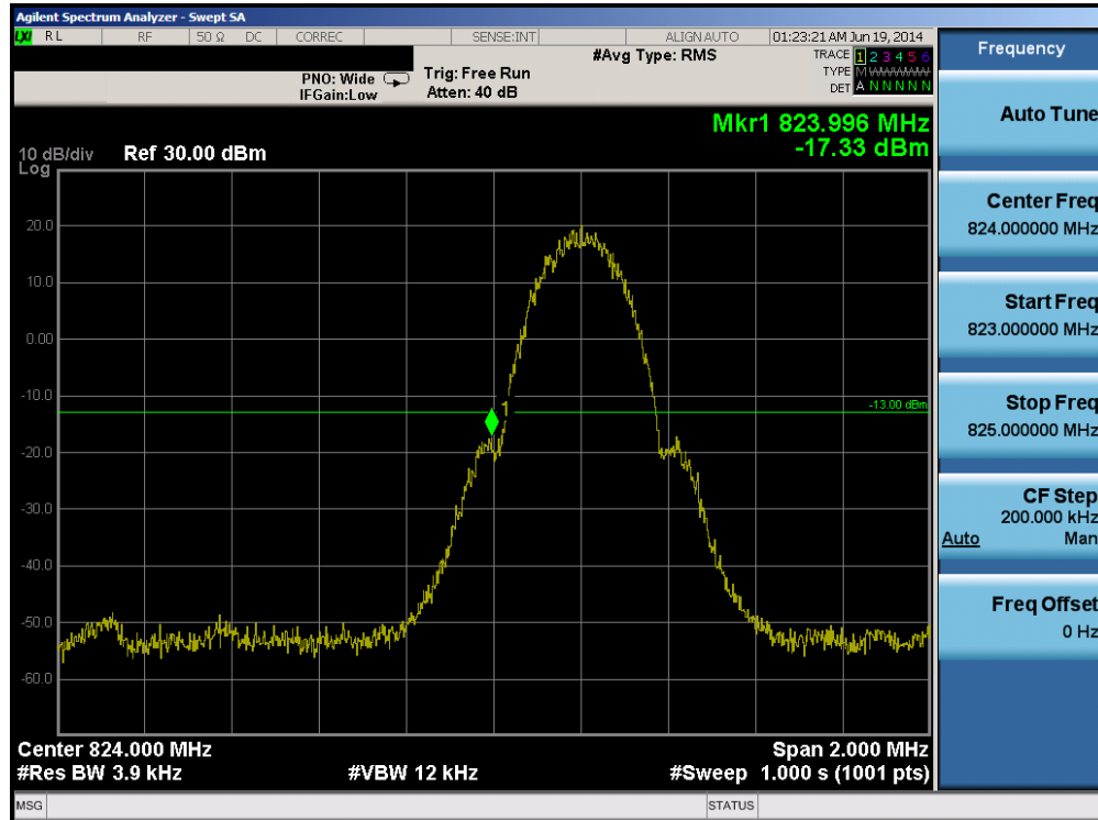
Plot 6-34. Band Edge Plot (Cellular GPRS Mode – Ch. 128)
