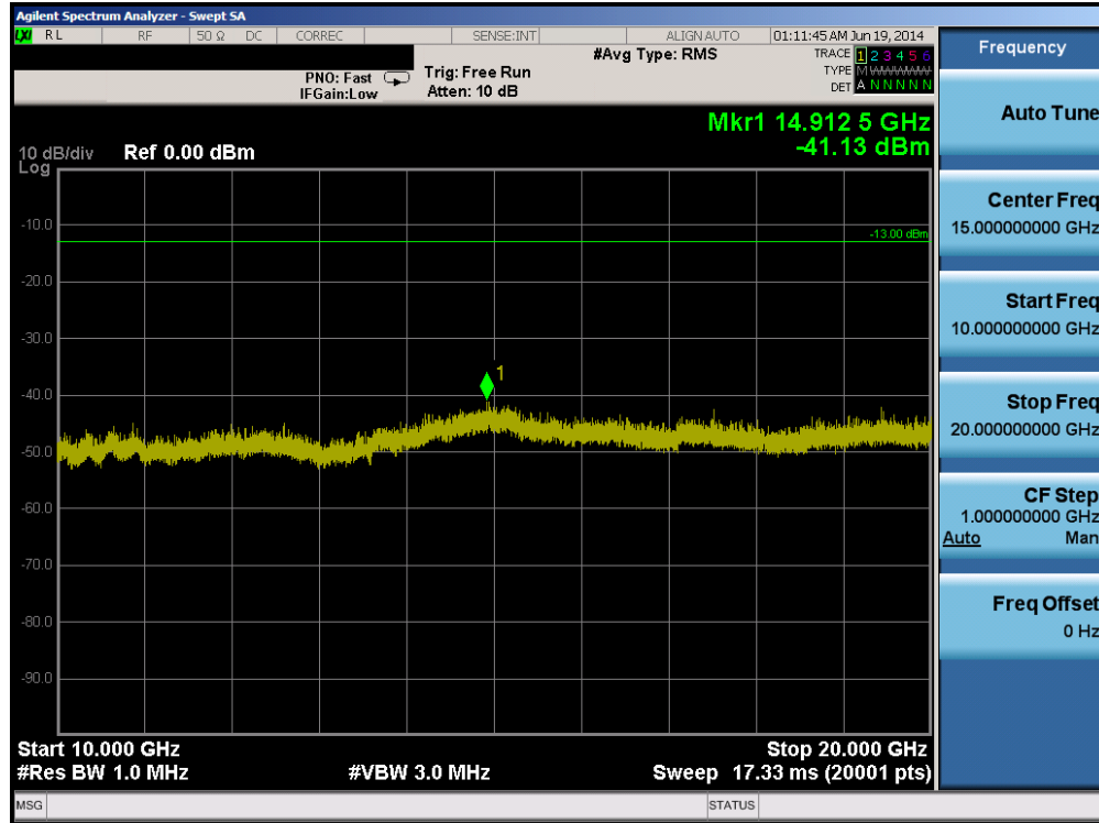
Plot 6-21. Conducted Spurious Plot (PCS GPRS Mode – Ch. 810)
