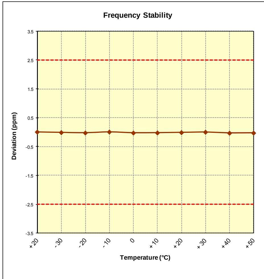
Figure 6-7. Frequency Stability Graph (Cellular GPRS Mode – Ch. 190)
