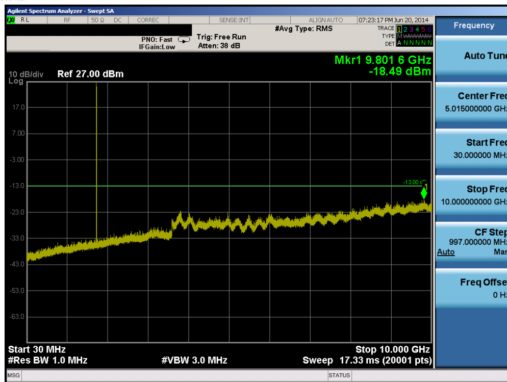
Plot 6-25. Conducted Spurious Plot (Band 4 – 5.0MHz QPSK – RB Size 1, RB Offset 0 – High Channel)
