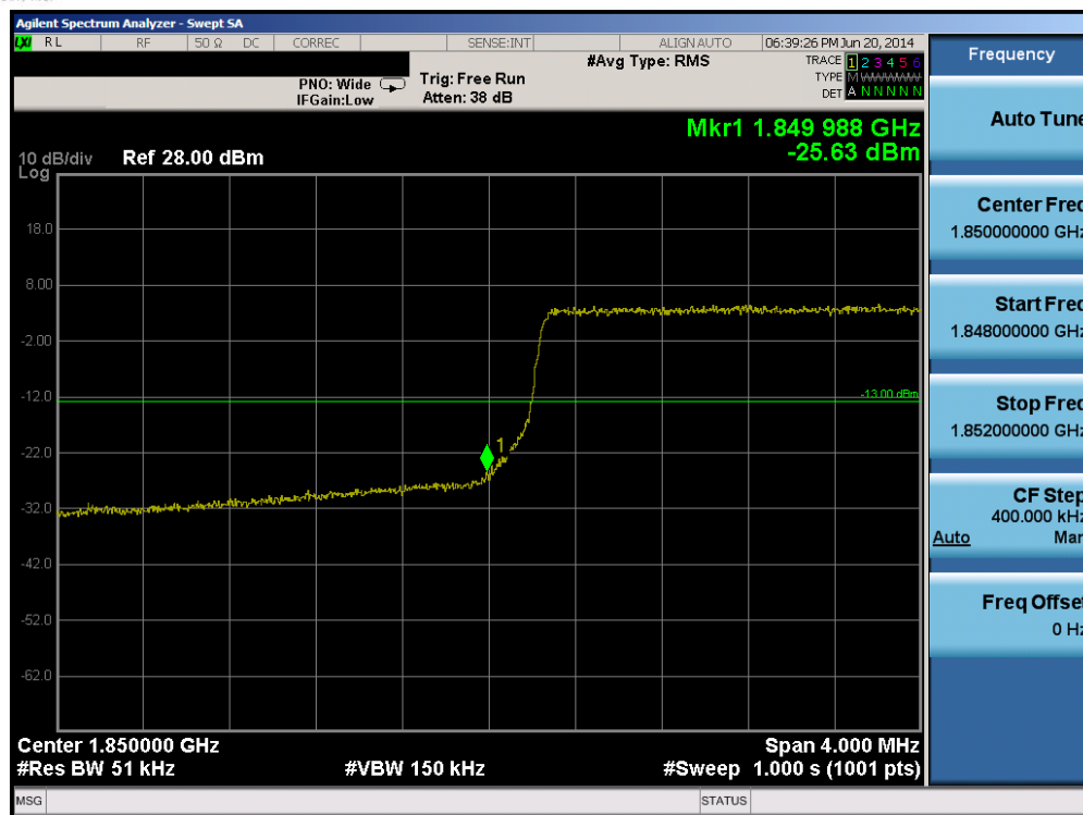
Plot 6-51. Lower Band Edge Plot (Band 2 – 5.0MHz QPSK – RB Size 25)
