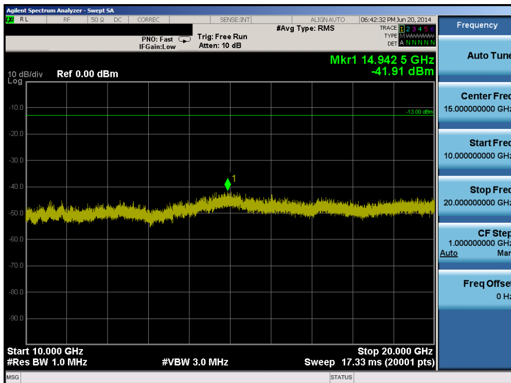
Plot 6-32. Conducted Spurious Plot (Band 2 – 5.0MHz QPSK – RB Size 1, RB Offset 0 – High Channel)
