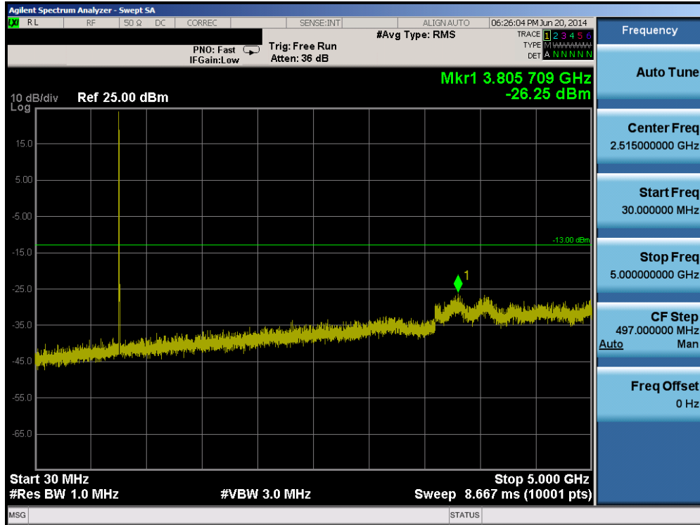
Plot 6-19. Conducted Spurious Plot (Band 13 – 10.0MHz QPSK – RB Size 1, RB Offset 0)
