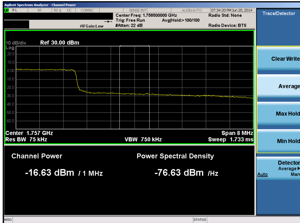
Plot 6-42. Upper Extended Band Edge Plot (Band 4 – 10.0MHz QPSK – RB Size 50)
