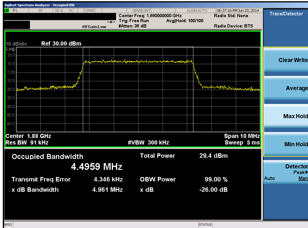
Plot 6-12. Occupied Bandwidth Plot (Band 2 – 5.0MHz 16-QAM – RB Size 25)
