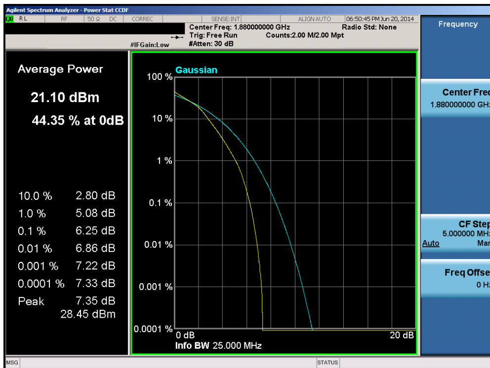
Plot 6-80. PAR Plot (Band 2 – 15.0MHz 16-QAM – RB Size 75)
