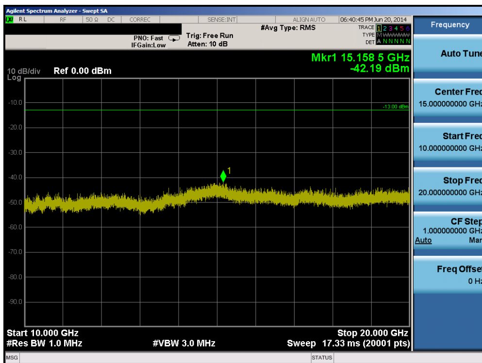
Plot 6-28. Conducted Spurious Plot (Band 2 – 5.0MHz QPSK – RB Size 1, RB Offset 0 – Low Channel)
