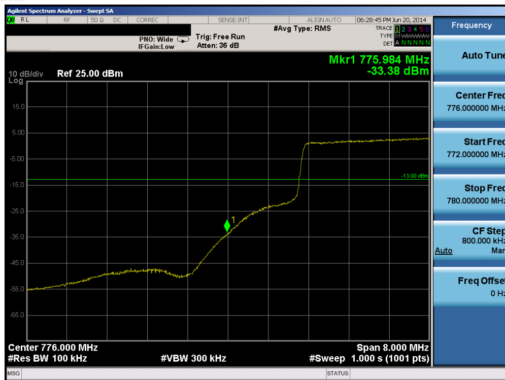
Plot 6-33. Lower Band Edge Plot (Band 13 – 10.0MHz QPSK – RB Size 50)
