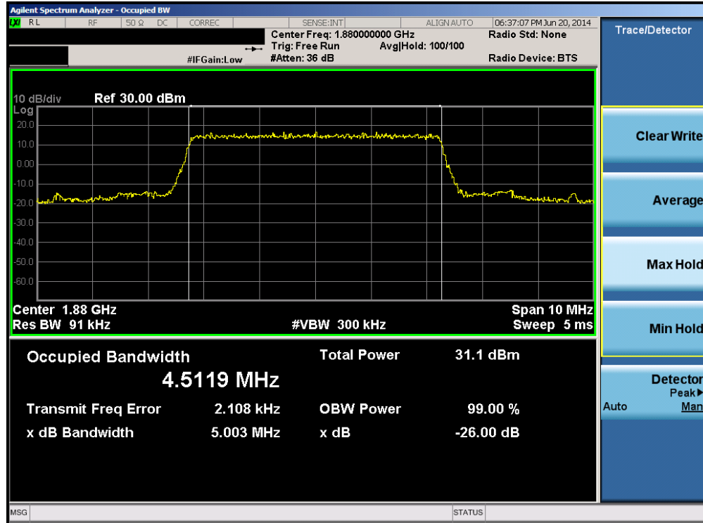
Plot 6-11. Occupied Bandwidth Plot (Band 2 – 5.0MHz QPSK – RB Size 25)
