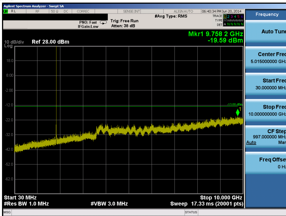
Plot 6-27. Conducted Spurious Plot (Band 2 – 5.0MHz QPSK – RB Size 1, RB Offset 0 – Low Channel)
