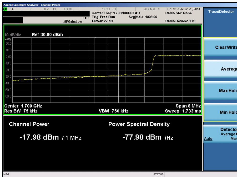
Plot 6-40. Lower Extended Band Edge Plot (Band 4 – 10.0MHz QPSK – RB Size 50)
