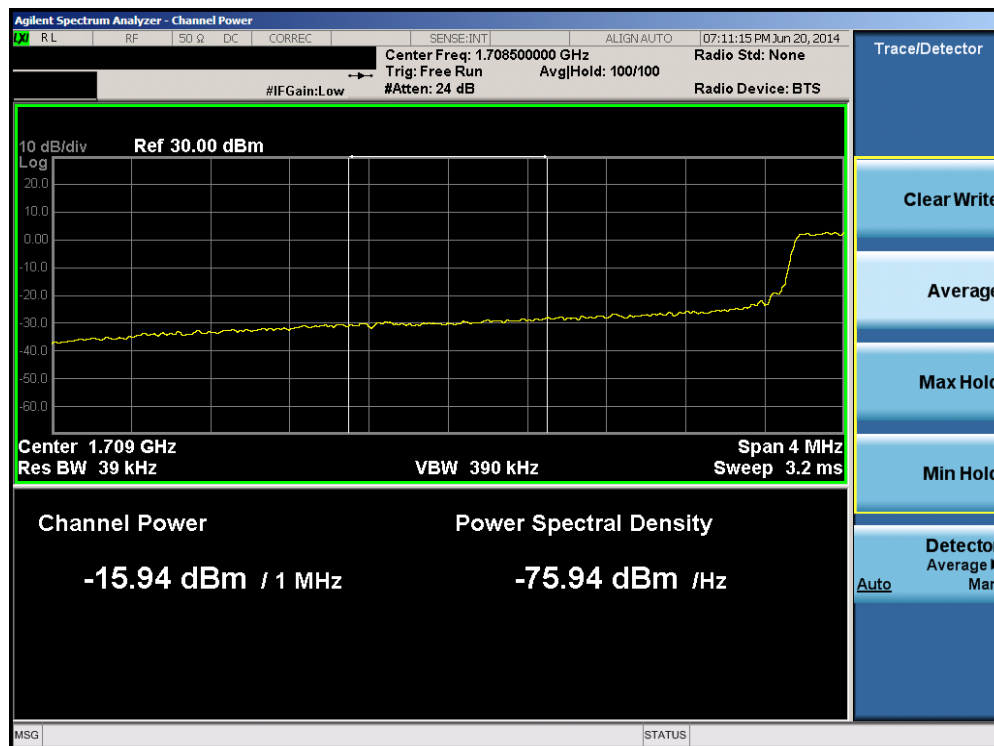
Plot 6-36. Lower Extended Band Edge Plot (Band 4 – 5.0MHz QPSK – RB Size 25)
