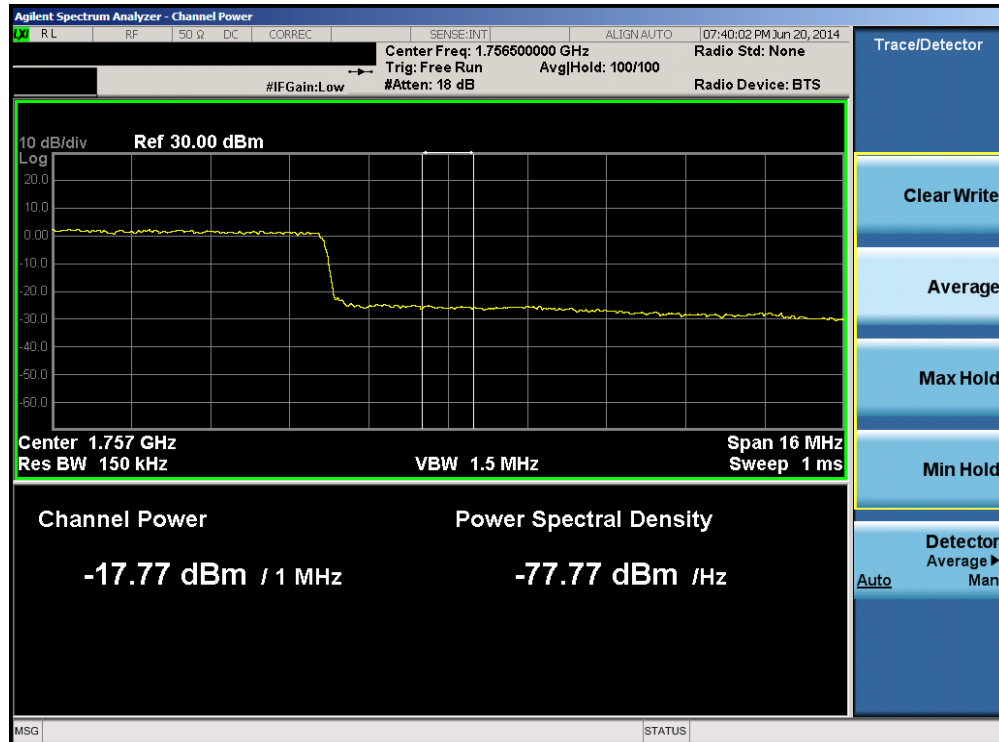
Plot 6-50. Upper Extended Band Edge Plot (Band 4 – 20.0MHz QPSK – RB Size 100)
