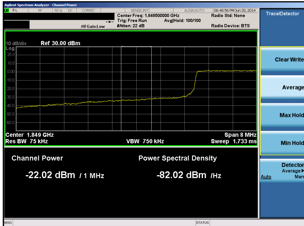
Plot 6-56. Lower Extended Band Edge Plot (Band 2 – 10.0MHz QPSK – RB Size 50)
