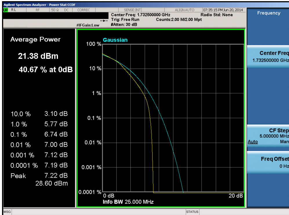
Plot 6-72. PAR Plot (Band 4 – 15.0MHz 16-QAM – RB Size 75)
