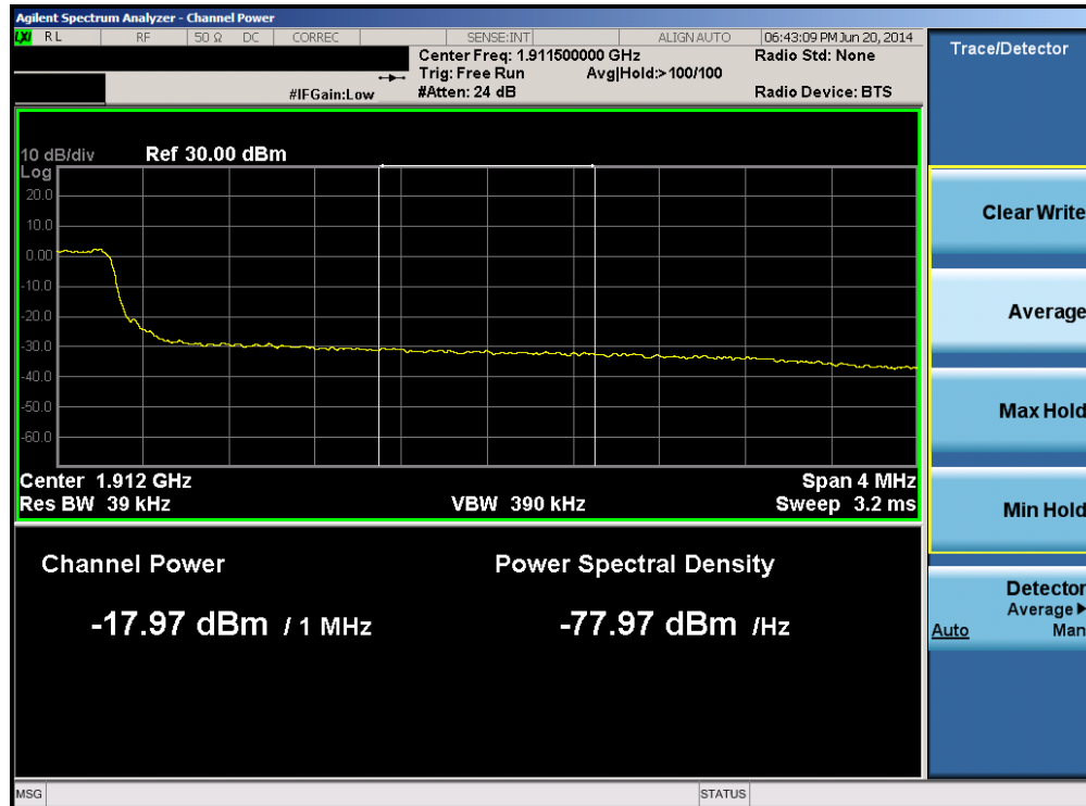
Plot 6-54. Upper Extended Band Edge Plot (Band 2 – 5.0MHz QPSK – RB Size 25)
