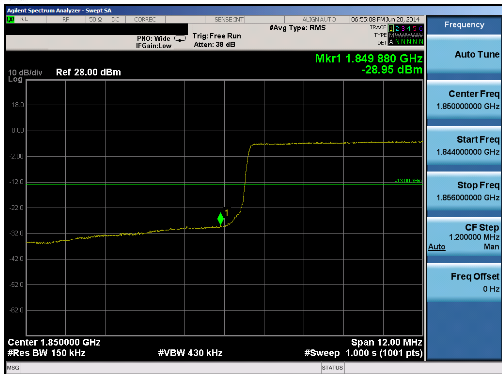
Plot 6-59. Lower Band Edge Plot (Band 2 – 15.0MHz QPSK – RB Size 75)
