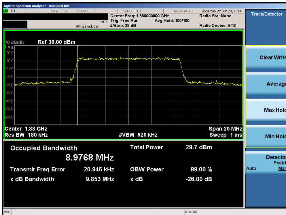
Plot 6-14. Occupied Bandwidth Plot (Band 2 – 10.0MHz 16-QAM – RB Size 50)
