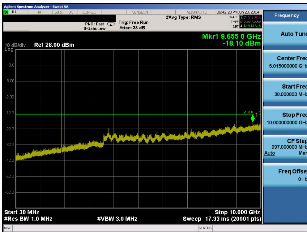
Plot 6-31. Conducted Spurious Plot (Band 2 – 5.0MHz QPSK – RB Size 1, RB Offset 0 – High Channel)
