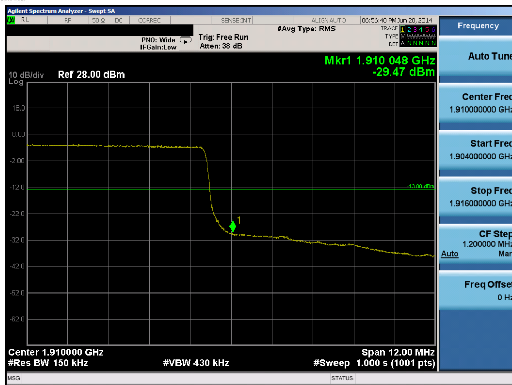
Plot 6-61. Upper Band Edge Plot (Band 2 – 15.0MHz QPSK – RB Size 75)
