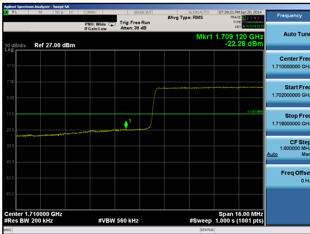
Plot 6-47. Lower Band Edge Plot (Band 4 - 20.0MHz QPSK - RB Size 100)
