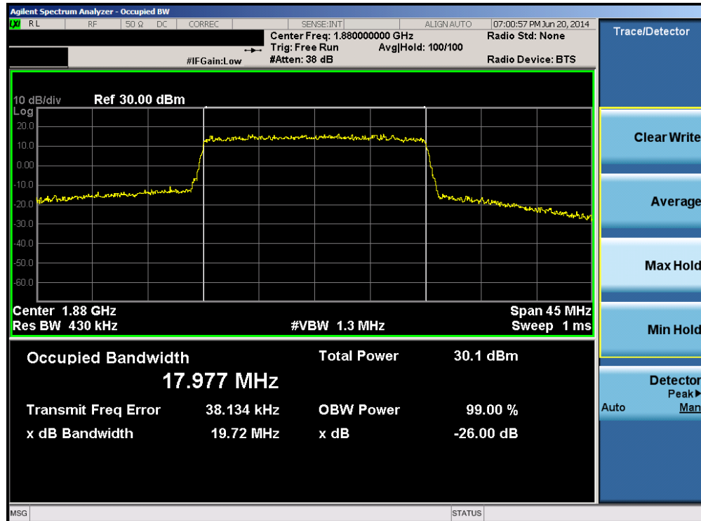
Plot 6-18. Occupied Bandwidth Plot (Band 2 – 20.0MHz 16-QAM – RB Size 100)
