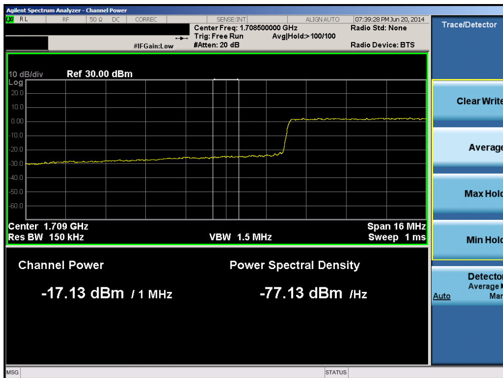
Plot 6-48. Lower Extended Band Edge Plot (Band 4 - 20.0MHz QPSK - RB Size 100)
