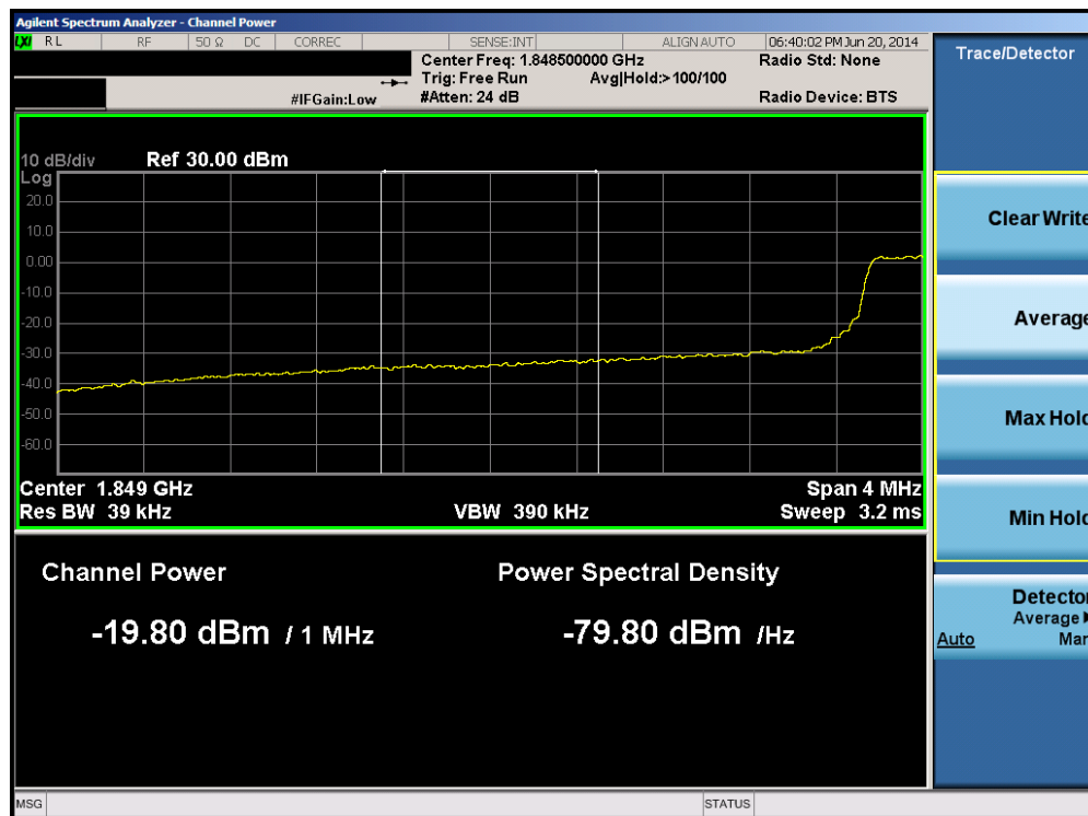
Plot 6-52. Lower Extended Band Edge Plot (Band 2 – 5.0MHz QPSK – RB Size 25)
