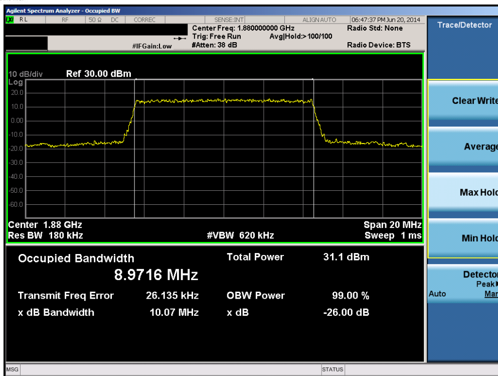
Plot 6-13. Occupied Bandwidth Plot (Band 2 – 10.0MHz QPSK – RB Size 50)
