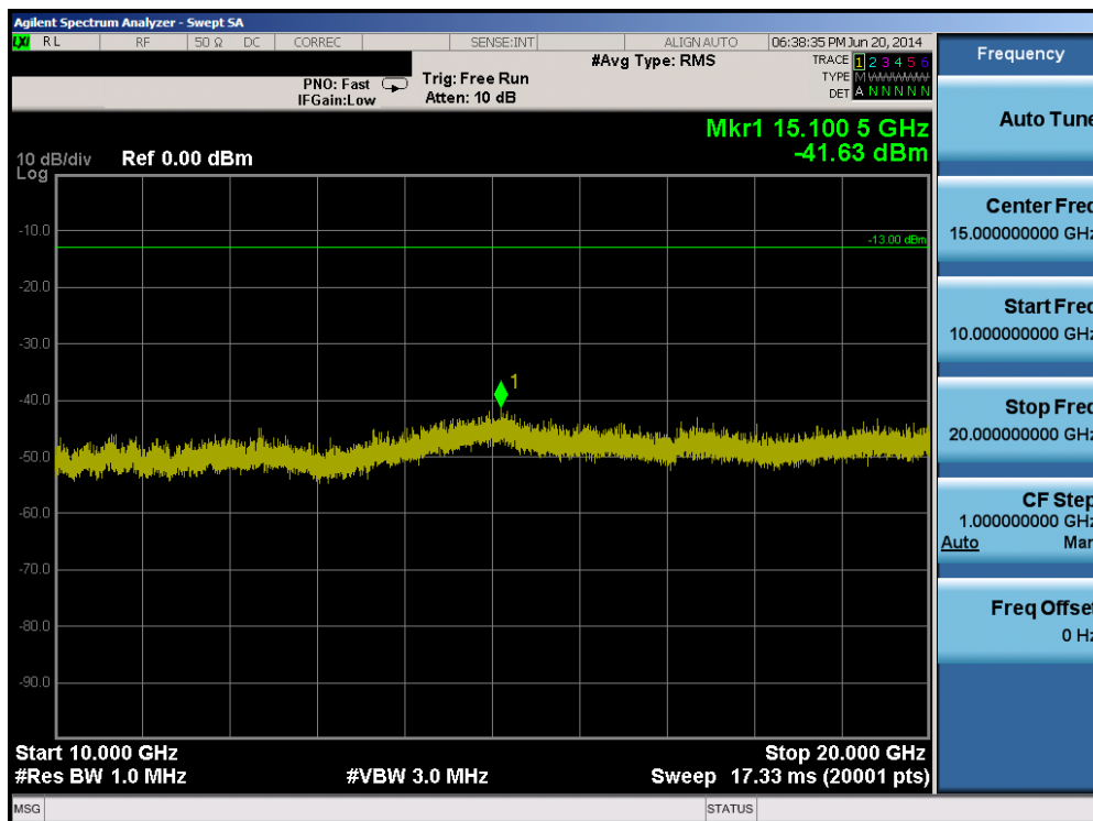
Plot 6-30. Conducted Spurious Plot (Band 2 – 5.0MHz QPSK – RB Size 1, RB Offset 0 – Mid Channel)
