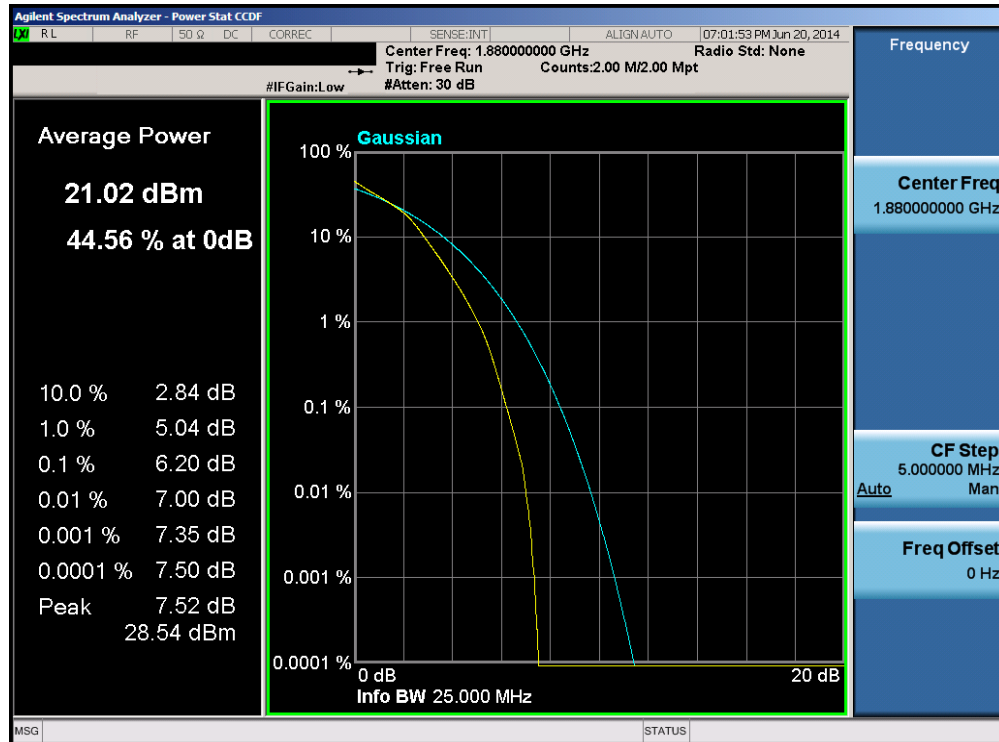
Plot 6-82. PAR Plot (Band 2 – 20.0MHz 16-QAM – RB Size 100)
