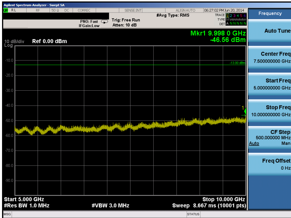
Plot 6-20. Conducted Spurious Plot (Band 13 – 10.0MHz QPSK – RB Size 1, RB Offset 0)
