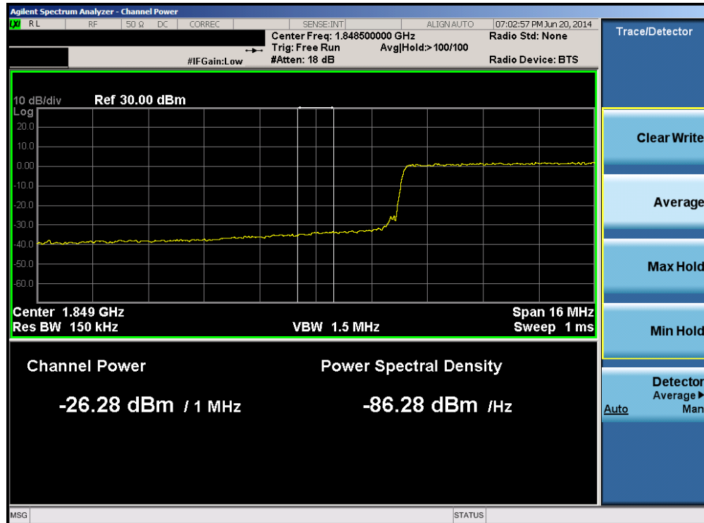
Plot 6-64. Lower Extended Band Edge Plot (Band 2 – 20.0MHz QPSK – RB Size 100)
