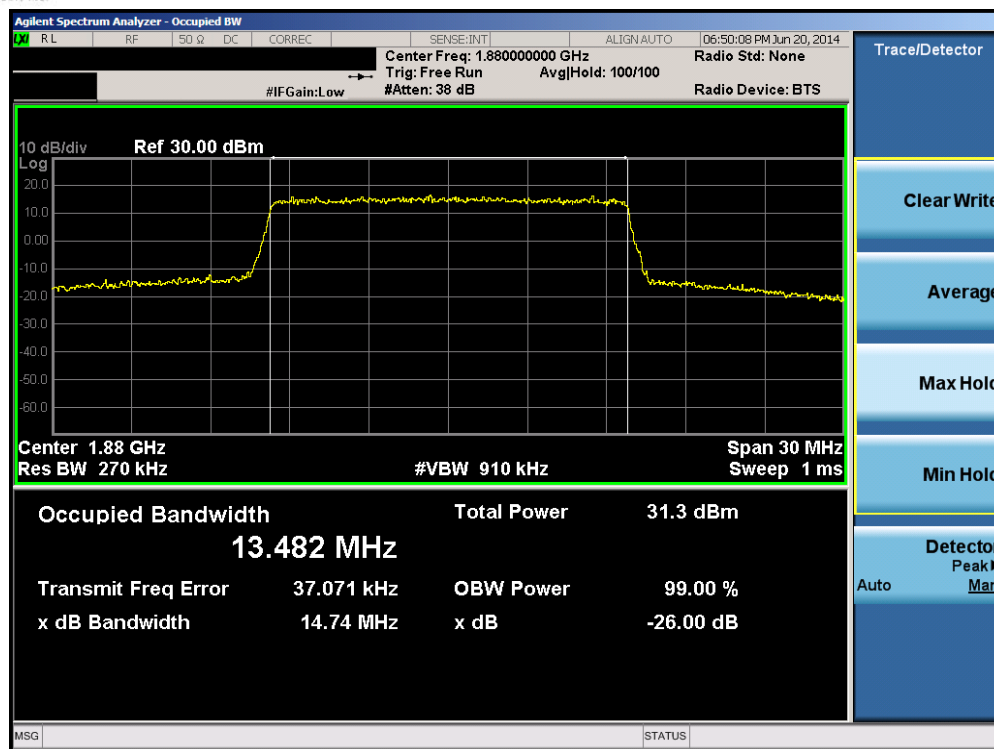
Plot 6-15. Occupied Bandwidth Plot (Band 2 – 15.0MHz QPSK – RB Size 75)
