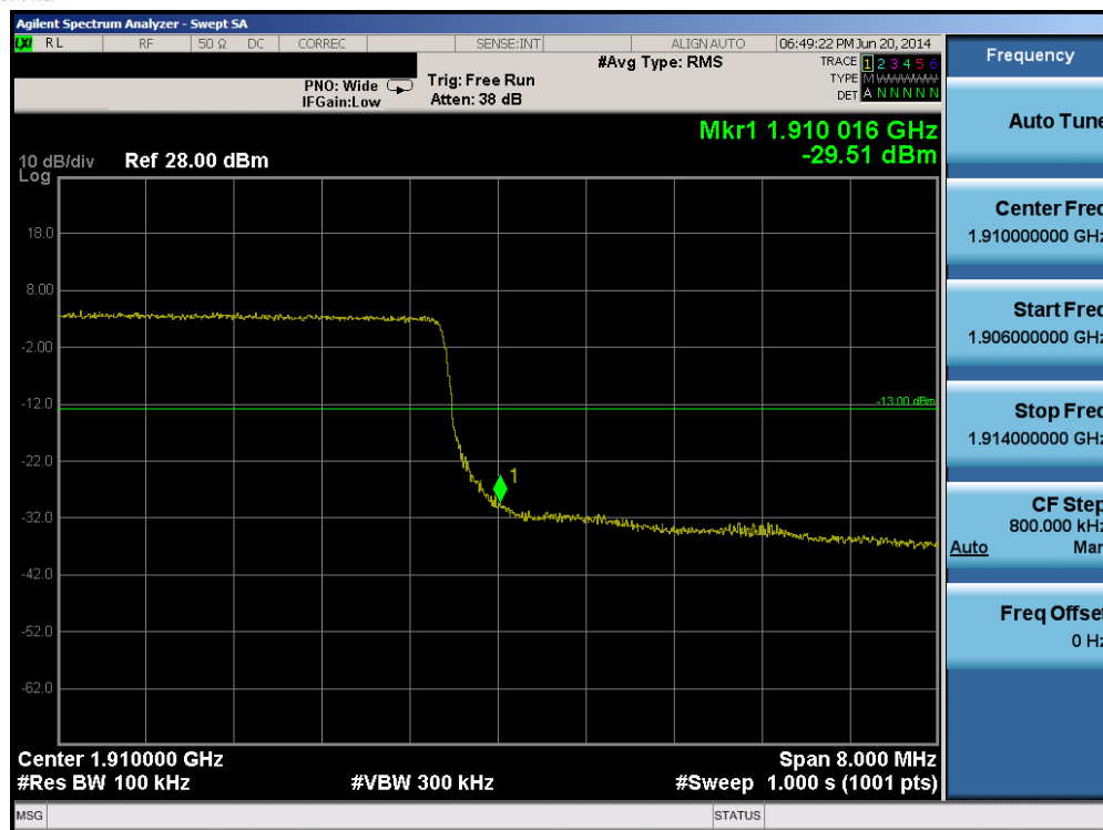
Plot 6-57. Upper Band Edge Plot (Band 2 – 10.0MHz QPSK – RB Size 50)
