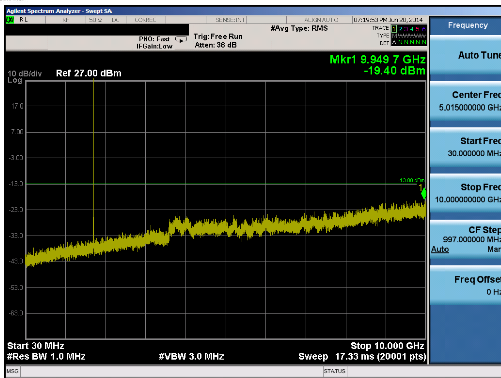
Plot 6-23. Conducted Spurious Plot (Band 4 – 5.0MHz QPSK – RB Size 1, RB Offset 0 – Mid Channel)
