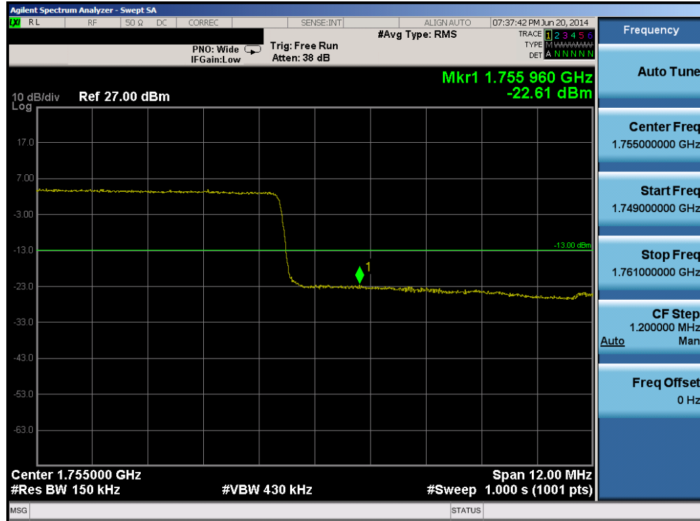
Plot 6-45. Upper Band Edge Plot (Band 4 – 15.0MHz QPSK – RB Size 75)
