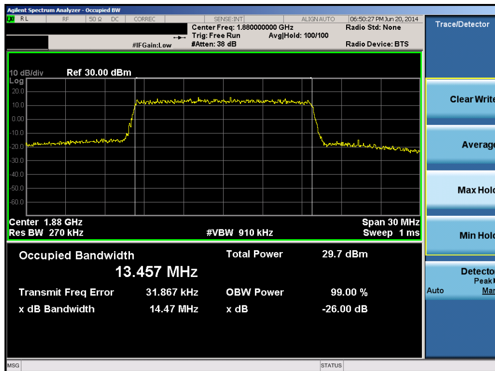
Plot 6-16. Occupied Bandwidth Plot (Band 2 – 15.0MHz 16-QAM – RB Size 75)
