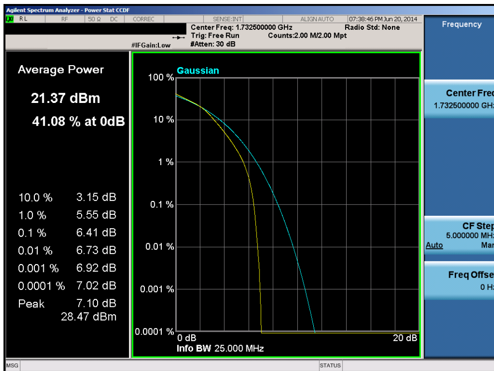
Plot 6-74. PAR Plot (Band 4 – 20.0MHz 16-QAM – RB Size 100)
