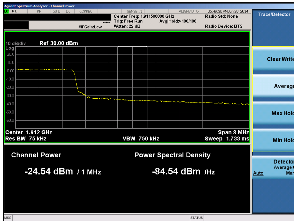
Plot 6-58. Upper Extended Band Edge Plot (Band 2 – 10.0MHz QPSK – RB Size 50)
