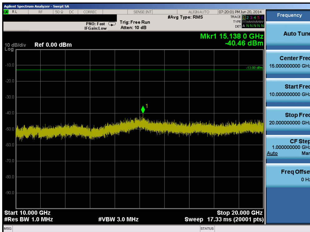
Plot 6-24. Conducted Spurious Plot (Band 4 – 5.0MHz OPSK – RB Size 1, RB Offset 0 – Mid Channel)
