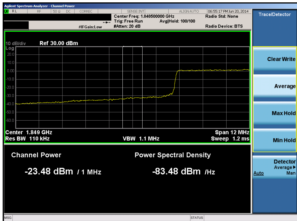
Plot 6-60. Lower Extended Band Edge Plot (Band 2 – 15.0MHz QPSK – RB Size 75)
