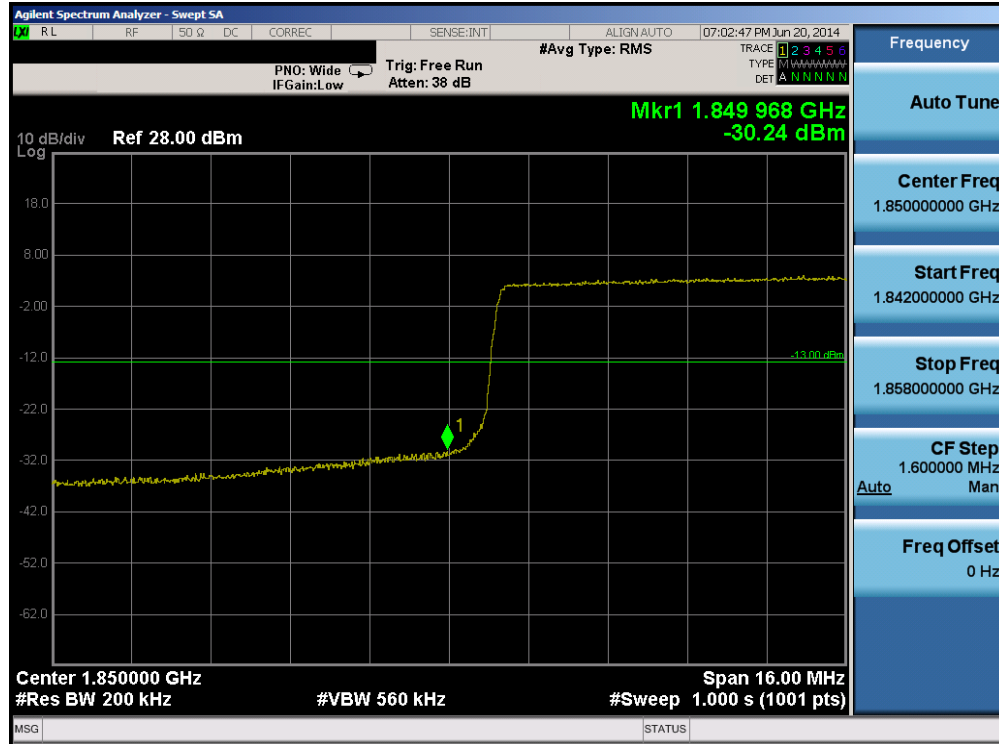
Plot 6-63. Lower Band Edge Plot (Band 2 – 20.0MHz QPSK – RB Size 100)
