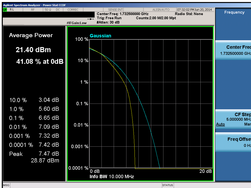
Plot 6-70. PAR Plot (Band 4 – 10.0MHz 16-QAM – RB Size 50)
