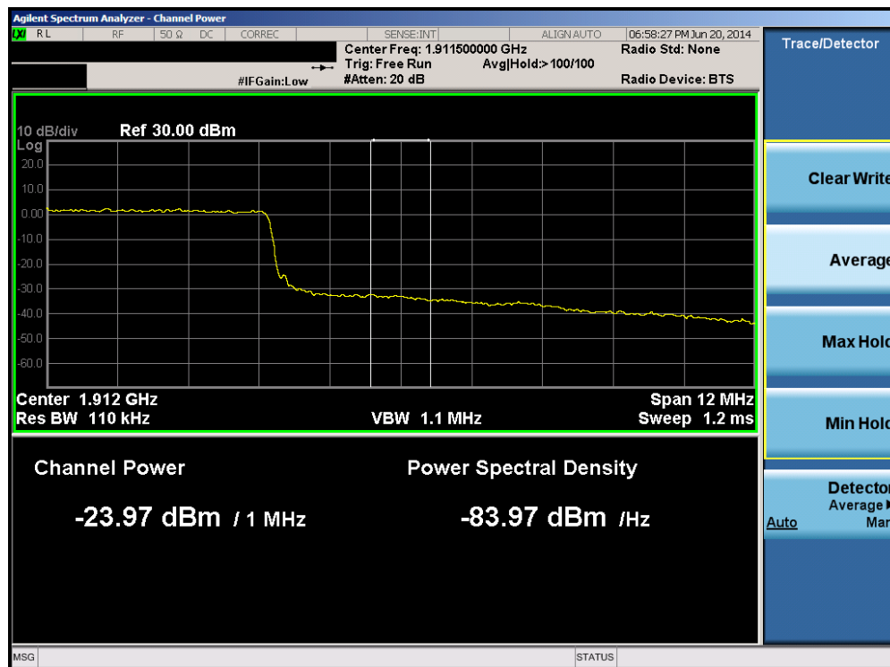
Plot 6-62. Upper Extended Band Edge Plot (Band 2 – 15.0MHz QPSK – RB Size 75)
