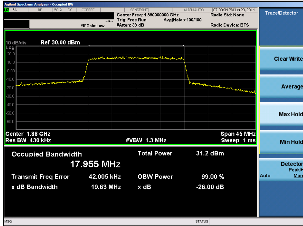
Plot 6-17. Occupied Bandwidth Plot (Band 2 – 20.0MHz QPSK – RB Size 100)
