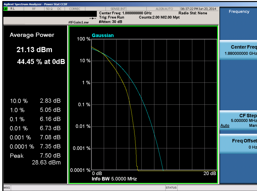
Plot 6-76. PAR Plot (Band 2 – 5.0MHz 16-QAM – RB Size 25)
