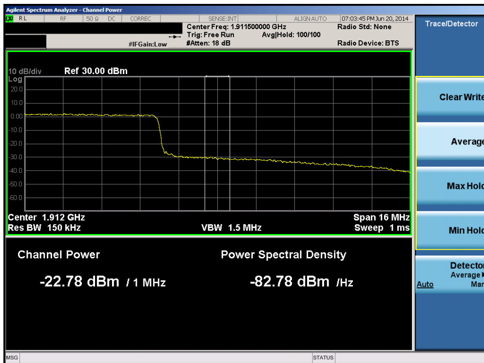
Plot 6-66. Upper Extended Band Edge Plot (Band 2 – 20.0MHz QPSK – RB Size 100)
