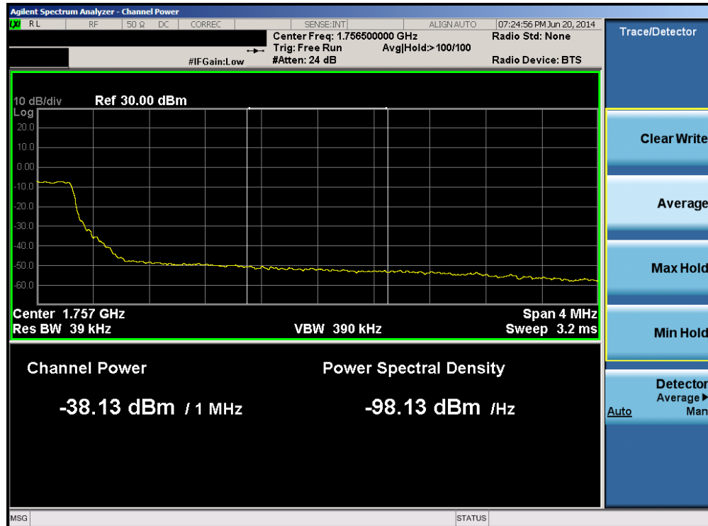
Plot 6-38. Upper Extended Band Edge Plot (Band 4 – 5.0MHz QPSK – RB Size 25)
