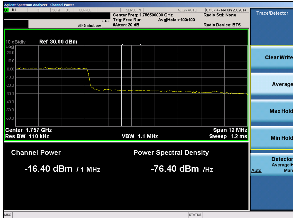
Plot 6-46. Upper Extended Band Edge Plot (Band 4 – 15.0MHz QPSK – RB Size 75)
