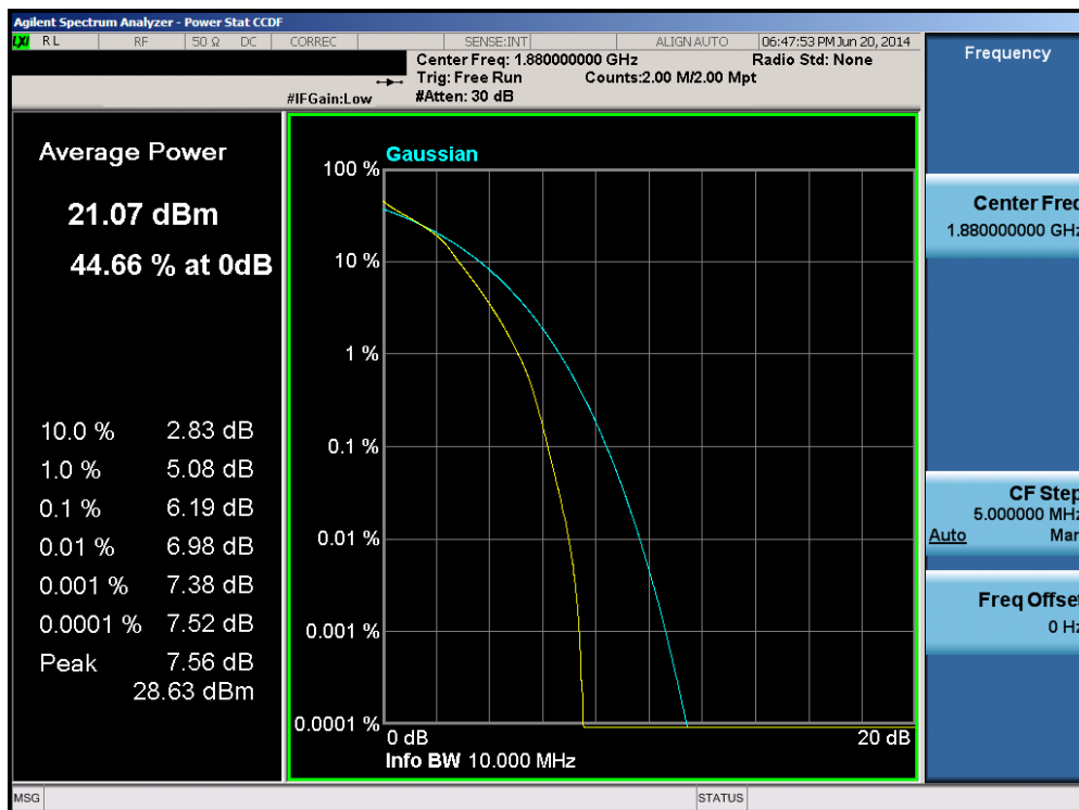
Plot 6-78. PAR Plot (Band 2 – 10.0MHz 16-QAM – RB Size 50)
