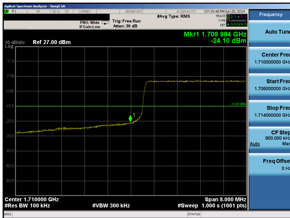
Plot 6-39. Lower Band Edge Plot (Band 4 – 10.0MHz QPSK – RB Size 50)
