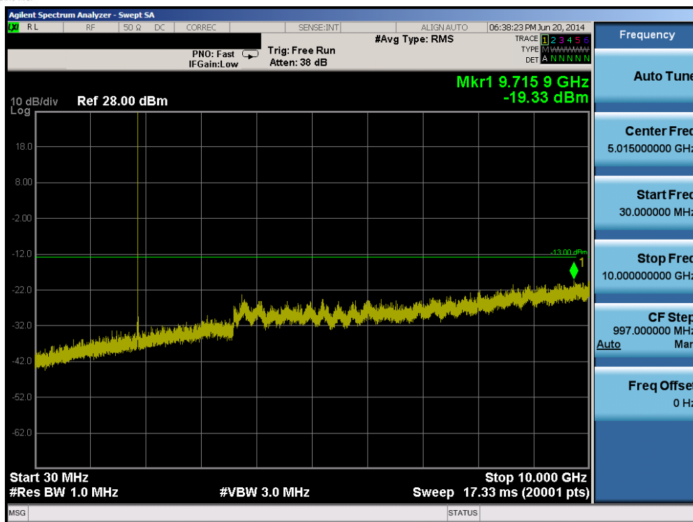
Plot 6-29. Conducted Spurious Plot (Band 2 – 5.0MHz QPSK – RB Size 1, RB Offset 0 – Mid Channel)
