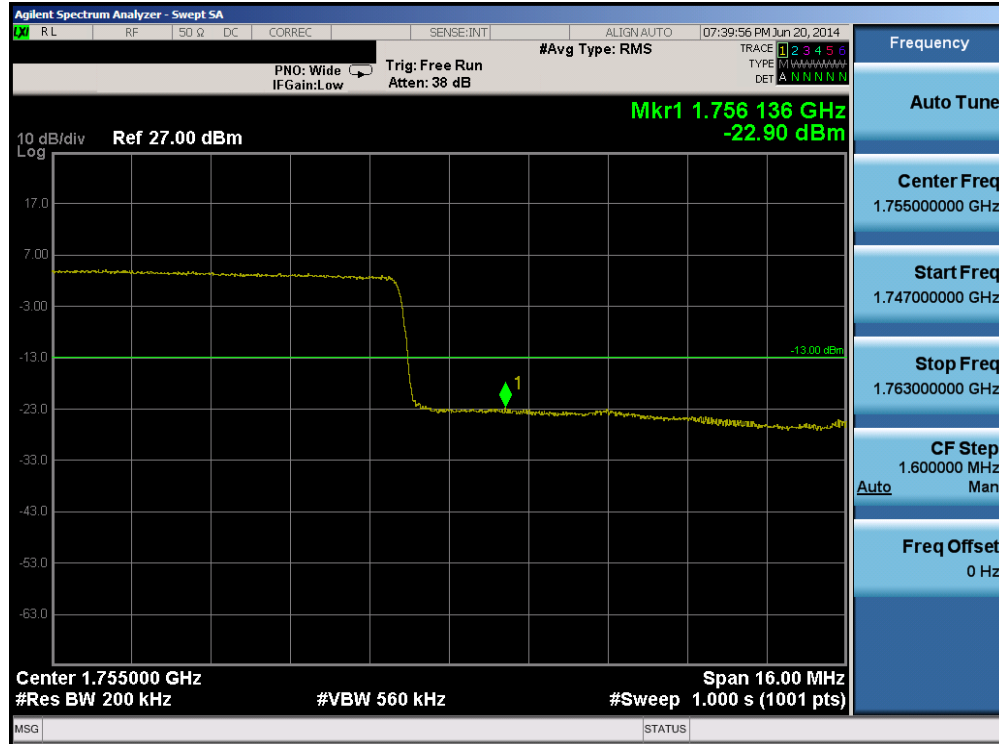
Plot 6-49. Upper Band Edge Plot (Band 4 – 20.0MHz QPSK – RB Size 100)
