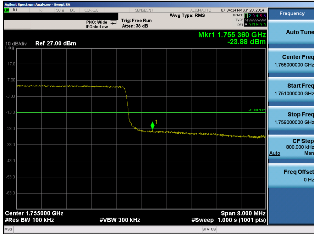
Plot 6-41. Upper Band Edge Plot (Band 4 – 10.0MHz QPSK – RB Size 50)
