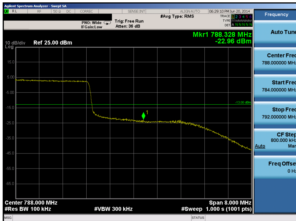
Plot 6-34. Upper Band Edge Plot (Band 13 – 10.0MHz QPSK – RB Size 50)
