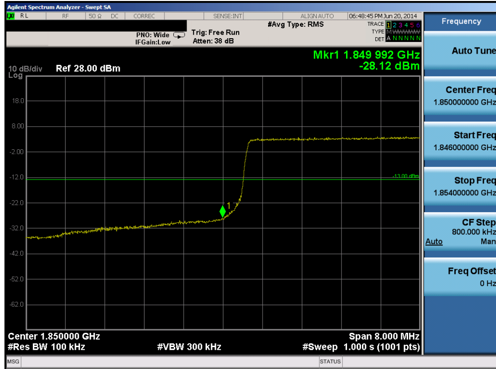
Plot 6-55. Lower Band Edge Plot (Band 2 – 10.0MHz QPSK – RB Size 50)
