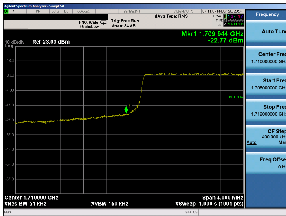
Plot 6-35. Lower Band Edge Plot (Band 4 – 5.0MHz QPSK – RB Size 25)
