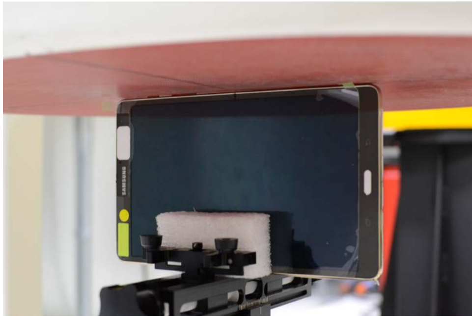
SAR Test Setup Photo 6: Right Edge at 0 mm
