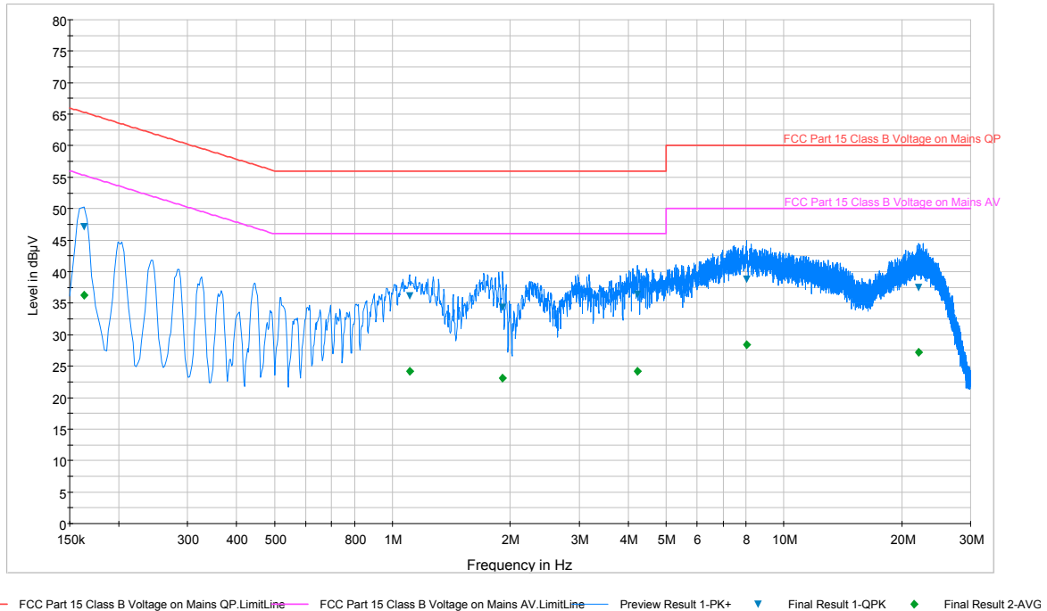
Plot 6-44. Line-Conducted Test Plot (L1)
