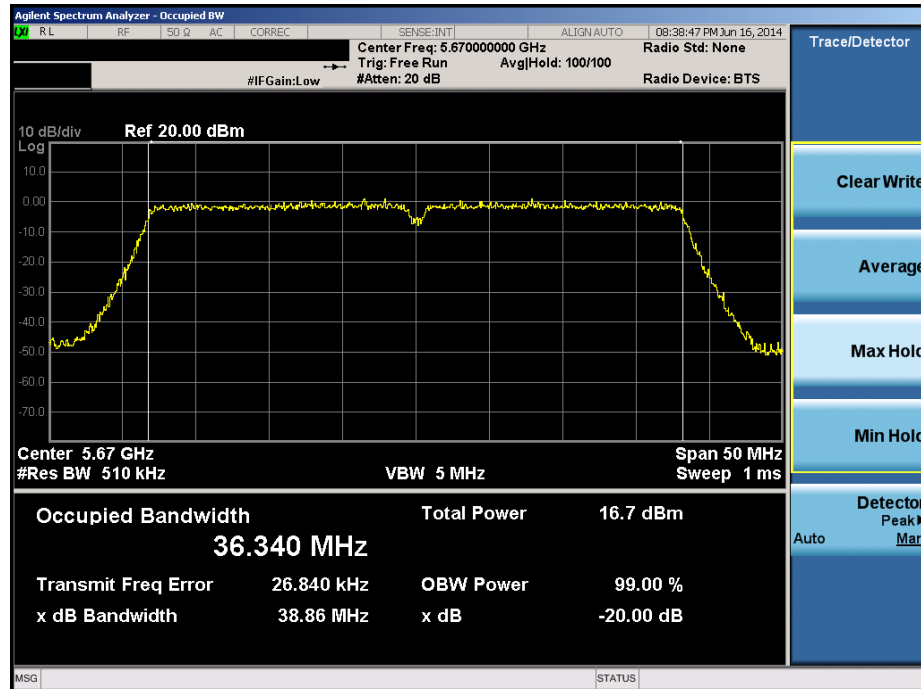
Plot 6-65. 20dB Bandwidth Plot (40MHz BW 802.11n (UNII Band 2C) – Ch. 134)
