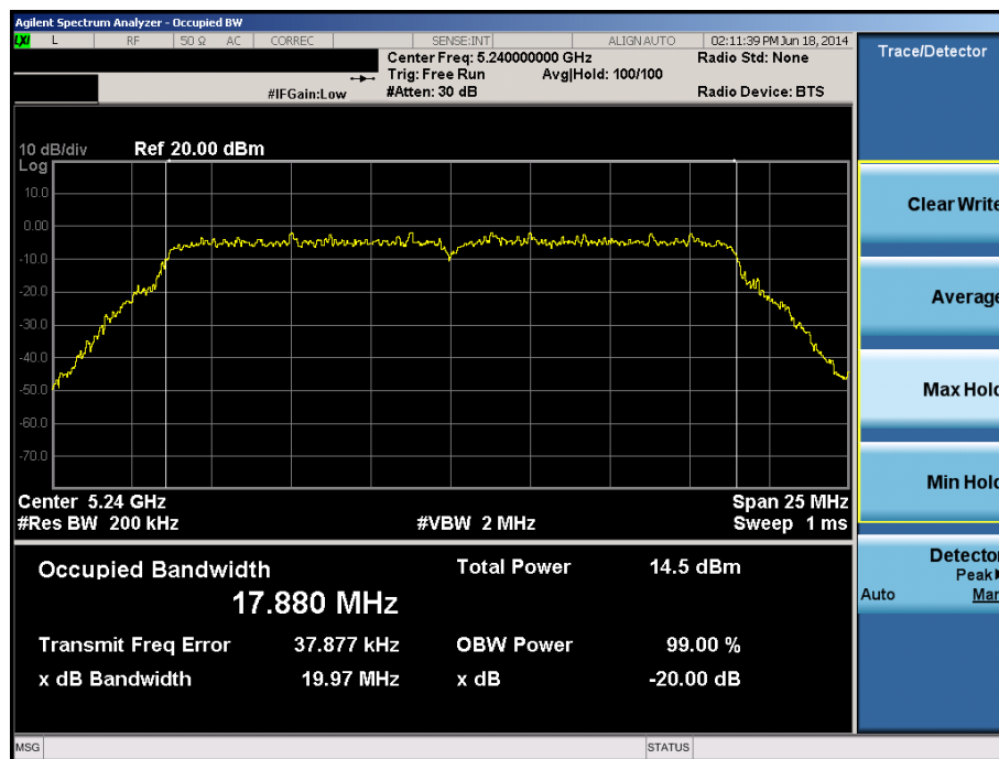
Plot 6-64. 20dB Bandwidth Plot (20MHz BW 802.11n (UNII Band 1) – Ch. 48)
