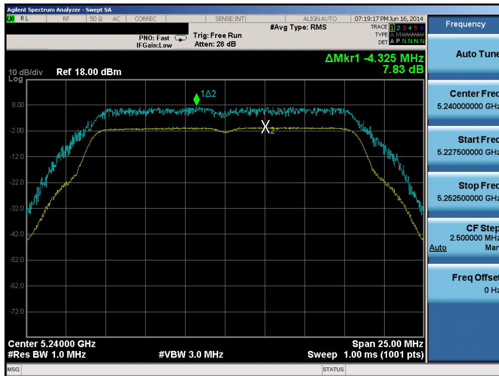
Plot 6-123. Peak Excursion Ratio Plot (802.11a (UNII Band 1) – Ch. 48)
