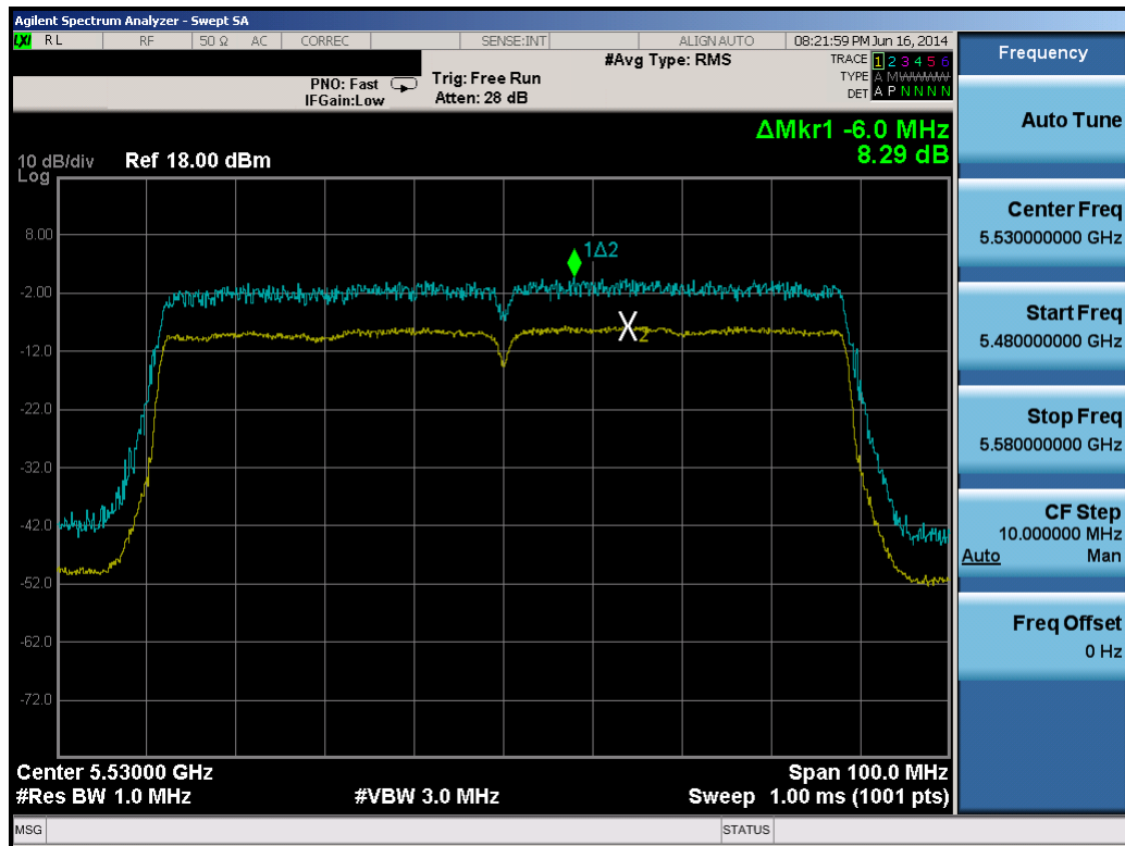
Plot 6-130. Peak Excursion Ratio Plot (80MHz BW 802.11ac (UNII Band 2C) – Ch. 106)
