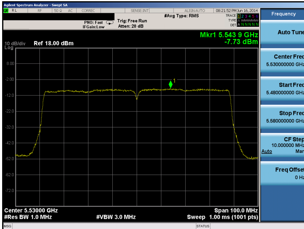
Plot 6-122. Peak Power Spectral Density Plot (80MHz BW 802.11ac (UNII Band 2C) – Ch. 106)
