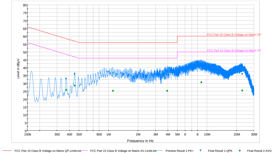
Plot 6-195. Line Conducted Plot with 802.11a UNII Band 2C (L1)
