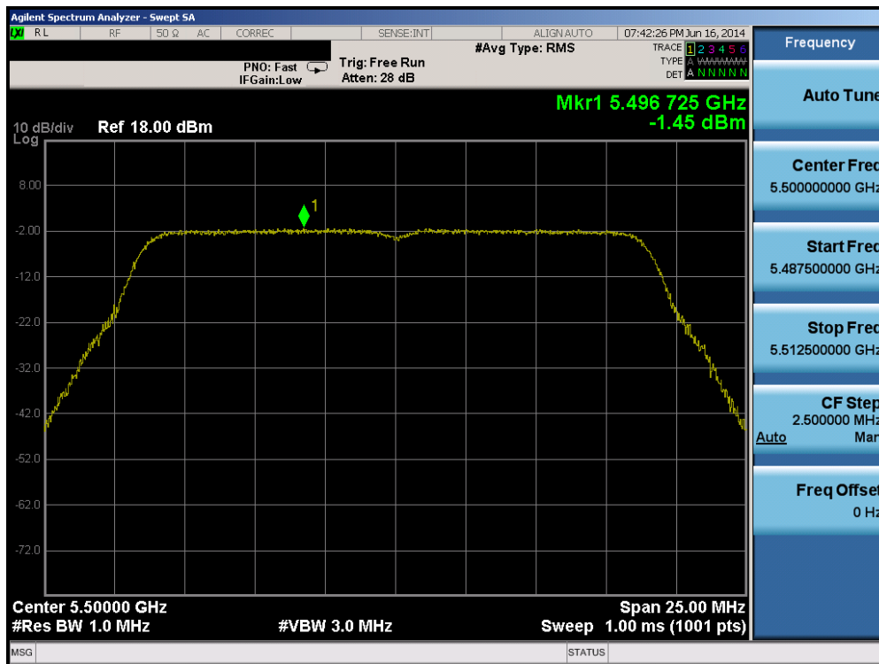
Plot 6-88. Peak Power Spectral Density Plot (20MHz BW 802.11n (UNII Band 2C) – Ch. 100)
