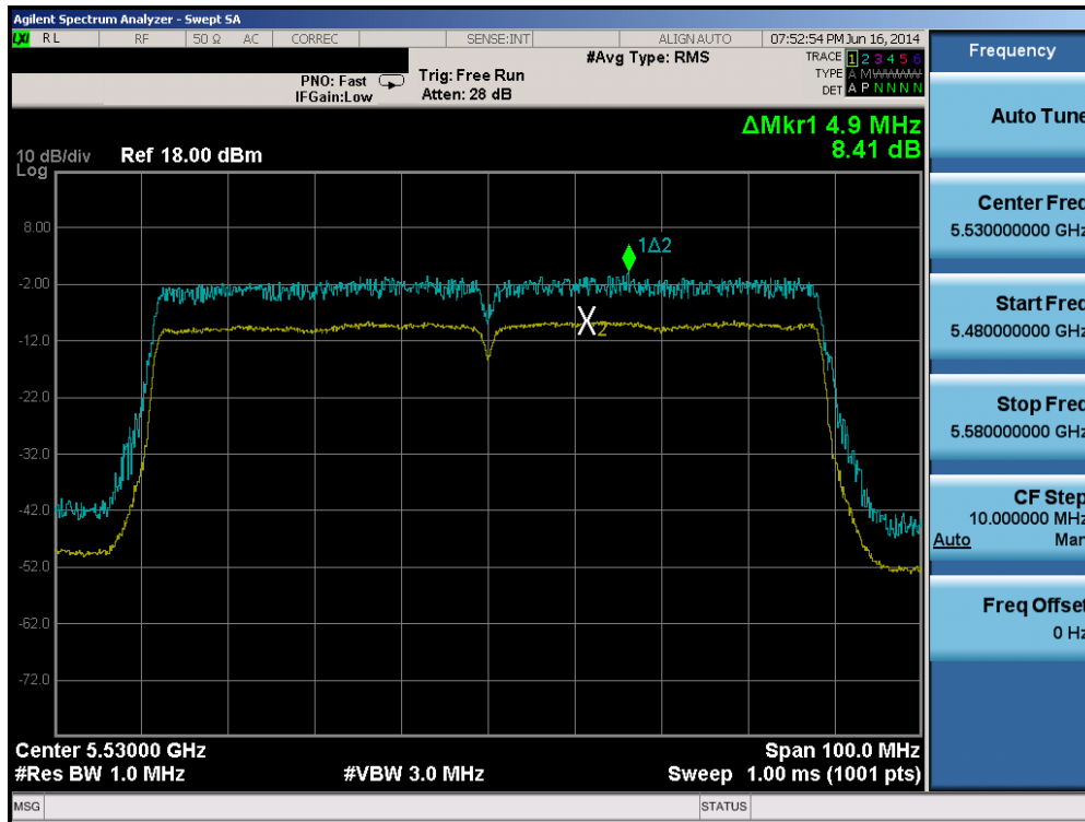
Plot 6-126. Peak Excursion Ratio Plot (80MHz BW 802.11ac (UNII Band 2C) – Ch. 106)
