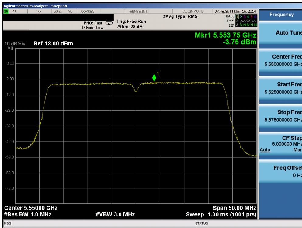
Plot 6-92. Peak Power Spectral Density Plot (40MHz BW 802.11n (UNII Band 2C) – Ch. 110)
