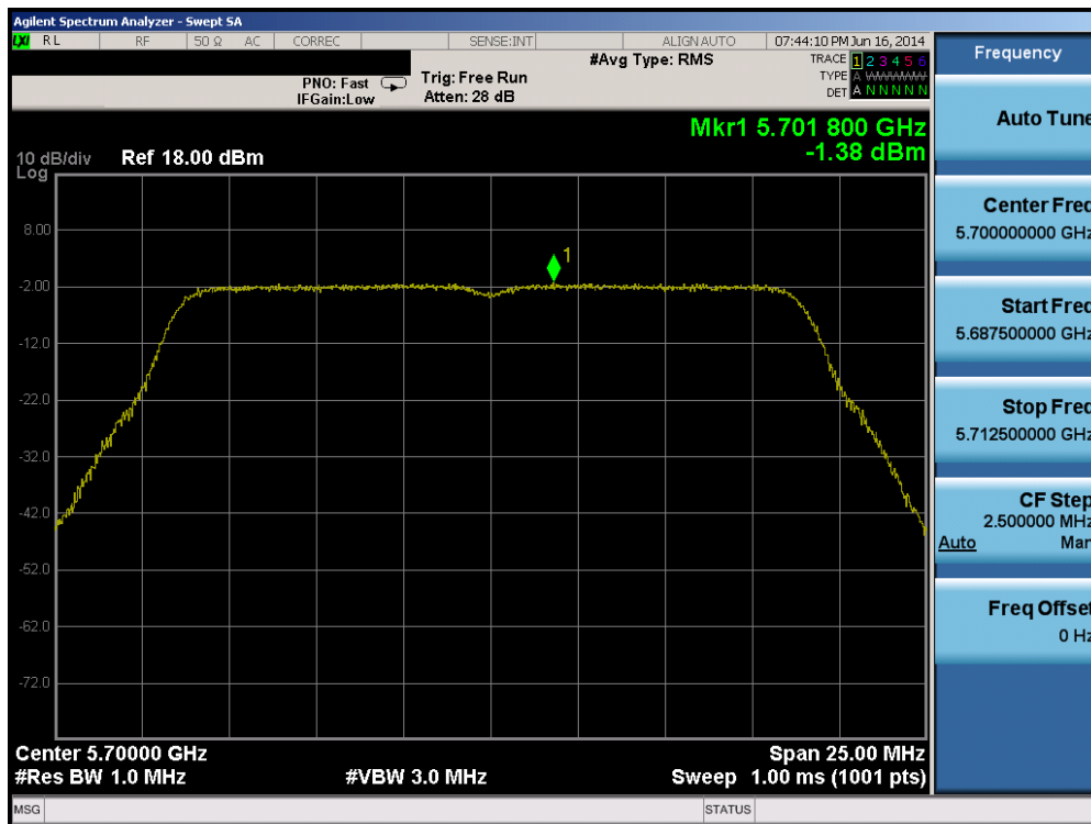
Plot 6-90. Peak Power Spectral Density Plot (20MHz BW 802.11n (UNII Band 2C) – Ch. 140)
