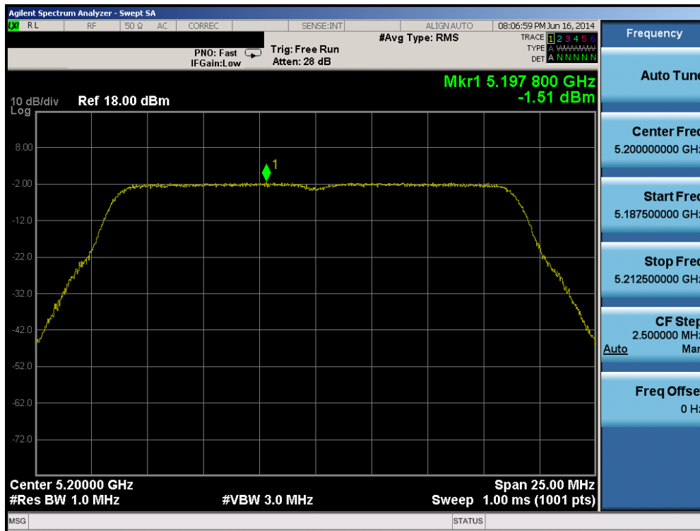
Plot 6-99. Peak Power Spectral Density Plot (20MHz BW 802.11n (UNII Band 1) – Ch. 40)
