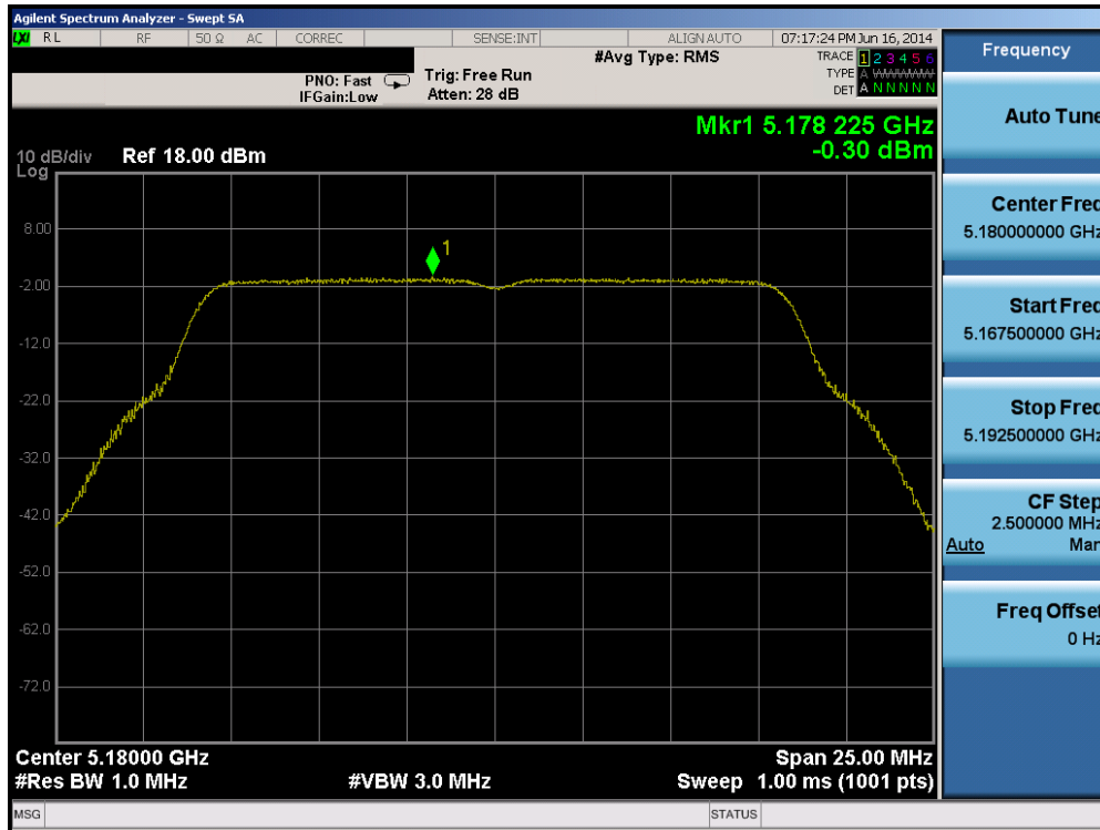
Plot 6-67. Peak Power Spectral Density Plot (802.11a (UNII Band 1) – Ch. 36)
