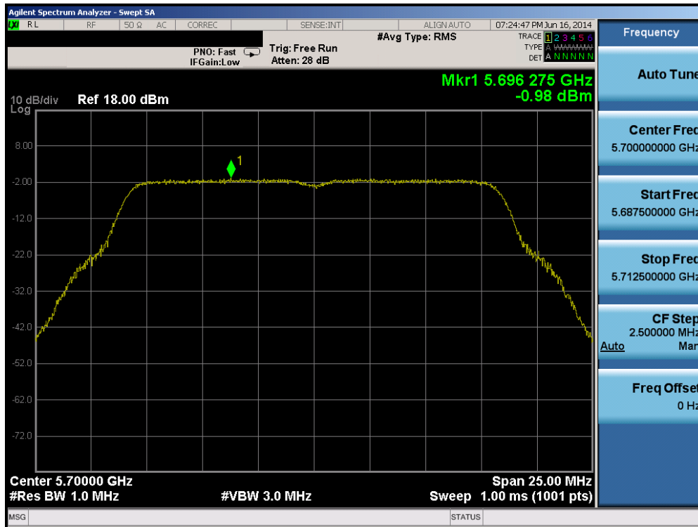
Plot 6-87. Peak Power Spectral Density Plot (802.11a (UNII Band 2C) – Ch. 140)
