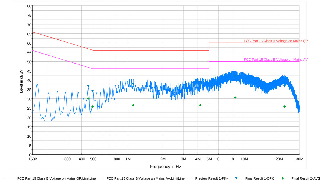
Plot 6-191. Line Conducted Plot with 802.11a UNII Band 1 (L1)
