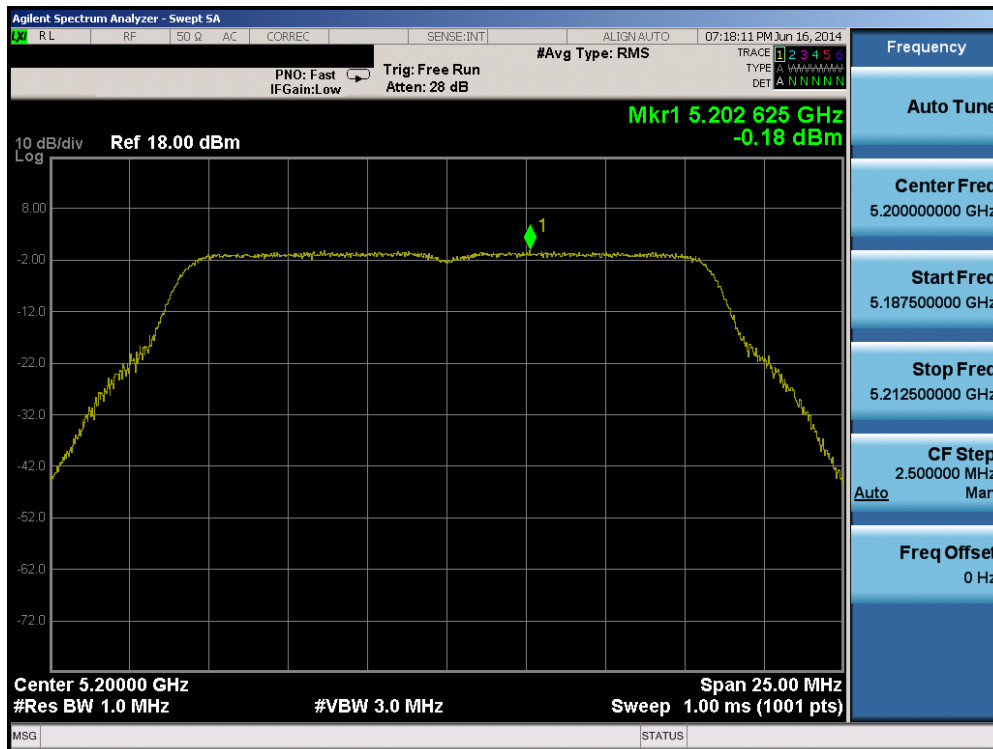
Plot 6-68. Peak Power Spectral Density Plot (802.11a (UNII Band 1) – Ch. 40)
