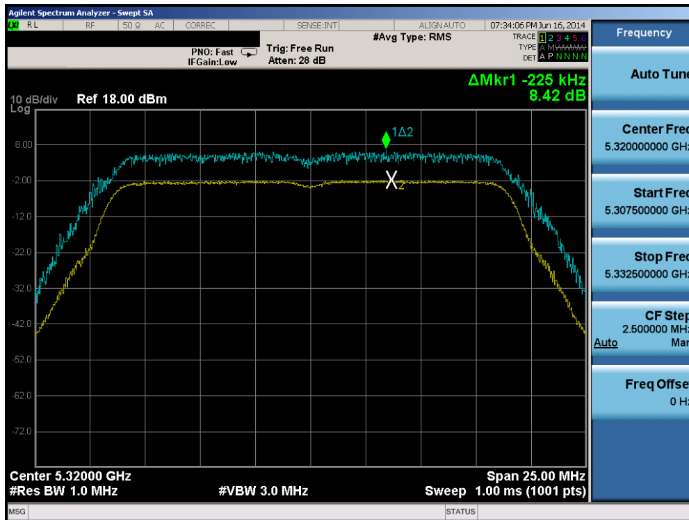
Plot 6-124. Peak Excursion Ratio Plot (20MHz BW 802.11n (UNII Band 2A) – Ch. 64)
