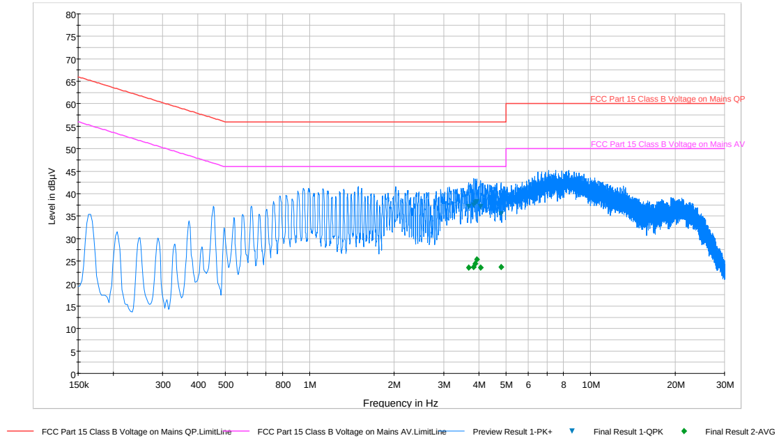
Plot 6-196. Line Conducted Plot with 802.11a UNII Band 2C (N)
