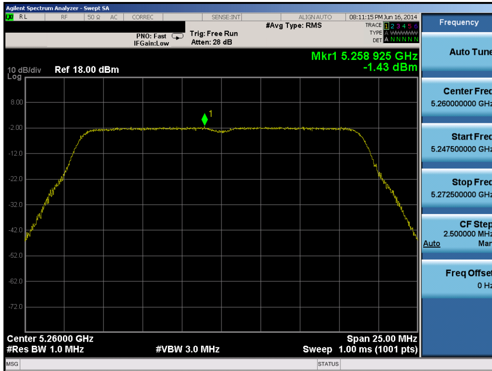
Plot 6-107. Peak Power Spectral Density Plot (20MHz BW 802.11n (UNII Band 2A) – Ch. 52)
