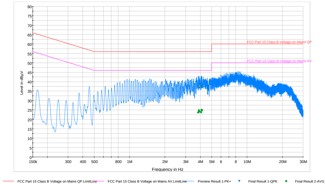
Plot 6-192. Line Conducted Plot with 802.11a UNII Band 1 (N)
