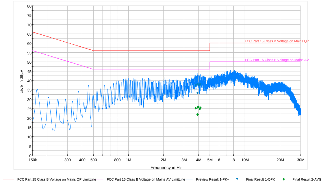
Plot 6-194. Line Conducted Plot with 802.11a UNII Band 2A (N)
