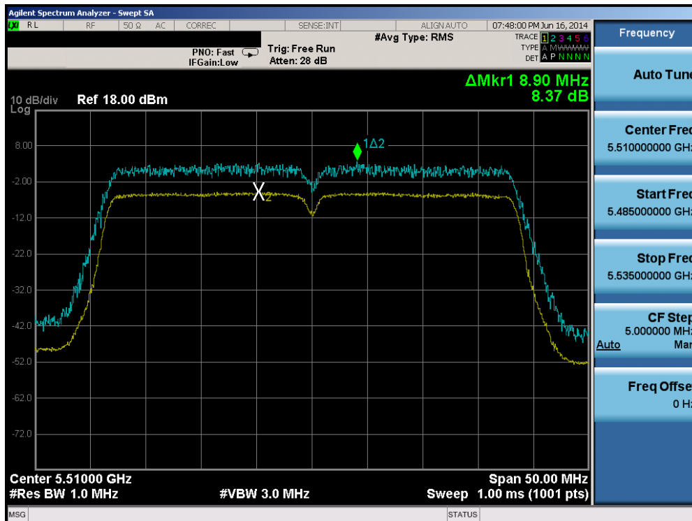
Plot 6-125. Peak Excursion Ratio Plot (40MHz BW 802.11n (UNII Band 2C) – Ch. 102)
