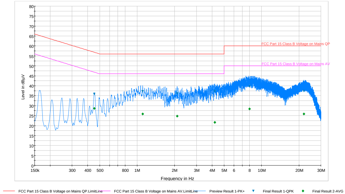
Plot 6-193. Line Conducted Plot with 802.11a UNII Band 2A (L1)
