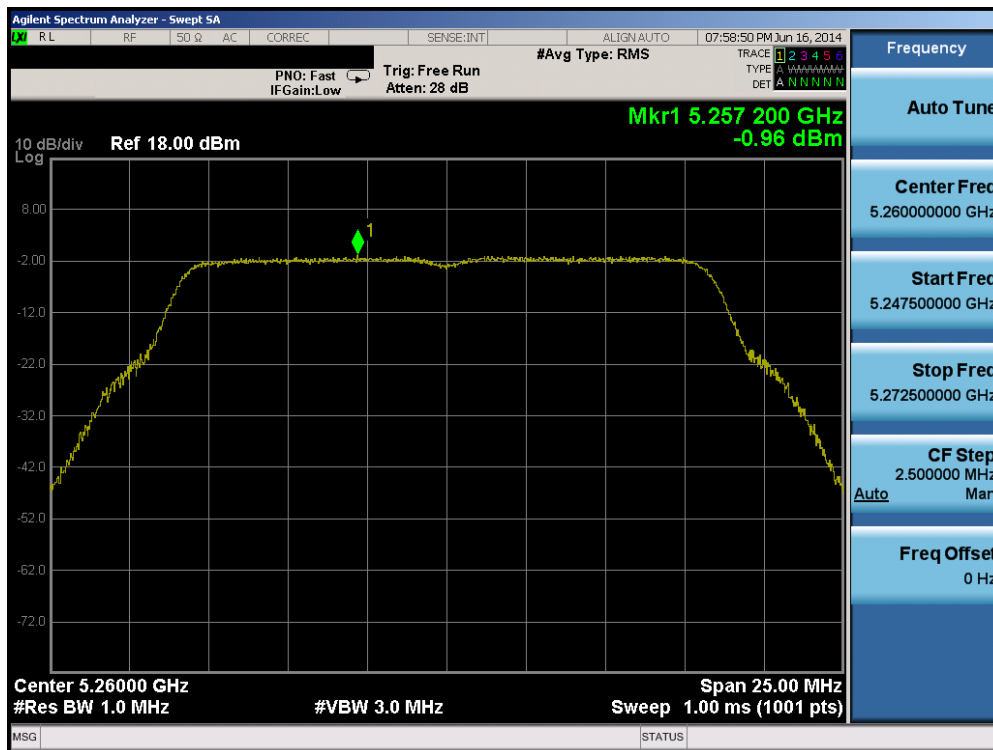
Plot 6-104. Peak Power Spectral Density Plot (802.11a (UNII Band 2A) – Ch. 52)
