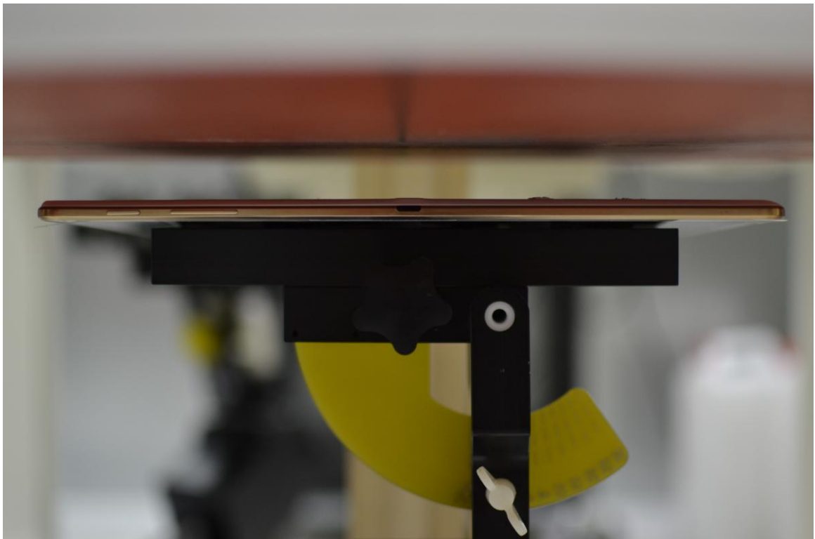
SAR Test Setup Photo 2: Back at 2.1 cm
