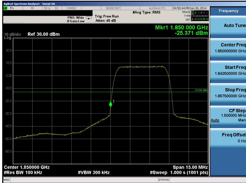
Plot 6-28. Band Edge Plot (PCS WCDMA Mode – Ch. 9262)
