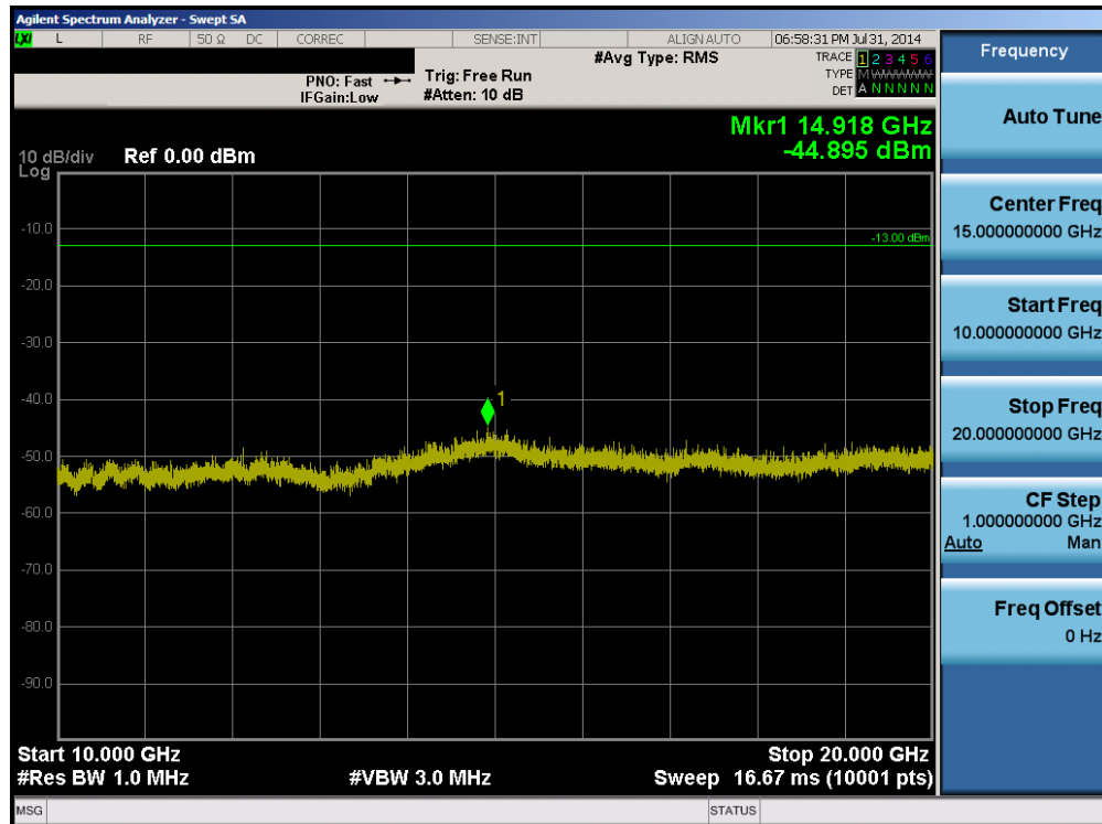
Plot 6-11. Conducted Spurious Plot (AWS WCDMA Mode – Ch. 1312)
