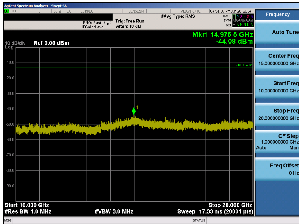
Plot 6-17. Conducted Spurious Plot (PCS WCDMA Mode – Ch. 9262)
