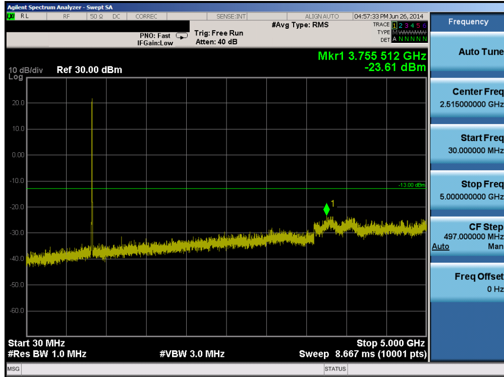
Plot 6-8. Conducted Spurious Plot (Cellular WCDMA Mode – Ch. 4233)
