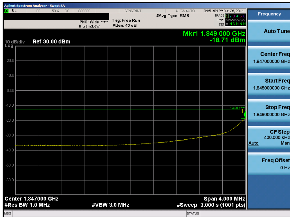
Plot 6-29. 4MHz Span Plot (PCS WCDMA Mode – Ch. 9262)
