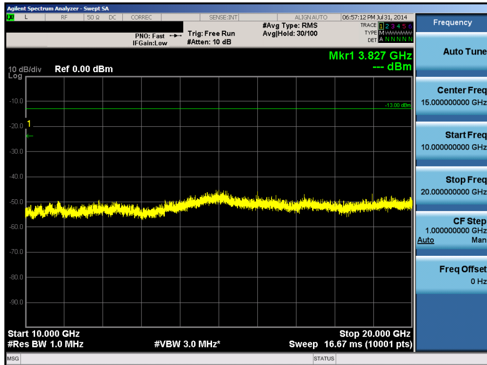
Plot 6-13. Conducted Spurious Plot (AWS WCDMA Mode – Ch. 1412)
