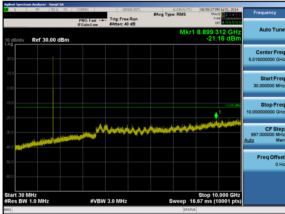
Plot 6-10. Conducted Spurious Plot (AWS WCDMA Mode – Ch. 1312)
