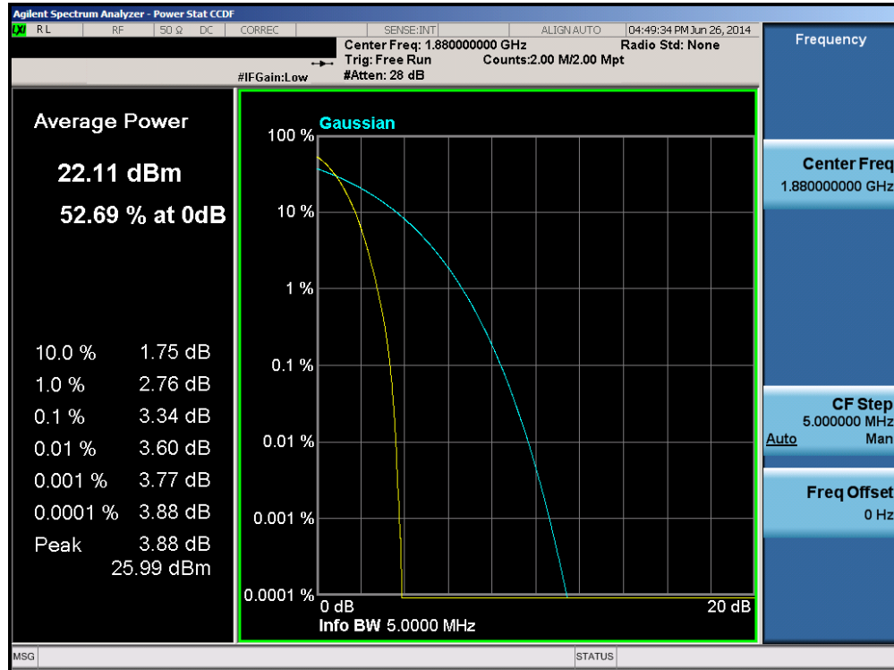
Plot 6-32. Peak-Average Ratio Plot (PCS WCDMA Mode – Ch. 9400)
