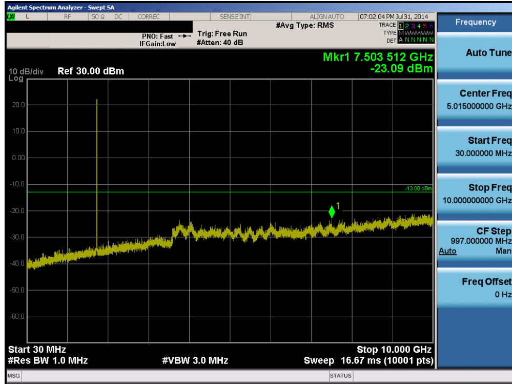
Plot 6-14. Conducted Spurious Plot (AWS WCDMA Mode – Ch. 1862)
