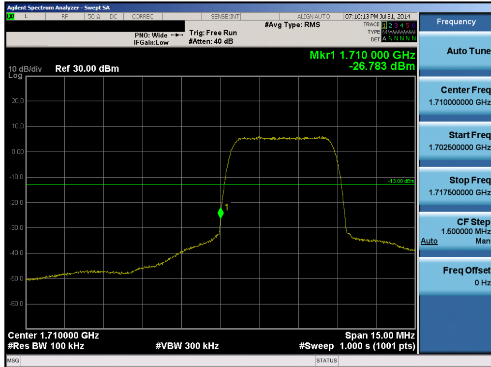
Plot 6-24. Band Edge Plot (AWS WCDMA Mode – Ch. 1312)
