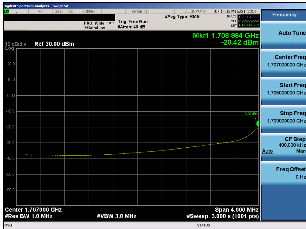
Plot 6-25. 4MHz Span Plot (AWS WCDMA Mode – Ch. 1312)
