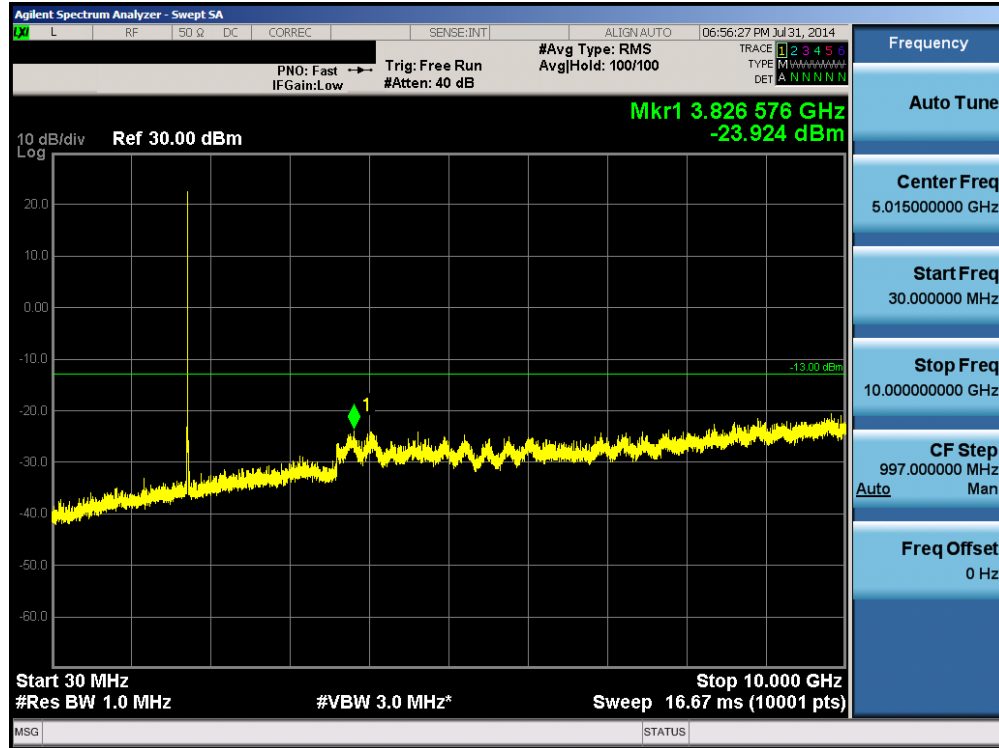
Plot 6-12. Conducted Spurious Plot (AWS WCDMA Mode – Ch. 1412)
