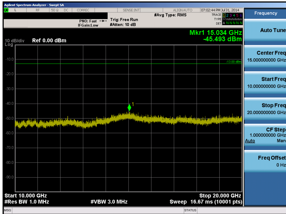
Plot 6-15. Conducted Spurious Plot (AWS WCDMA Mode – Ch. 1862)
