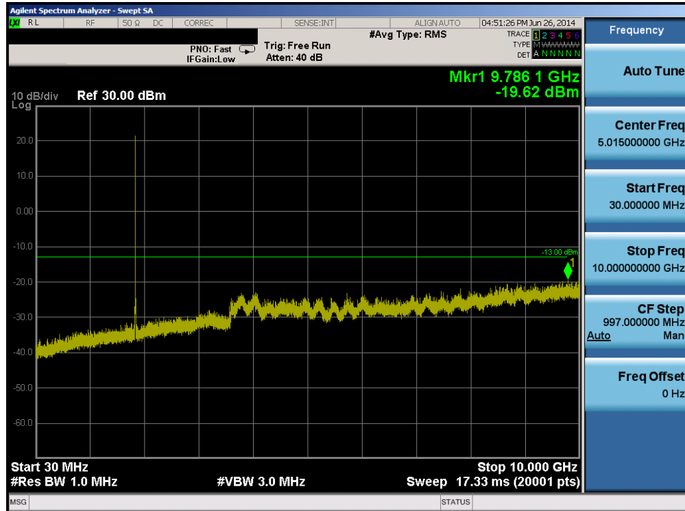
Plot 6-16. Conducted Spurious Plot (PCS WCDMA Mode – Ch. 9262)
