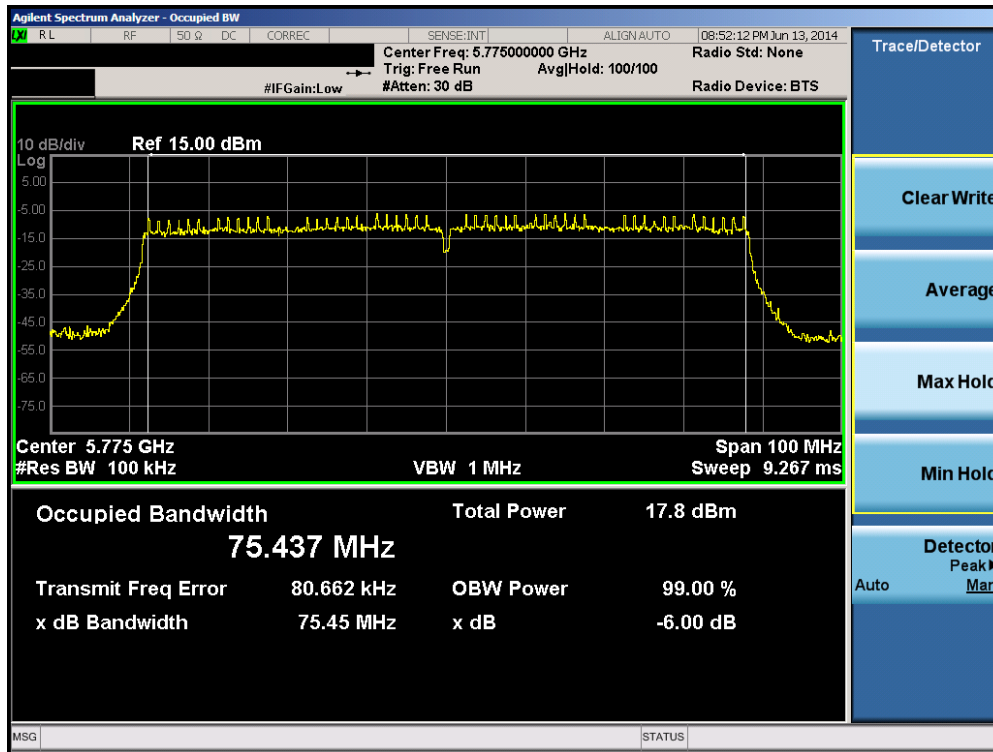
Plot 6-37. 6dB Bandwidth Plot (80MHz BW 802.11ac (5.8GHz) – Ch. 155)
