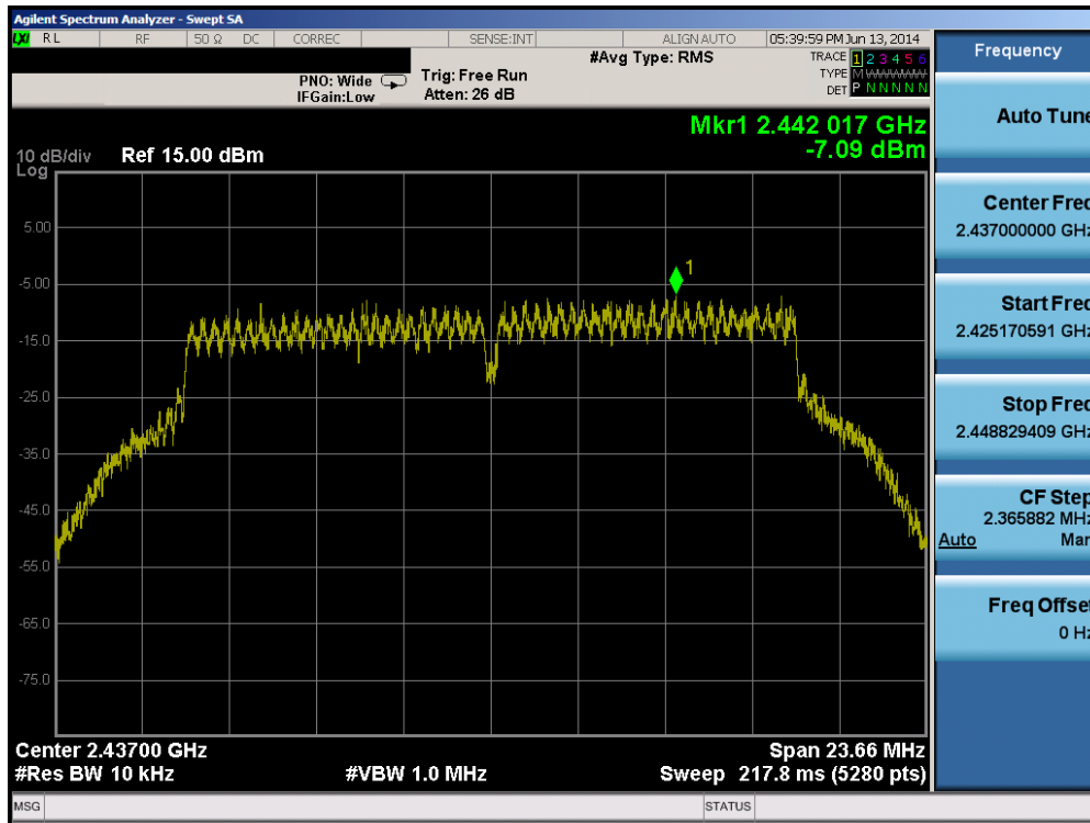
Plot 6-42. Power Spectral Density Plot (802.11g – Ch. 6)
