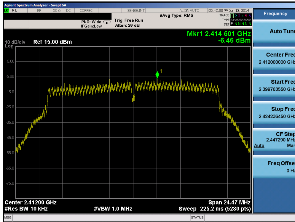
Plot 6-44. Power Spectral Density Plot (802.11n (2.4GHz) – Ch. 1)
