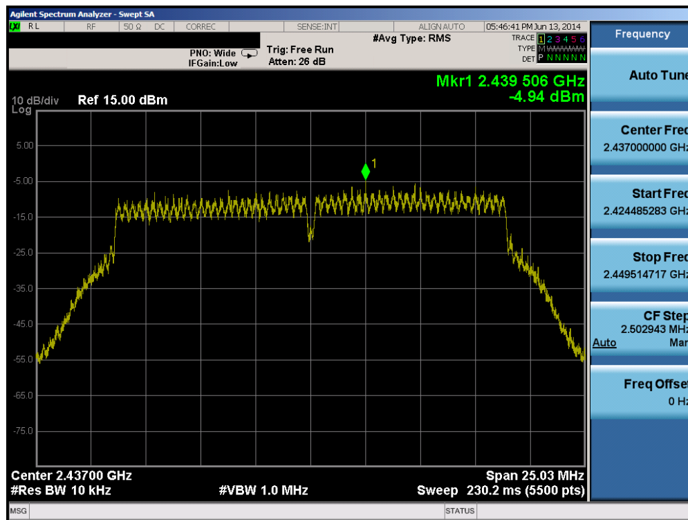
Plot 6-45. Power Spectral Density Plot (802.11n (2.4GHz) – Ch. 6)
