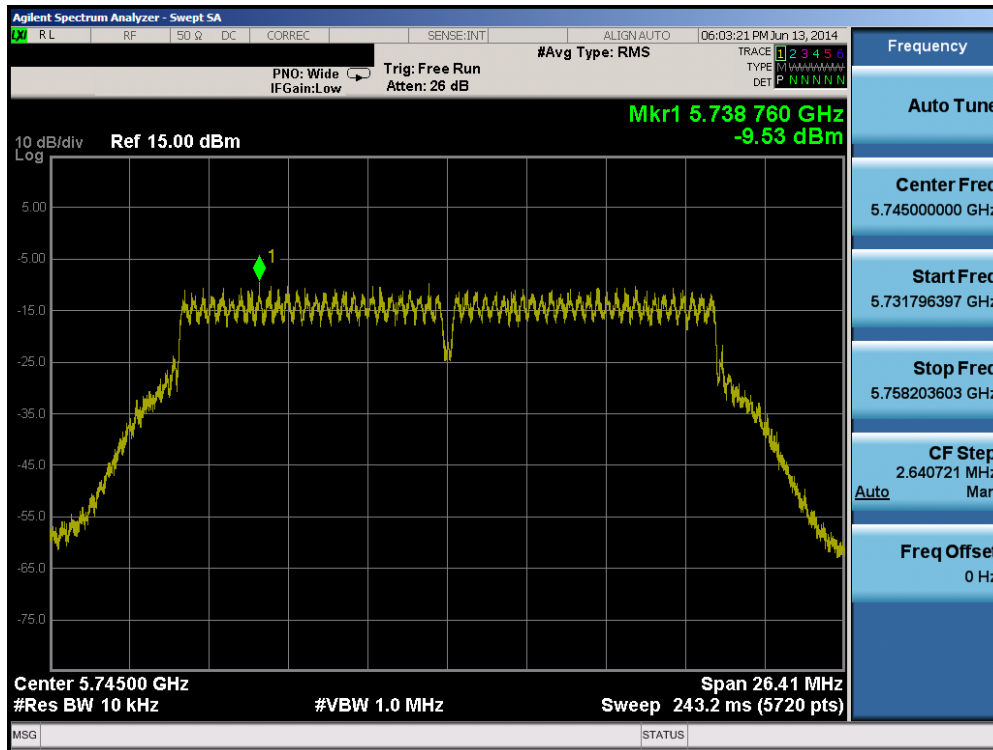
Plot 6-50. Power Spectral Density Plot (20MHz BW 802.11n (5.8GHz) – Ch. 149)
