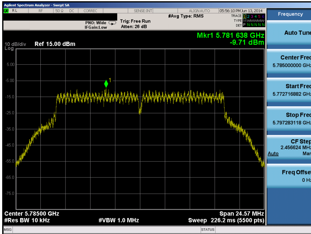
Plot 6-48. Power Spectral Density Plot (802.11a – Ch. 157)
