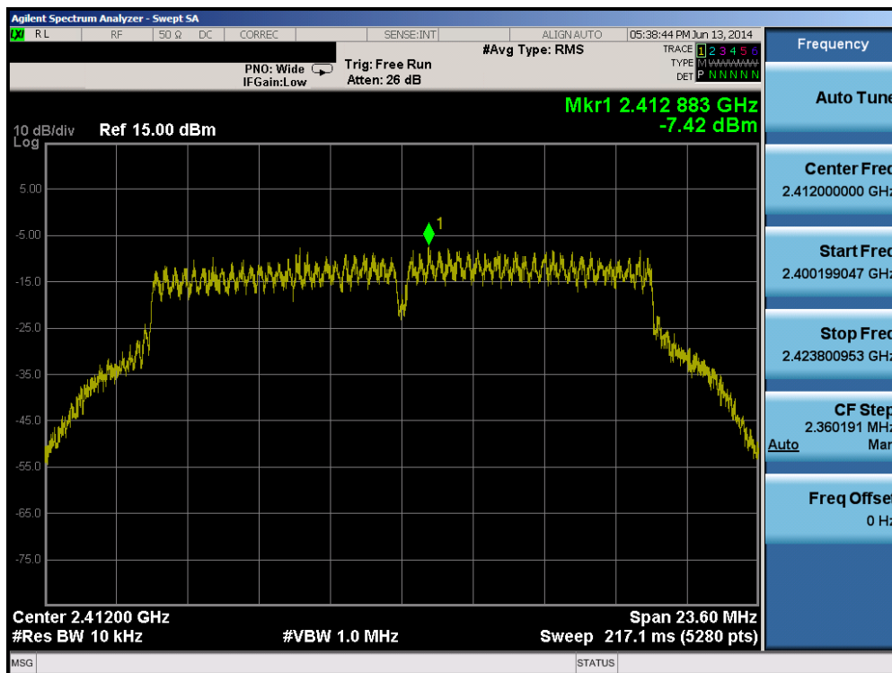
Plot 6-41. Power Spectral Density Plot (802.11g – Ch. 1)
