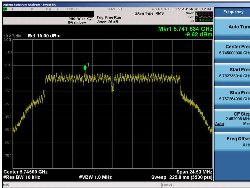
Plot 6-47. Power Spectral Density Plot (802.11a – Ch. 149)
