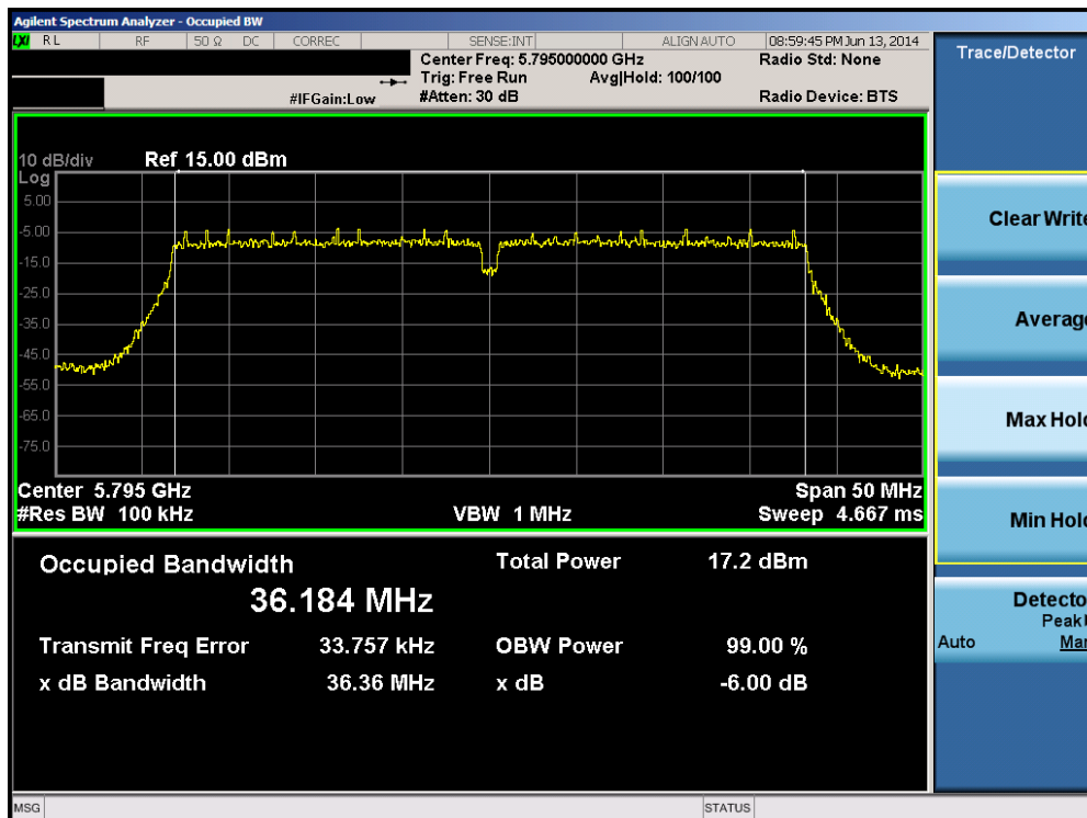
Plot 6-36. 6dB Bandwidth Plot (40MHz BW 802.11n (5.8GHz) – Ch. 159)
