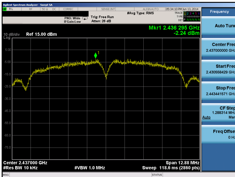
Plot 6-39. Power Spectral Density Plot (802.11b – Ch. 6)
