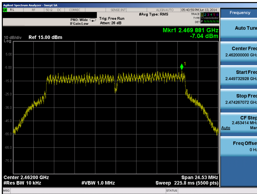
Plot 6-43. Power Spectral Density Plot (802.11g – Ch. 11)
