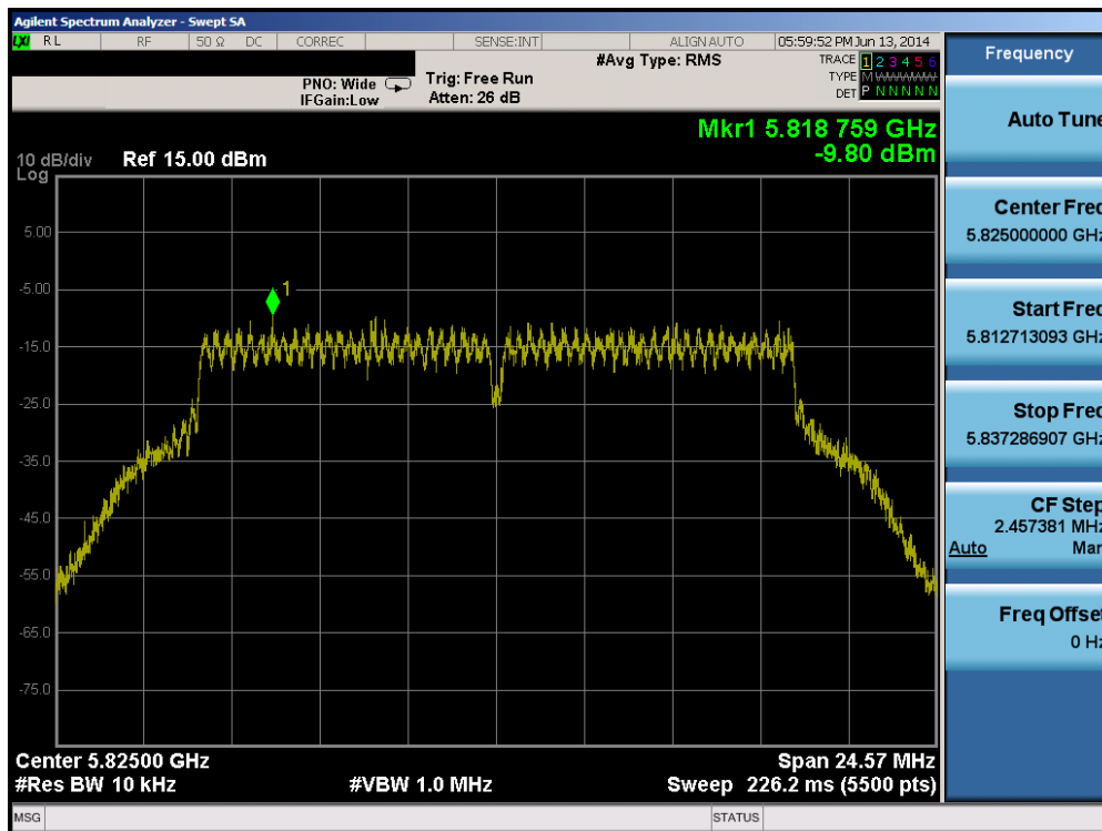
Plot 6-49. Power Spectral Density Plot (802.11a – Ch. 165)
