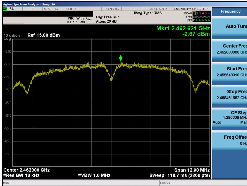
Plot 6-40. Power Spectral Density Plot (802.11b – Ch. 11)
