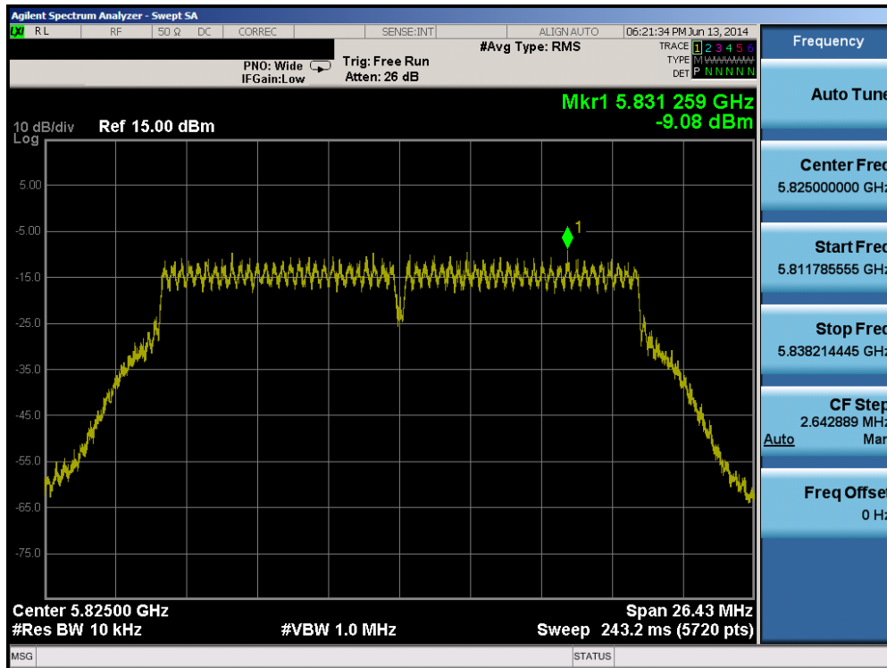
Plot 6-52. Power Spectral Density Plot (20MHz BW 802.11n (5.8GHz) – Ch. 165)
