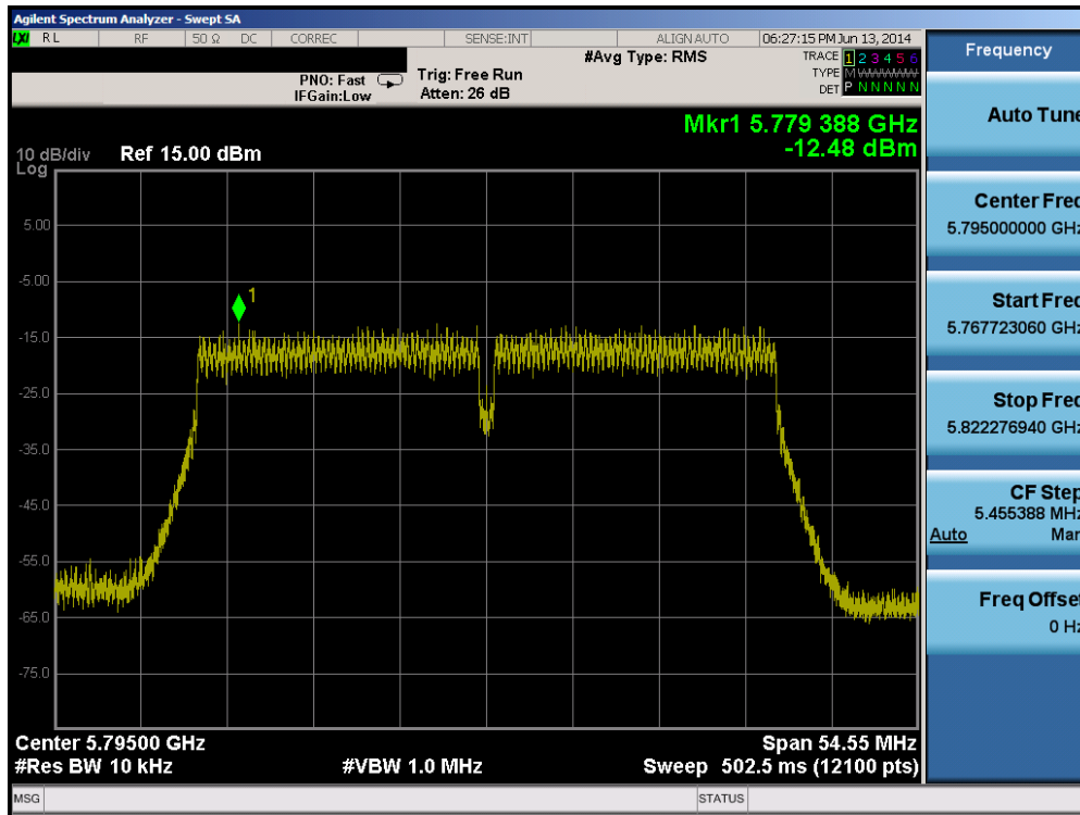
Plot 6-54. Power Spectral Density Plot (40MHz BW 802.11n (5.8GHz) – Ch. 159)
