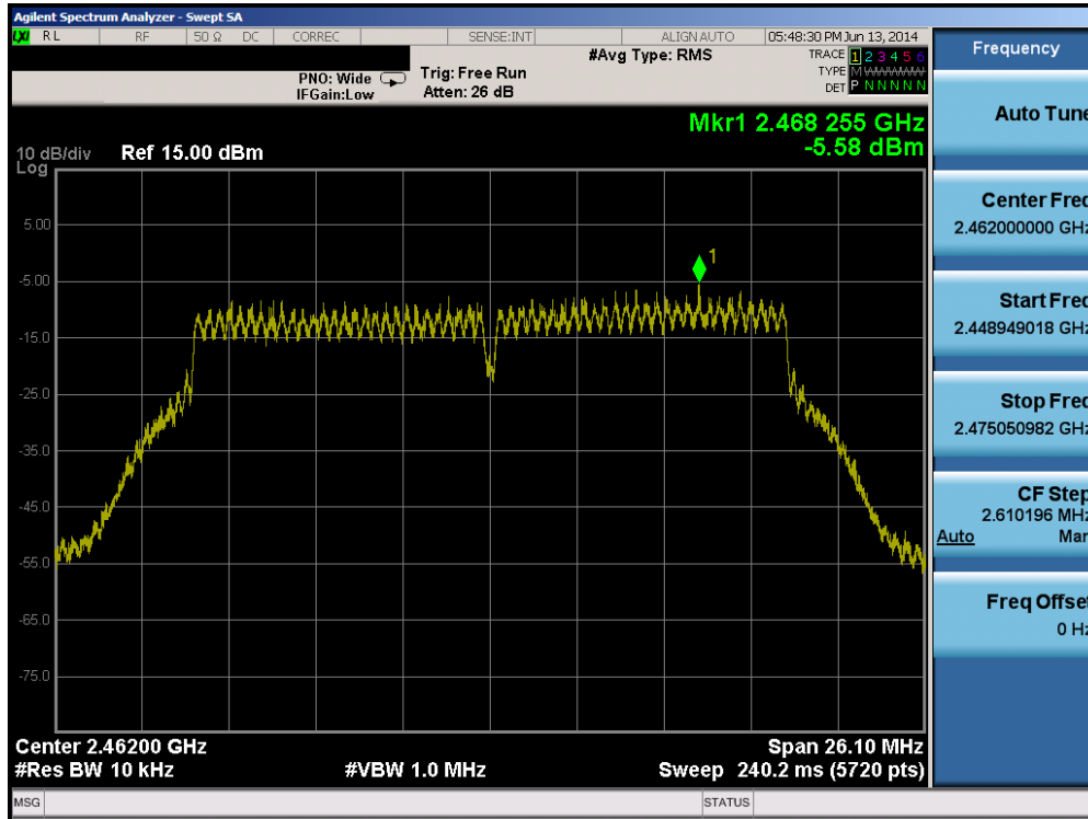
Plot 6-46. Power Spectral Density Plot (802.11n (2.4GHz) – Ch. 11)
