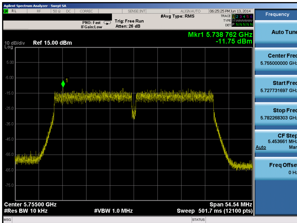
Plot 6-53. Power Spectral Density Plot (40MHz BW 802.11n (5.8GHz) – Ch. 151)
