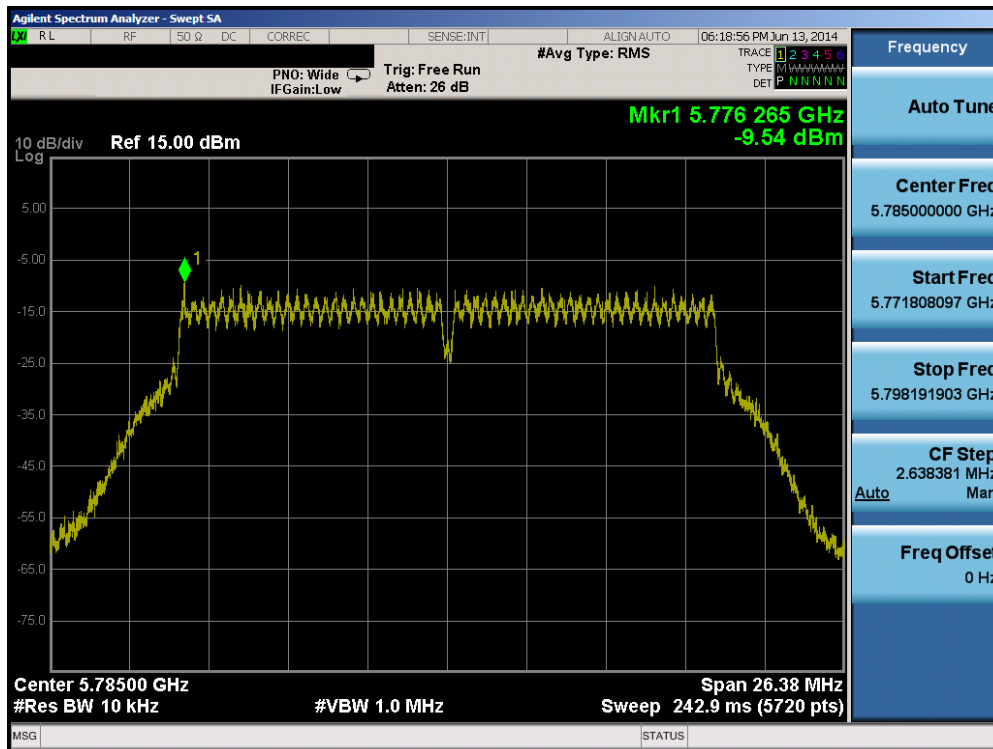
Plot 6-51. Power Spectral Density Plot (20MHz BW 802.11n (5.8GHz) – Ch. 157)
