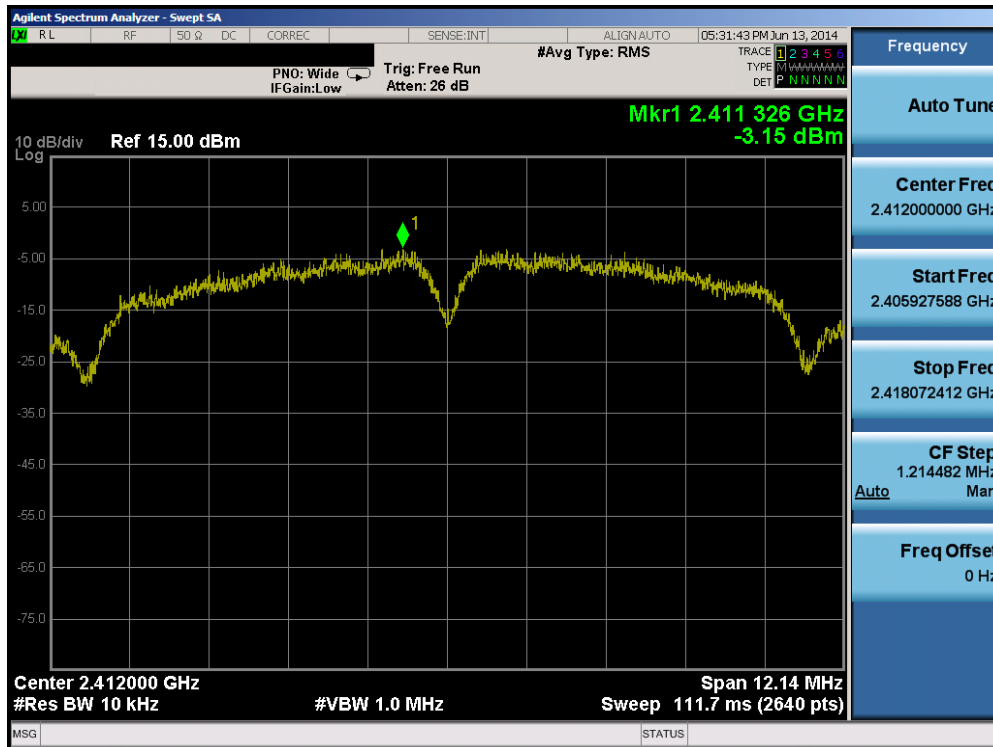
Plot 6-38. Power Spectral Density Plot (802.11b – Ch. 1)
