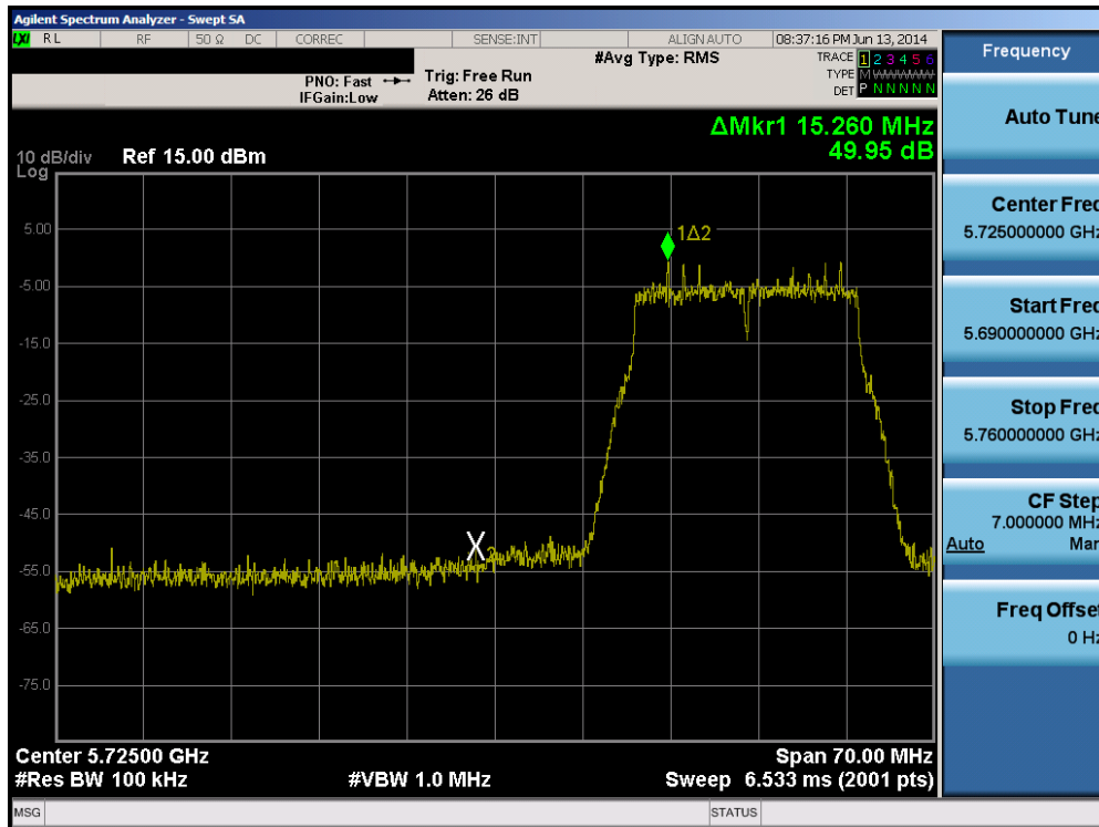
Plot 6-96. Band Edge Plot (20MHz BW 802.11n (5.8GHz) – Ch. 149)
