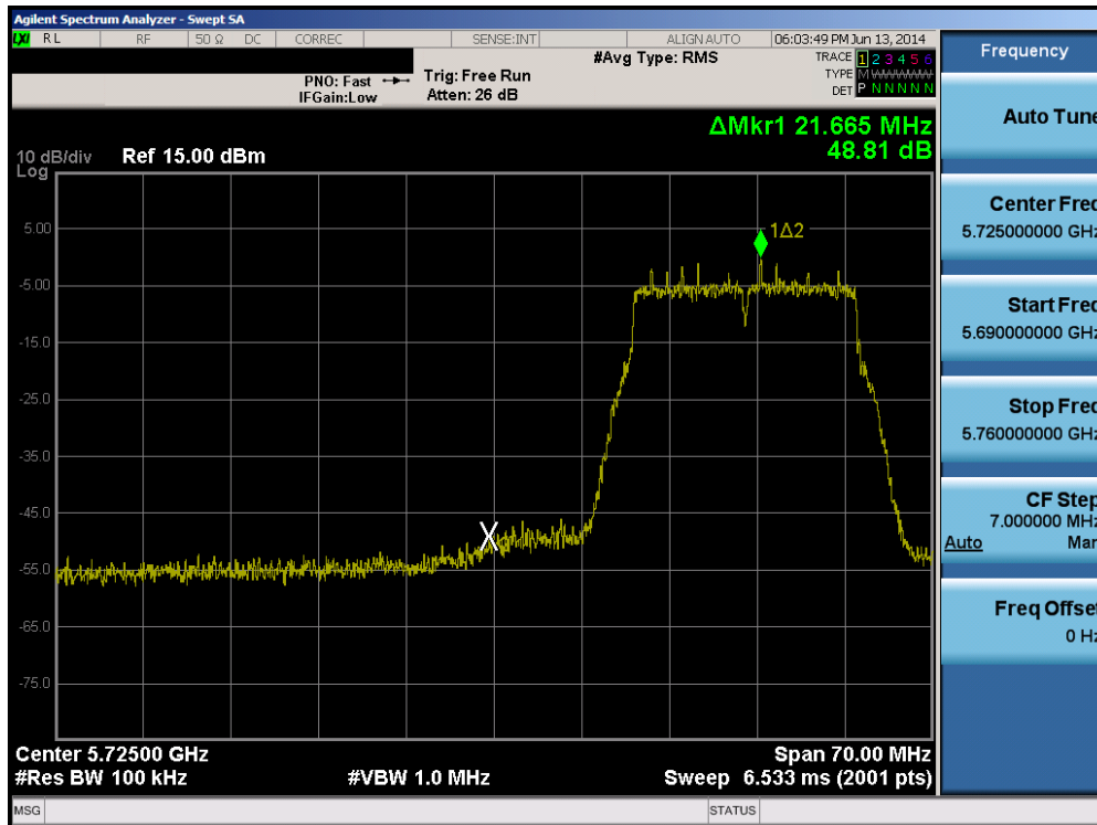
Plot 6-82. Band Edge Plot (20MHz BW 802.11n (5.8GHz) – Ch. 149)
