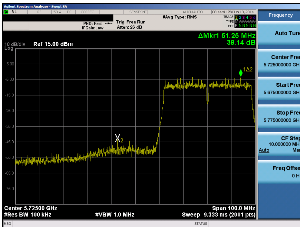
Plot 6-98. Band Edge Plot (40MHz BW 802.11n (5.8GHz) – Ch. 151)
