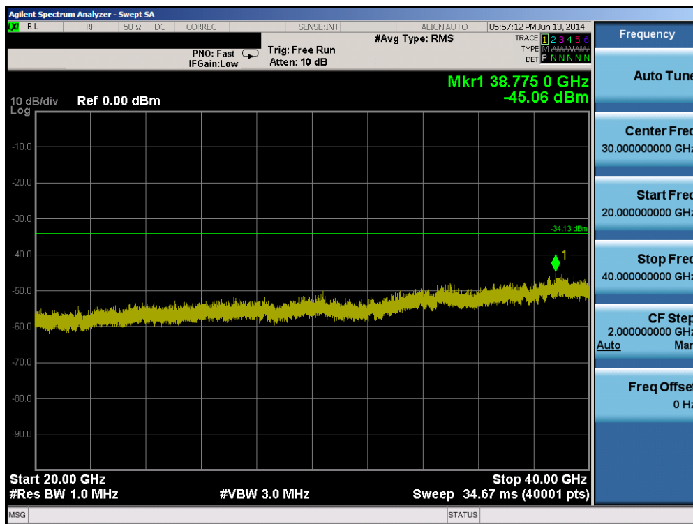
Plot 6-111. Conducted Spurious Plot (802.11a – Ch. 157)
