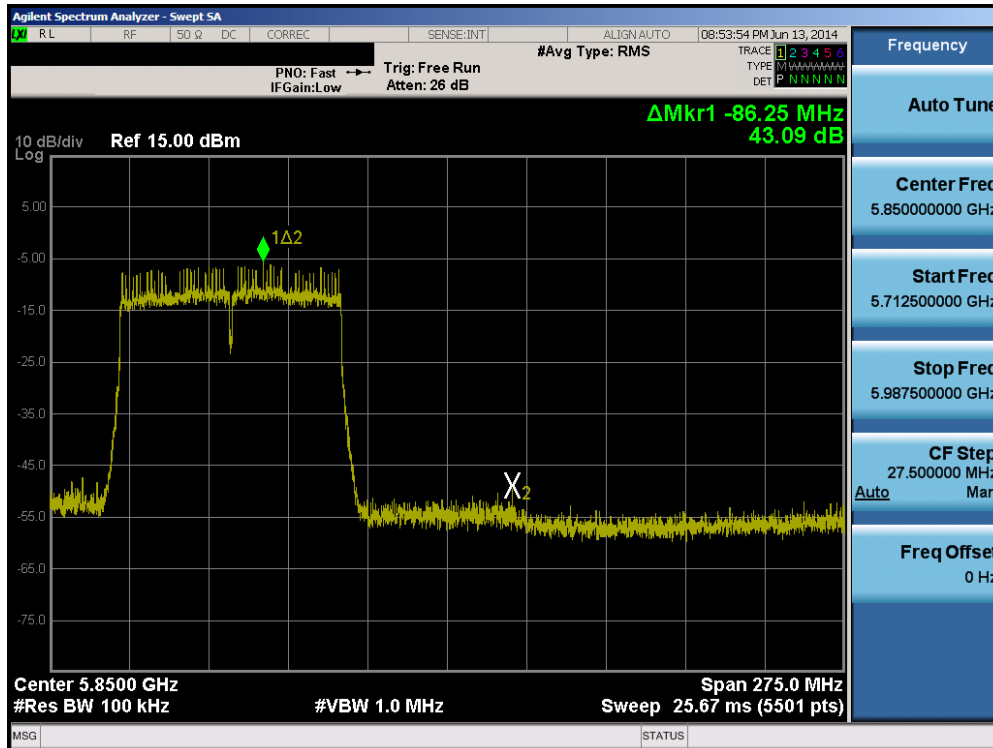
Plot 6-101. Band Edge Plot (80MHz BW 802.11ac (5.8GHz) – Ch. 155)
