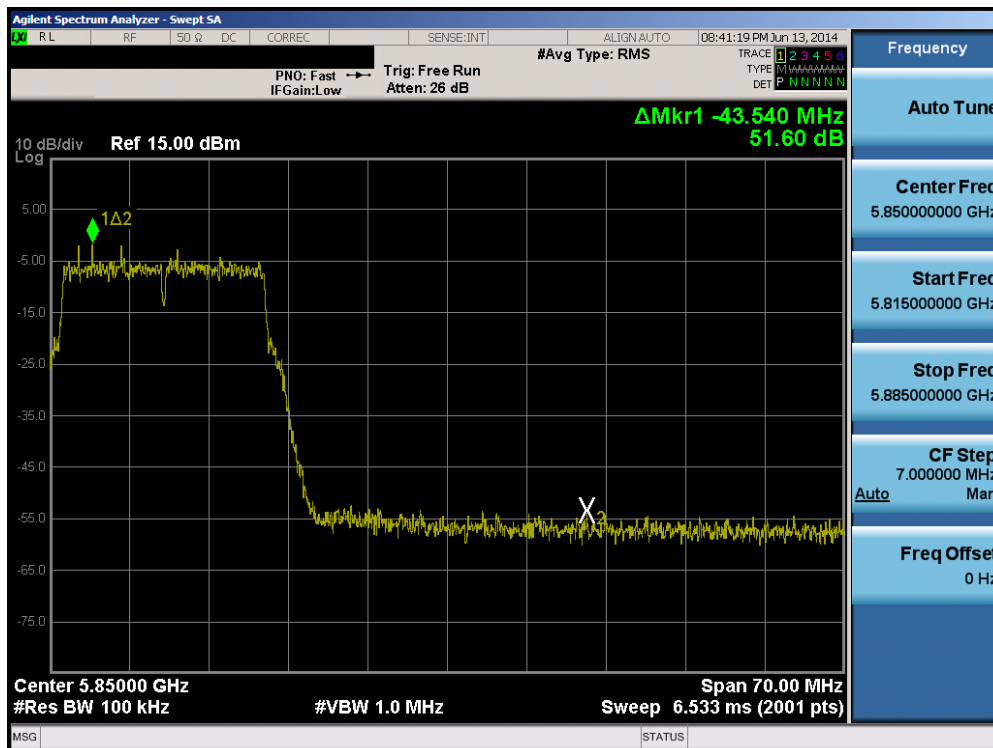
Plot 6-97. Band Edge Plot (20MHz BW 802.11n (5.8GHz) – Ch. 165)
