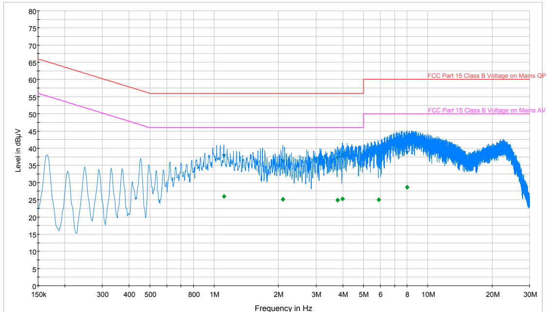
Plot 6-138. Line Conducted Plot with 802.11b (L1)
