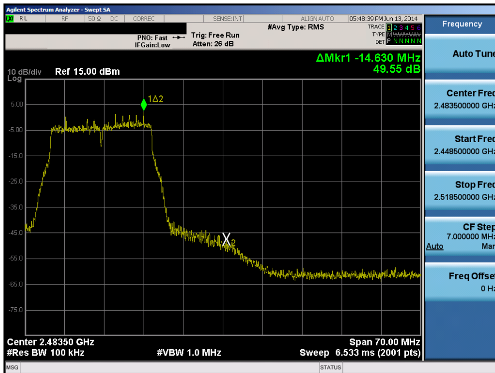
Plot 6-79. Band Edge Plot (802.11n (2.4GHz) – Ch. 11)
