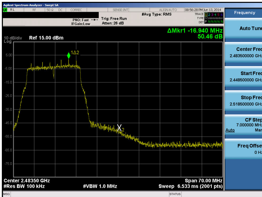
Plot 6-93. Band Edge Plot (802.11n (2.4GHz) – Ch. 11)
