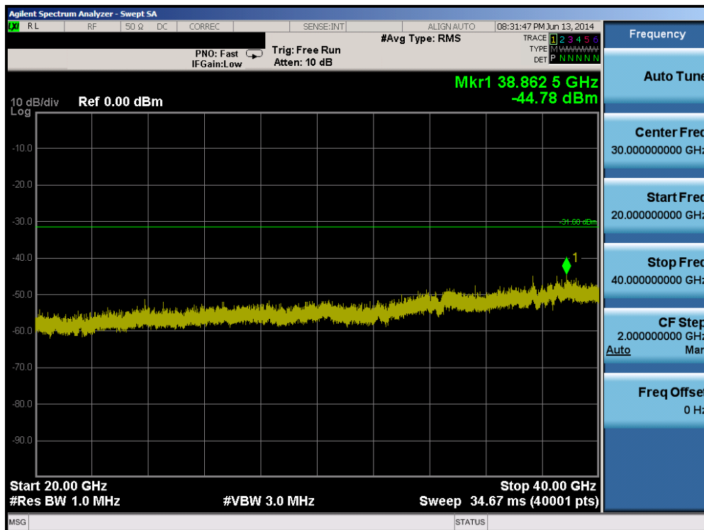
Plot 6-121. Conducted Spurious Plot (802.11a – Ch. 149)
