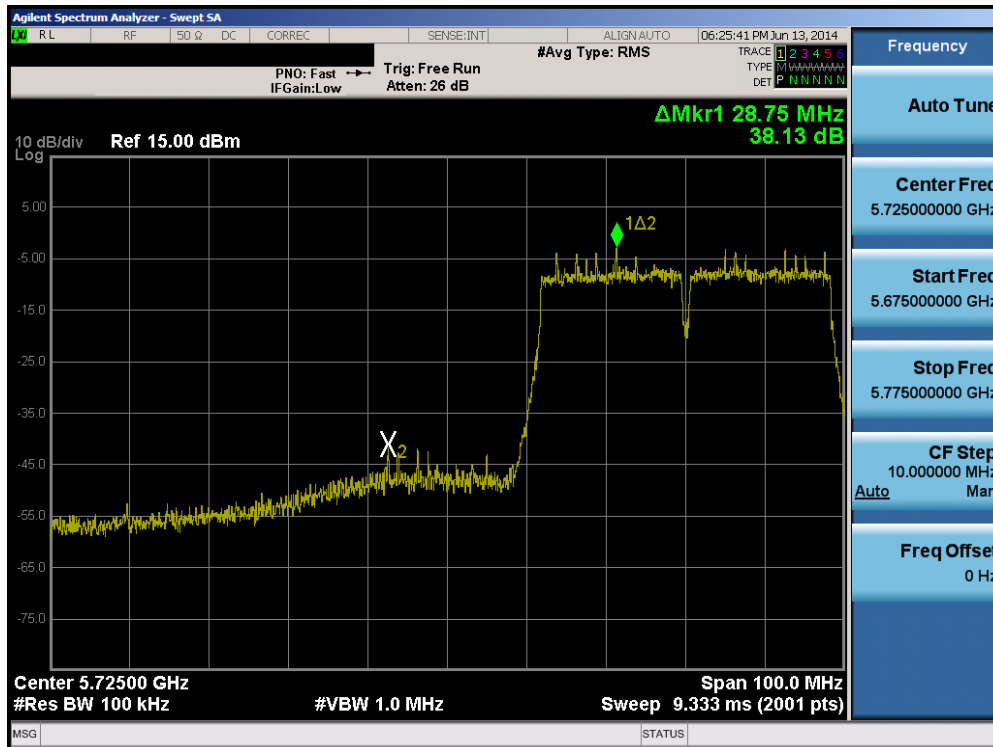
Plot 6-84. Band Edge Plot (40MHz BW 802.11n (5.8GHz) – Ch. 151)
