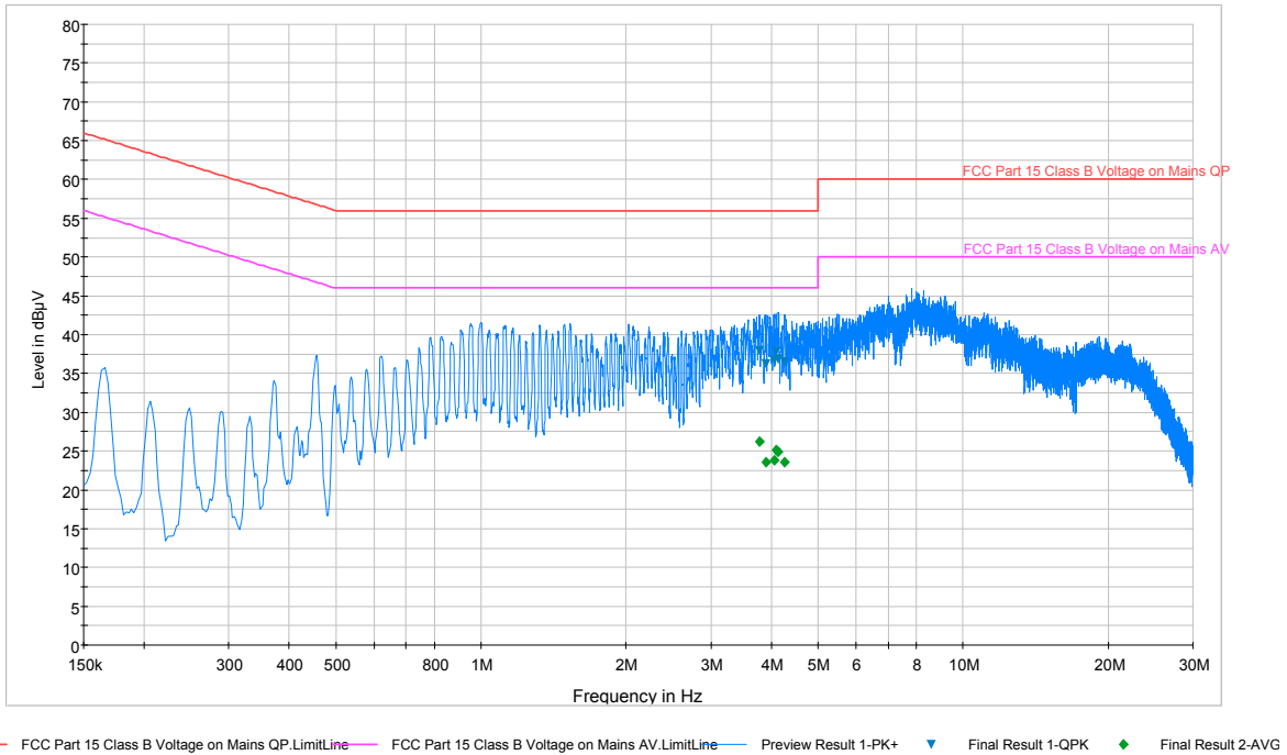
Plot 6-141. Line Conducted Plot with 802.11a (N)
