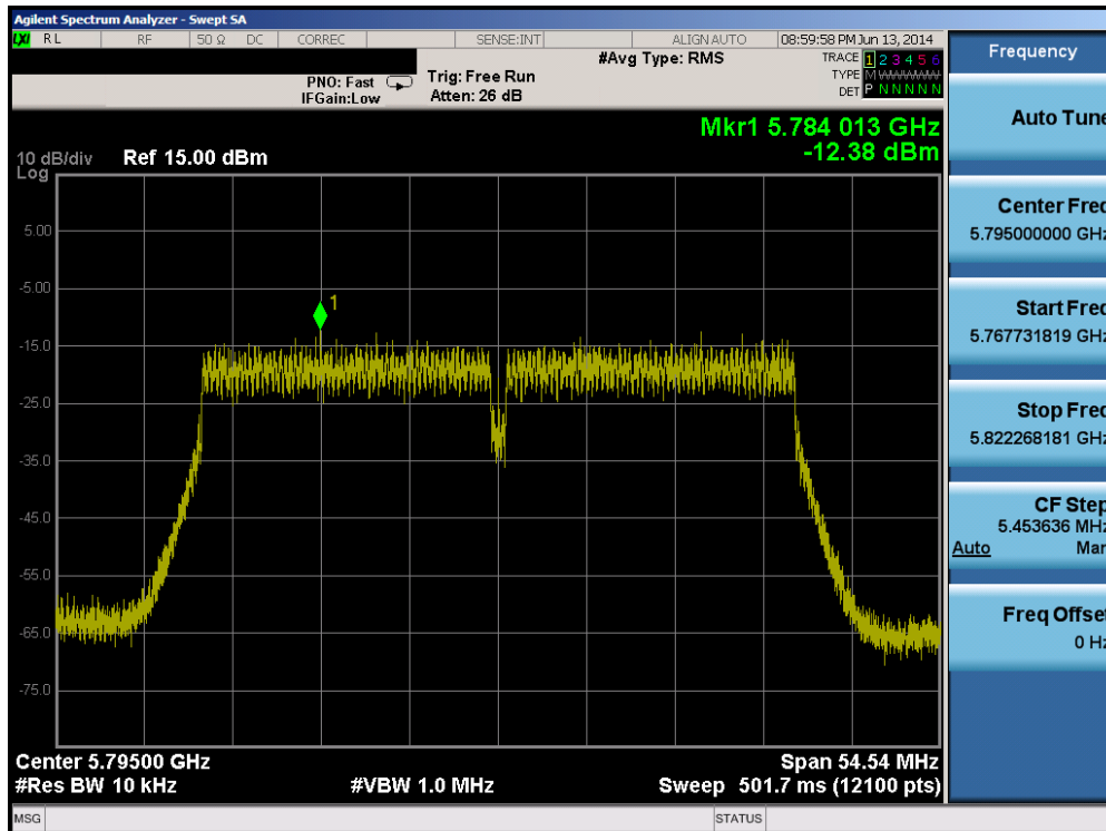
Plot 6-72. Power Spectral Density Plot (40MHz BW 802.11n (5.8GHz) – Ch. 159)
