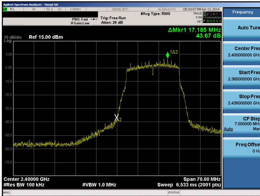
Plot 6-78. Band Edge Plot (802.11n (2.4GHz) – Ch. 1)
