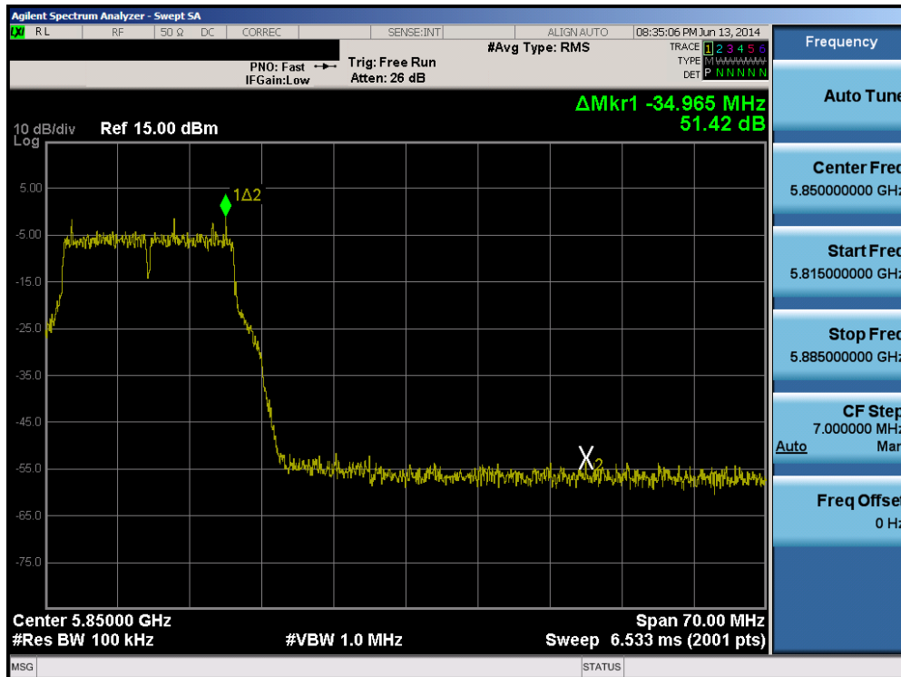
Plot 6-95. Band Edge Plot (802.11a – Ch. 165)
