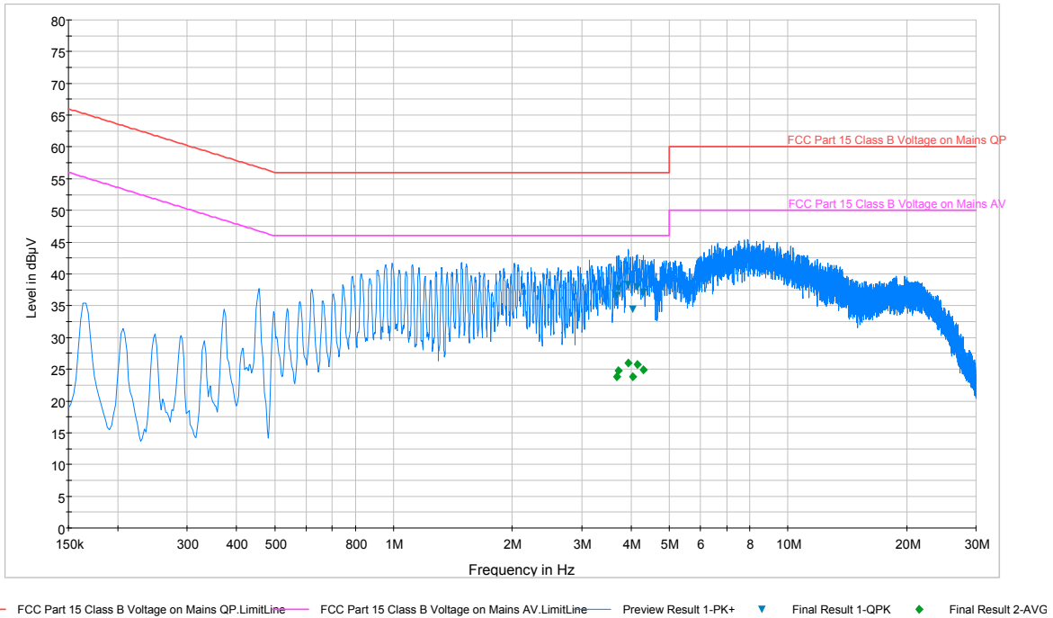
Plot 6-139. Line Conducted Plot with 802.11b (N)
