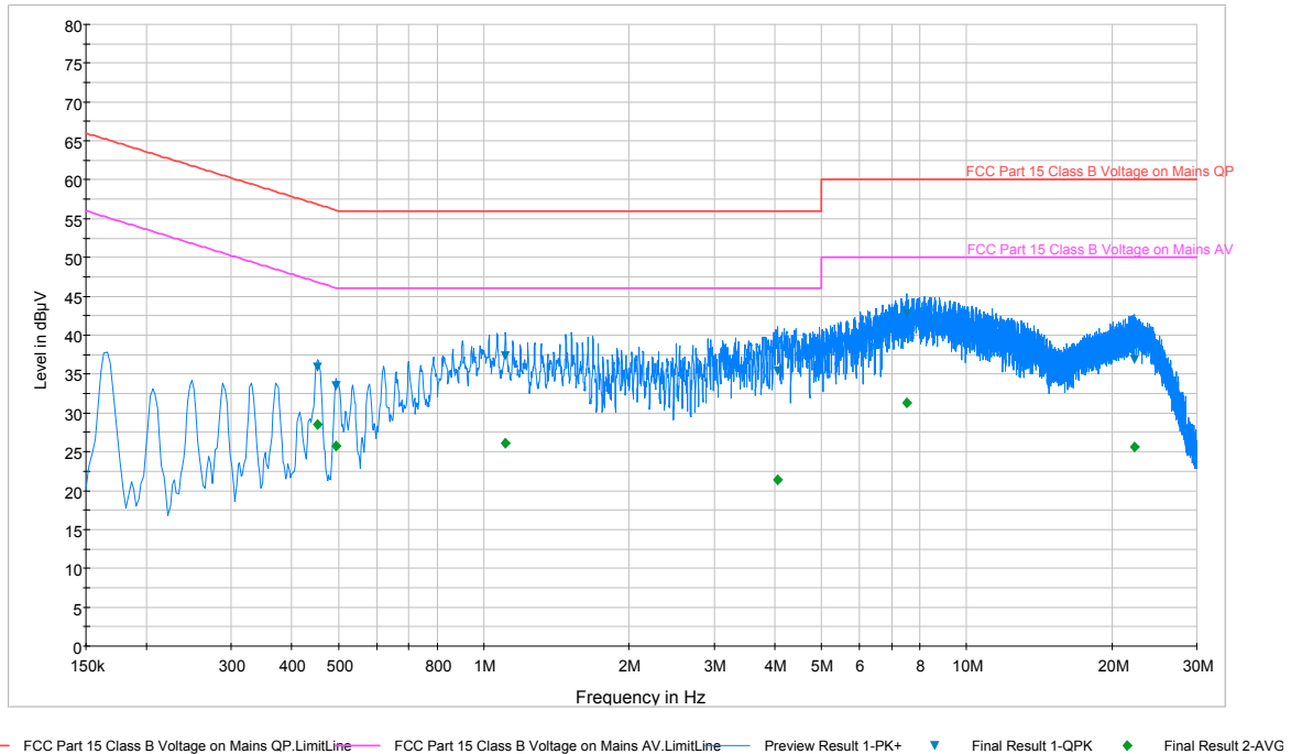
Plot 6-140. Line Conducted Plot with 802.11a (L1)
