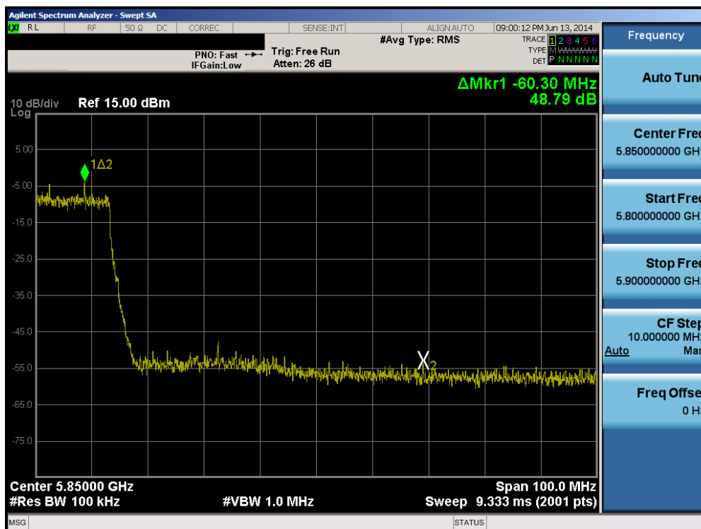
Plot 6-99. Band Edge Plot (40MHz BW 802.11n (5.8GHz) – Ch. 159)
