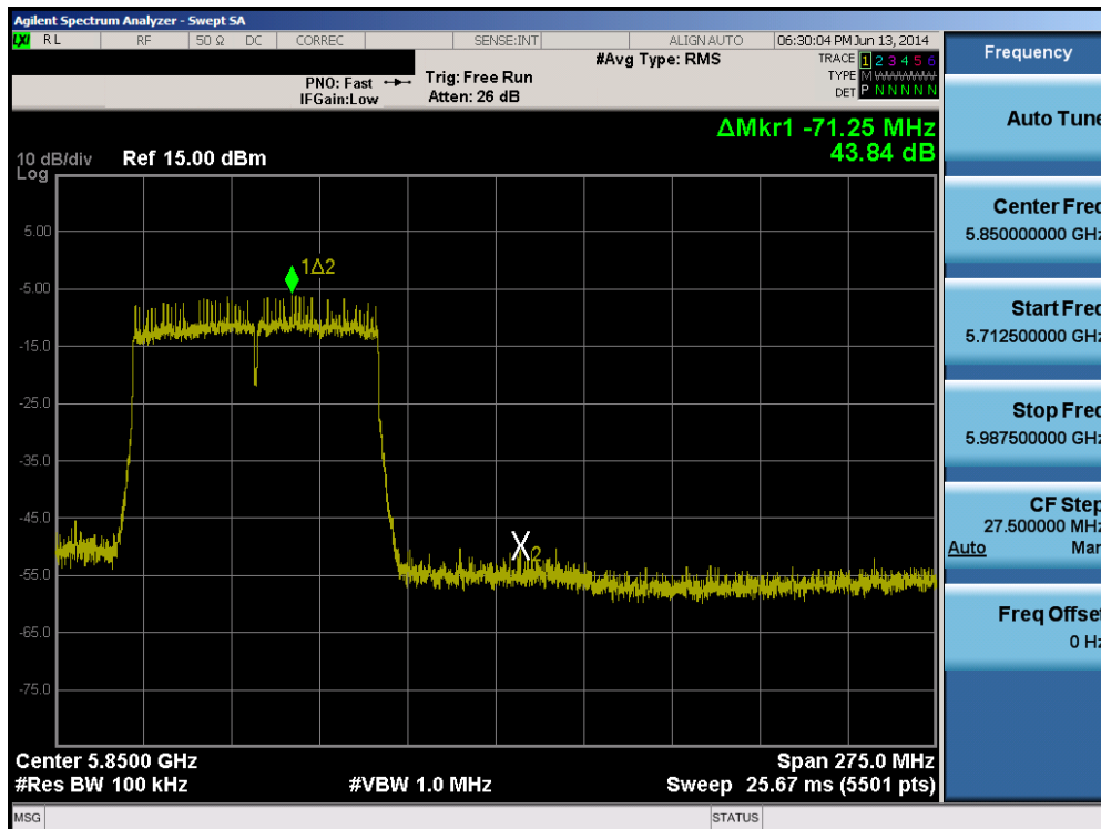
Plot 6-87. Band Edge Plot (80MHz BW 802.11ac (5.8GHz) – Ch. 155)
