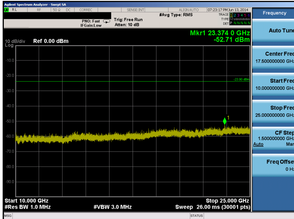
Plot 6-115. Conducted Spurious Plot (802.11b – Ch. 1)
