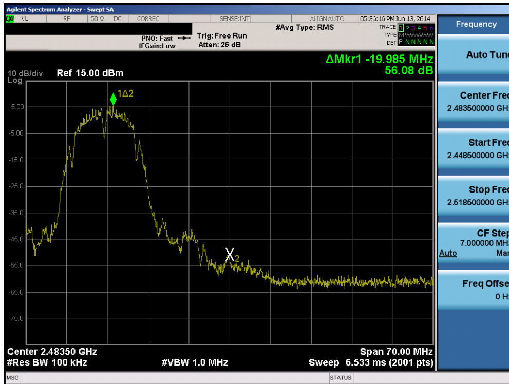
Plot 6-75. Band Edge Plot (802.11b – Ch. 11)
