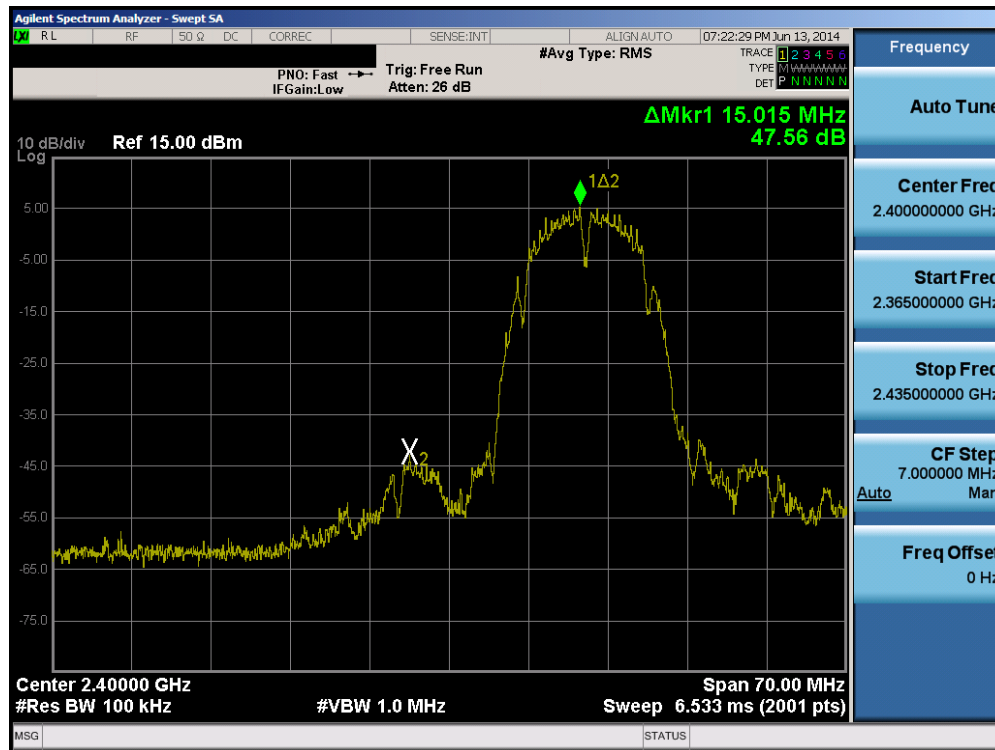
Plot 6-88. Band Edge Plot (802.11b – Ch. 1)
