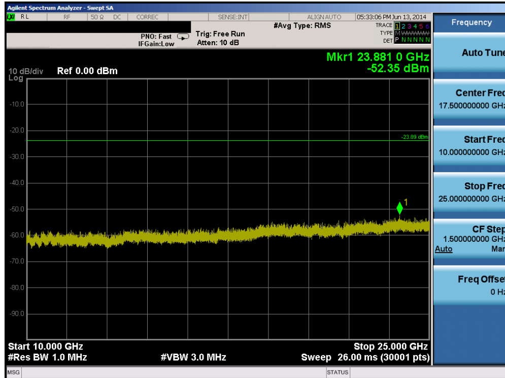
Plot 6-103. Conducted Spurious Plot (802.11b – Ch. 1)
