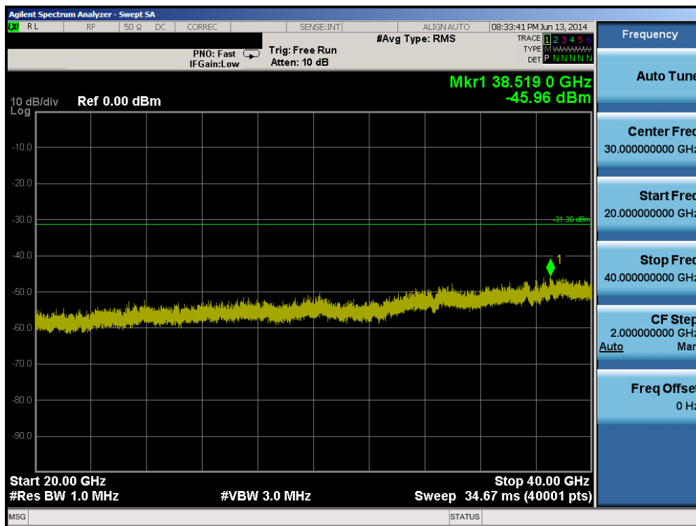
Plot 6-123. Conducted Spurious Plot (802.11a – Ch. 157)
