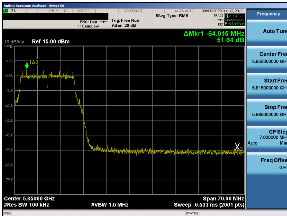
Plot 6-81. Band Edge Plot (802.11a – Ch. 165)
