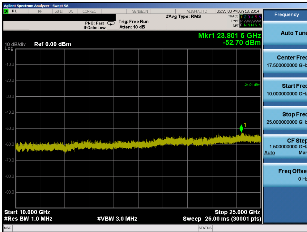
Plot 6-105. Conducted Spurious Plot (802.11b – Ch. 6)
