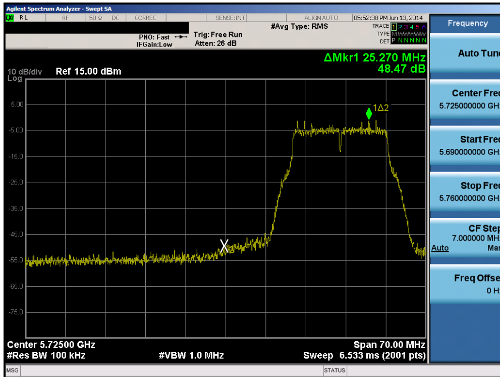
Plot 6-80. Band Edge Plot (802.11a – Ch. 149)
