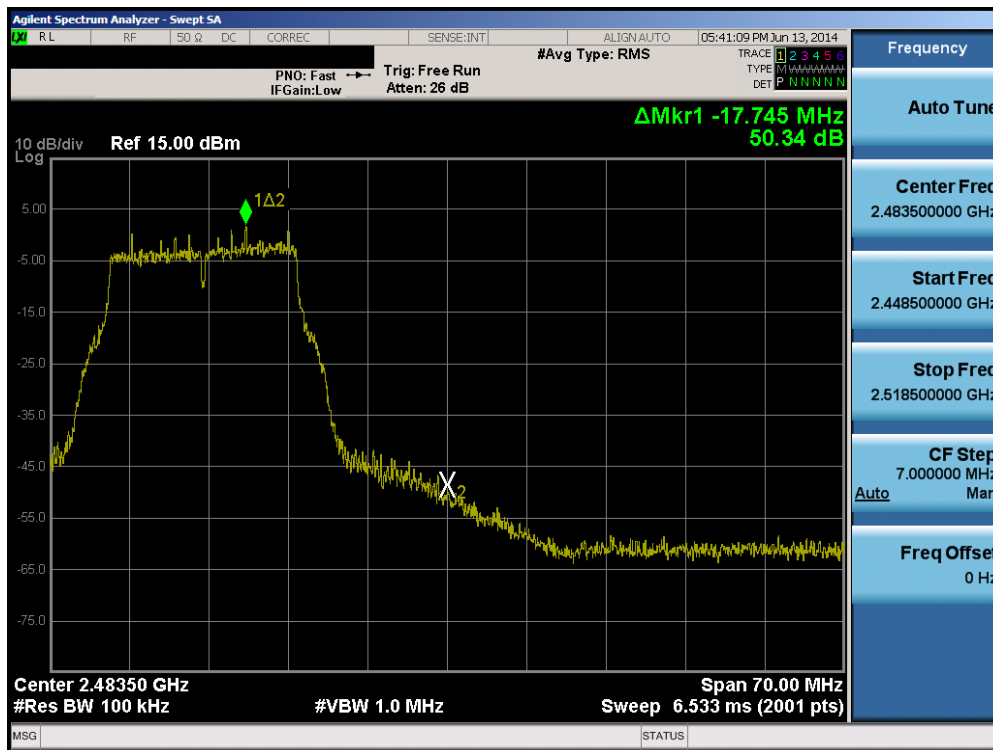
Plot 6-77. Band Edge Plot (802.11g – Ch. 11)
