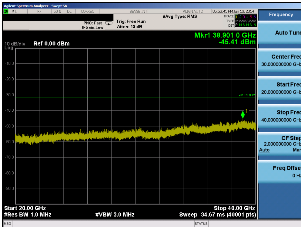
Plot 6-109. Conducted Spurious Plot (802.11a – Ch. 149)
