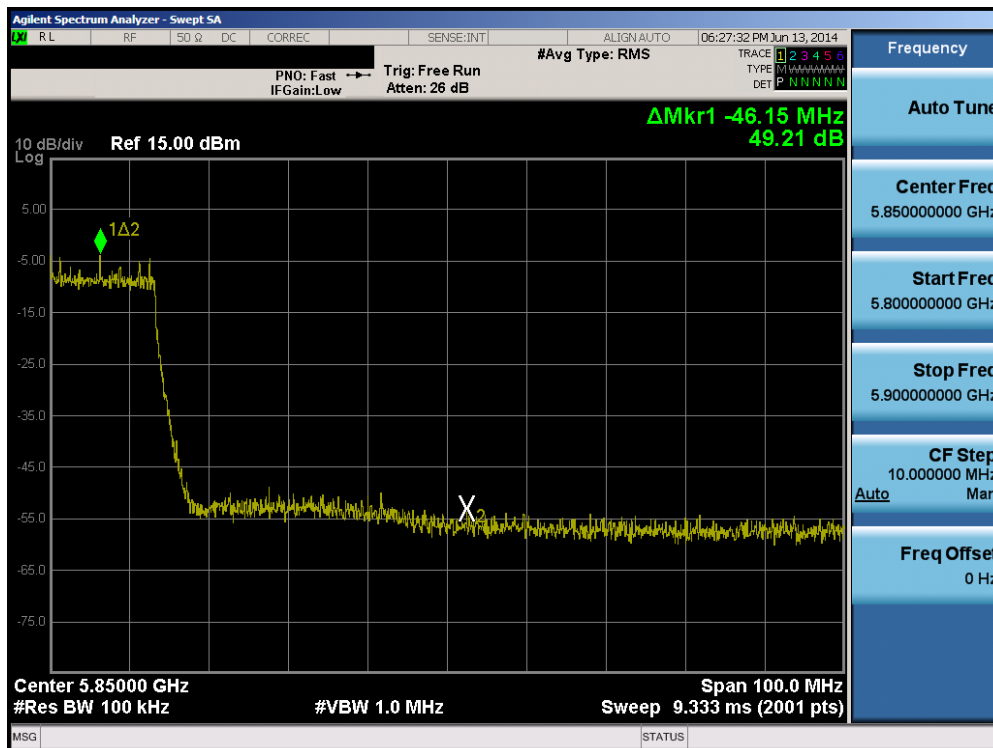
Plot 6-85. Band Edge Plot (40MHz BW 802.11n (5.8GHz) – Ch. 159)
