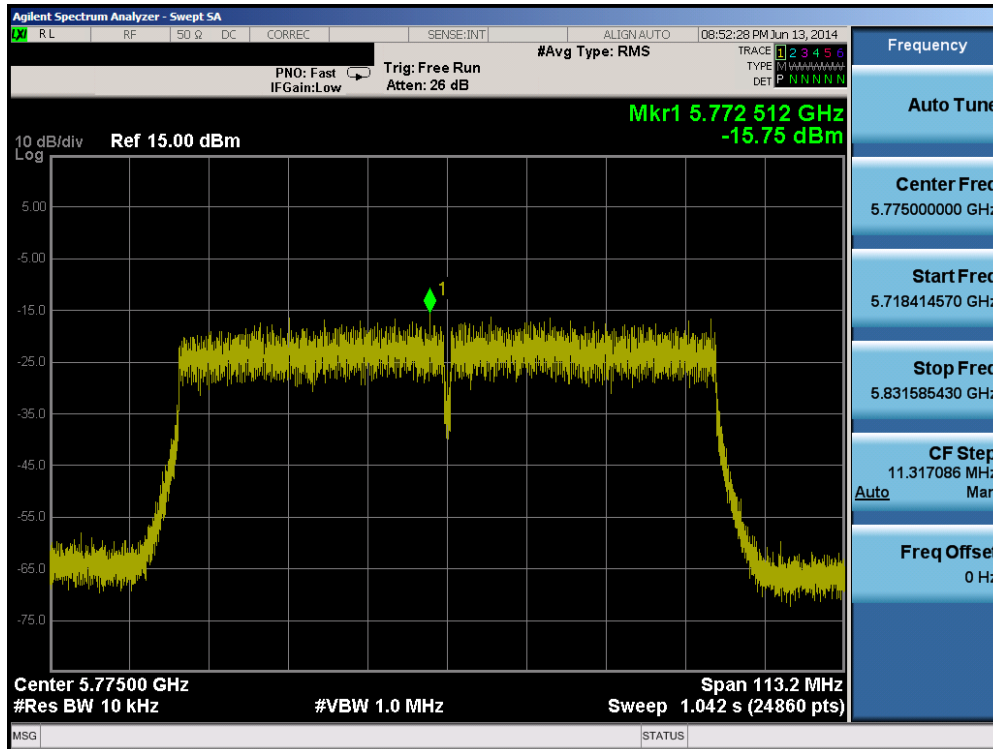
Plot 6-73. Power Spectral Density Plot (80MHz BW 802.11ac (5.8GHz) – Ch. 155)
