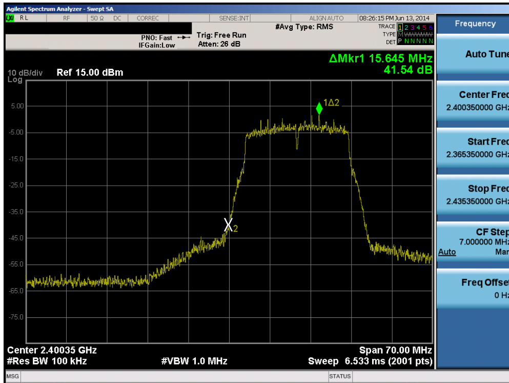
Plot 6-92. Band Edge Plot (802.11n (2.4GHz) – Ch. 1)
