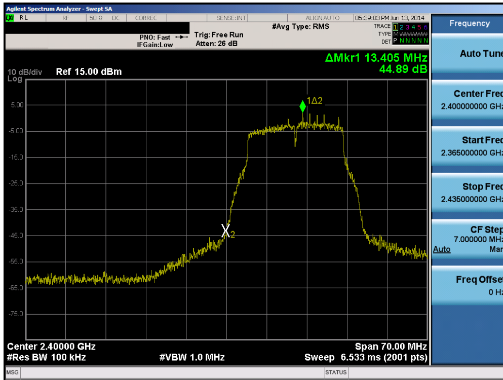
Plot 6-76. Band Edge Plot (802.11g– Ch. 1)
