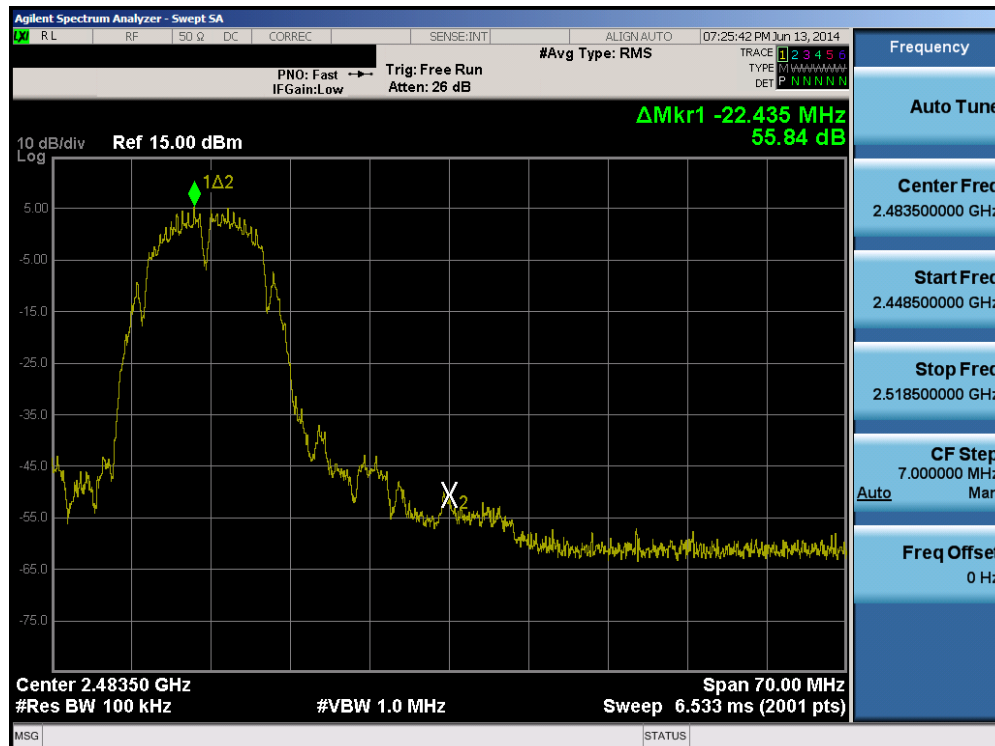
Plot 6-89. Band Edge Plot (802.11b – Ch. 11)
