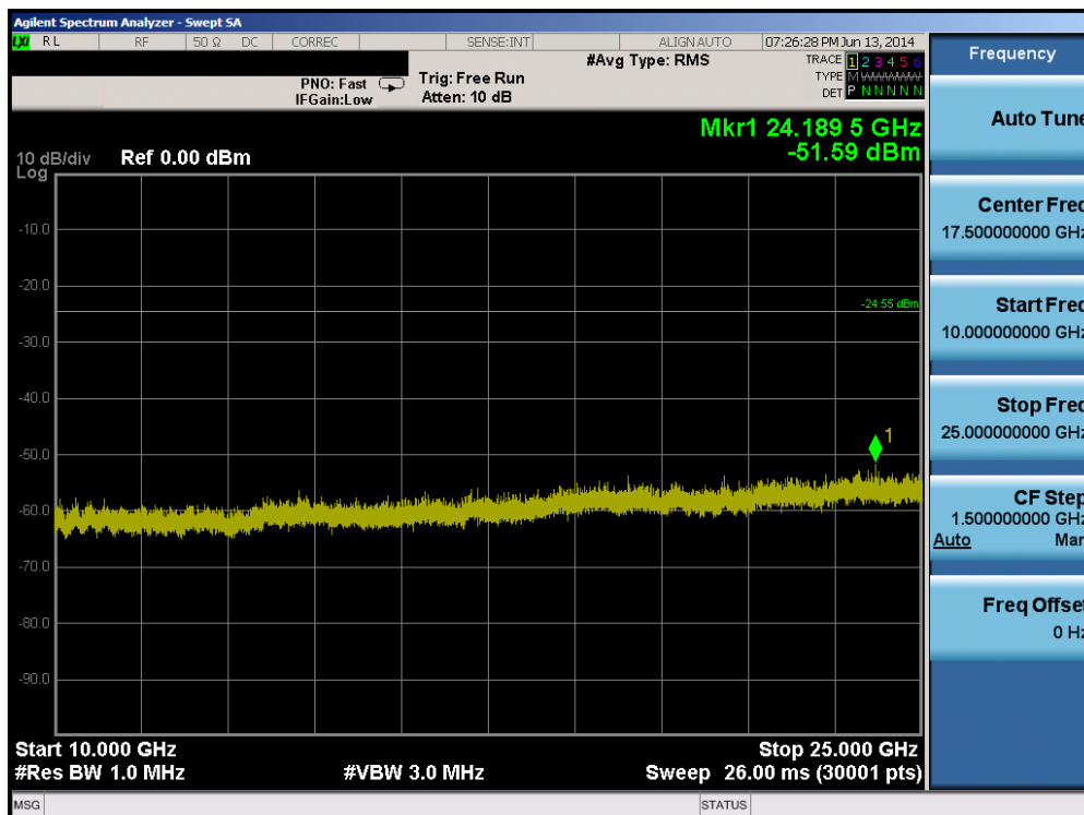
Plot 6-119. Conducted Spurious Plot (802.11b – Ch. 11)
