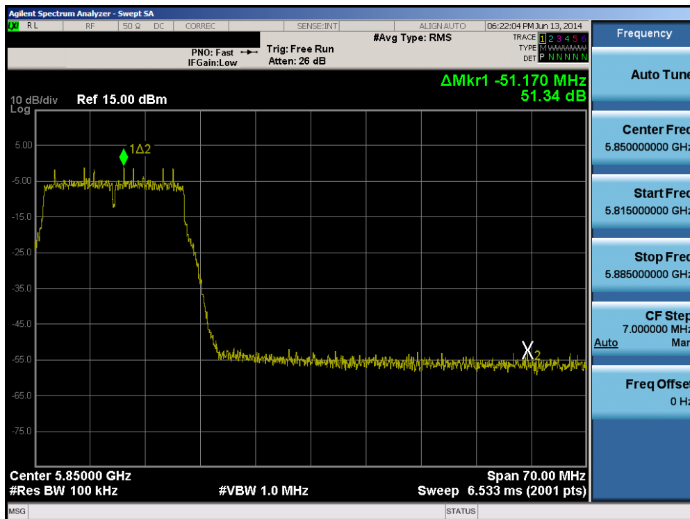
Plot 6-83. Band Edge Plot (20MHz BW 802.11n (5.8GHz) – Ch. 165)
