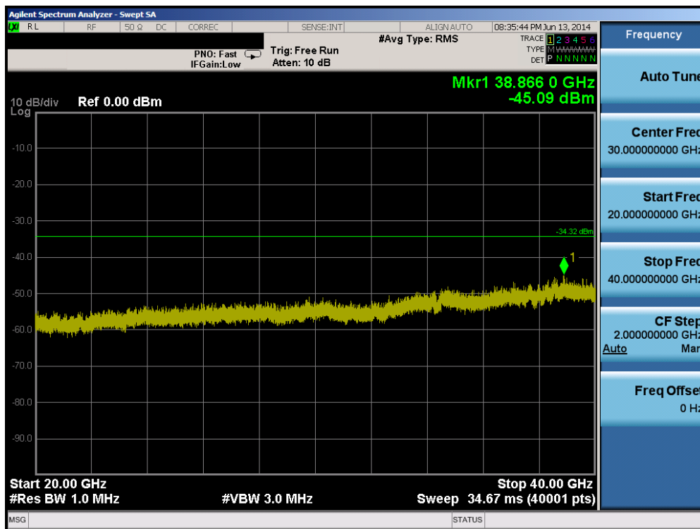
Plot 6-125. Conducted Spurious Plot (802.11a – Ch. 165)
