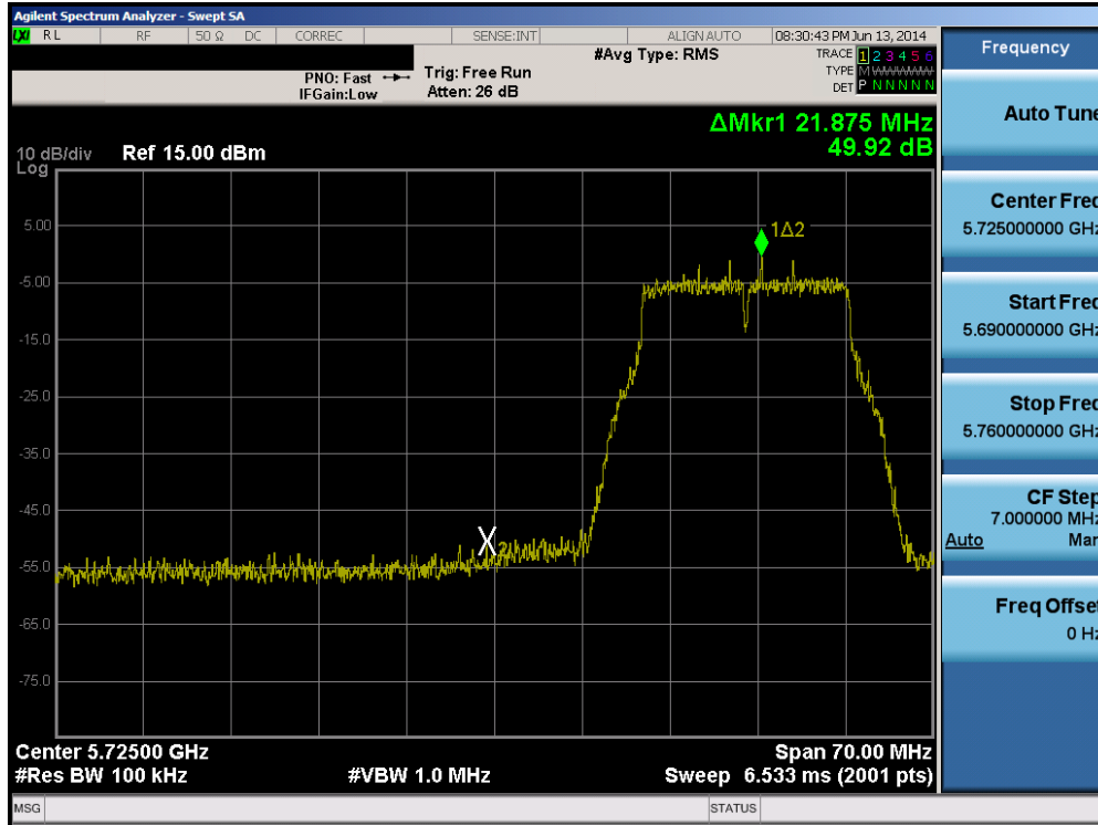
Plot 6-94. Band Edge Plot (802.11a – Ch. 149)
