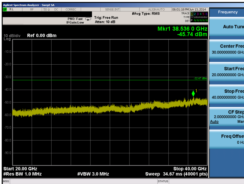
Plot 6-113. Conducted Spurious Plot (802.11a – Ch. 165)
