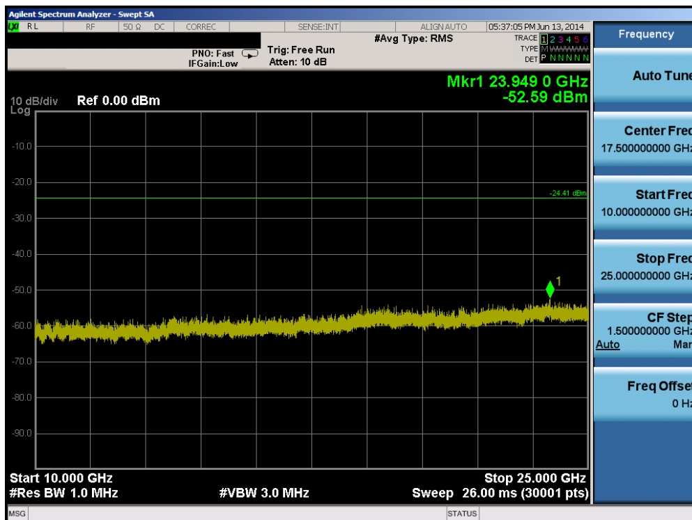
Plot 6-107. Conducted Spurious Plot (802.11b – Ch. 11)
