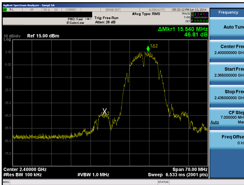
Plot 6-74. Band Edge Plot (802.11b – Ch. 1)
