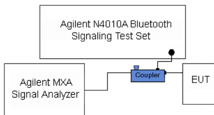
Figure 6-2. Test Instrument & Measurement Setup
