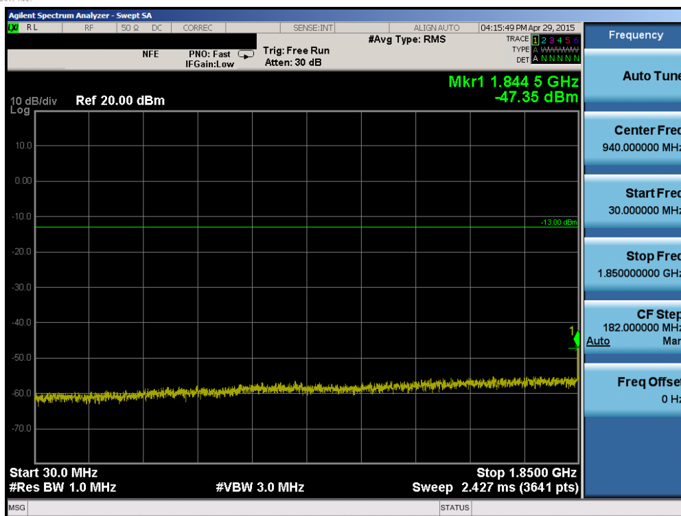
Plot 6-71. Conducted Spurious Plot (Band 2 – 20.0MHz QPSK – RB Size 1, RB Offset 0 – Mid Channel)
