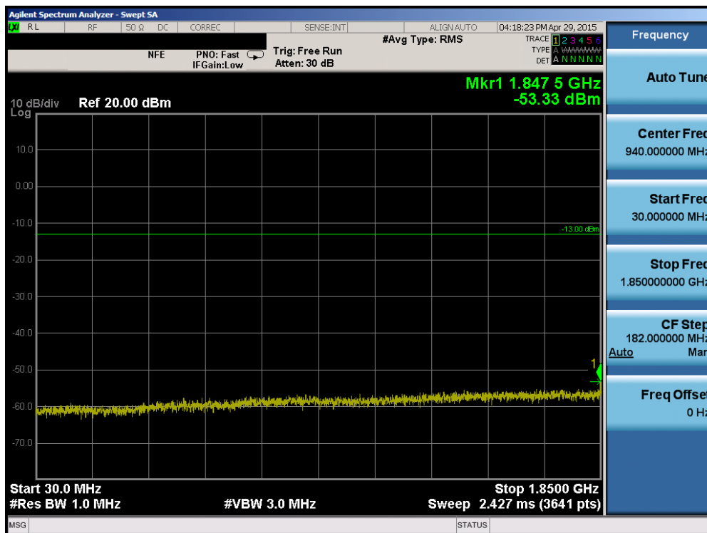
Plot 6-74. Conducted Spurious Plot (Band 2 – 20.0MHz QPSK – RB Size 1, RB Offset 0 – High Channel)
