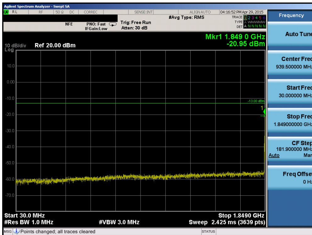
Plot 6-68. Conducted Spurious Plot (Band 2 – 20.0MHz QPSK – RB Size 1, RB Offset 0– Low Channel)
