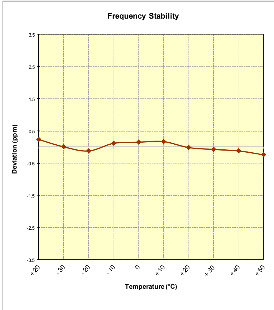
Figure 6-8. Frequency Stability Graph (PCS WCDMA Mode – Ch. 9400)
