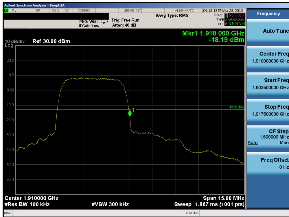
Plot 6-26. Band Edge Plot (PCS WCDMA Mode – Ch. 9538)
