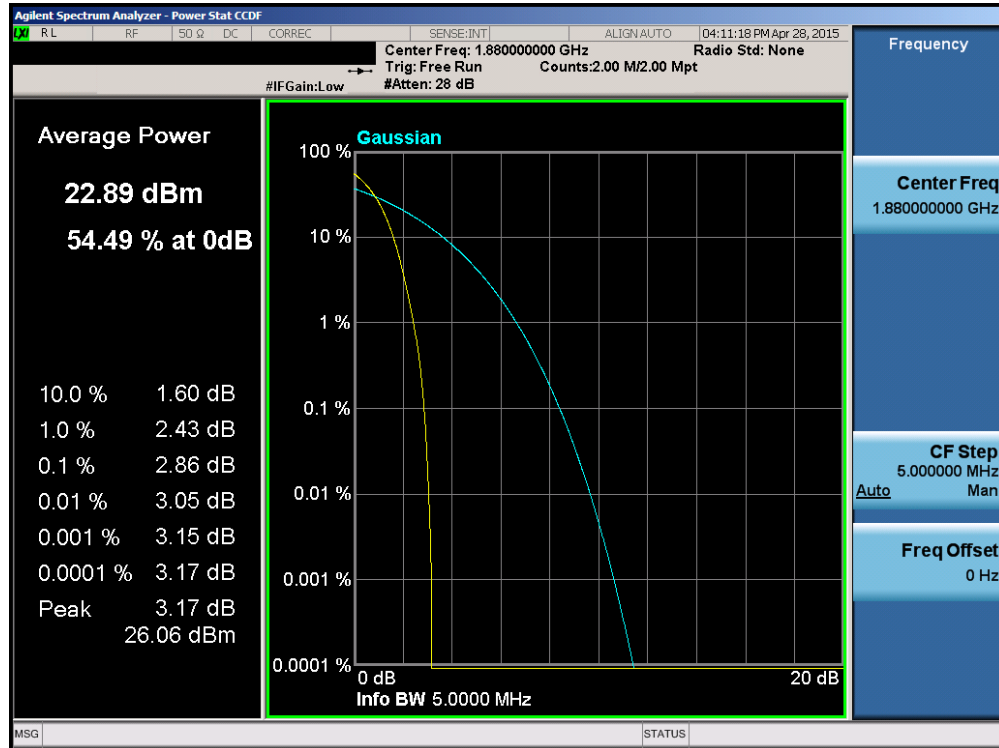
Plot 6-28. Peak-Average Ratio Plot (PCS WCDMA Mode – Ch. 9400)
