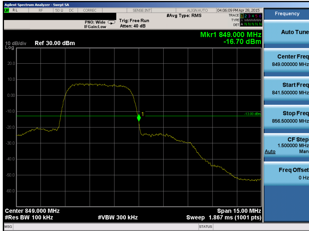
Plot 6-23. Band Edge Plot (Cellular WCDMA Mode – Ch. 4233)
