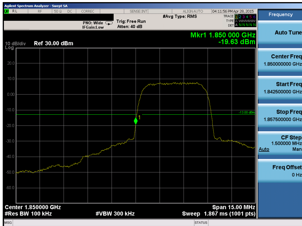
Plot 6-24. Band Edge Plot (PCS WCDMA Mode – Ch. 9262)
