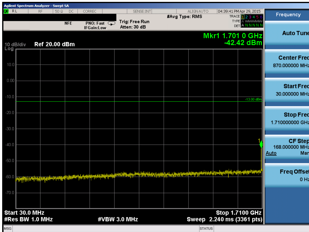
Plot 6-78. Conducted Spurious Plot (Band 4 – 20.0MHz QPSK – RB Size 1, RB Offset 0 – High Channel)
