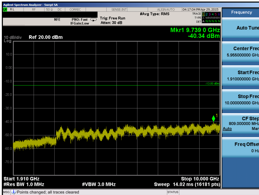
Plot 6-82. Conducted Spurious Plot (Band 2 – 20.0MHz QPSK – RB Size 1, RB Offset 0 – Low Channel)
