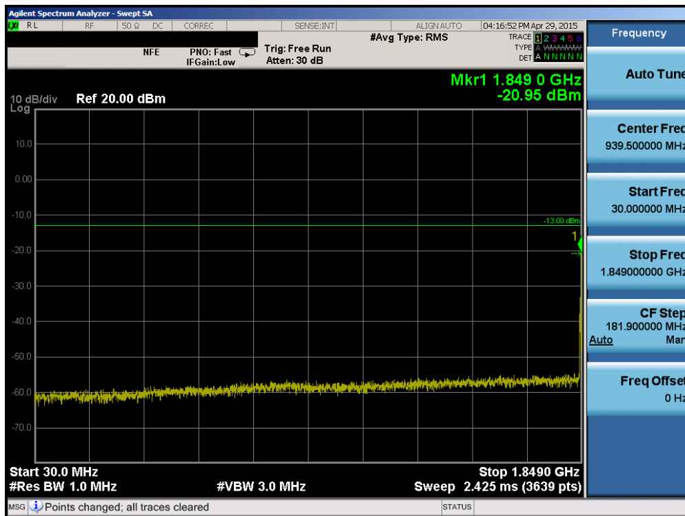
Plot 6-81. Conducted Spurious Plot (Band 2 – 20.0MHz QPSK – RB Size 1, RB Offset 0– Low Channel)
