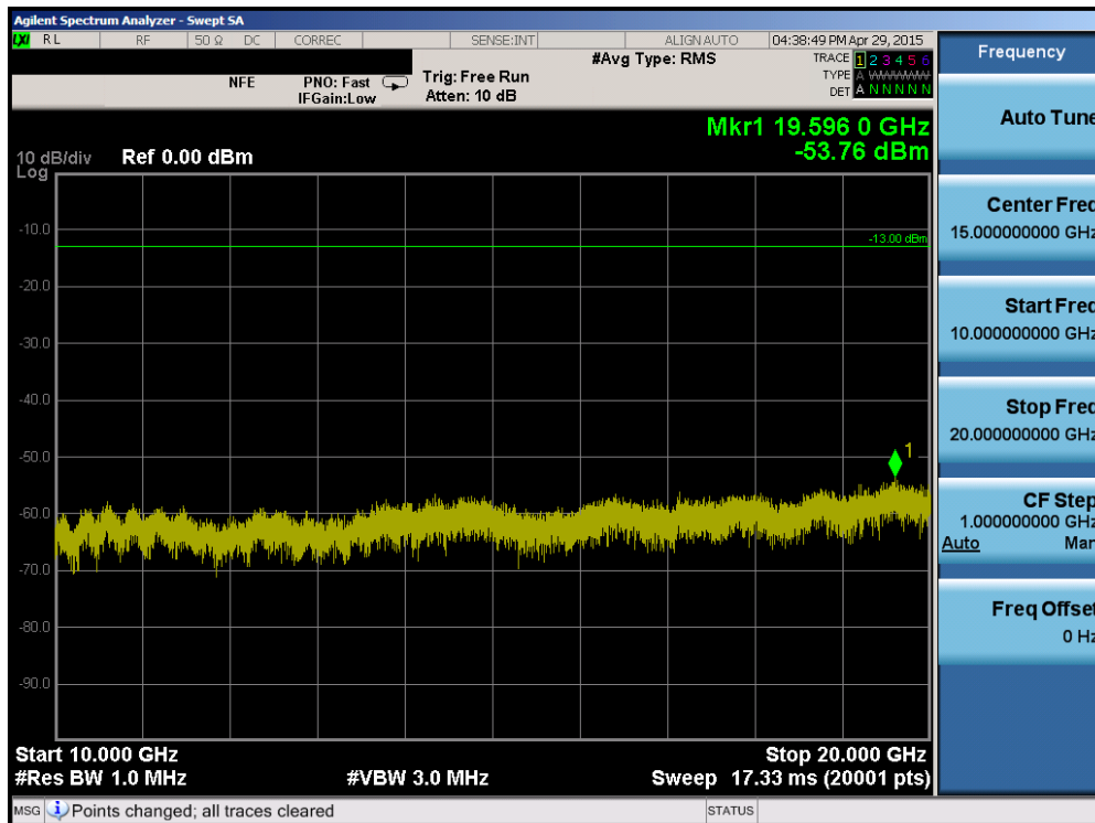
Plot 6-74. Conducted Spurious Plot (Band 4 – 20.0MHz QPSK – RB Size 1, RB Offset 0 – Low Channel)
