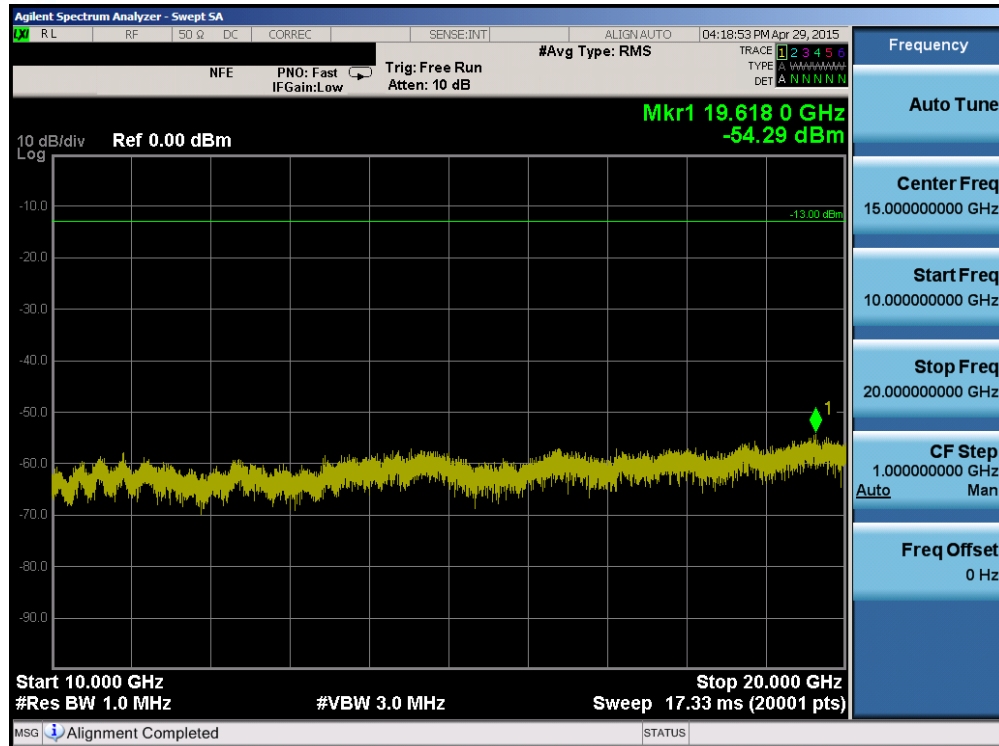
Plot 6-89. Conducted Spurious Plot (Band 2 – 20.0MHz QPSK – RB Size 1, RB Offset 0 – High Channel)
