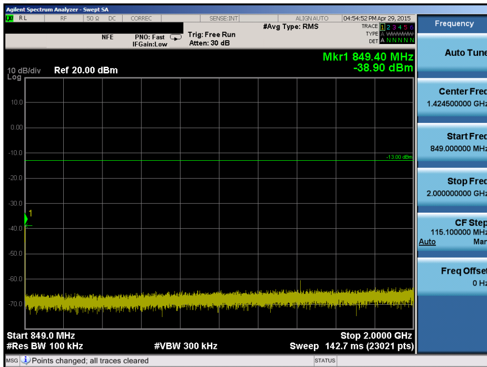
Plot 6-67. Conducted Spurious Plot (Band 5 – 10.0MHz QPSK – RB Size 1, RB Offset 0 – Mid Channel)
