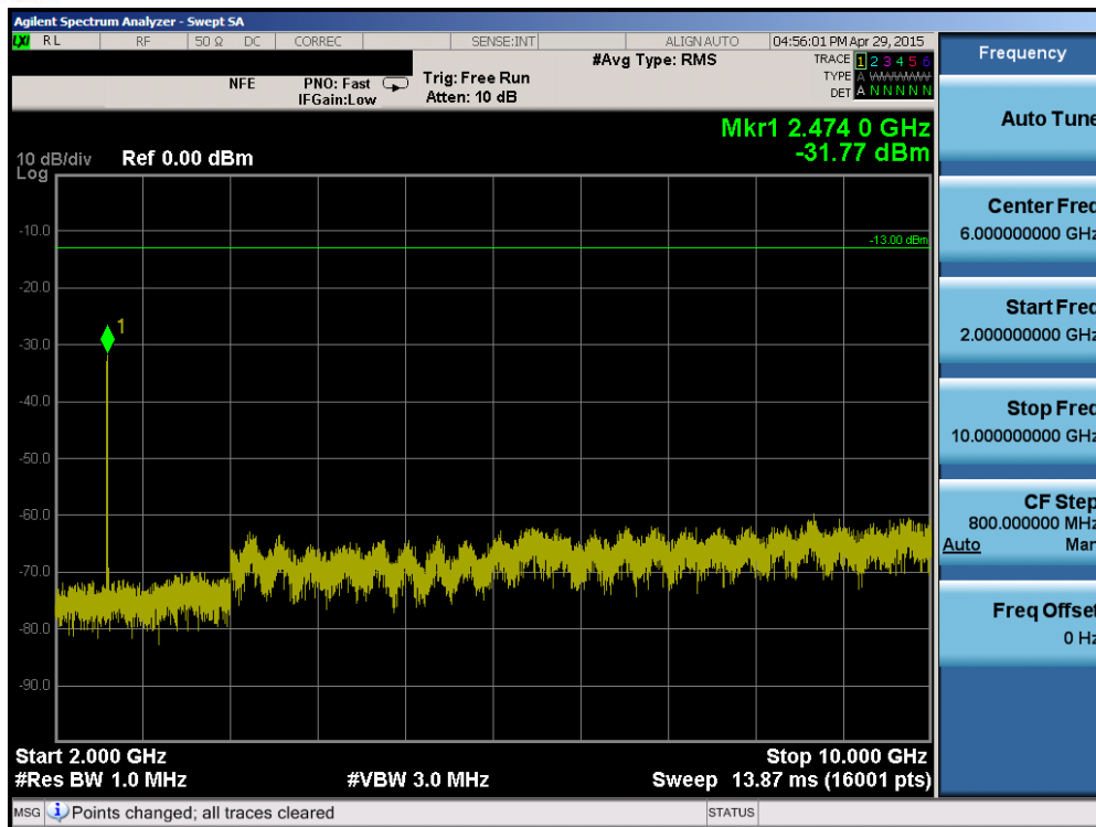
Plot 6-65. Conducted Spurious Plot (Band 5 – 10.0MHz QPSK – RB Size 1, RB Offset 0 – Low Channel)
