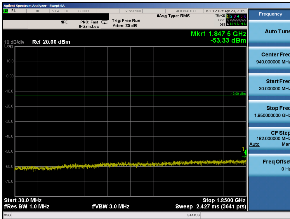
Plot 6-87. Conducted Spurious Plot (Band 2 – 20.0MHz QPSK – RB Size 1, RB Offset 0 – High Channel)
