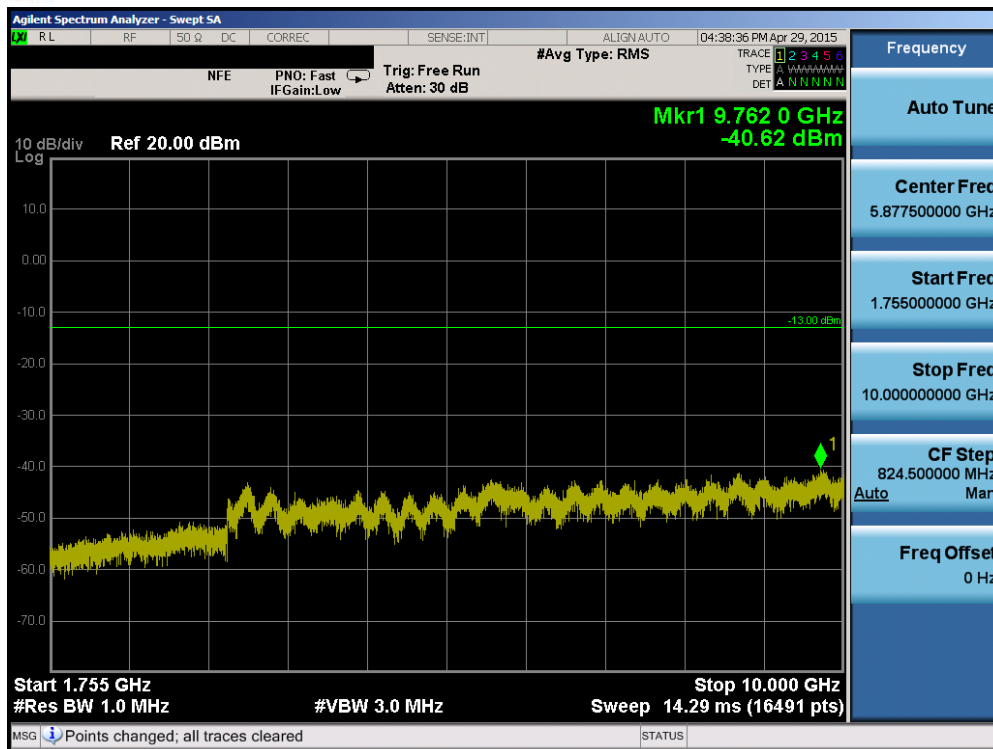
Plot 6-73. Conducted Spurious Plot (Band 4 – 20.0MHz QPSK – RB Size 1, RB Offset 0 – Low Channel)
