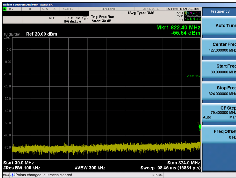
Plot 6-69. Conducted Spurious Plot (Band 5 – 10.0MHz QPSK – RB Size 1, RB Offset 0 – High Channel)
