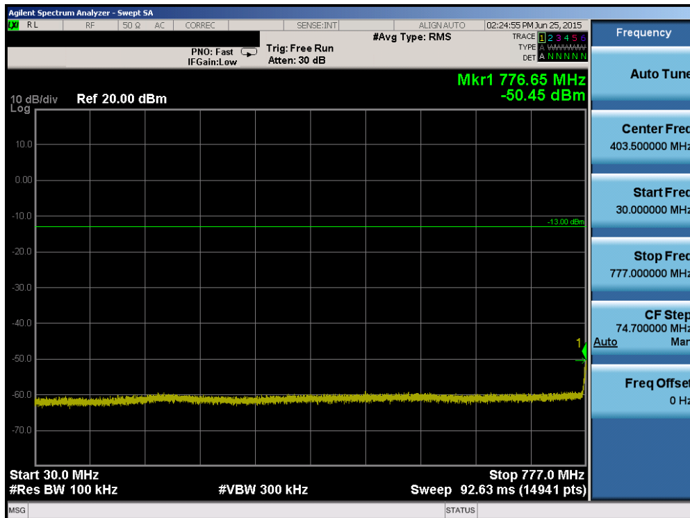
Plot 6-60. Conducted Spurious Plot (Band 13 – 5.0MHz QPSK – RB Size 1, RB Offset 0 – High Channel)
