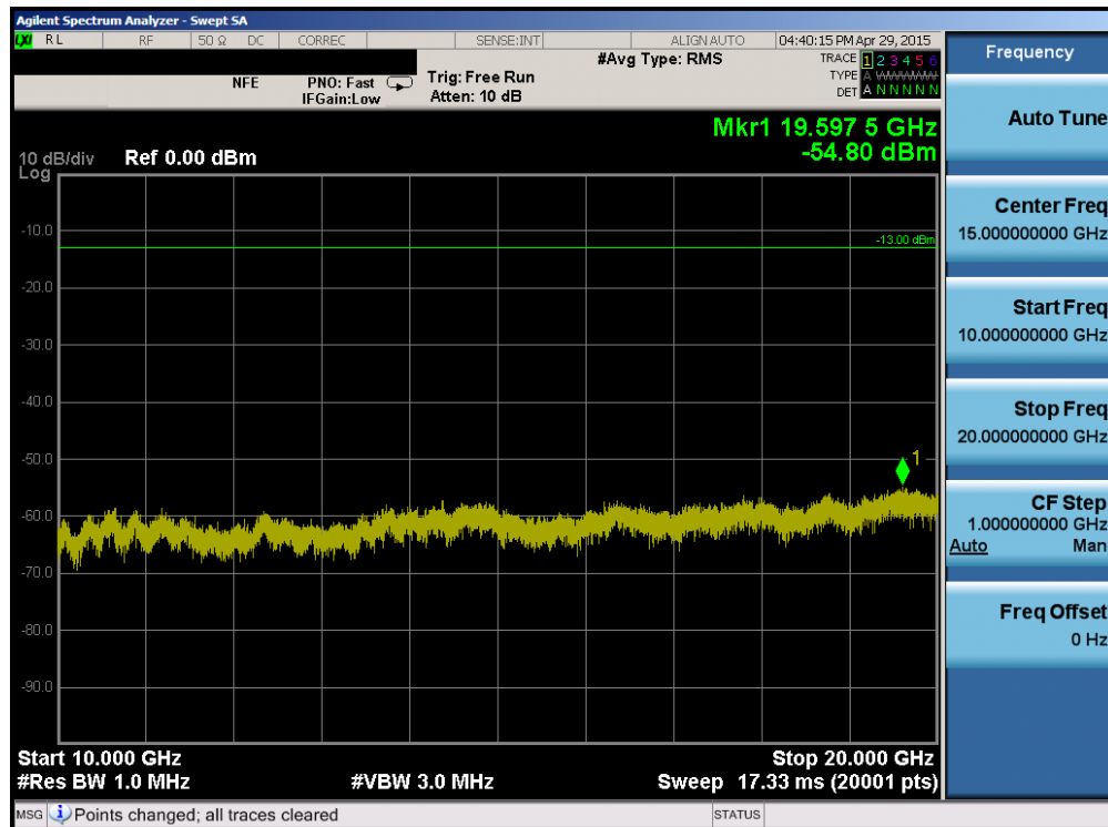
Plot 6-80. Conducted Spurious Plot (Band 4 – 20.0MHz QPSK – RB Size 1, RB Offset 0 – High Channel)
