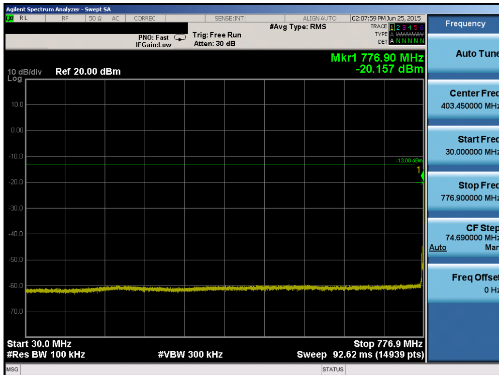
Plot 6-54. Conducted Spurious Plot (Band 13 – 5.0MHz QPSK – RB Size 1, RB Offset 0 – Low Channel)
