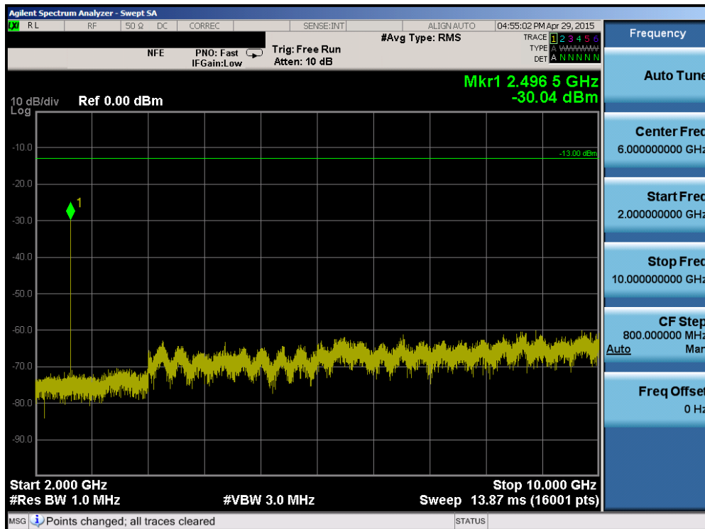
Plot 6-68. Conducted Spurious Plot (Band 5 – 10.0MHz QPSK – RB Size 1, RB Offset 0 – Mid Channel)
