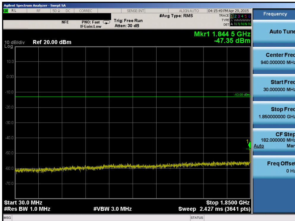
Plot 6-84. Conducted Spurious Plot (Band 2 – 20.0MHz QPSK – RB Size 1, RB Offset 0 – Mid Channel)
