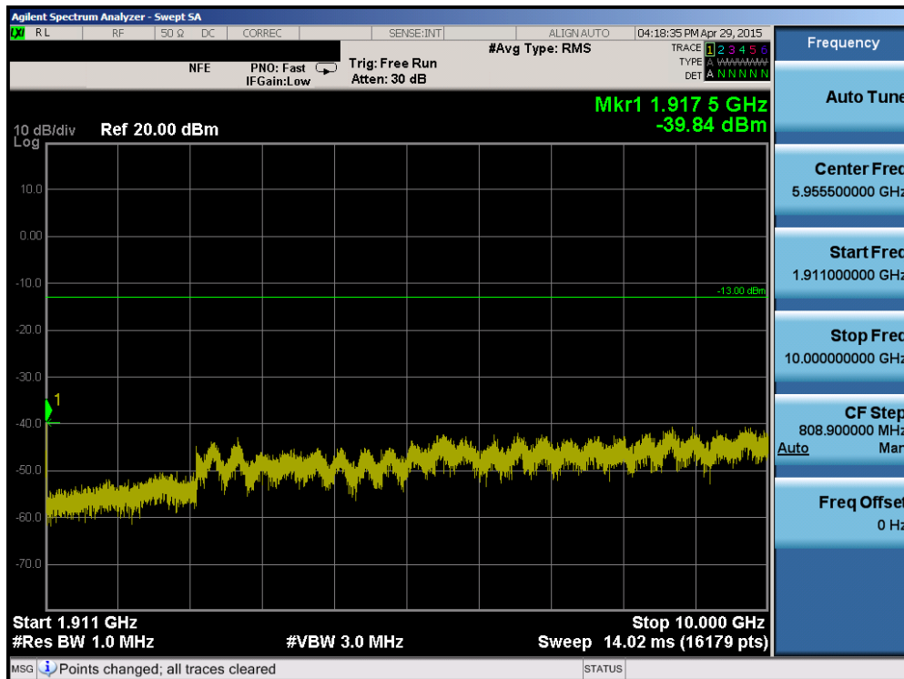
Plot 6-88. Conducted Spurious Plot (Band 2 – 20.0MHz QPSK – RB Size 1, RB Offset 0 – High Channel)
