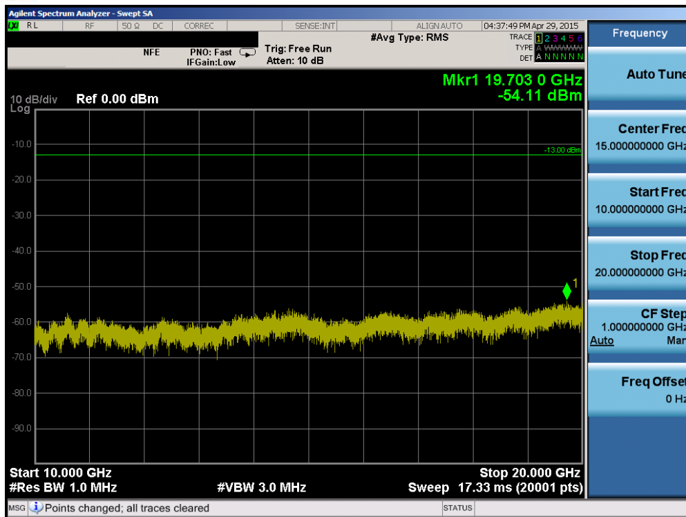
Plot 6-77. Conducted Spurious Plot (Band 4 – 20.0MHz QPSK – RB Size 1, RB Offset 0 – Mid Channel)
