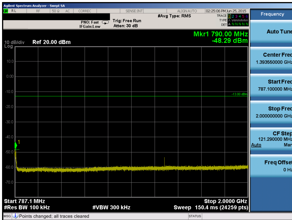
Plot 6-61. Conducted Spurious Plot (Band 13 – 5.0MHz QPSK – RB Size 1, RB Offset 0 – High Channel)
