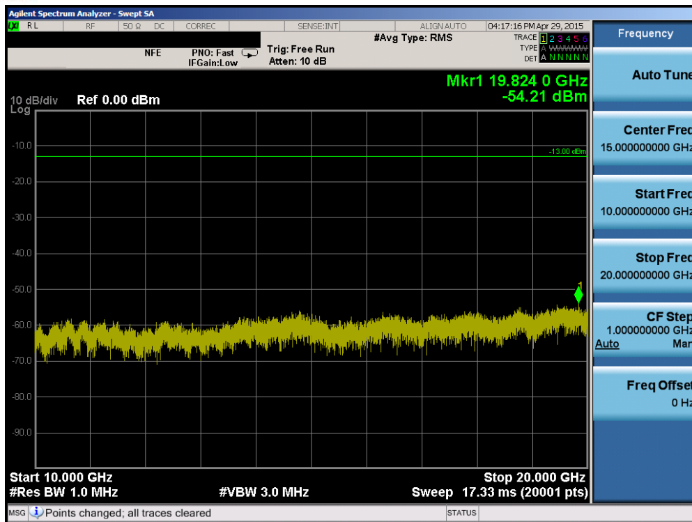
Plot 6-83. Conducted Spurious Plot (Band 2 – 20.0MHz QPSK – RB Size 1, RB Offset 0 – Low Channel)
