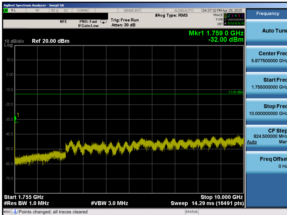
Plot 6-76. Conducted Spurious Plot (Band 4 – 20.0MHz QPSK – RB Size 1, RB Offset 0 – Mid Channel)
