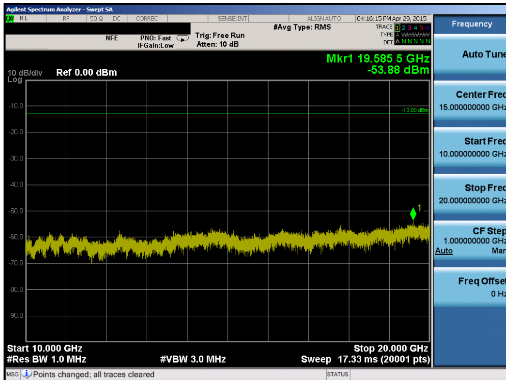
Plot 6-86. Conducted Spurious Plot (Band 2 – 20.0MHz QPSK – RB Size 1, RB Offset 0 – Mid Channel)
