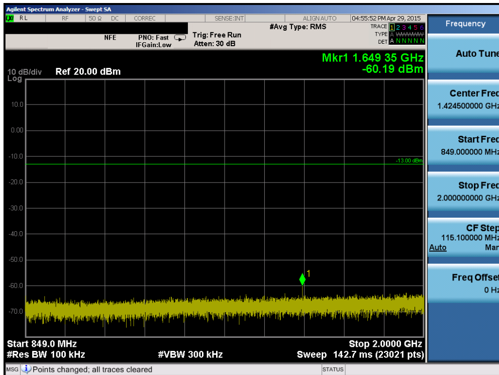
Plot 6-64. Conducted Spurious Plot (Band 5 – 10.0MHz QPSK – RB Size 1, RB Offset 0 – Low Channel)
