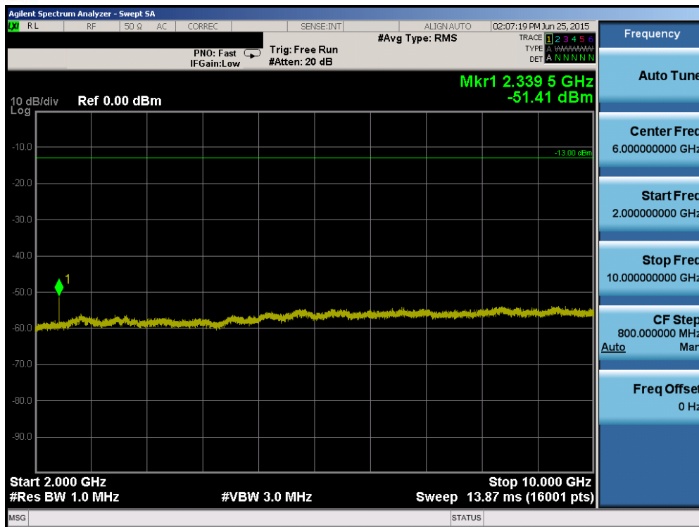
Plot 6-59. Conducted Spurious Plot (Band 13 – 5.0MHz QPSK – RB Size 1, RB Offset 0 – Mid Channel)
