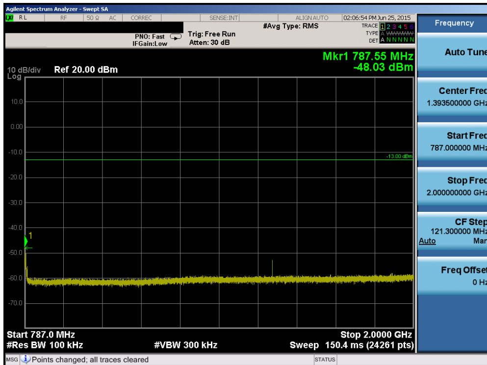
Plot 6-58. Conducted Spurious Plot (Band 13 – 5.0MHz QPSK – RB Size 1, RB Offset 0 – Mid Channel)
