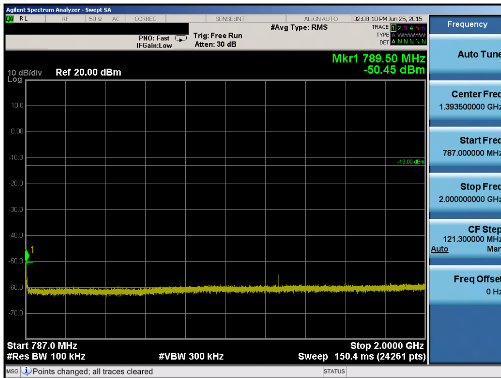
Plot 6-55. Conducted Spurious Plot (Band 13 – 5.0MHz QPSK – RB Size 1, RB Offset 0 – Low Channel)
