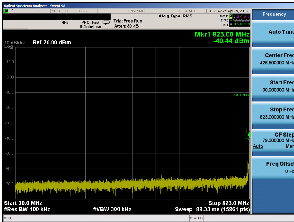
Plot 6-63. Conducted Spurious Plot (Band 5 – 10.0MHz QPSK – RB Size 1, RB Offset 0– Low Channel)
