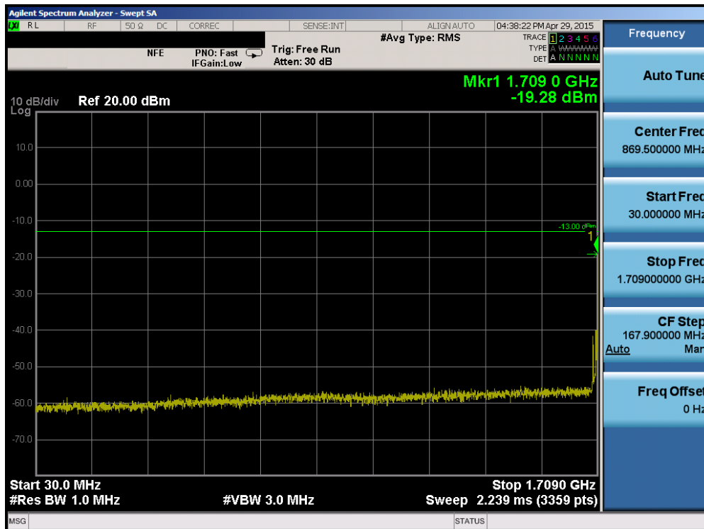
Plot 6-72. Conducted Spurious Plot (Band 4 – 20.0MHz QPSK – RB Size 1, RB Offset 0– Low Channel)
