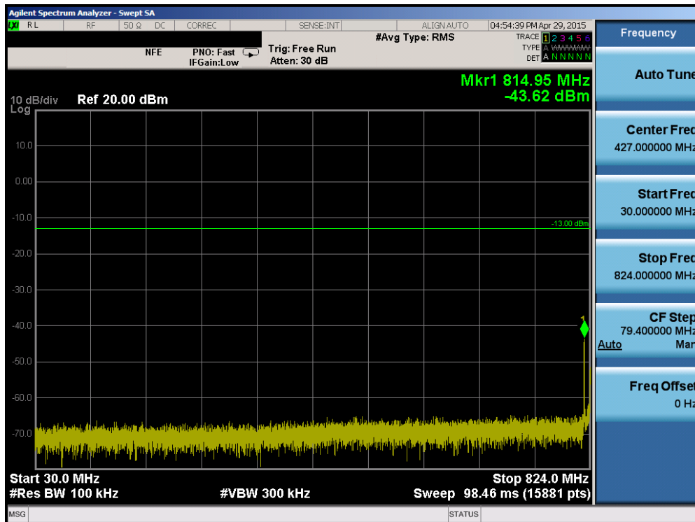
Plot 6-66. Conducted Spurious Plot (Band 5 – 10.0MHz QPSK – RB Size 1, RB Offset 0 – Mid Channel)
