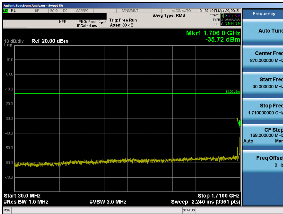
Plot 6-75. Conducted Spurious Plot (Band 4 – 20.0MHz QPSK – RB Size 1, RB Offset 0 – Mid Channel)
