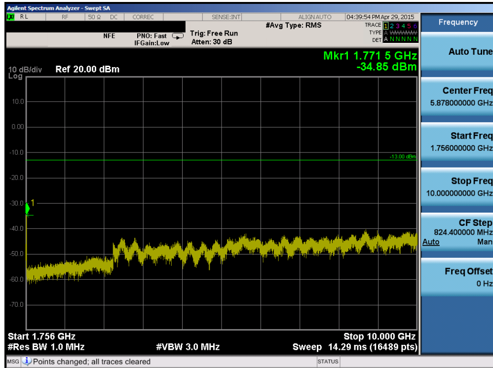
Plot 6-79. Conducted Spurious Plot (Band 4 – 20.0MHz QPSK – RB Size 1, RB Offset 0 – High Channel)
