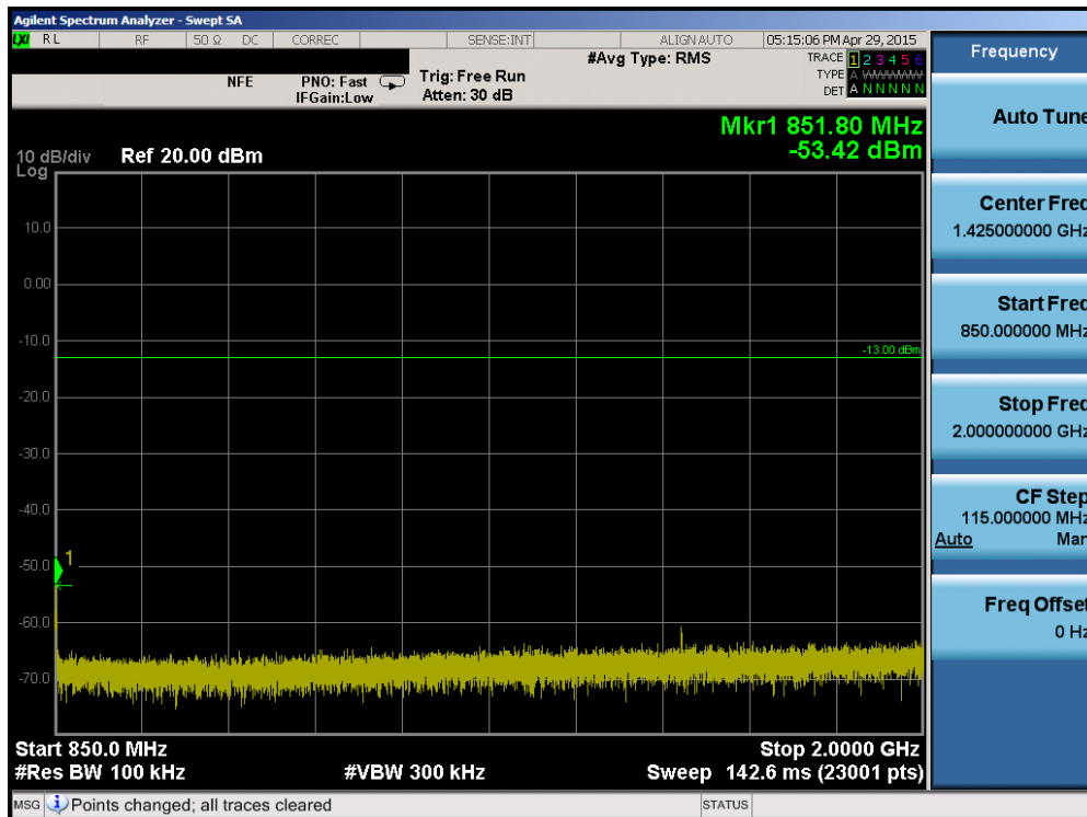
Plot 6-70. Conducted Spurious Plot (Band 5 – 10.0MHz QPSK – RB Size 1, RB Offset 0 – High Channel)
