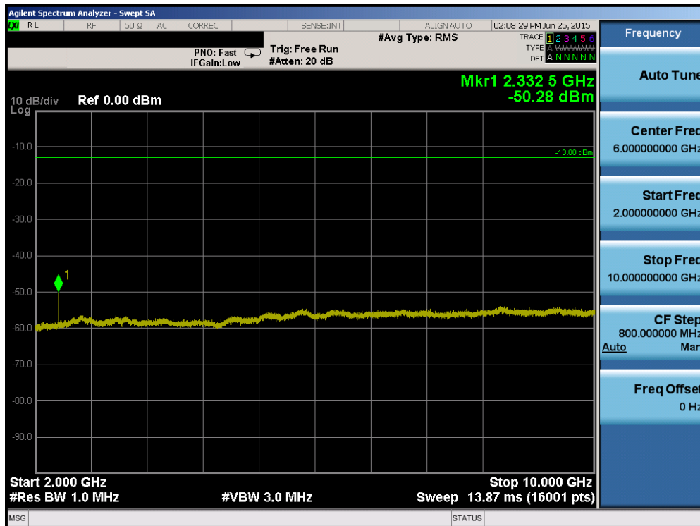
Plot 6-56. Conducted Spurious Plot (Band 13 – 5.0MHz QPSK – RB Size 1, RB Offset 0 – Low Channel)
