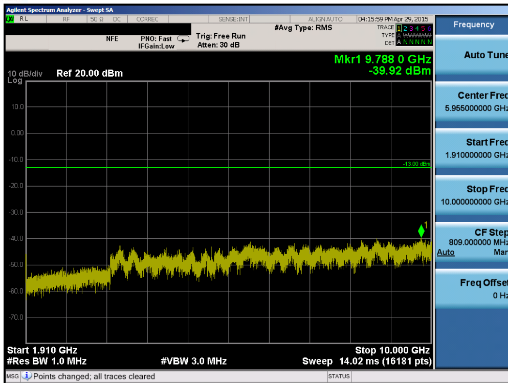
Plot 6-85. Conducted Spurious Plot (Band 2 – 20.0MHz QPSK – RB Size 1, RB Offset 0 – Mid Channel)
