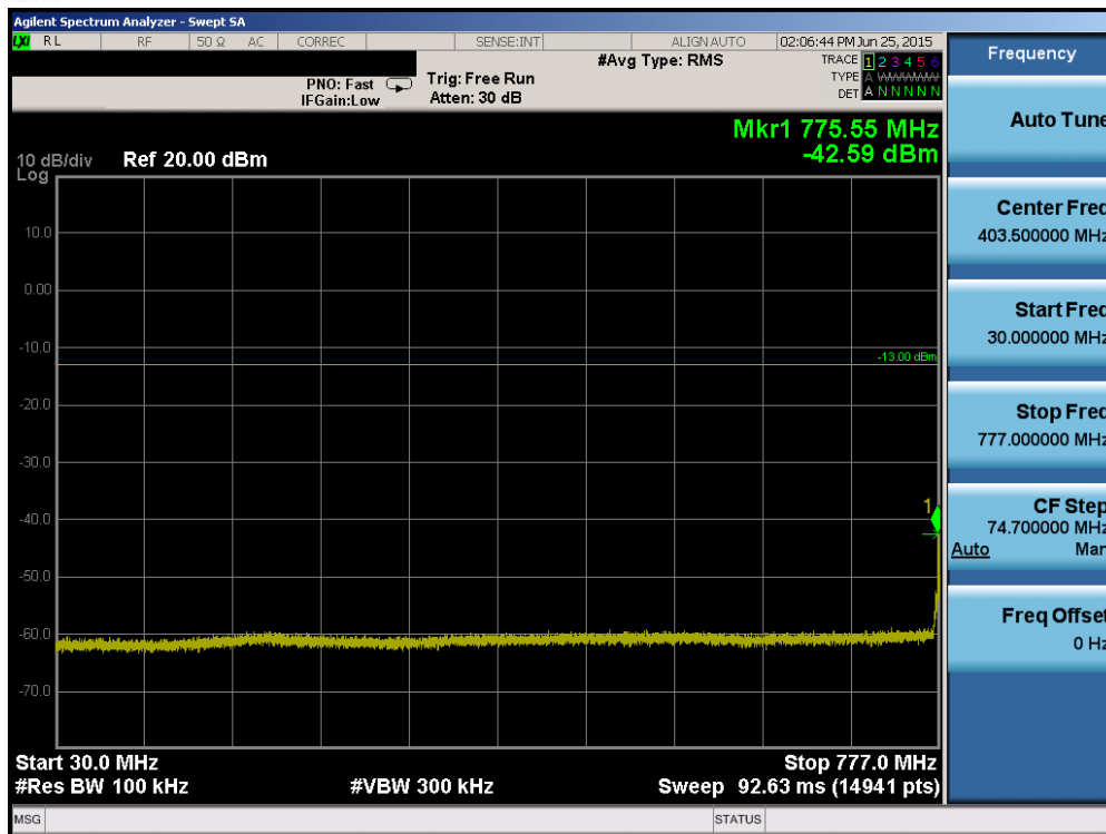
Plot 6-57. Conducted Spurious Plot (Band 13 – 5.0MHz QPSK – RB Size 1, RB Offset 0 – Mid Channel)
